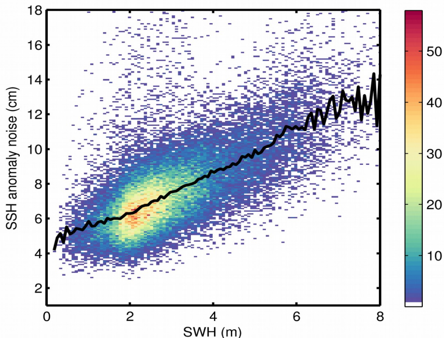
Figure 9. 2D histogram showing flag-valid SSH anomaly noise as a function of SWH for 22/12/2019. The black line denotes the median SSH anomaly noise as a function of SWH.
