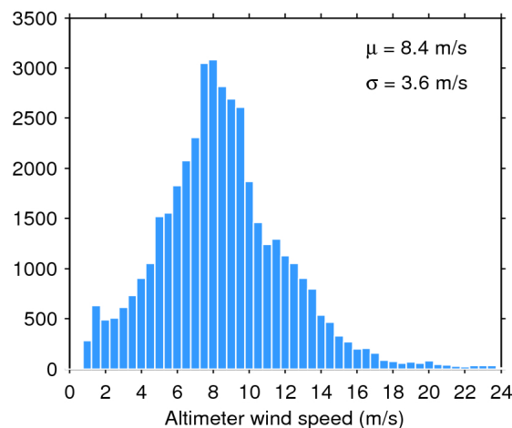
Figure 35. Histogram of science-valid wind over oceans and lakes for 22/12/2019. The mean ( \mu ) and standard deviation ( \sigma ) are also shown. Note that values larger than 24 m/s are excluded from the histogram for the sake of readability but not from the computation of \mu and \sigma .
