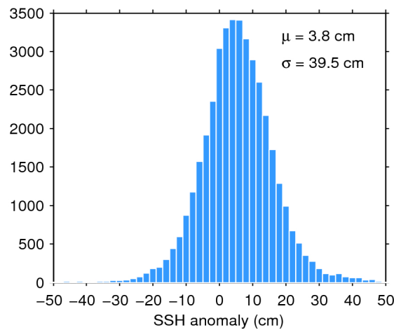
Figure 7. Histogram of flag-valid SSH anomaly over oceans and lakes for 22/12/2019. The mean ( \mu ) and standard deviation ( \sigma ) are also shown. Note that values outside [-50 50] cm are excluded from the histogram for the sake of readability but not from the computation of \mu and \sigma .
