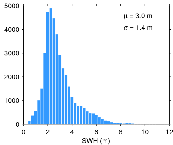
Figure 17. Histogram of flag-valid SWH over oceans and lakes for 22/12/2019. The mean ( \mu ) and standard deviation ( \sigma ) are also shown. Note that values larger than 12 m are excluded from the histogram for the sake of readability but not from the computation of \mu and \sigma .
