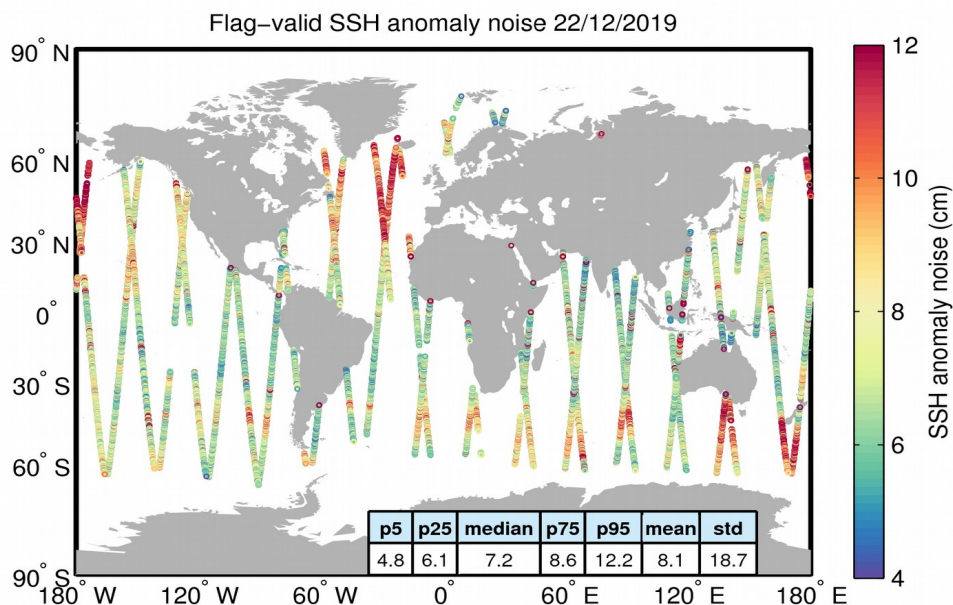
Figure 8. Geographical distribution of flag-valid 20-Hz SSH anomaly measurement noise over oceans and lakes for 22/12/2019. The statistical values shown in the table refer to the SSH anomaly noise and are calculated over all measurements shown in the figure.
