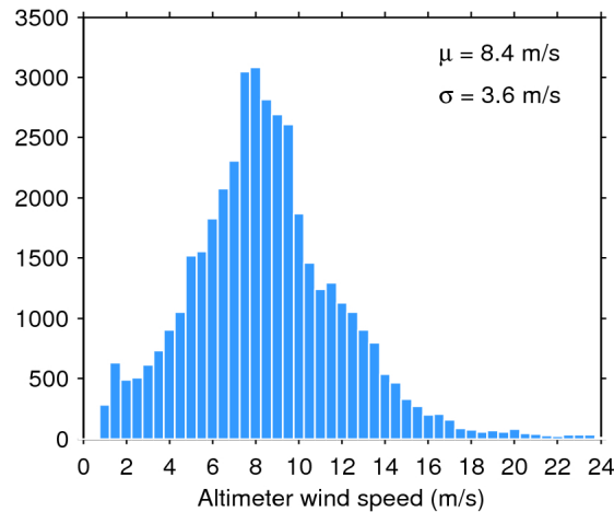
Figure 33. Histogram of flag-valid wind over oceans and lakes for 22/12/2019. The mean ( \mu ) and standard deviation ( \sigma ) are also shown. Note that values larger than 24 m/s are excluded from the histogram for the sake of readability but not from the computation of \mu and \sigma .
