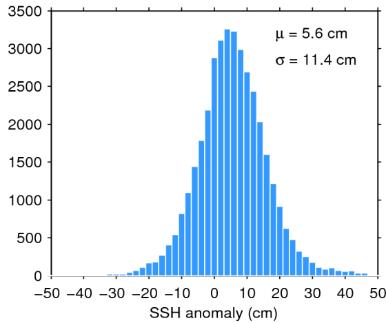
Figure 11. Histogram of science-valid SSH anomaly over oceans and lakes for 22/12/2019. The mean ( \mu ) and standard deviation ( \sigma ) are also shown. Note that values outside [-50 50] cm are excluded from the histogram for the sake of readability but not from the computation of \mu and \sigma .
