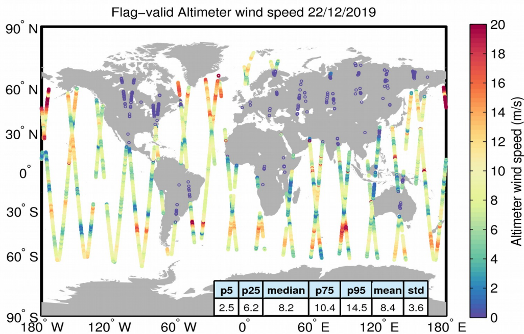
Figure 31. Geographical distribution of flag-valid wind data over oceans and lakes for 22/12/2019. The statistical values shown in the table refer to the wind in m/s and are calculated over all measurements shown in the figure.
