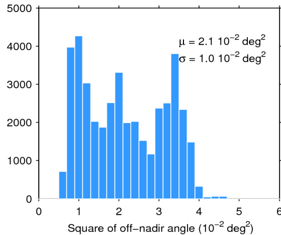
Figure 39. Histogram of flag-valid mispointing over oceans and lakes for 22/12/2019. The mean ( \mu ) and standard deviation ( \sigma ) are also shown. Note that values larger than 6 \cdot 10^{-2} \text{ deg}^2 are excluded from the histogram for the sake of readability but not from the computation of \mu and \sigma .
