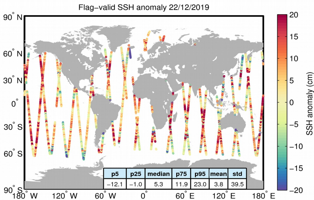
Figure 5. Geographical distribution of flag-valid 1-Hz SSH anomaly data over oceans and lakes for 22/12/2019. The statistical values shown in the table refer to the SSH anomaly in cm and are calculated over all measurements shown in the figure.
