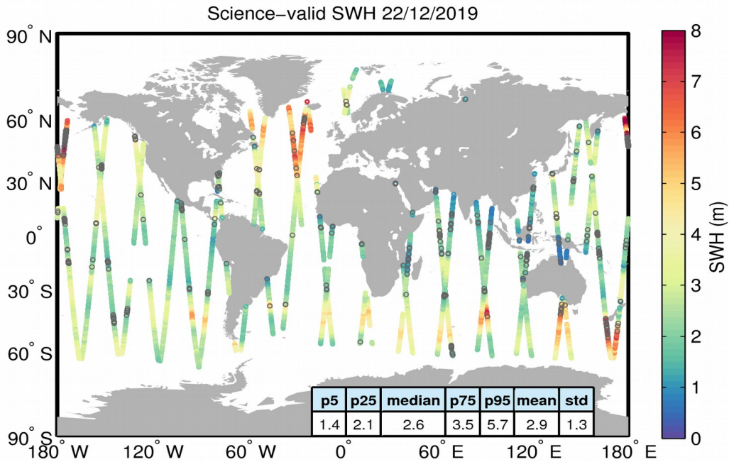
Figure 19. Geographical distribution of science-valid SWH data over oceans and lakes for 22/12/2019. The statistical values shown in the table refer to the SWH in m and are calculated over all measurements shown in the figure. Gray circles denote records that have been rejected based on the editing criteria described in Table 3.
