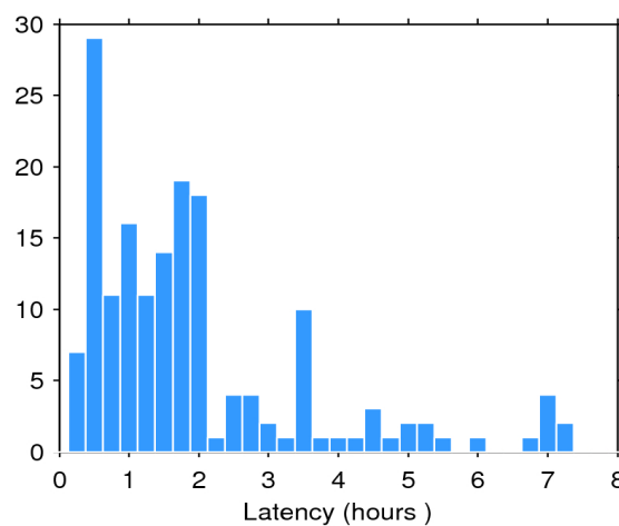
Figure 2. Histogram of the data latency for 22/12/2019. The y-axis denotes the number of files that are made available with a delay of x-hours with respect to the mean time of the records stored in the file.
