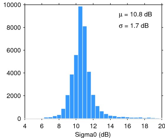
Figure 25. Histogram of flag-valid sigma0 over oceans and lakes for 22/12/2019. The mean ( \mu ) and standard deviation ( \sigma ) are also shown. Note that values outside [4 20] dB are excluded from the histogram for the sake of readability but not from the computation of \mu and \sigma .
