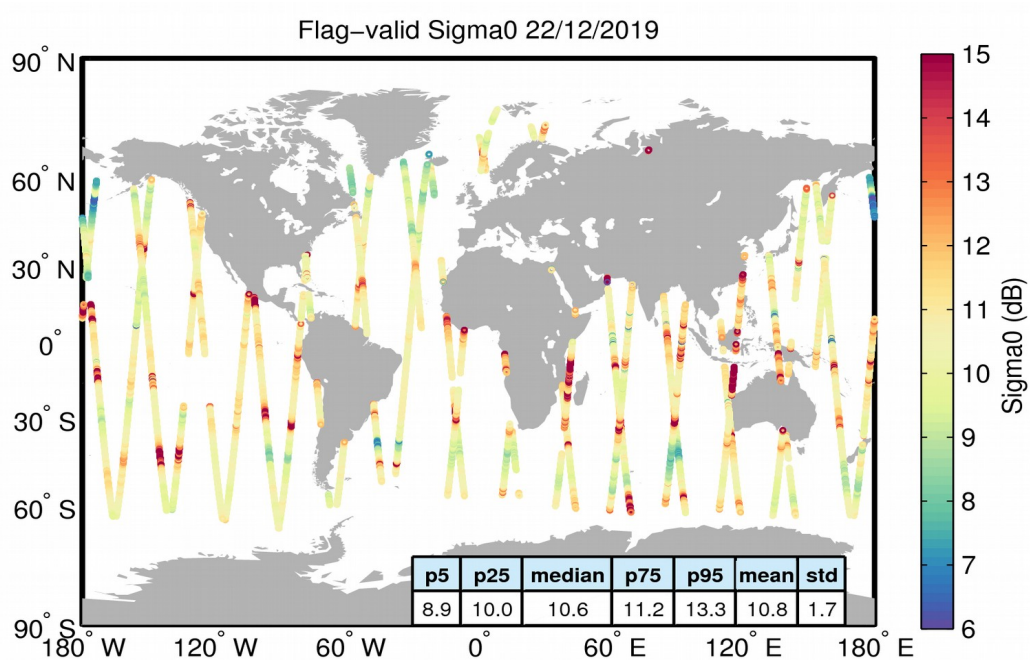
Figure 23. Geographical distribution of flag-valid sigma0 data over oceans and lakes for 22/12/2019. The statistical values shown in the table refer to the sigma0 in dB and are calculated over all measurements shown in the figure.
