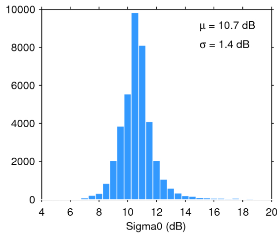
Figure 28. Histogram of science-valid sigma0 over oceans and lakes for 22/12/2019. The mean ( \mu ) and standard deviation ( \sigma ) are also shown. Note that values outside [4 20] dB are excluded from the histogram for the sake of readability but not from the computation of \mu and \sigma .
