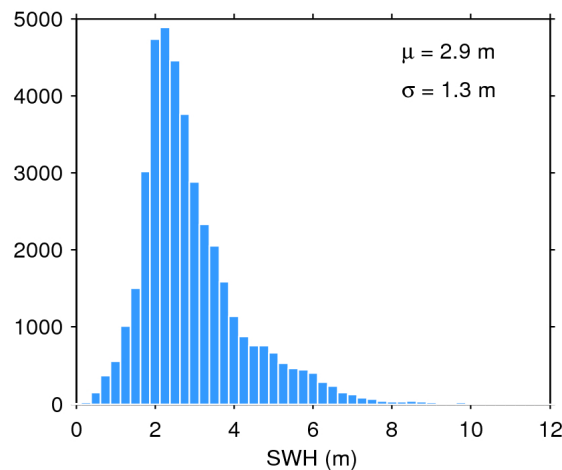
Figure 20. Histogram of science-valid SWH over oceans and lakes for 22/12/2019. The mean ( \mu ) and standard deviation ( \sigma ) are also shown. Note that values larger than 12 m are excluded from the histogram for the sake of readability but not from the computation of \mu and \sigma .
