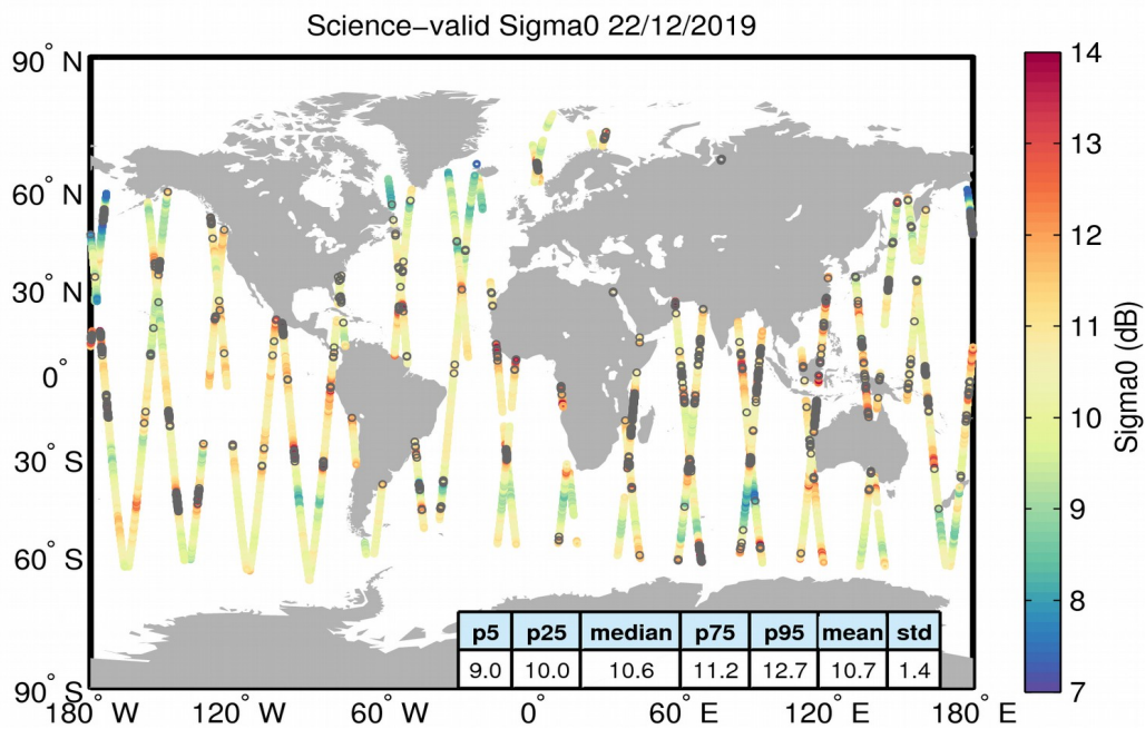
Figure 27. Geographical distribution of science-valid sigma0 data over oceans and lakes for 22/12/2019. The statistical values shown in the table refer to the sigma0 in dB and are calculated over all measurements shown in the figure. Gray circles denote records that have been rejected based on the editing criteria described in Table 4.
