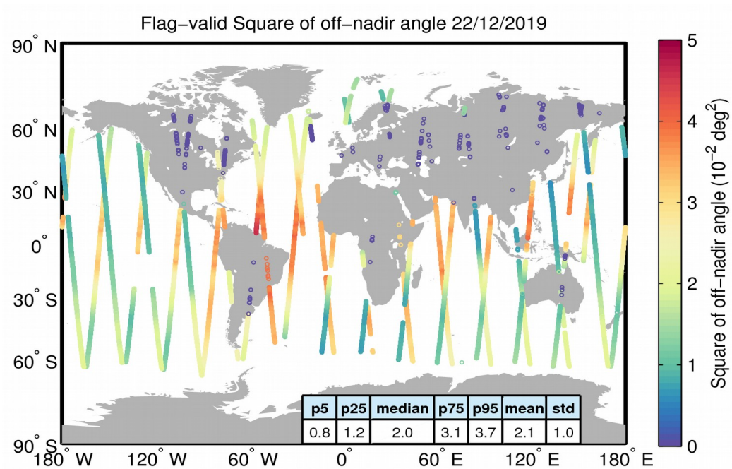
Figure 37. Geographical distribution of flag-valid mispointing data over oceans and lakes for 22/12/2019. The statistical values shown in the table refer to the mispointing in 10^{-2} deg 2 and are calculated over all measurements shown in the figure.
