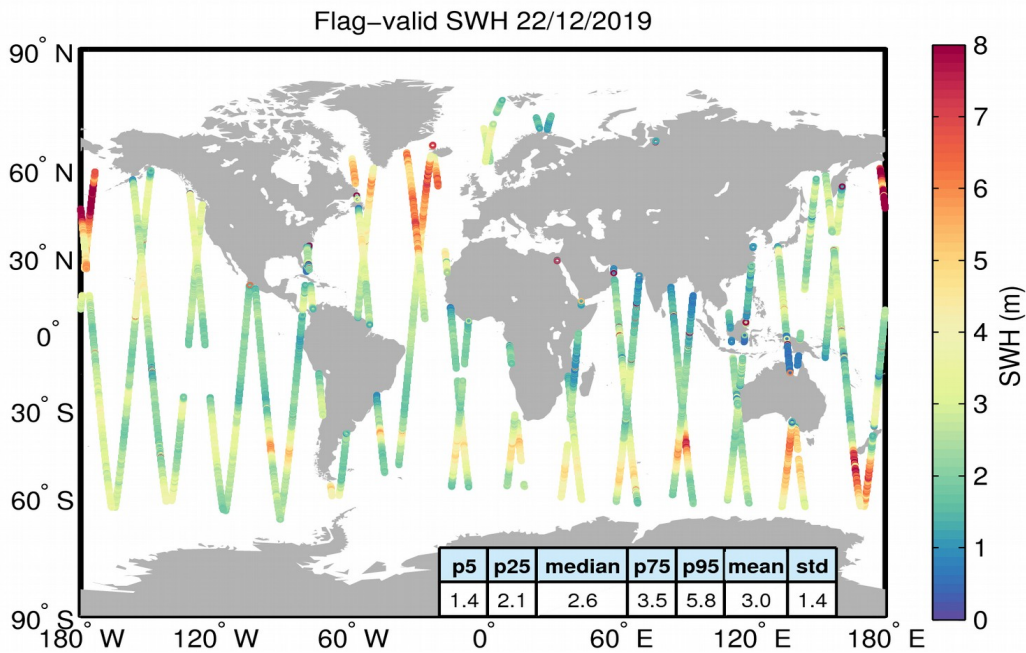
Figure 15. Geographical distribution of flag-valid SWH data over oceans and lakes for 22/12/2019. The statistical values shown in the table refer to the SWH in m and are calculated over all measurements shown in the figure.
