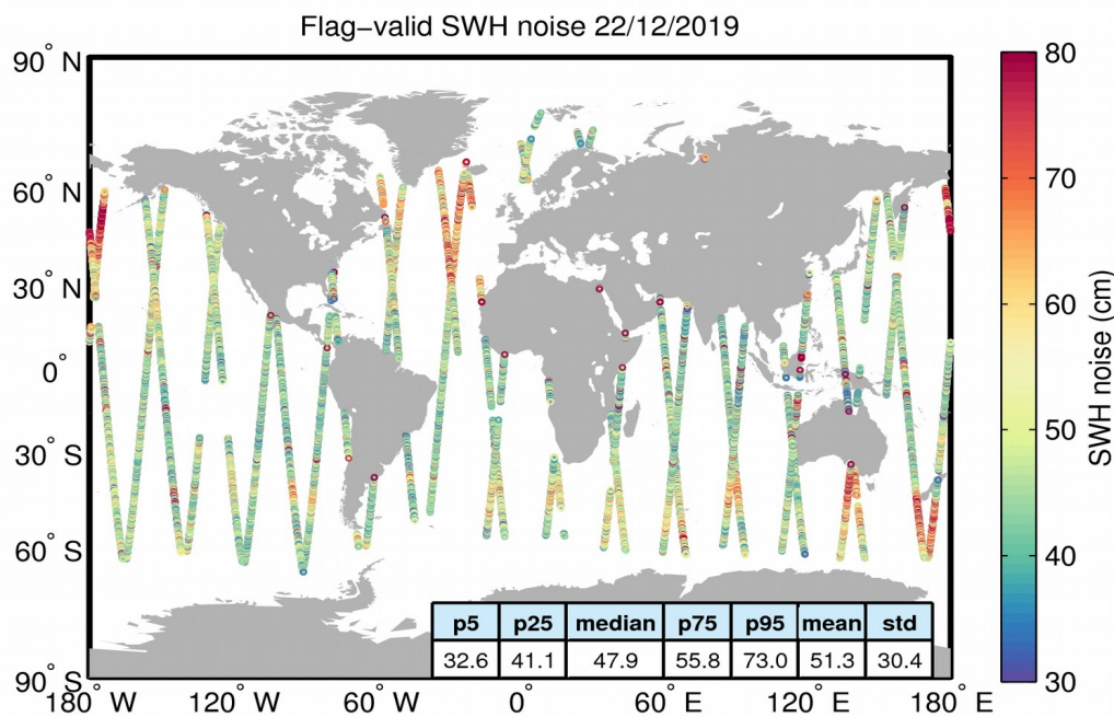
Figure 18. Geographical distribution of flag-valid 20-Hz SWH measurement noise over oceans and lakes for 22/12/2019. The statistical values shown in the figure refer to the SWH noise and are calculated over all measurements shown in the figure.
