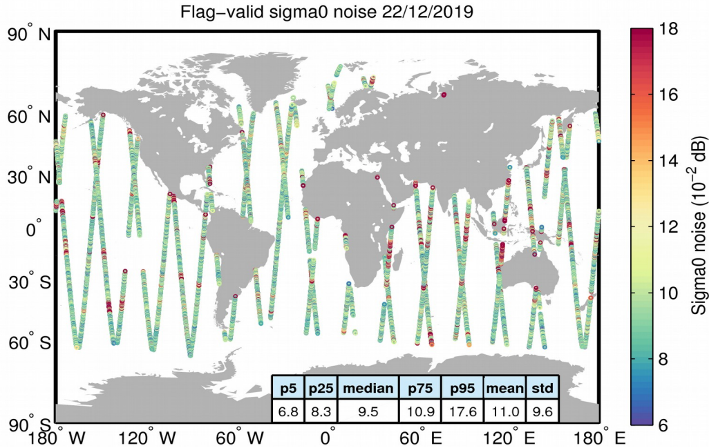
Figure 26. Geographical distribution of flag-valid 20-Hz sigma0 measurement noise over oceans and lakes for 22/12/2019. The statistical values shown in the table refer to the sigma0 noise and are calculated over all measurements shown in the figure.
