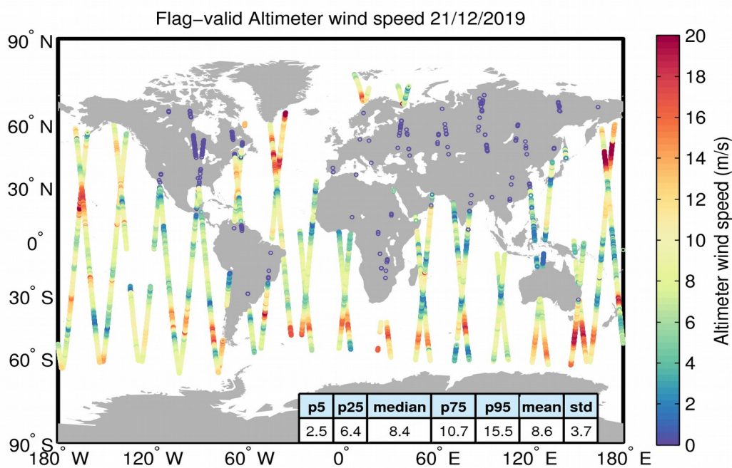
Figure 31. Geographical distribution of flag-valid wind data over oceans and lakes for 21/12/2019. The statistical values shown in the table refer to the wind in m/s and are calculated over all measurements shown in the figure.
