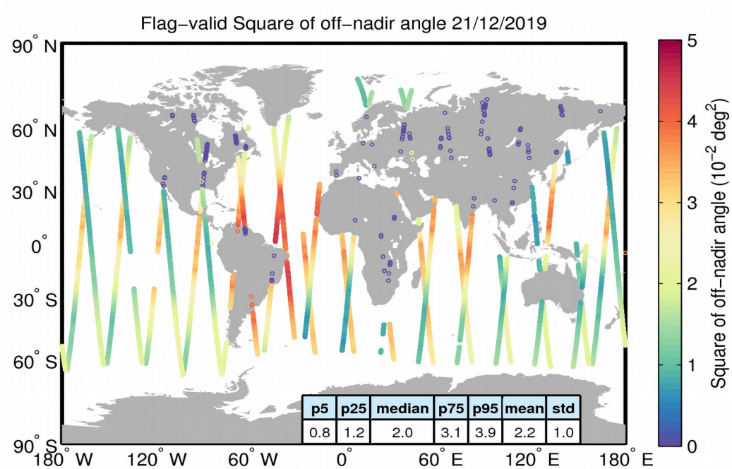
Figure 37. Geographical distribution of flag-valid mispointing data over oceans and lakes for 21/12/2019. The statistical values shown in the table refer to the mispointing in 10^{-2} \text{ deg}^2 and are calculated over all measurements shown in the figure.
