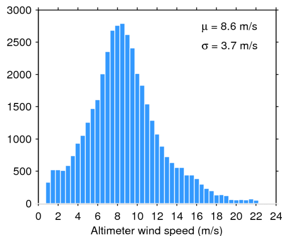
Figure 35. Histogram of science-valid wind over oceans and lakes for 21/12/2019. The mean ( \mu ) and standard deviation ( \sigma ) are also shown. Note that values larger than 24 m/s are excluded from the histogram for the sake of readability but not from the computation of \mu and \sigma .
