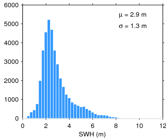
Figure 20. Histogram of science-valid SWH over oceans and lakes for 21/12/2019. The mean ( \mu ) and standard deviation ( \sigma ) are also shown. Note that values larger than 12 m are excluded from the histogram for the sake of readability but not from the computation of \mu and \sigma .
