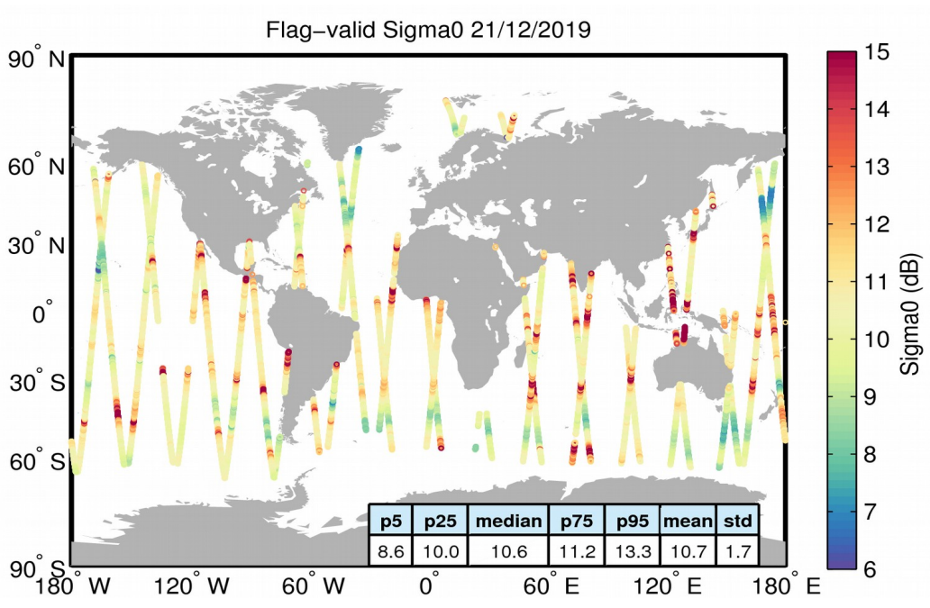
Figure 23. Geographical distribution of flag-valid sigma0 data over oceans and lakes for 21/12/2019. The statistical values shown in the table refer to the sigma0 in dB and are calculated over all measurements shown in the figure.
