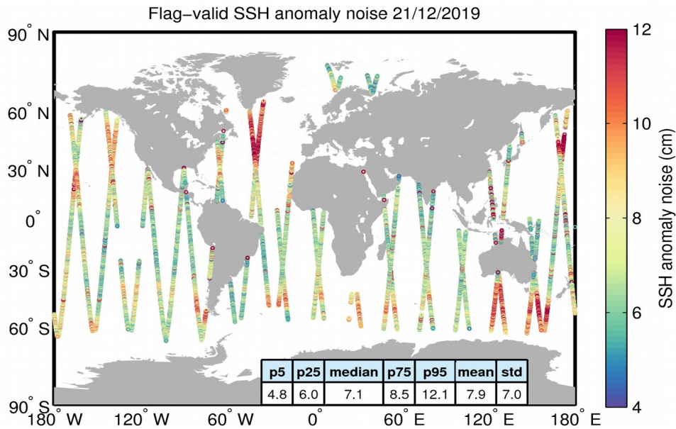
Figure 8. Geographical distribution of flag-valid 20-Hz SSH anomaly measurement noise over oceans and lakes for 21/12/2019. The statistical values shown in the table refer to the SSH anomaly noise and are calculated over all measurements shown in the figure.
