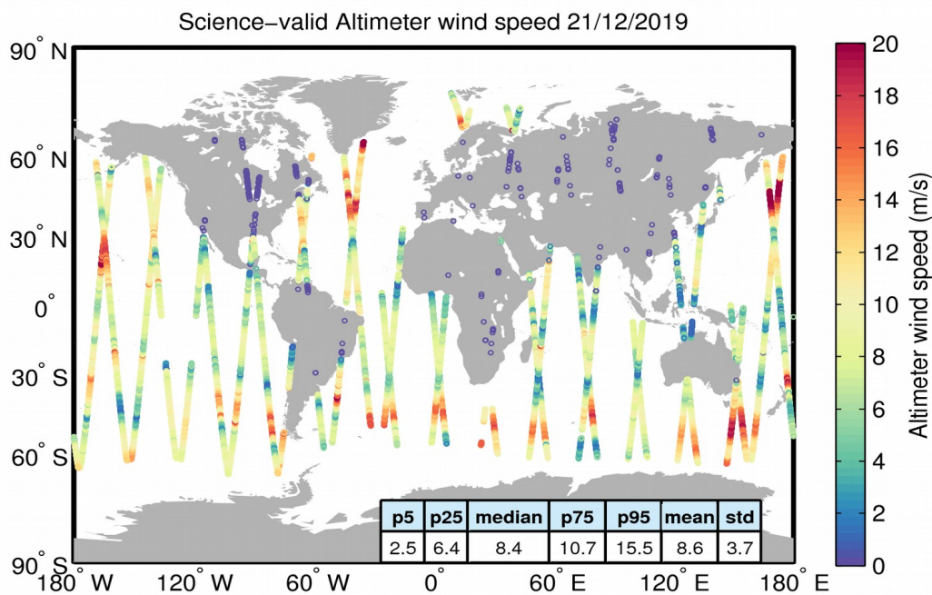
Figure 34. Geographical distribution of science-valid wind data over oceans and lakes for 21/12/2019. The statistical values shown in the table refer to the wind in m/s and are calculated over all measurements shown in the figure. Gray circles denote records that have been rejected based on the editing criteria described in Table 5.
