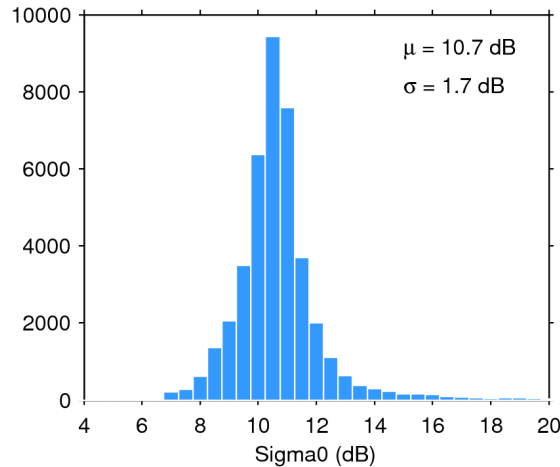
Figure 25. Histogram of flag-valid sigma0 over oceans and lakes for 21/12/2019. The mean ( \mu ) and standard deviation ( \sigma ) are also shown. Note that values outside [4 20] dB are excluded from the histogram for the sake of readability but not from the computation of \mu and \sigma .
