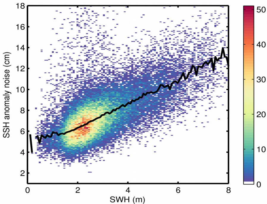
Figure 9. 2D histogram showing flag-valid SSH anomaly noise as a function of SWH for 21/12/2019. The black line denotes the median SSH anomaly noise as a function of SWH.
