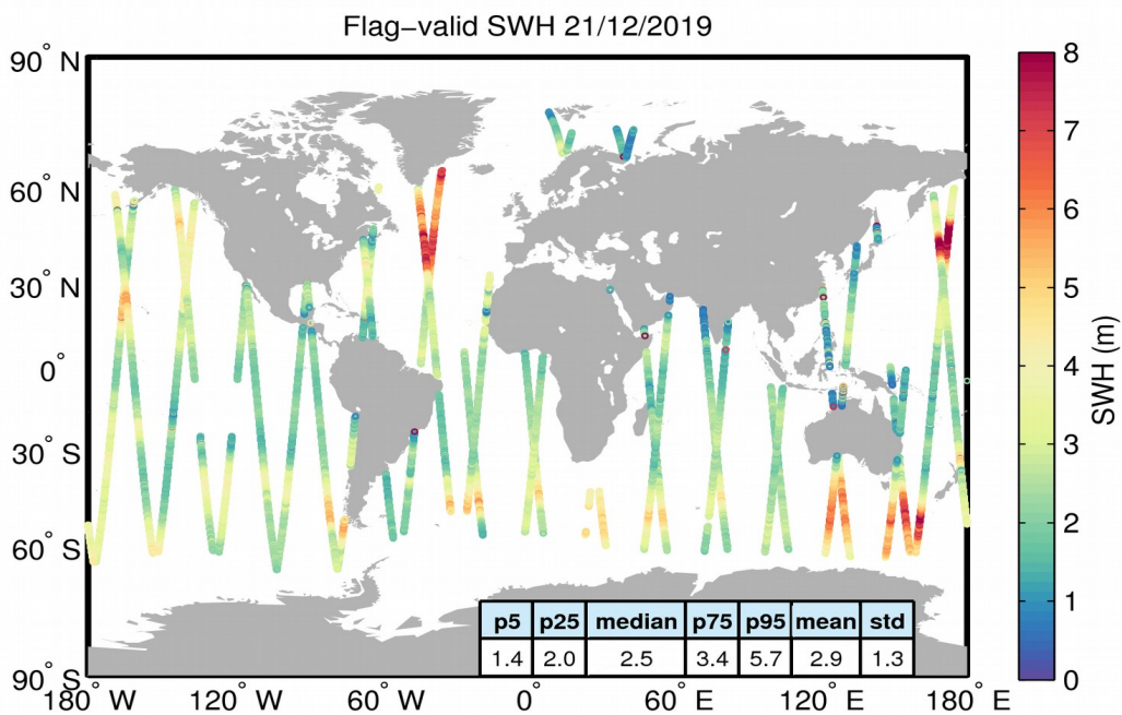
Figure 15. Geographical distribution of flag-valid SWH data over oceans and lakes for 21/12/2019. The statistical values shown in the table refer to the SWH in m and are calculated over all measurements shown in the figure.
