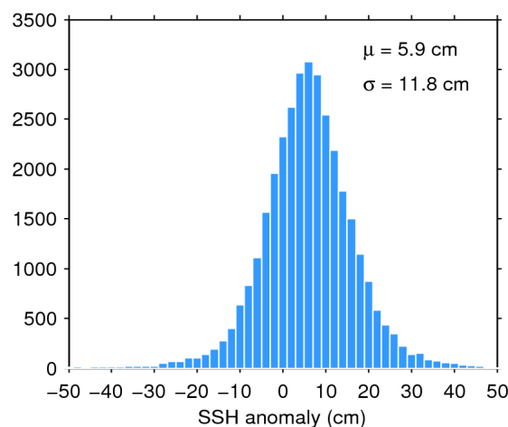
Figure 11. Histogram of science-valid SSH anomaly over oceans and lakes for 21/12/2019. The mean ( \mu ) and standard deviation ( \sigma ) are also shown. Note that values outside [-50 50] cm are excluded from the histogram for the sake of readability but not from the computation of \mu and \sigma .
