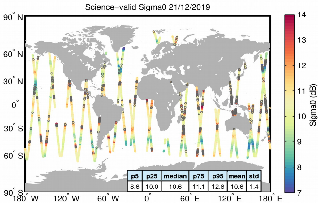
Figure 27. Geographical distribution of science-valid sigma0 data over oceans and lakes for 21/12/2019. The statistical values shown in the table refer to the sigma0 in dB and are calculated over all measurements shown in the figure. Gray circles denote records that have been rejected based on the editing criteria described in Table 4.
