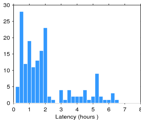
Figure 2. Histogram of the data latency for 21/12/2019. The y-axis denotes the number of files that are made available with a delay of x-hours with respect to the mean time of the records stored in the file.
