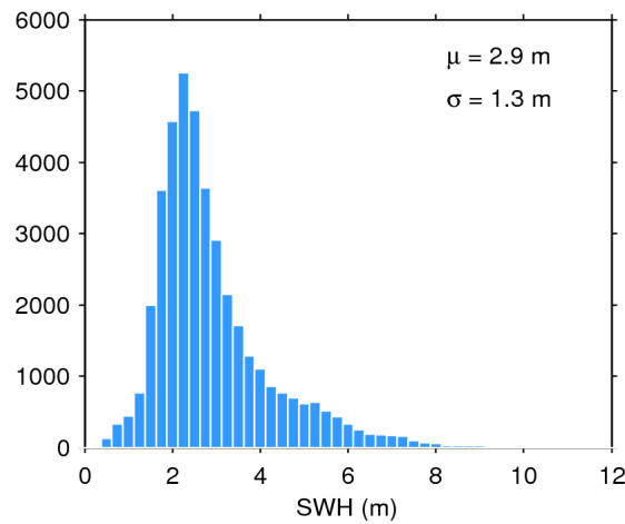
Figure 17. Histogram of flag-valid SWH over oceans and lakes for 21/12/2019. The mean ( \mu ) and standard deviation ( \sigma ) are also shown. Note that values larger than 12 m are excluded from the histogram for the sake of readability but not from the computation of \mu and \sigma .
