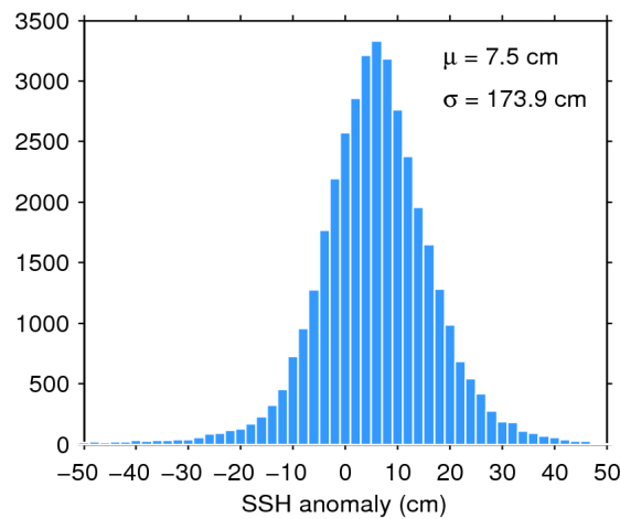
Figure 7. Histogram of flag-valid SSH anomaly over oceans and lakes for 21/12/2019. The mean ( \mu ) and standard deviation ( \sigma ) are also shown. Note that values outside [-50 50] cm are excluded from the histogram for the sake of readability but not from the computation of \mu and \sigma .
