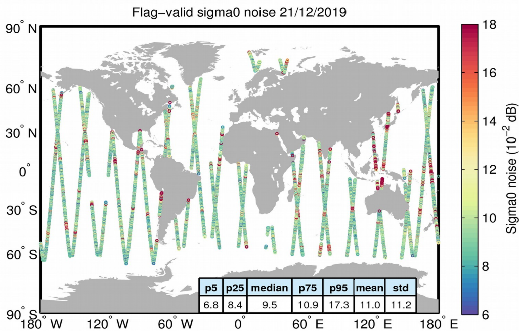
Figure 26. Geographical distribution of flag-valid 20-Hz sigma0 measurement noise over oceans and lakes for 21/12/2019. The statistical values shown in the table refer to the sigma0 noise and are calculated over all measurements shown in the figure.
