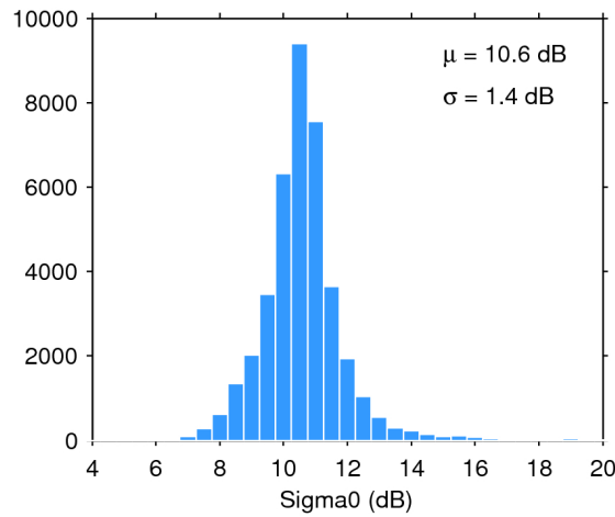
Figure 28. Histogram of science-valid sigma0 over oceans and lakes for 21/12/2019. The mean ( \mu ) and standard deviation ( \sigma ) are also shown. Note that values outside [4 20] dB are excluded from the histogram for the sake of readability but not from the computation of \mu and \sigma .
