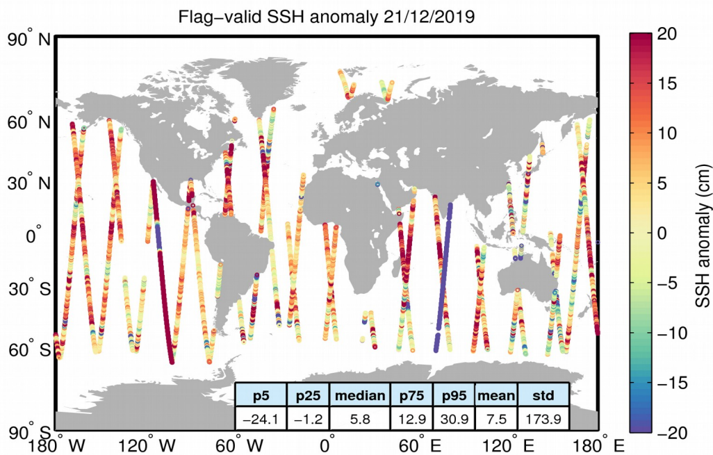
Figure 5. Geographical distribution of flag-valid 1-Hz SSH anomaly data over oceans and lakes for 21/12/2019. The statistical values shown in the table refer to the SSH anomaly in cm and are calculated over all measurements shown in the figure.
