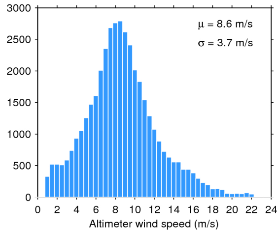
Figure 33. Histogram of flag-valid wind over oceans and lakes for 21/12/2019. The mean ( \mu ) and standard deviation ( \sigma ) are also shown. Note that values larger than 24 m/s are excluded from the histogram for the sake of readability but not from the computation of \mu and \sigma .
