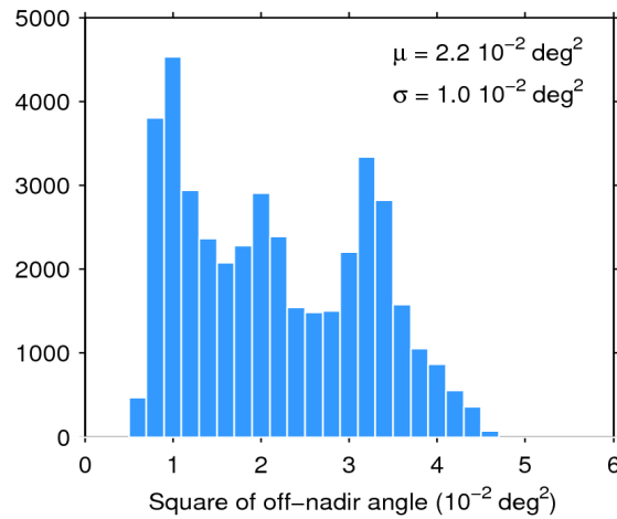
Figure 39. Histogram of flag-valid mispointing over oceans and lakes for 21/12/2019. The mean ( \mu ) and standard deviation ( \sigma ) are also shown. Note that values larger than 6 \cdot 10^{-2} \text{ deg}^2 are excluded from the histogram for the sake of readability but not from the computation of \mu and \sigma .
