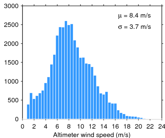
Figure 35. Histogram of science-valid wind over oceans and lakes for 19/12/2019. The mean ( \mu ) and standard deviation ( \sigma ) are also shown. Note that values larger than 24 m/s are excluded from the histogram for the sake of readability but not from the computation of \mu and \sigma .
