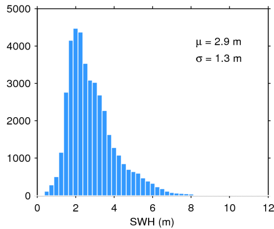
Figure 17. Histogram of flag-valid SWH over oceans and lakes for 19/12/2019. The mean ( \mu ) and standard deviation ( \sigma ) are also shown. Note that values larger than 12 m are excluded from the histogram for the sake of readability but not from the computation of \mu and \sigma .
