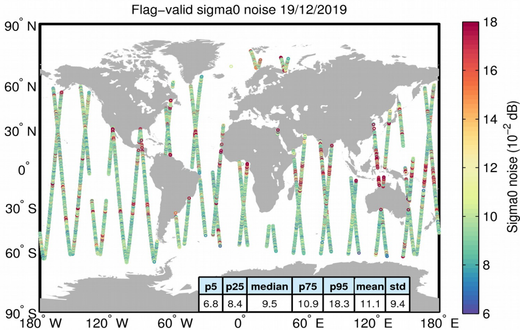
Figure 26. Geographical distribution of flag-valid 20-Hz sigma0 measurement noise over oceans and lakes for 19/12/2019. The statistical values shown in the table refer to the sigma0 noise and are calculated over all measurements shown in the figure.
