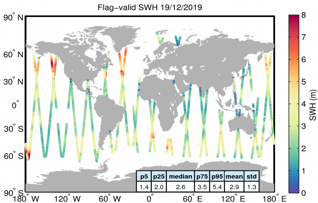
Figure 15. Geographical distribution of flag-valid SWH data over oceans and lakes for 19/12/2019. The statistical values shown in the table refer to the SWH in m and are calculated over all measurements shown in the figure.
