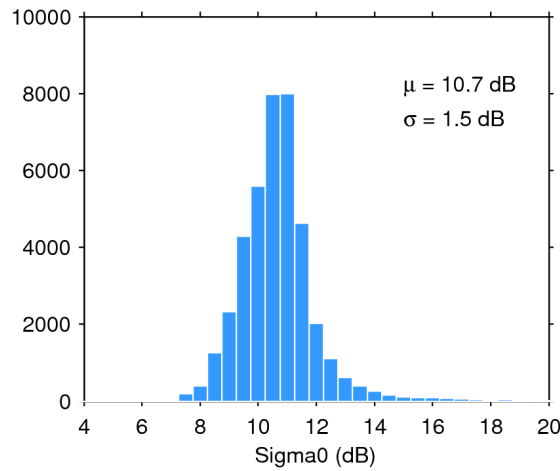
Figure 28. Histogram of science-valid sigma0 over oceans and lakes for 19/12/2019. The mean ( \mu ) and standard deviation ( \sigma ) are also shown. Note that values outside [4 20] dB are excluded from the histogram for the sake of readability but not from the computation of \mu and \sigma .
