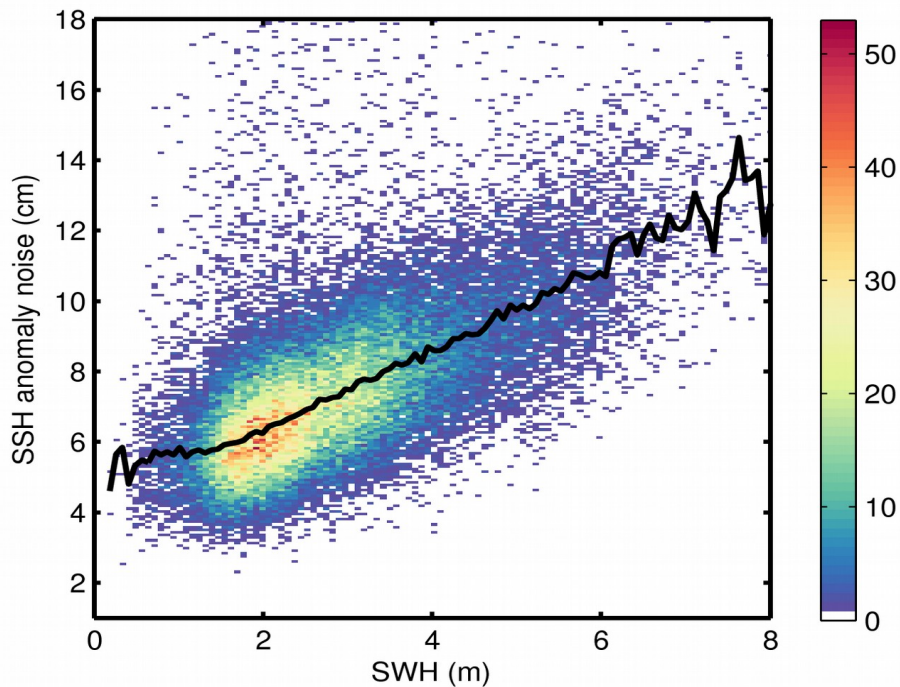
Figure 9. 2D histogram showing flag-valid SSH anomaly noise as a function of SWH for 19/12/2019. The black line denotes the median SSH anomaly noise as a function of SWH.
