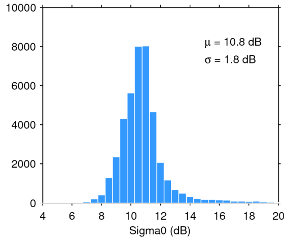
Figure 25. Histogram of flag-valid sigma0 over oceans and lakes for 19/12/2019. The mean ( \mu ) and standard deviation ( \sigma ) are also shown. Note that values outside [4 20] dB are excluded from the histogram for the sake of readability but not from the computation of \mu and \sigma .
