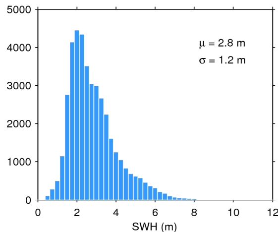
Figure 20. Histogram of science-valid SWH over oceans and lakes for 19/12/2019. The mean ( \mu ) and standard deviation ( \sigma ) are also shown. Note that values larger than 12 m are excluded from the histogram for the sake of readability but not from the computation of \mu and \sigma .
