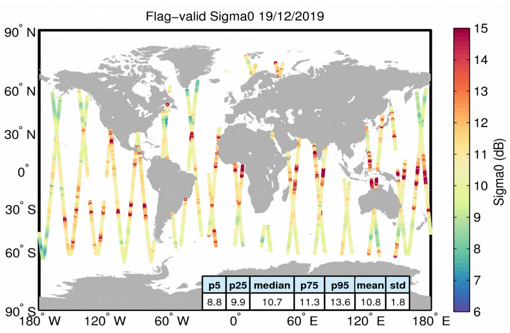
Figure 23. Geographical distribution of flag-valid sigma0 data over oceans and lakes for 19/12/2019. The statistical values shown in the table refer to the sigma0 in dB and are calculated over all measurements shown in the figure.
