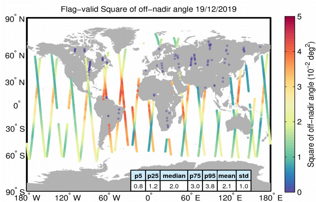
Figure 37. Geographical distribution of flag-valid mispointing data over oceans and lakes for 19/12/2019. The statistical values shown in the table refer to the mispointing in 10^{-2} deg 2 and are calculated over all measurements shown in the figure.
