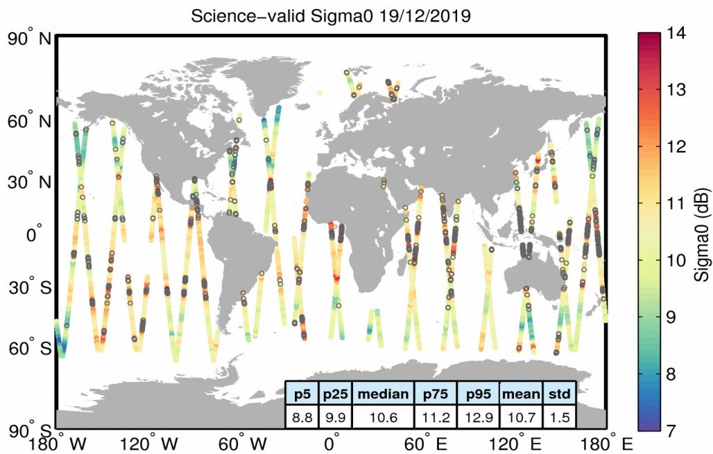
Figure 27. Geographical distribution of science-valid sigma0 data over oceans and lakes for 19/12/2019. The statistical values shown in the table refer to the sigma0 in dB and are calculated over all measurements shown in the figure. Gray circles denote records that have been rejected based on the editing criteria described in Table 4.
