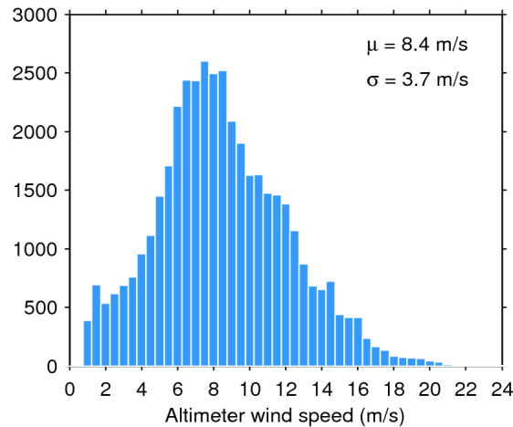
Figure 33. Histogram of flag-valid wind over oceans and lakes for 19/12/2019. The mean ( \mu ) and standard deviation ( \sigma ) are also shown. Note that values larger than 24 m/s are excluded from the histogram for the sake of readability but not from the computation of \mu and \sigma .
