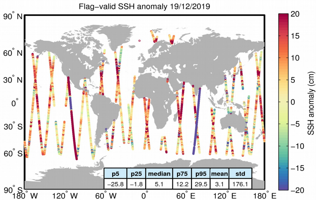
Figure 5. Geographical distribution of flag-valid 1-Hz SSH anomaly data over oceans and lakes for 19/12/2019. The statistical values shown in the table refer to the SSH anomaly in cm and are calculated over all measurements shown in the figure.
