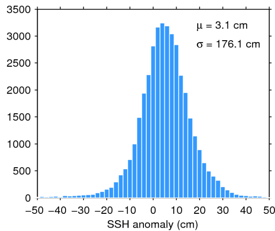
Figure 7. Histogram of flag-valid SSH anomaly over oceans and lakes for 19/12/2019. The mean ( \mu ) and standard deviation ( \sigma ) are also shown. Note that values outside [-50\ 50] cm are excluded from the histogram for the sake of readability but not from the computation of \mu and \sigma .
