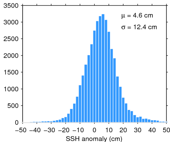
Figure 11. Histogram of science-valid SSH anomaly over oceans and lakes for 18/12/2019. The mean ( \mu ) and standard deviation ( \sigma ) are also shown. Note that values outside [-50 \text{ } 50] cm are excluded from the histogram for the sake of readability but not from the computation of \mu and \sigma .
