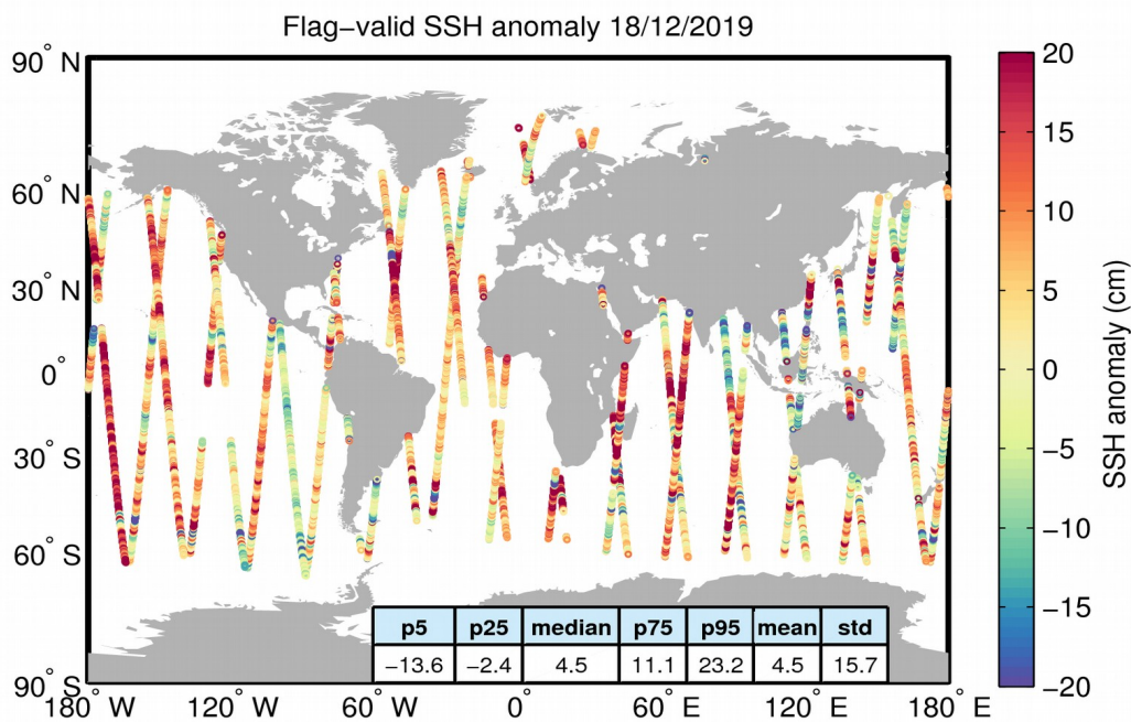
Figure 5. Geographical distribution of flag-valid 1-Hz SSH anomaly data over oceans and lakes for 18/12/2019. The statistical values shown in the table refer to the SSH anomaly in cm and are calculated over all measurements shown in the figure.
