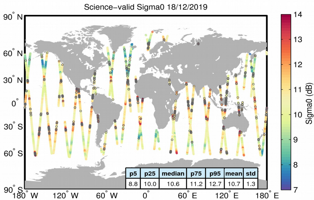
Figure 27. Geographical distribution of science-valid sigma0 data over oceans and lakes for 18/12/2019. The statistical values shown in the table refer to the sigma0 in dB and are calculated over all measurements shown in the figure. Gray circles denote records that have been rejected based on the editing criteria described in Table 4.
