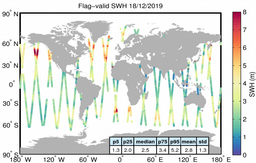
Figure 15. Geographical distribution of flag-valid SWH data over oceans and lakes for 18/12/2019. The statistical values shown in the table refer to the SWH in m and are calculated over all measurements shown in the figure.
