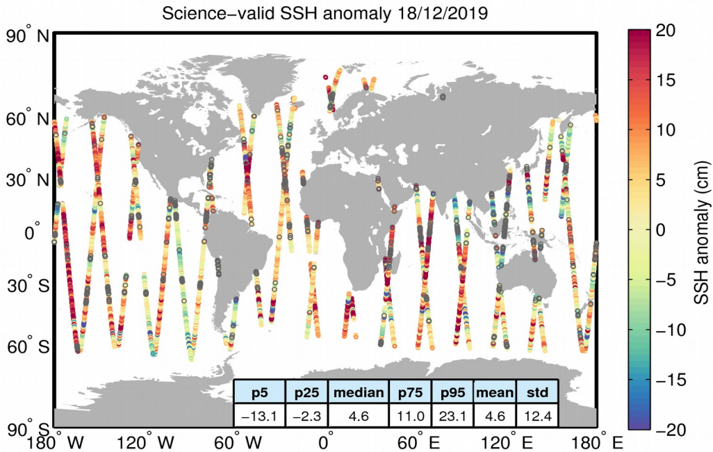
Figure 10. Geographical distribution of science-valid SSH anomaly data over oceans and lakes for 18/12/2019. The statistical values shown in the table refer to the SSH anomaly in cm and are calculated over all measurements shown in the figure. Gray circles denote records that have been rejected based on the editing criteria described in Table 2.
