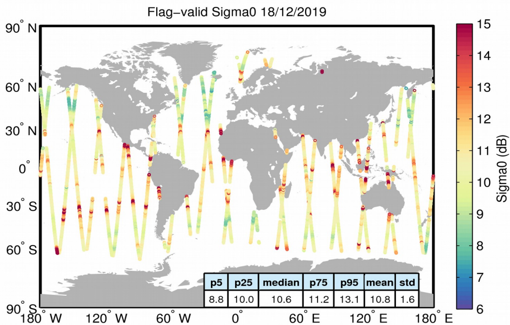
Figure 23. Geographical distribution of flag-valid sigma0 data over oceans and lakes for 18/12/2019. The statistical values shown in the table refer to the sigma0 in dB and are calculated over all measurements shown in the figure.
