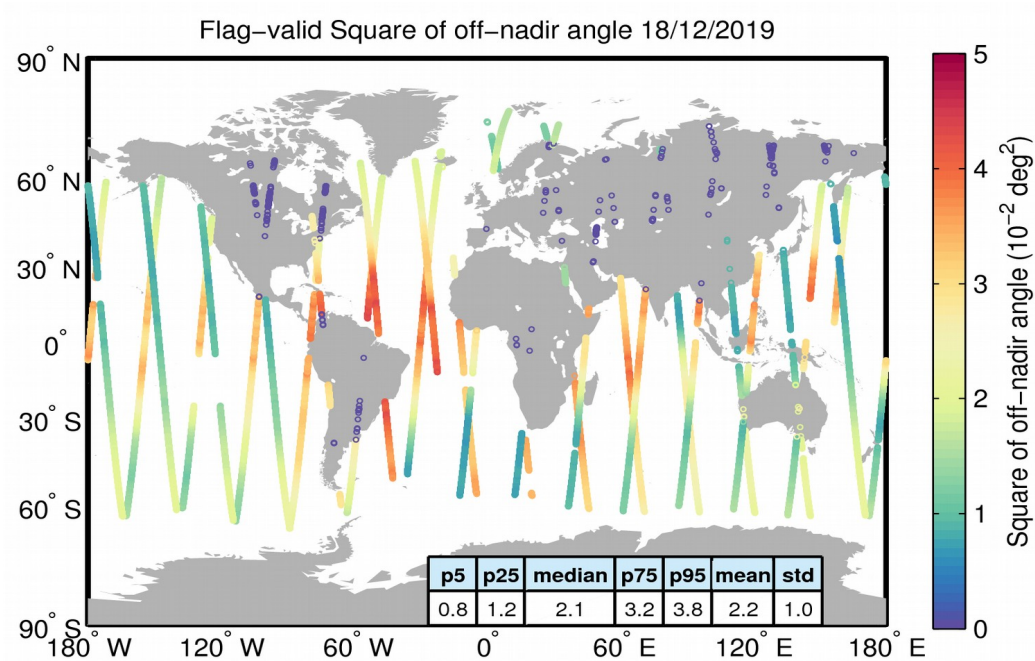
Figure 37. Geographical distribution of flag-valid mispointing data over oceans and lakes for 18/12/2019. The statistical values shown in the table refer to the mispointing in 10^{-2} deg 2 and are calculated over all measurements shown in the figure.
