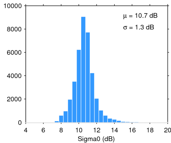
Figure 28. Histogram of science-valid sigma0 over oceans and lakes for 18/12/2019. The mean ( \mu ) and standard deviation ( \sigma ) are also shown. Note that values outside [4 20] dB are excluded from the histogram for the sake of readability but not from the computation of \mu and \sigma .
