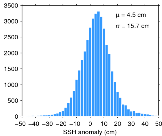
Figure 7. Histogram of flag-valid SSH anomaly over oceans and lakes for 18/12/2019. The mean ( \mu ) and standard deviation ( \sigma ) are also shown. Note that values outside [-50 50] cm are excluded from the histogram for the sake of readability but not from the computation of \mu and \sigma .
