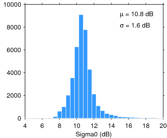
Figure 25. Histogram of flag-valid sigma0 over oceans and lakes for 18/12/2019. The mean ( \mu ) and standard deviation ( \sigma ) are also shown. Note that values outside [4 20] dB are excluded from the histogram for the sake of readability but not from the computation of \mu and \sigma .
