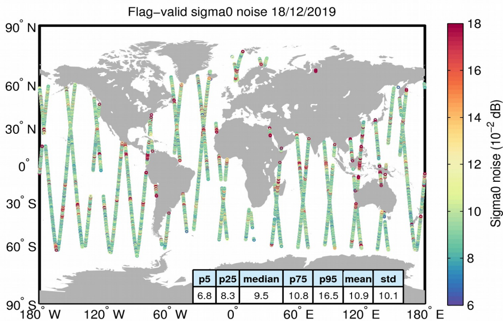
Figure 26. Geographical distribution of flag-valid 20-Hz sigma0 measurement noise over oceans and lakes for 18/12/2019. The statistical values shown in the table refer to the sigma0 noise and are calculated over all measurements shown in the figure.
