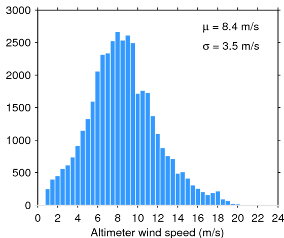
Figure 35. Histogram of science-valid wind over oceans and lakes for 18/12/2019. The mean ( \mu ) and standard deviation ( \sigma ) are also shown. Note that values larger than 24 m/s are excluded from the histogram for the sake of readability but not from the computation of \mu and \sigma .
