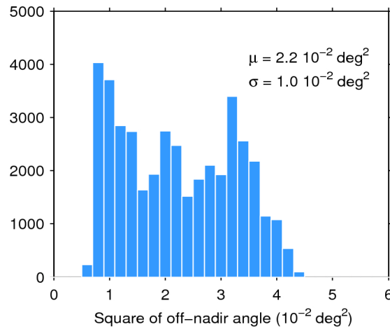
Figure 39. Histogram of flag-valid mispointing over oceans and lakes for 18/12/2019. The mean ( \mu ) and standard deviation ( \sigma ) are also shown. Note that values larger than 6 \cdot 10^{-2} \text{ deg}^2 are excluded from the histogram for the sake of readability but not from the computation of \mu and \sigma .
