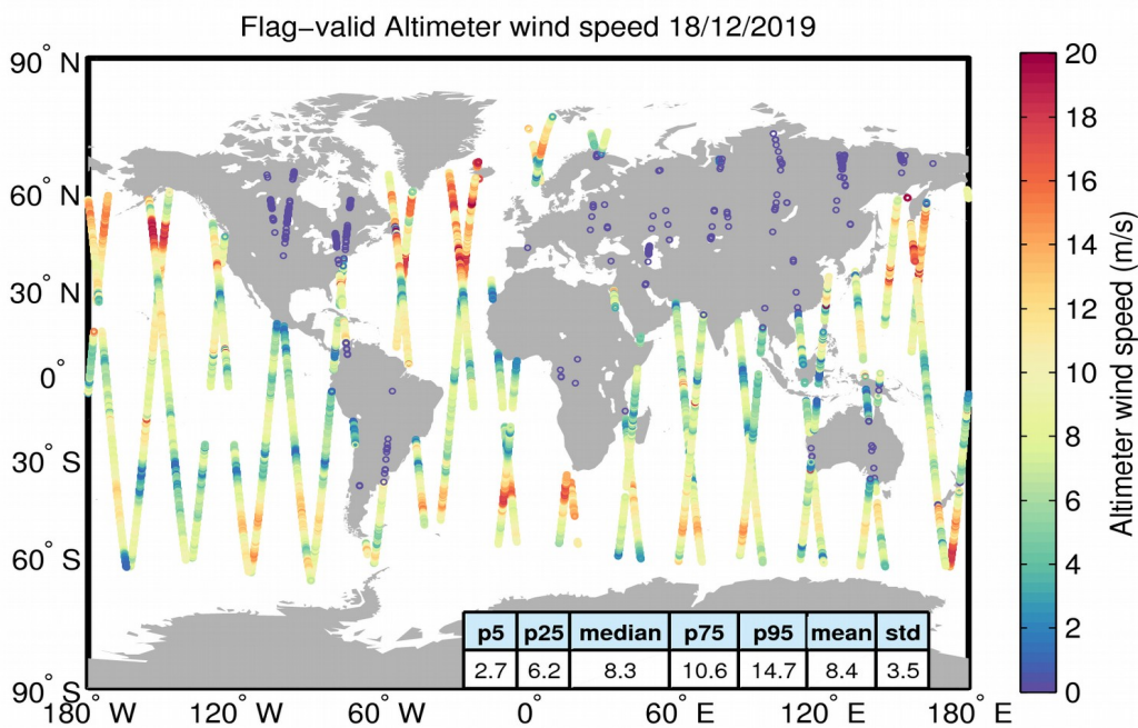
Figure 31. Geographical distribution of flag-valid wind data over oceans and lakes for 18/12/2019. The statistical values shown in the table refer to the wind in m/s and are calculated over all measurements shown in the figure.
