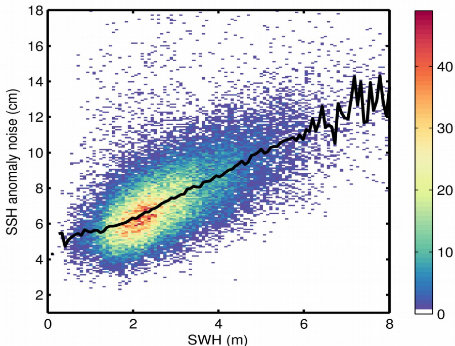
Figure 9. 2D histogram showing flag-valid SSH anomaly noise as a function of SWH for 18/12/2019. The black line denotes the median SSH anomaly noise as a function of SWH.
