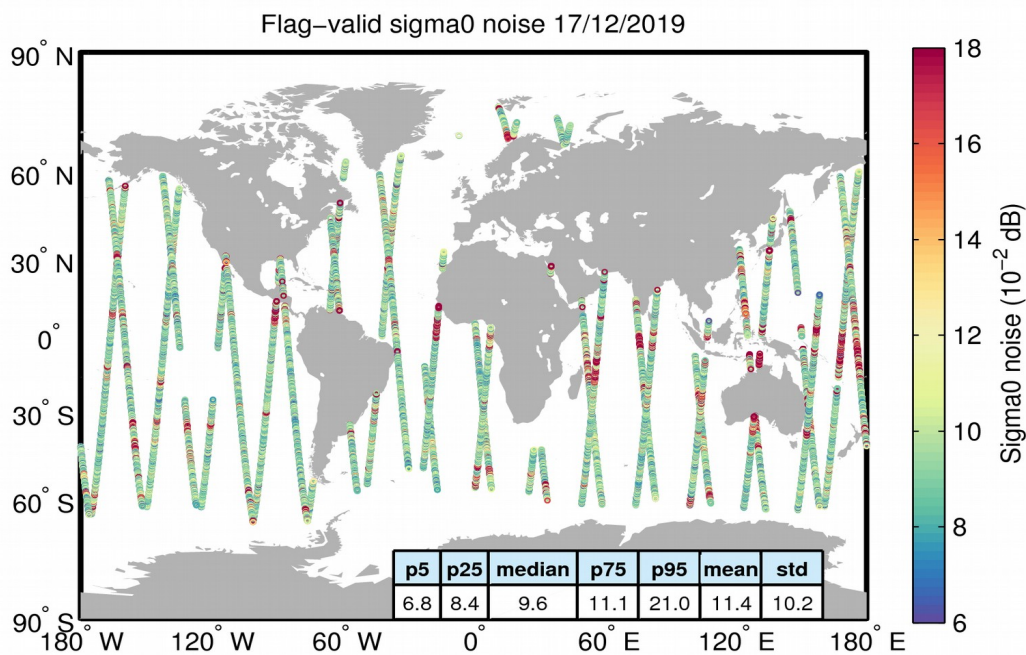
Figure 26. Geographical distribution of flag-valid 20-Hz sigma0 measurement noise over oceans and lakes for 17/12/2019. The statistical values shown in the table refer to the sigma0 noise and are calculated over all measurements shown in the figure.
