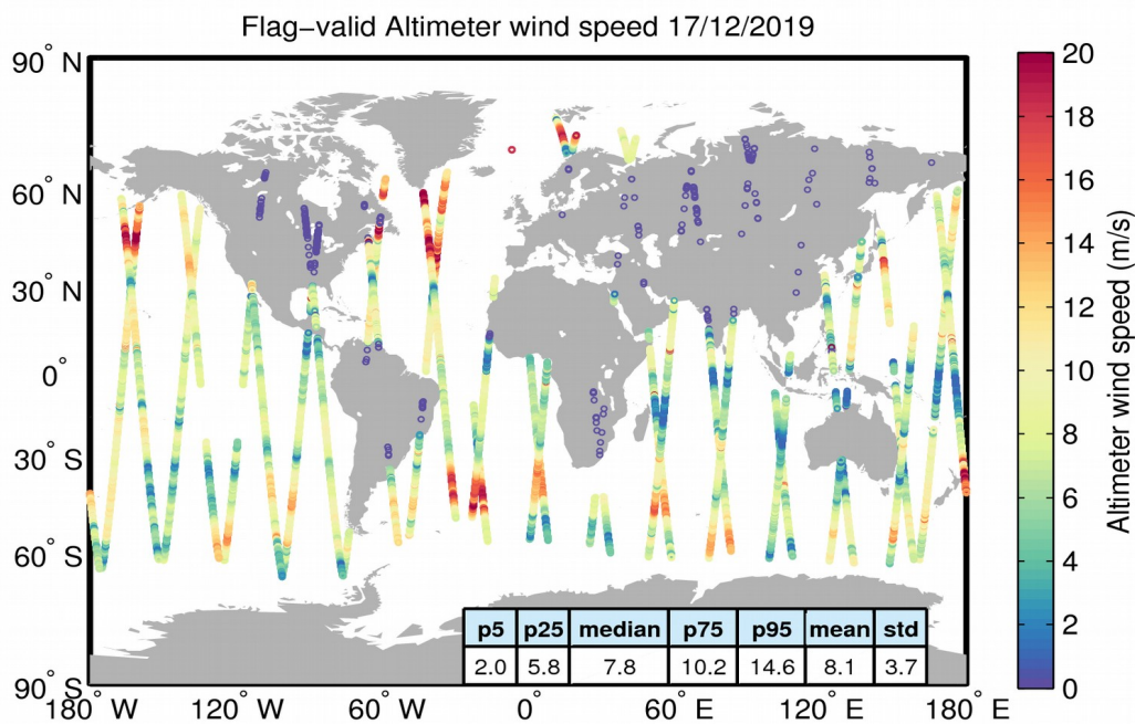
Figure 31. Geographical distribution of flag-valid wind data over oceans and lakes for 17/12/2019. The statistical values shown in the table refer to the wind in m/s and are calculated over all measurements shown in the figure.
