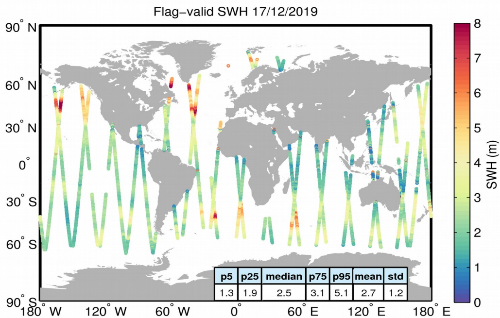
Figure 15. Geographical distribution of flag-valid SWH data over oceans and lakes for 17/12/2019. The statistical values shown in the table refer to the SWH in m and are calculated over all measurements shown in the figure.
