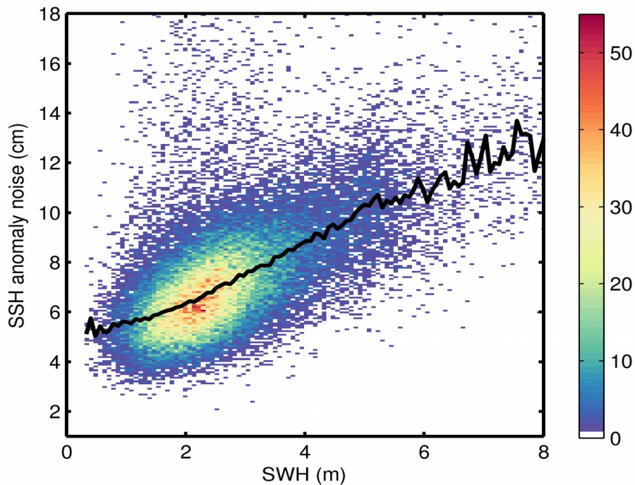
Figure 9. 2D histogram showing flag-valid SSH anomaly noise as a function of SWH for 17/12/2019. The black line denotes the median SSH anomaly noise as a function of SWH.
