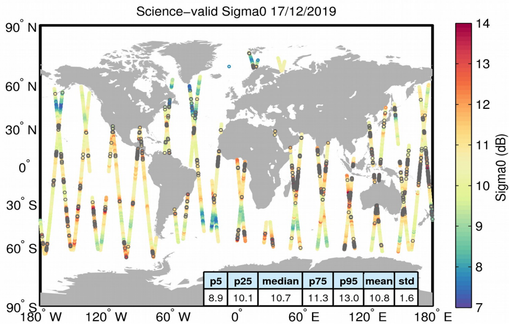
Figure 27. Geographical distribution of science-valid sigma0 data over oceans and lakes for 17/12/2019. The statistical values shown in the table refer to the sigma0 in dB and are calculated over all measurements shown in the figure. Gray circles denote records that have been rejected based on the editing criteria described in Table 4.
