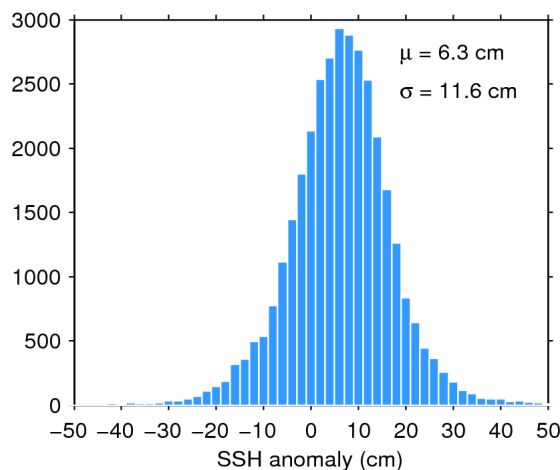
Figure 11. Histogram of science-valid SSH anomaly over oceans and lakes for 17/12/2019. The mean ( \mu ) and standard deviation ( \sigma ) are also shown. Note that values outside [-50 50] cm are excluded from the histogram for the sake of readability but not from the computation of \mu and \sigma .
