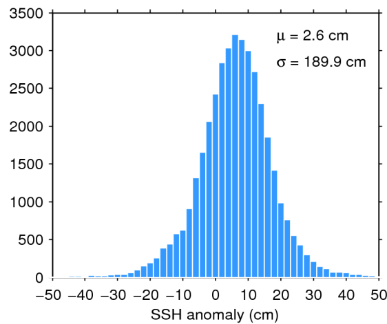
Figure 7. Histogram of flag-valid SSH anomaly over oceans and lakes for 17/12/2019. The mean ( \mu ) and standard deviation ( \sigma ) are also shown. Note that values outside [-50 50] cm are excluded from the histogram for the sake of readability but not from the computation of \mu and \sigma .
