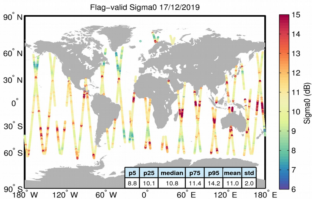
Figure 23. Geographical distribution of flag-valid sigma0 data over oceans and lakes for 17/12/2019. The statistical values shown in the table refer to the sigma0 in dB and are calculated over all measurements shown in the figure.
