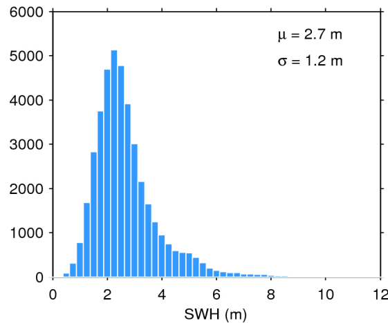
Figure 20. Histogram of science-valid SWH over oceans and lakes for 17/12/2019. The mean ( \mu ) and standard deviation ( \sigma ) are also shown. Note that values larger than 12 m are excluded from the histogram for the sake of readability but not from the computation of \mu and \sigma .
