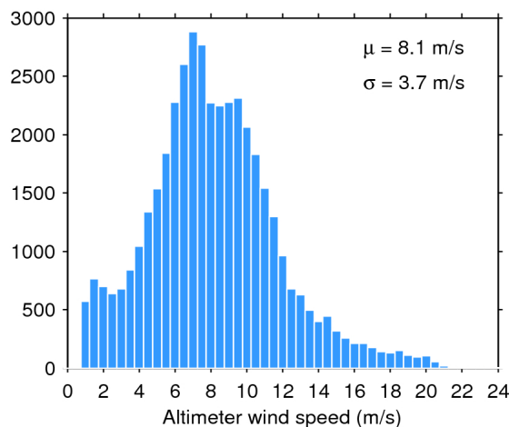
Figure 35. Histogram of science-valid wind over oceans and lakes for 17/12/2019. The mean ( \mu ) and standard deviation ( \sigma ) are also shown. Note that values larger than 24 m/s are excluded from the histogram for the sake of readability but not from the computation of \mu and \sigma .
