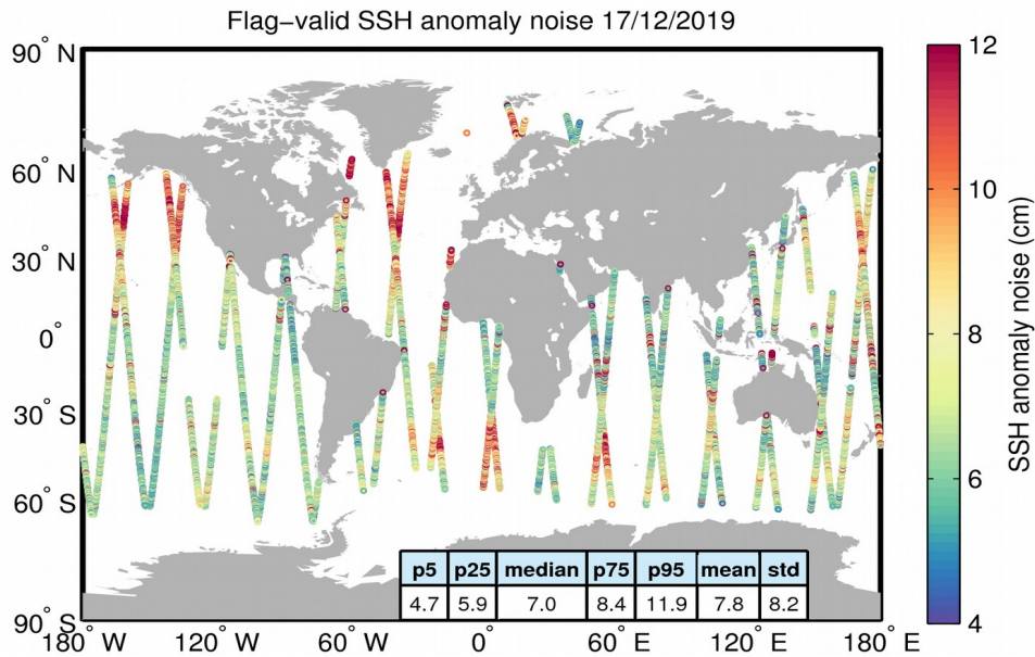
Figure 8. Geographical distribution of flag-valid 20-Hz SSH anomaly measurement noise over oceans and lakes for 17/12/2019. The statistical values shown in the table refer to the SSH anomaly noise and are calculated over all measurements shown in the figure.
