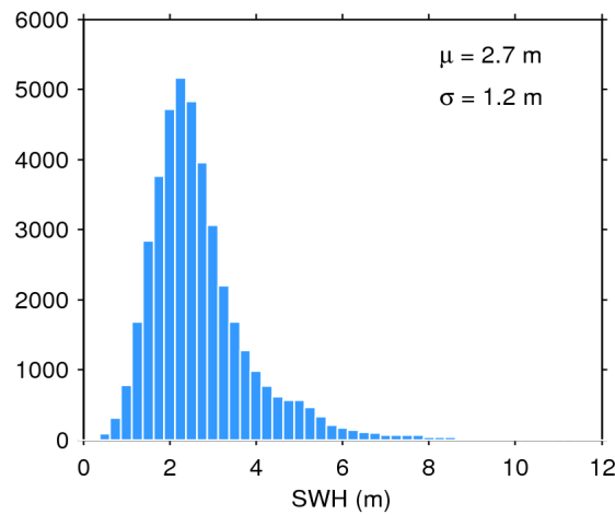
Figure 17. Histogram of flag-valid SWH over oceans and lakes for 17/12/2019. The mean ( \mu ) and standard deviation ( \sigma ) are also shown. Note that values larger than 12 m are excluded from the histogram for the sake of readability but not from the computation of \mu and \sigma .
