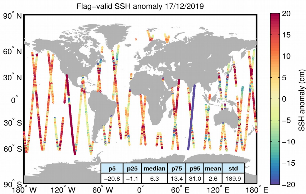
Figure 5. Geographical distribution of flag-valid 1-Hz SSH anomaly data over oceans and lakes for 17/12/2019. The statistical values shown in the table refer to the SSH anomaly in cm and are calculated over all measurements shown in the figure.
