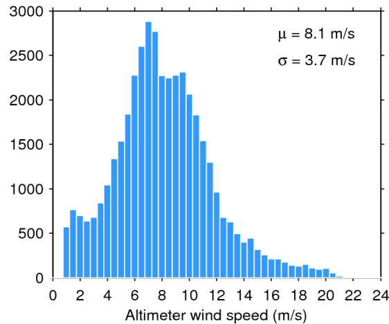
Figure 33. Histogram of flag-valid wind over oceans and lakes for 17/12/2019. The mean ( \mu ) and standard deviation ( \sigma ) are also shown. Note that values larger than 24 m/s are excluded from the histogram for the sake of readability but not from the computation of \mu and \sigma .
