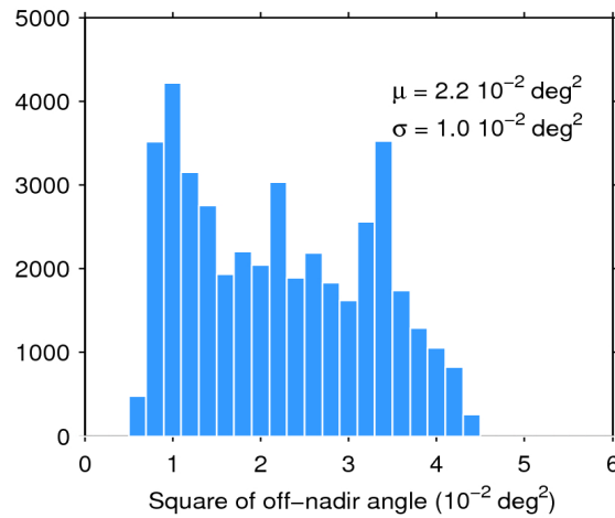
Figure 39. Histogram of flag-valid mispointing over oceans and lakes for 17/12/2019. The mean ( \mu ) and standard deviation ( \sigma ) are also shown. Note that values larger than 6 \cdot 10^{-2} \text{ deg}^2 are excluded from the histogram for the sake of readability but not from the computation of \mu and \sigma .
