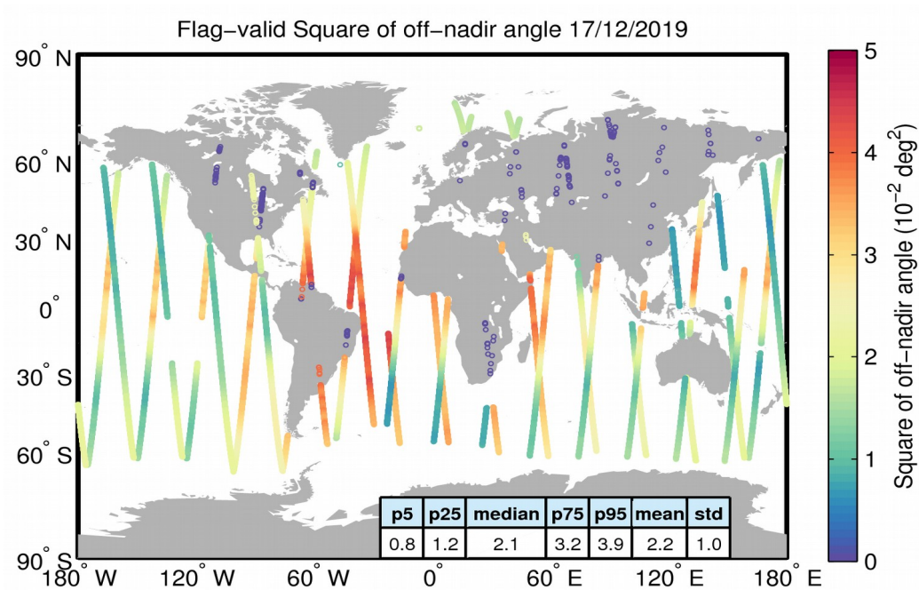
Figure 37. Geographical distribution of flag-valid mispointing data over oceans and lakes for 17/12/2019. The statistical values shown in the table refer to the mispointing in 10^{-2} deg 2 and are calculated over all measurements shown in the figure.
