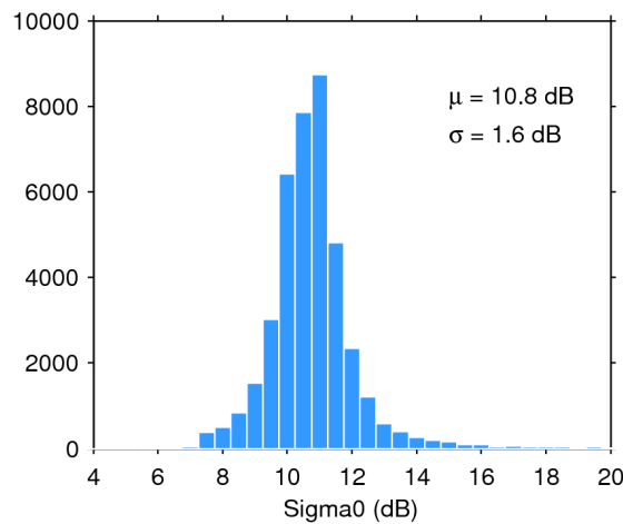
Figure 28. Histogram of science-valid sigma0 over oceans and lakes for 17/12/2019. The mean ( \mu ) and standard deviation ( \sigma ) are also shown. Note that values outside [4 20] dB are excluded from the histogram for the sake of readability but not from the computation of \mu and \sigma .
