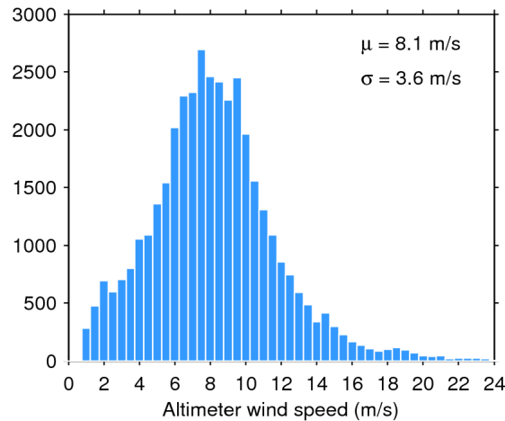
Figure 33. Histogram of flag-valid wind over oceans and lakes for 16/12/2019. The mean ( \mu ) and standard deviation ( \sigma ) are also shown. Note that values larger than 24 m/s are excluded from the histogram for the sake of readability but not from the computation of \mu and \sigma .
