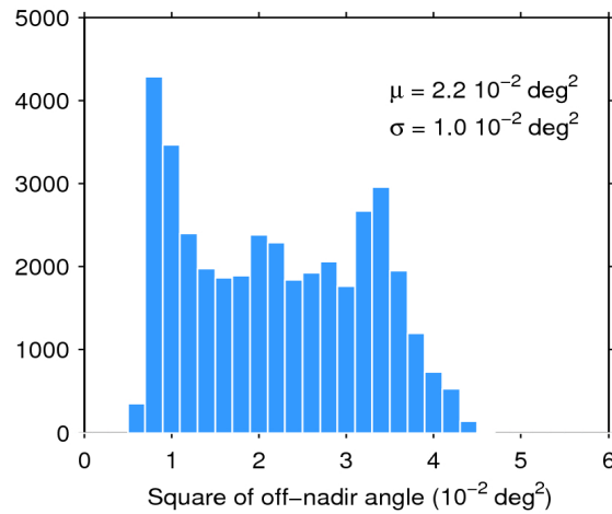
Figure 39. Histogram of flag-valid mispointing over oceans and lakes for 16/12/2019. The mean ( \mu ) and standard deviation ( \sigma ) are also shown. Note that values larger than 6 \cdot 10^{-2} \text{ deg}^2 are excluded from the histogram for the sake of readability but not from the computation of \mu and \sigma .
