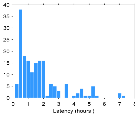
Figure 2. Histogram of the data latency for 16/12/2019. The y-axis denotes the number of files that are made available with a delay of x-hours with respect to the mean time of the records stored in the file.
