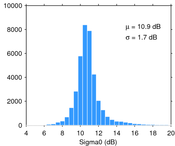
Figure 25. Histogram of flag-valid sigma0 over oceans and lakes for 16/12/2019. The mean ( \mu ) and standard deviation ( \sigma ) are also shown. Note that values outside [4 20] dB are excluded from the histogram for the sake of readability but not from the computation of \mu and \sigma .
