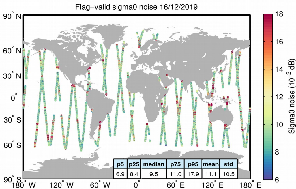
Figure 26. Geographical distribution of flag-valid 20-Hz sigma0 measurement noise over oceans and lakes for 16/12/2019. The statistical values shown in the table refer to the sigma0 noise and are calculated over all measurements shown in the figure.
