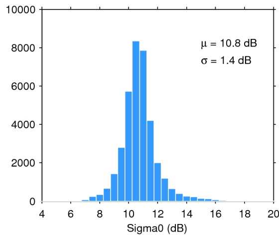
Figure 28. Histogram of science-valid sigma0 over oceans and lakes for 16/12/2019. The mean ( \mu ) and standard deviation ( \sigma ) are also shown. Note that values outside [4 20] dB are excluded from the histogram for the sake of readability but not from the computation of \mu and \sigma .
