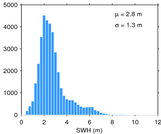
Figure 20. Histogram of science-valid SWH over oceans and lakes for 16/12/2019. The mean ( \mu ) and standard deviation ( \sigma ) are also shown. Note that values larger than 12 m are excluded from the histogram for the sake of readability but not from the computation of \mu and \sigma .
