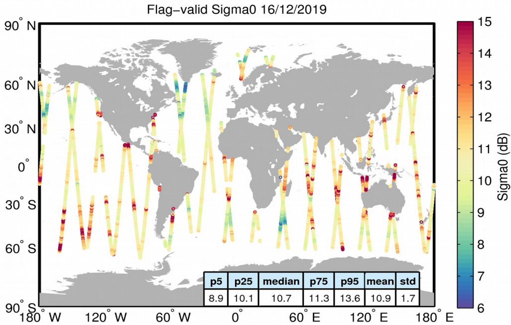
Figure 23. Geographical distribution of flag-valid sigma0 data over oceans and lakes for 16/12/2019. The statistical values shown in the table refer to the sigma0 in dB and are calculated over all measurements shown in the figure.
