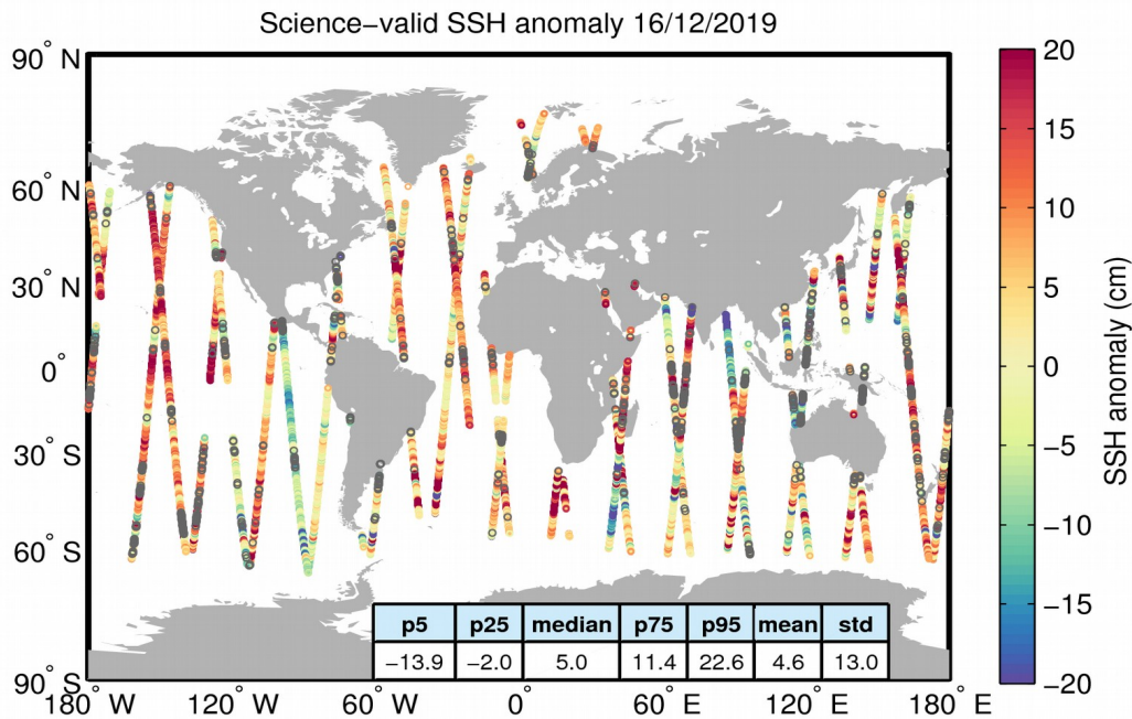
Figure 10. Geographical distribution of science-valid SSH anomaly data over oceans and lakes for 16/12/2019. The statistical values shown in the table refer to the SSH anomaly in cm and are calculated over all measurements shown in the figure. Gray circles denote records that have been rejected based on the editing criteria described in Table 2.
