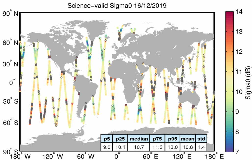
Figure 27. Geographical distribution of science-valid sigma0 data over oceans and lakes for 16/12/2019. The statistical values shown in the table refer to the sigma0 in dB and are calculated over all measurements shown in the figure. Gray circles denote records that have been rejected based on the editing criteria described in Table 4.
