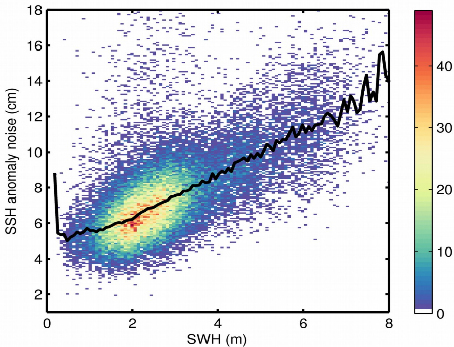
Figure 9. 2D histogram showing flag-valid SSH anomaly noise as a function of SWH for 16/12/2019. The black line denotes the median SSH anomaly noise as a function of SWH.
