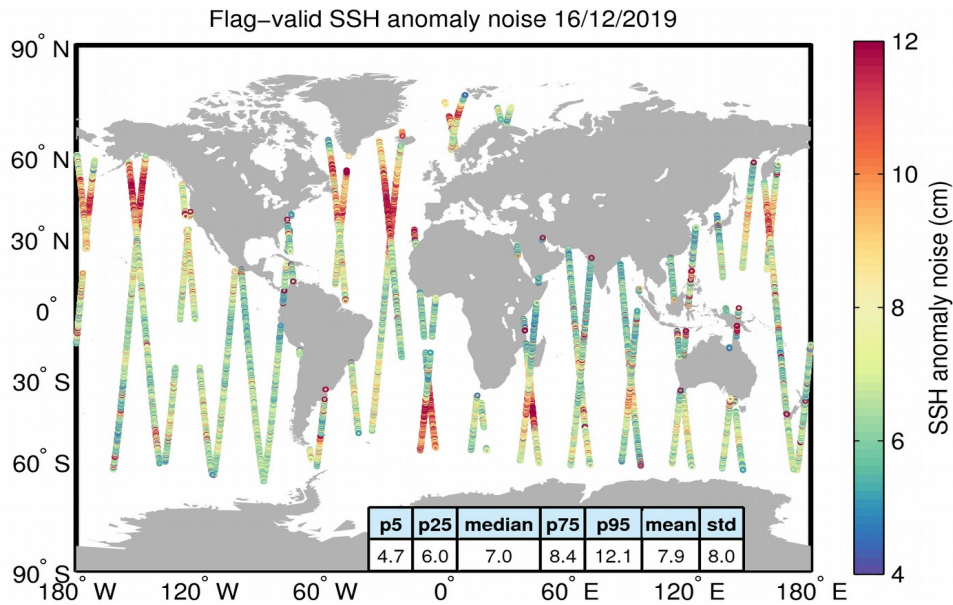
Figure 8. Geographical distribution of flag-valid 20-Hz SSH anomaly measurement noise over oceans and lakes for 16/12/2019. The statistical values shown in the table refer to the SSH anomaly noise and are calculated over all measurements shown in the figure.
