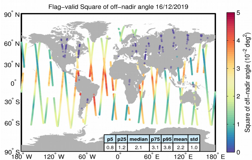
Figure 37. Geographical distribution of flag-valid mispointing data over oceans and lakes for 16/12/2019. The statistical values shown in the table refer to the mispointing in 10^{-2} \text{ deg}^2 and are calculated over all measurements shown in the figure.
