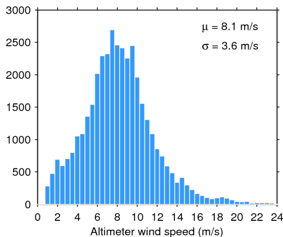
Figure 35. Histogram of science-valid wind over oceans and lakes for 16/12/2019. The mean ( \mu ) and standard deviation ( \sigma ) are also shown. Note that values larger than 24 m/s are excluded from the histogram for the sake of readability but not from the computation of \mu and \sigma .
