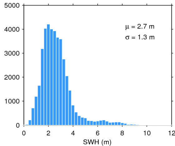
Figure 20. Histogram of science-valid SWH over oceans and lakes for 15/12/2019. The mean ( \mu ) and standard deviation ( \sigma ) are also shown. Note that values larger than 12 m are excluded from the histogram for the sake of readability but not from the computation of \mu and \sigma .
