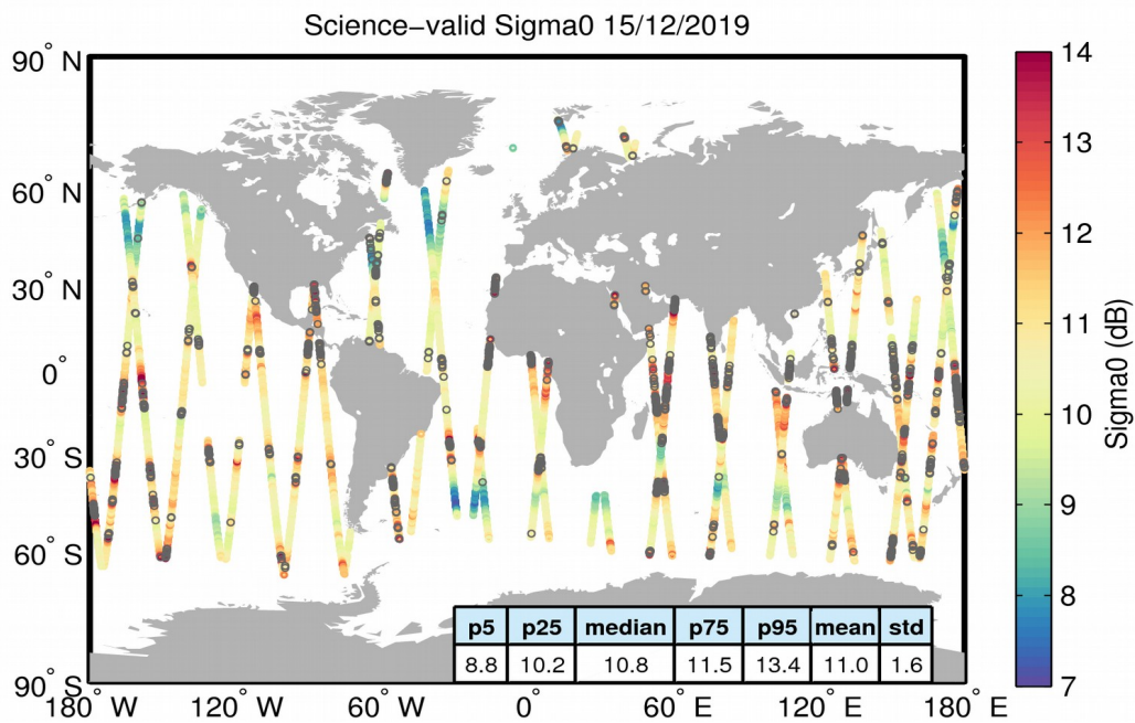
Figure 27. Geographical distribution of science-valid sigma0 data over oceans and lakes for 15/12/2019. The statistical values shown in the table refer to the sigma0 in dB and are calculated over all measurements shown in the figure. Gray circles denote records that have been rejected based on the editing criteria described in Table 4.
