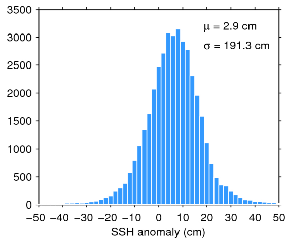
Figure 7. Histogram of flag-valid SSH anomaly over oceans and lakes for 15/12/2019. The mean ( \mu ) and standard deviation ( \sigma ) are also shown. Note that values outside [-50\ 50] cm are excluded from the histogram for the sake of readability but not from the computation of \mu and \sigma .
