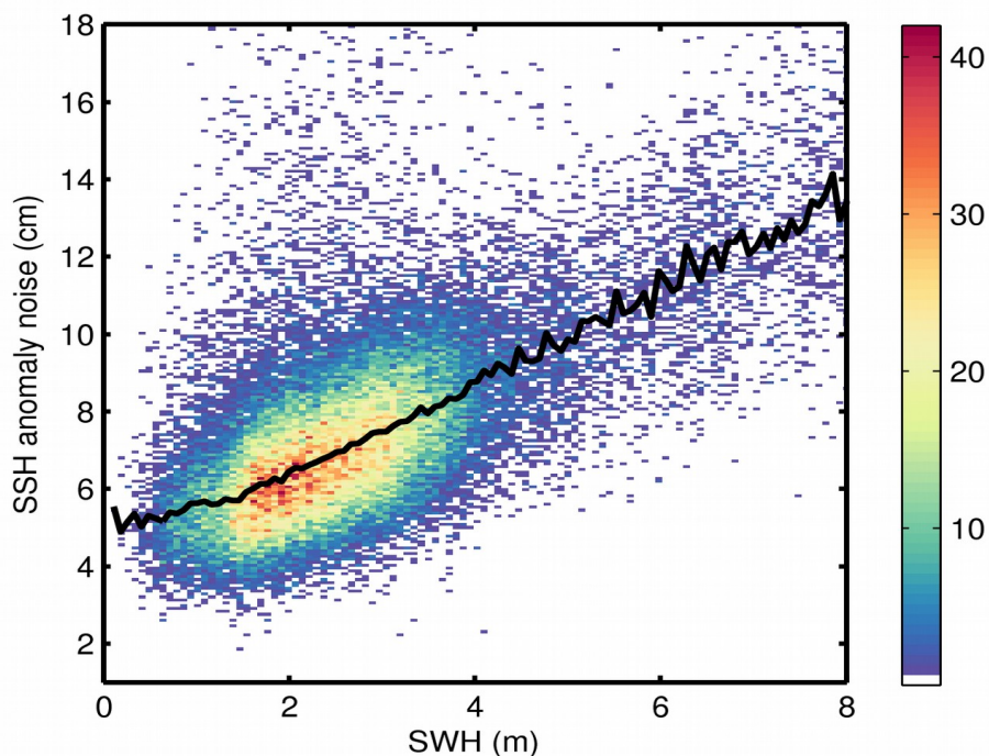
Figure 9. 2D histogram showing flag-valid SSH anomaly noise as a function of SWH for 15/12/2019. The black line denotes the median SSH anomaly noise as a function of SWH.
