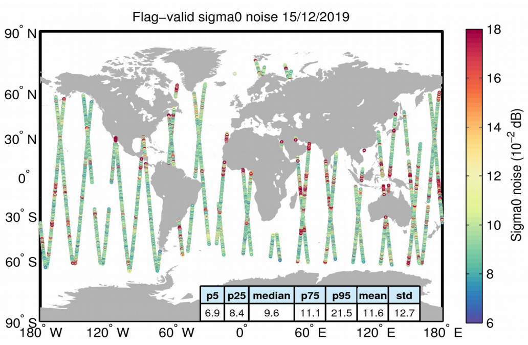
Figure 26. Geographical distribution of flag-valid 20-Hz sigma0 measurement noise over oceans and lakes for 15/12/2019. The statistical values shown in the table refer to the sigma0 noise and are calculated over all measurements shown in the figure.
