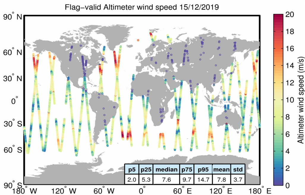
Figure 31. Geographical distribution of flag-valid wind data over oceans and lakes for 15/12/2019. The statistical values shown in the table refer to the wind in m/s and are calculated over all measurements shown in the figure.
