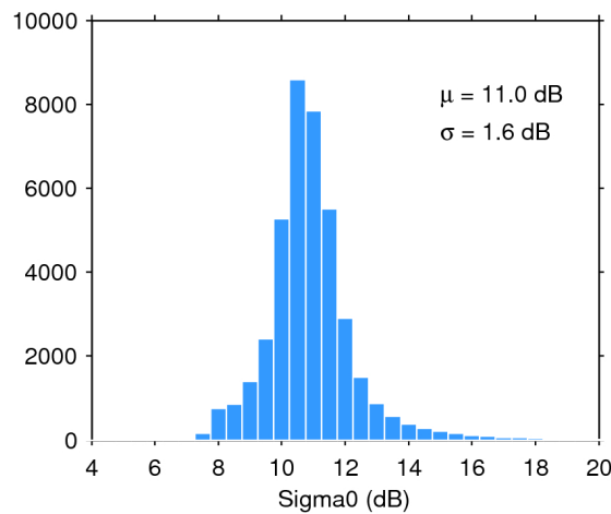
Figure 28. Histogram of science-valid sigma0 over oceans and lakes for 15/12/2019. The mean ( \mu ) and standard deviation ( \sigma ) are also shown. Note that values outside [4 20] dB are excluded from the histogram for the sake of readability but not from the computation of \mu and \sigma .
