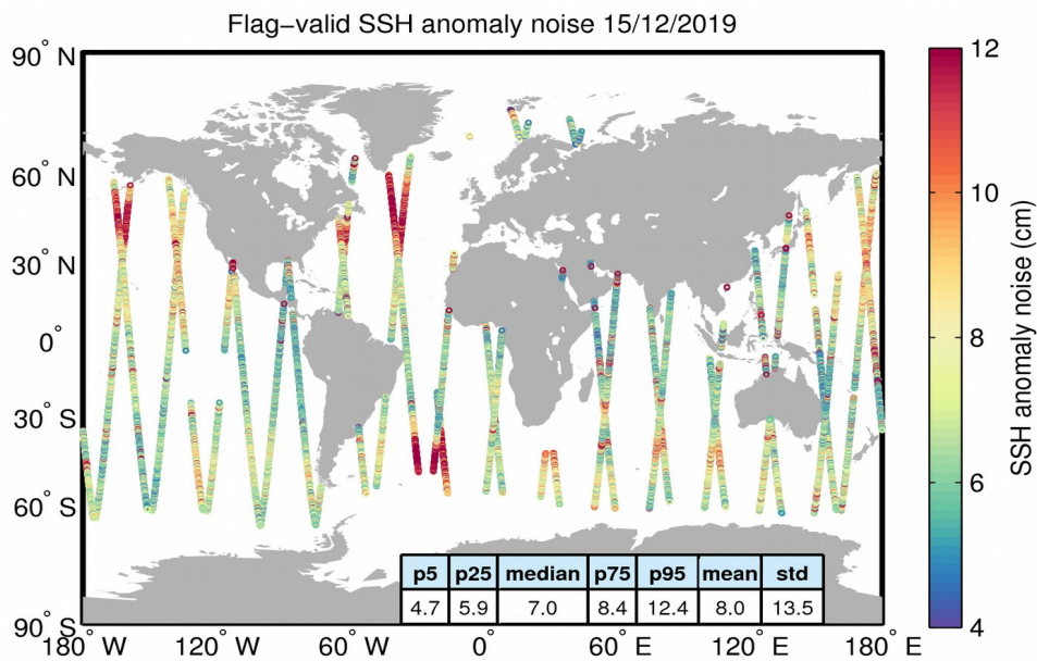
Figure 8. Geographical distribution of flag-valid 20-Hz SSH anomaly measurement noise over oceans and lakes for 15/12/2019. The statistical values shown in the table refer to the SSH anomaly noise and are calculated over all measurements shown in the figure.
