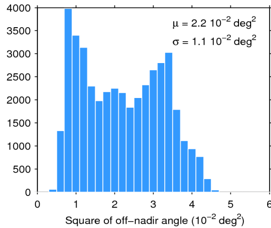
Figure 39. Histogram of flag-valid mispointing over oceans and lakes for 15/12/2019. The mean ( \mu ) and standard deviation ( \sigma ) are also shown. Note that values larger than 6 \cdot 10^{-2} \text{ deg}^2 are excluded from the histogram for the sake of readability but not from the computation of \mu and \sigma .
