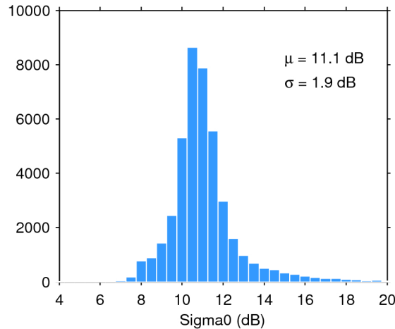
Figure 25. Histogram of flag-valid sigma0 over oceans and lakes for 15/12/2019. The mean ( \mu ) and standard deviation ( \sigma ) are also shown. Note that values outside [4 20] dB are excluded from the histogram for the sake of readability but not from the computation of \mu and \sigma .
