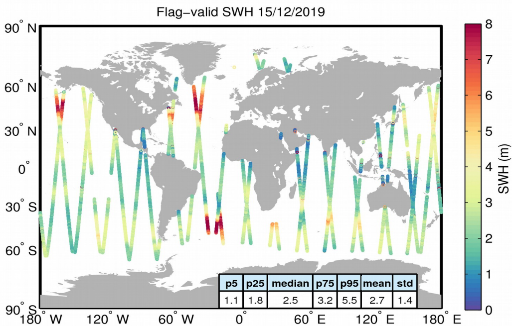
Figure 15. Geographical distribution of flag-valid SWH data over oceans and lakes for 15/12/2019. The statistical values shown in the table refer to the SWH in m and are calculated over all measurements shown in the figure.
