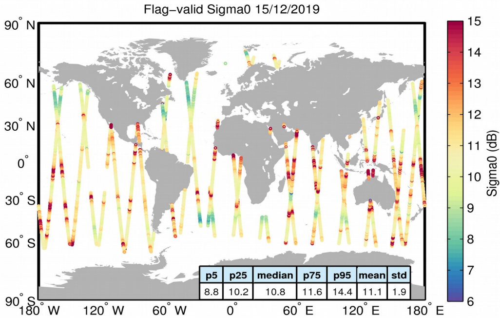
Figure 23. Geographical distribution of flag-valid sigma0 data over oceans and lakes for 15/12/2019. The statistical values shown in the table refer to the sigma0 in dB and are calculated over all measurements shown in the figure.
