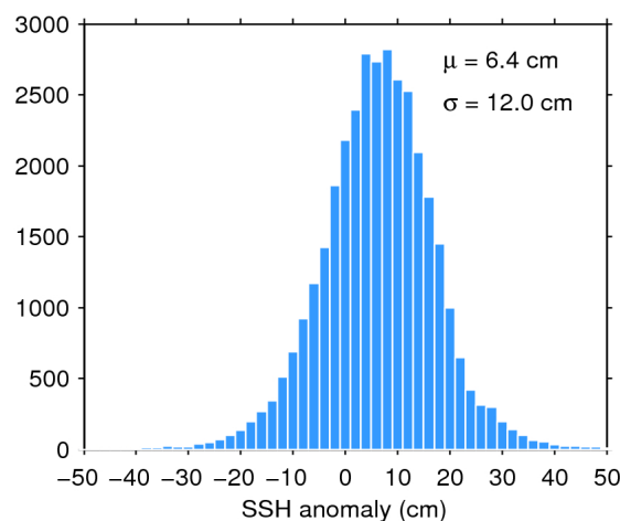
Figure 11. Histogram of science-valid SSH anomaly over oceans and lakes for 15/12/2019. The mean ( \mu ) and standard deviation ( \sigma ) are also shown. Note that values outside [-50 50] cm are excluded from the histogram for the sake of readability but not from the computation of \mu and \sigma .
