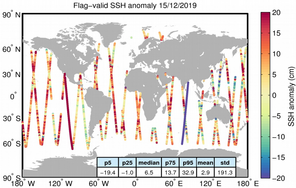
Figure 5. Geographical distribution of flag-valid 1-Hz SSH anomaly data over oceans and lakes for 15/12/2019. The statistical values shown in the table refer to the SSH anomaly in cm and are calculated over all measurements shown in the figure.
