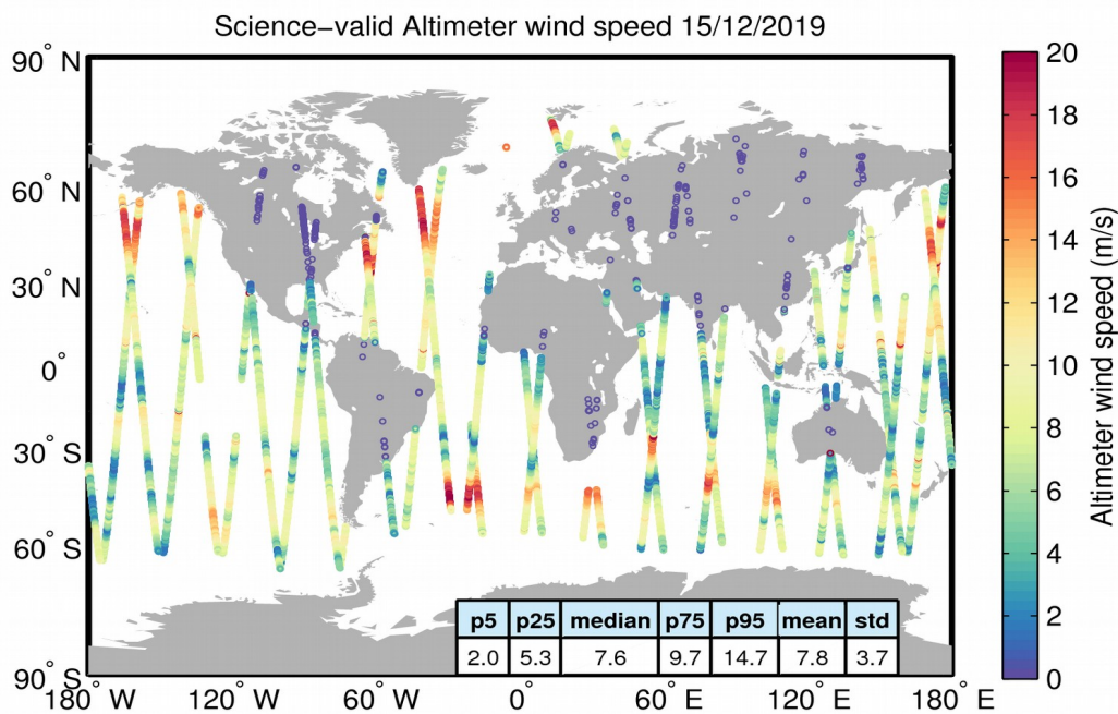
Figure 34. Geographical distribution of science-valid wind data over oceans and lakes for 15/12/2019. The statistical values shown in the table refer to the wind in m/s and are calculated over all measurements shown in the figure. Gray circles denote records that have been rejected based on the editing criteria described in Table 5.
