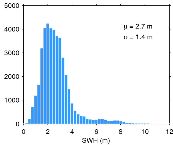
Figure 17. Histogram of flag-valid SWH over oceans and lakes for 15/12/2019. The mean ( \mu ) and standard deviation ( \sigma ) are also shown. Note that values larger than 12 m are excluded from the histogram for the sake of readability but not from the computation of \mu and \sigma .
