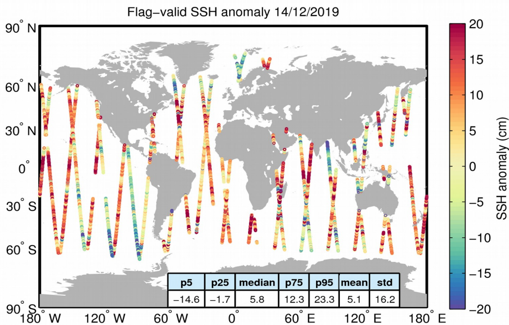
Figure 5. Geographical distribution of flag-valid 1-Hz SSH anomaly data over oceans and lakes for 14/12/2019. The statistical values shown in the table refer to the SSH anomaly in cm and are calculated over all measurements shown in the figure.
