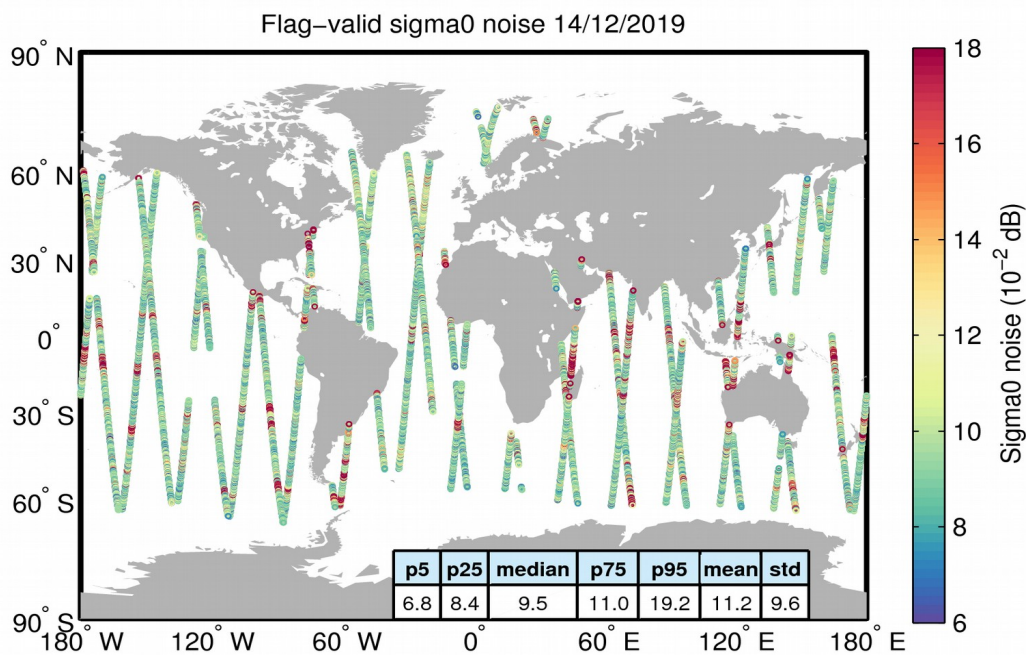
Figure 26. Geographical distribution of flag-valid 20-Hz sigma0 measurement noise over oceans and lakes for 14/12/2019. The statistical values shown in the table refer to the sigma0 noise and are calculated over all measurements shown in the figure.
