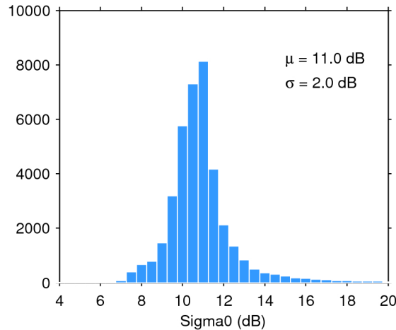
Figure 25. Histogram of flag-valid sigma0 over oceans and lakes for 14/12/2019. The mean ( \mu ) and standard deviation ( \sigma ) are also shown. Note that values outside [4 20] dB are excluded from the histogram for the sake of readability but not from the computation of \mu and \sigma .
