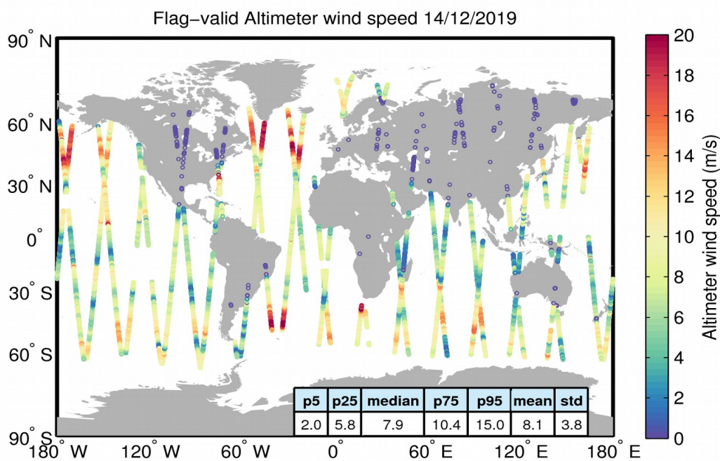
Figure 31. Geographical distribution of flag-valid wind data over oceans and lakes for 14/12/2019. The statistical values shown in the table refer to the wind in m/s and are calculated over all measurements shown in the figure.
