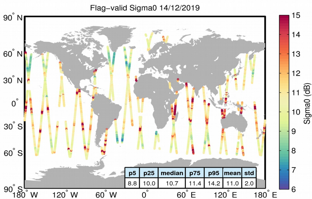
Figure 23. Geographical distribution of flag-valid sigma0 data over oceans and lakes for 14/12/2019. The statistical values shown in the table refer to the sigma0 in dB and are calculated over all measurements shown in the figure.
