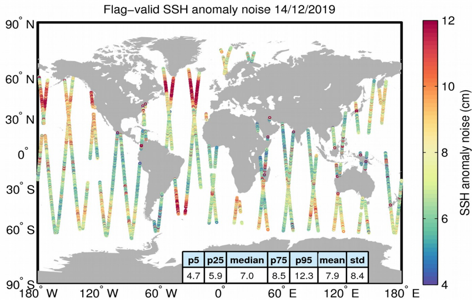
Figure 8. Geographical distribution of flag-valid 20-Hz SSH anomaly measurement noise over oceans and lakes for 14/12/2019. The statistical values shown in the table refer to the SSH anomaly noise and are calculated over all measurements shown in the figure.
