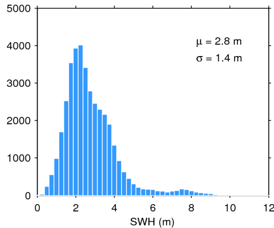
Figure 20. Histogram of science-valid SWH over oceans and lakes for 14/12/2019. The mean ( \mu ) and standard deviation ( \sigma ) are also shown. Note that values larger than 12 m are excluded from the histogram for the sake of readability but not from the computation of \mu and \sigma .
