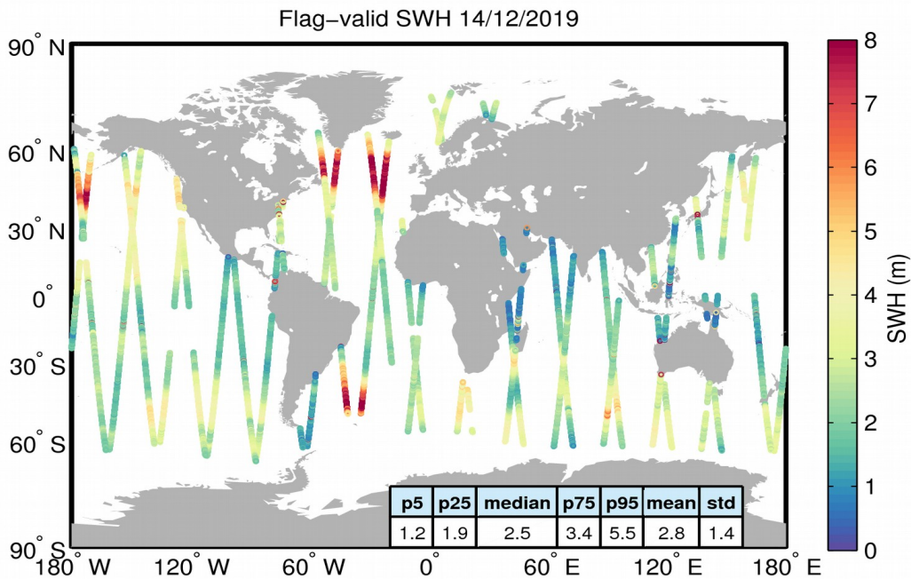
Figure 15. Geographical distribution of flag-valid SWH data over oceans and lakes for 14/12/2019. The statistical values shown in the table refer to the SWH in m and are calculated over all measurements shown in the figure.
