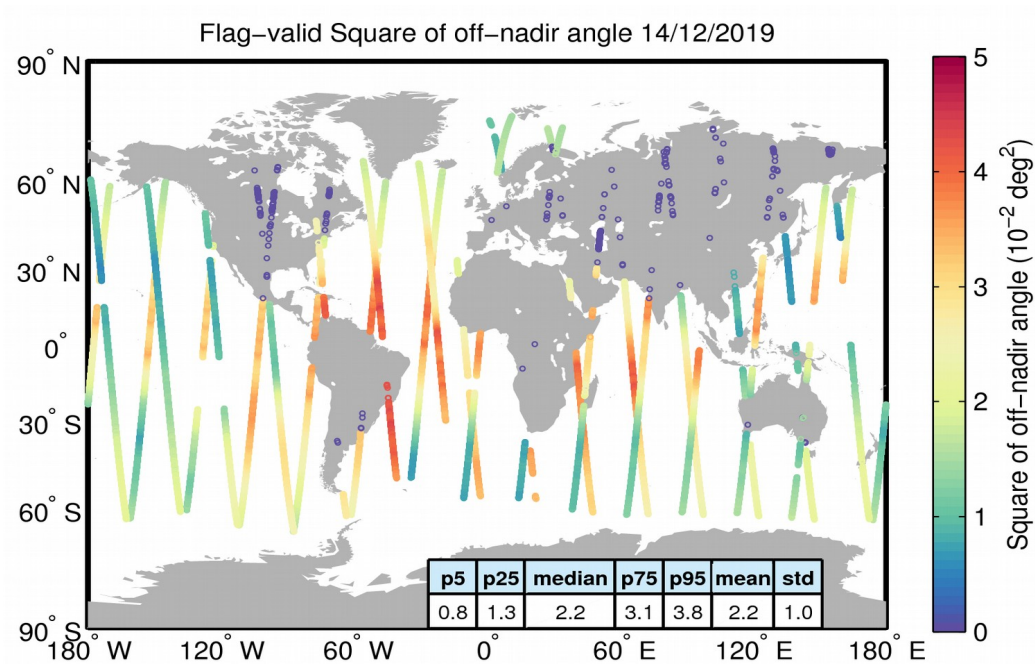
Figure 37. Geographical distribution of flag-valid mispointing data over oceans and lakes for 14/12/2019. The statistical values shown in the table refer to the mispointing in 10^{-2} deg 2 and are calculated over all measurements shown in the figure.
