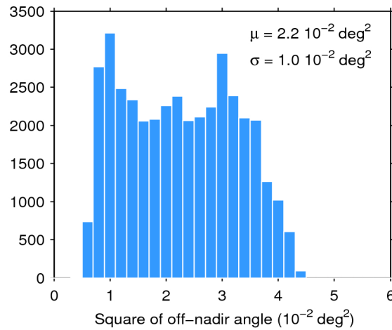
Figure 39. Histogram of flag-valid mispointing over oceans and lakes for 14/12/2019. The mean ( \mu ) and standard deviation ( \sigma ) are also shown. Note that values larger than 6 \cdot 10^{-2} \text{ deg}^2 are excluded from the histogram for the sake of readability but not from the computation of \mu and \sigma .
