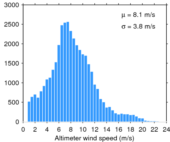
Figure 33. Histogram of flag-valid wind over oceans and lakes for 14/12/2019. The mean ( \mu ) and standard deviation ( \sigma ) are also shown. Note that values larger than 24 m/s are excluded from the histogram for the sake of readability but not from the computation of \mu and \sigma .
