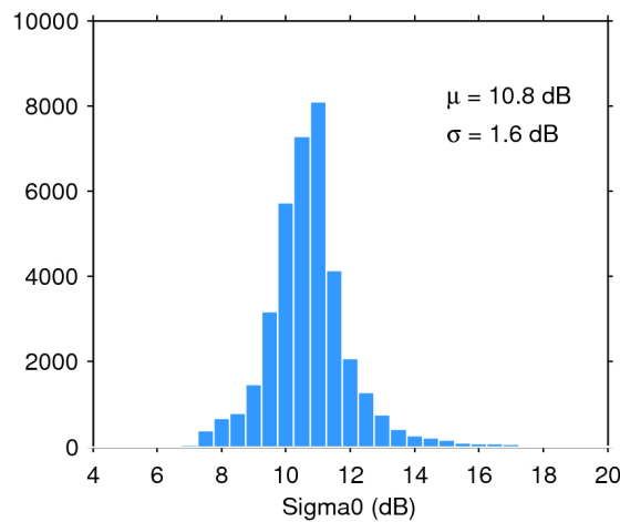
Figure 28. Histogram of science-valid sigma0 over oceans and lakes for 14/12/2019. The mean ( \mu ) and standard deviation ( \sigma ) are also shown. Note that values outside [4 20] dB are excluded from the histogram for the sake of readability but not from the computation of \mu and \sigma .
