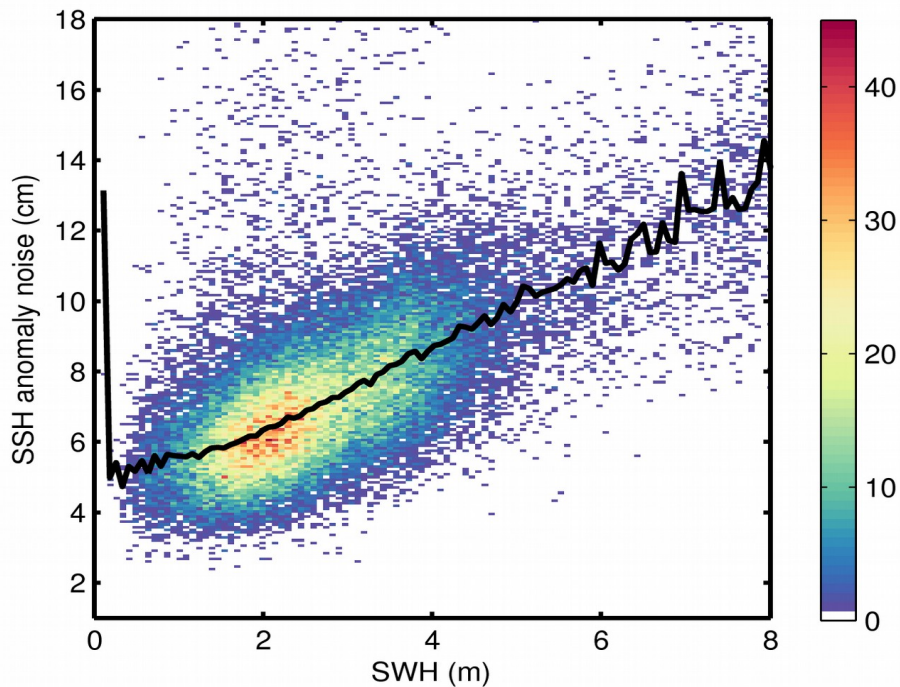
Figure 9. 2D histogram showing flag-valid SSH anomaly noise as a function of SWH for 14/12/2019. The black line denotes the median SSH anomaly noise as a function of SWH.
