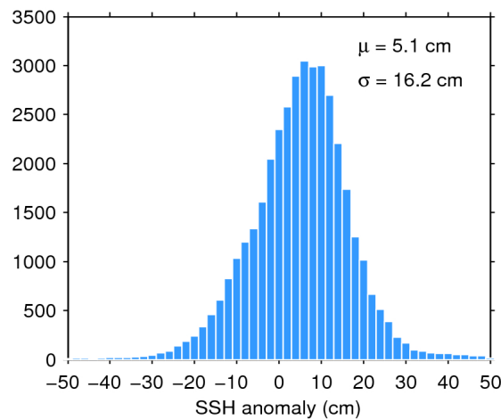
Figure 7. Histogram of flag-valid SSH anomaly over oceans and lakes for 14/12/2019. The mean ( \mu ) and standard deviation ( \sigma ) are also shown. Note that values outside [-50 50] cm are excluded from the histogram for the sake of readability but not from the computation of \mu and \sigma .
