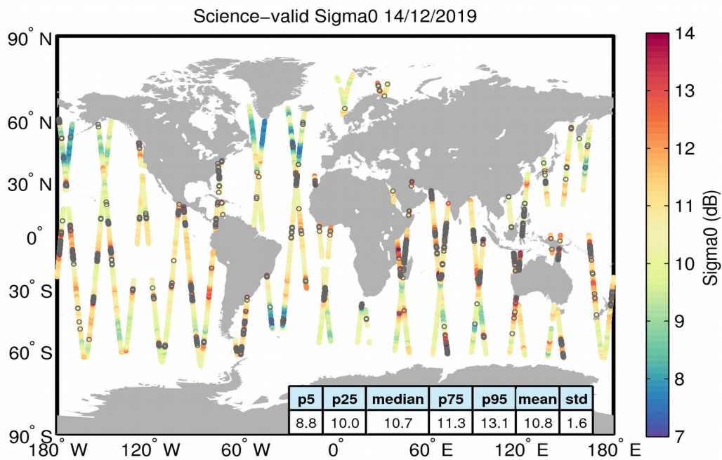
Figure 27. Geographical distribution of science-valid sigma0 data over oceans and lakes for 14/12/2019. The statistical values shown in the table refer to the sigma0 in dB and are calculated over all measurements shown in the figure. Gray circles denote records that have been rejected based on the editing criteria described in Table 4.
