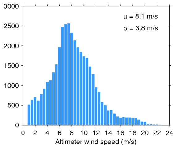
Figure 35. Histogram of science-valid wind over oceans and lakes for 14/12/2019. The mean ( \mu ) and standard deviation ( \sigma ) are also shown. Note that values larger than 24 m/s are excluded from the histogram for the sake of readability but not from the computation of \mu and \sigma .
