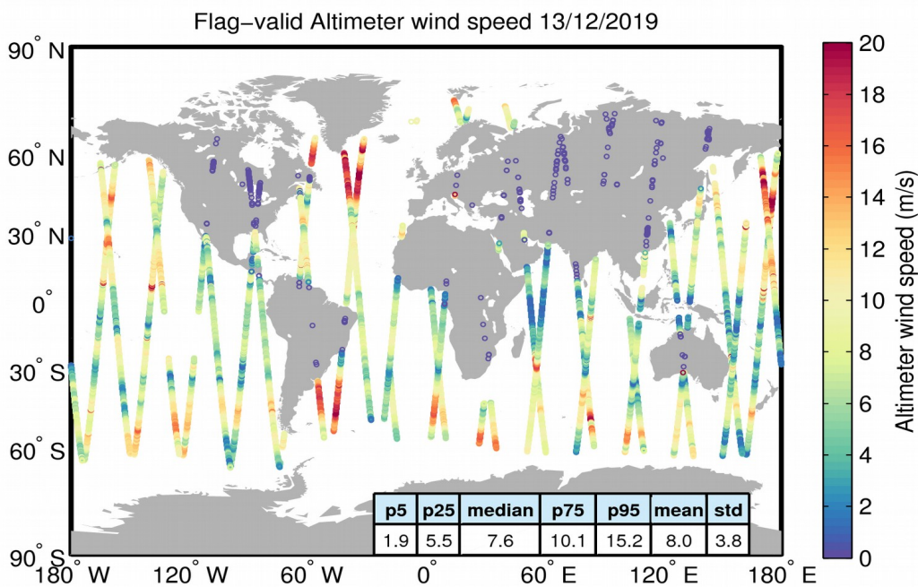
Figure 31. Geographical distribution of flag-valid wind data over oceans and lakes for 13/12/2019. The statistical values shown in the table refer to the wind in m/s and are calculated over all measurements shown in the figure.
