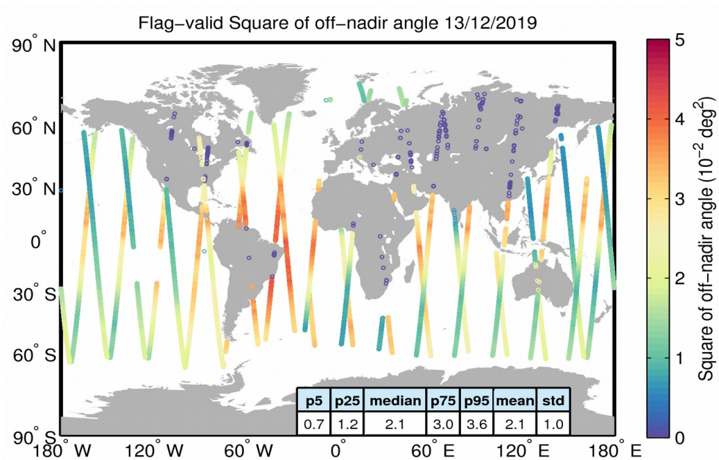
Figure 37. Geographical distribution of flag-valid mispointing data over oceans and lakes for 13/12/2019. The statistical values shown in the table refer to the mispointing in 10^{-2} \text{ deg}^2 and are calculated over all measurements shown in the figure.
