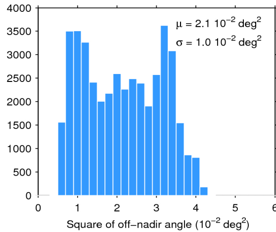
Figure 39. Histogram of flag-valid mispointing over oceans and lakes for 13/12/2019. The mean ( \mu ) and standard deviation ( \sigma ) are also shown. Note that values larger than 6 \cdot 10^{-2} \text{ deg}^2 are excluded from the histogram for the sake of readability but not from the computation of \mu and \sigma .
