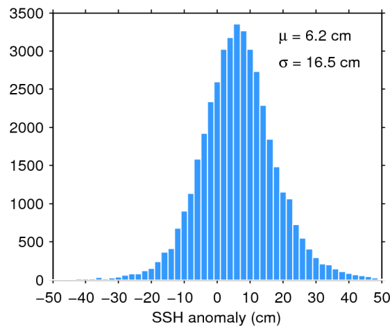
Figure 7. Histogram of flag-valid SSH anomaly over oceans and lakes for 13/12/2019. The mean ( \mu ) and standard deviation ( \sigma ) are also shown. Note that values outside [-50\ 50] cm are excluded from the histogram for the sake of readability but not from the computation of \mu and \sigma .
