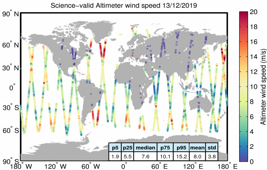
Figure 34. Geographical distribution of science-valid wind data over oceans and lakes for 13/12/2019. The statistical values shown in the table refer to the wind in m/s and are calculated over all measurements shown in the figure. Gray circles denote records that have been rejected based on the editing criteria described in Table 5.
