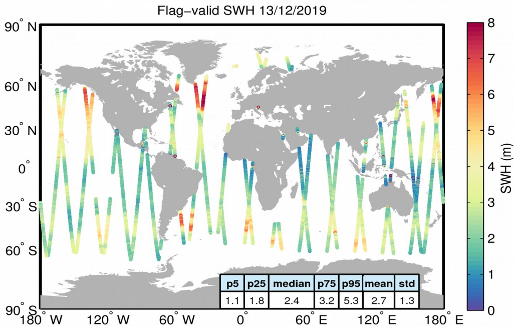
Figure 15. Geographical distribution of flag-valid SWH data over oceans and lakes for 13/12/2019. The statistical values shown in the table refer to the SWH in m and are calculated over all measurements shown in the figure.
