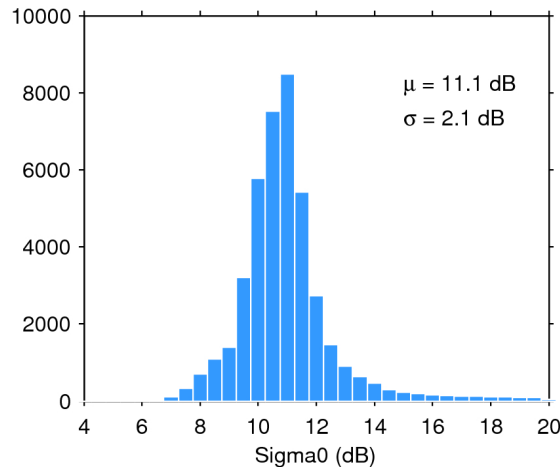
Figure 25. Histogram of flag-valid sigma0 over oceans and lakes for 13/12/2019. The mean ( \mu ) and standard deviation ( \sigma ) are also shown. Note that values outside [4 20] dB are excluded from the histogram for the sake of readability but not from the computation of \mu and \sigma .
