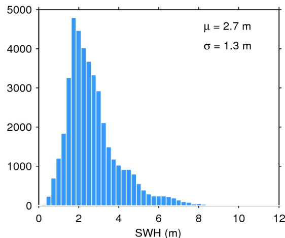
Figure 20. Histogram of science-valid SWH over oceans and lakes for 13/12/2019. The mean ( \mu ) and standard deviation ( \sigma ) are also shown. Note that values larger than 12 m are excluded from the histogram for the sake of readability but not from the computation of \mu and \sigma .
