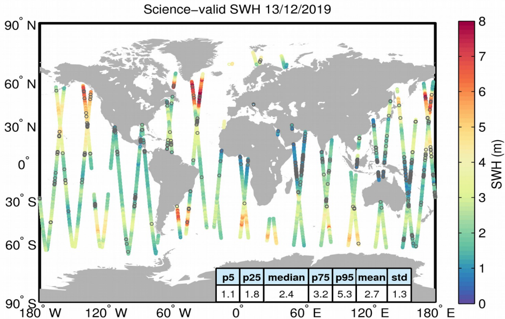
Figure 19. Geographical distribution of science-valid SWH data over oceans and lakes for 13/12/2019. The statistical values shown in the table refer to the SWH in m and are calculated over all measurements shown in the figure. Gray circles denote records that have been rejected based on the editing criteria described in Table 3.
