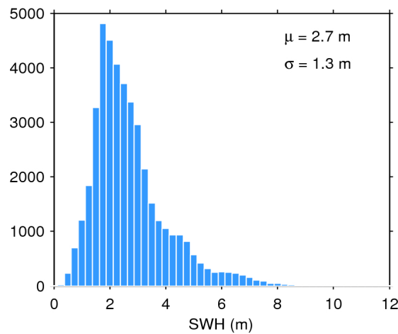
Figure 17. Histogram of flag-valid SWH over oceans and lakes for 13/12/2019. The mean ( \mu ) and standard deviation ( \sigma ) are also shown. Note that values larger than 12 m are excluded from the histogram for the sake of readability but not from the computation of \mu and \sigma .
