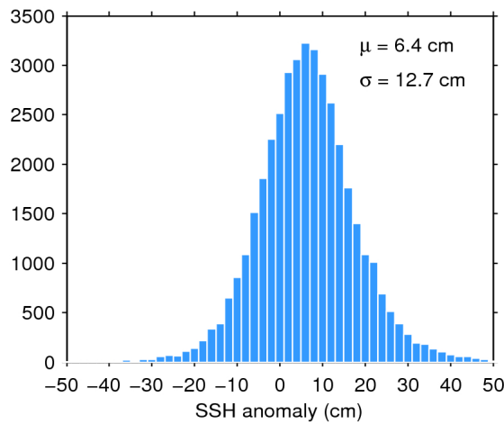
Figure 11. Histogram of science-valid SSH anomaly over oceans and lakes for 13/12/2019. The mean ( \mu ) and standard deviation ( \sigma ) are also shown. Note that values outside [-50 50] cm are excluded from the histogram for the sake of readability but not from the computation of \mu and \sigma .
