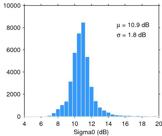
Figure 28. Histogram of science-valid sigma0 over oceans and lakes for 13/12/2019. The mean ( \mu ) and standard deviation ( \sigma ) are also shown. Note that values outside [4 20] dB are excluded from the histogram for the sake of readability but not from the computation of \mu and \sigma .
