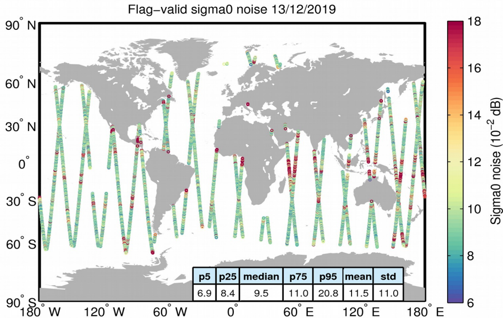
Figure 26. Geographical distribution of flag-valid 20-Hz sigma0 measurement noise over oceans and lakes for 13/12/2019. The statistical values shown in the table refer to the sigma0 noise and are calculated over all measurements shown in the figure.
