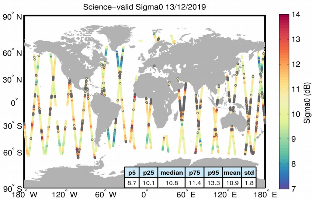
Figure 27. Geographical distribution of science-valid sigma0 data over oceans and lakes for 13/12/2019. The statistical values shown in the table refer to the sigma0 in dB and are calculated over all measurements shown in the figure. Gray circles denote records that have been rejected based on the editing criteria described in Table 4.
