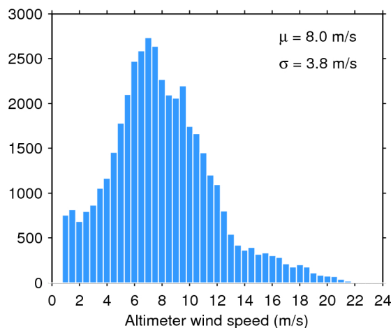
Figure 35. Histogram of science-valid wind over oceans and lakes for 13/12/2019. The mean ( \mu ) and standard deviation ( \sigma ) are also shown. Note that values larger than 24 m/s are excluded from the histogram for the sake of readability but not from the computation of \mu and \sigma .
