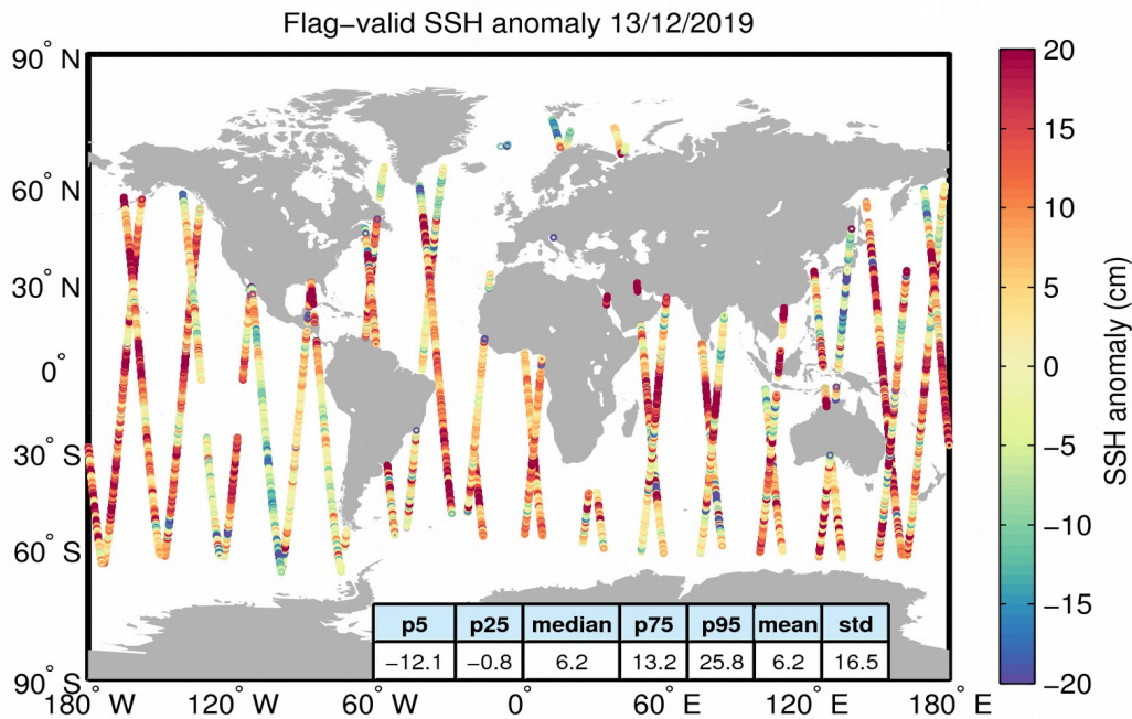
Figure 5. Geographical distribution of flag-valid 1-Hz SSH anomaly data over oceans and lakes for 13/12/2019. The statistical values shown in the table refer to the SSH anomaly in cm and are calculated over all measurements shown in the figure.
