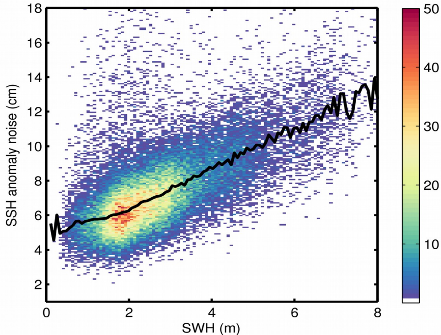
Figure 9. 2D histogram showing flag-valid SSH anomaly noise as a function of SWH for 13/12/2019. The black line denotes the median SSH anomaly noise as a function of SWH.
