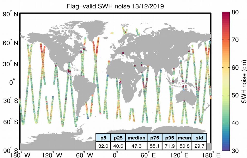
Figure 18. Geographical distribution of flag-valid 20-Hz SWH measurement noise over oceans and lakes for 13/12/2019. The statistical values shown in the figure refer to the SWH noise and are calculated over all measurements shown in the figure.
