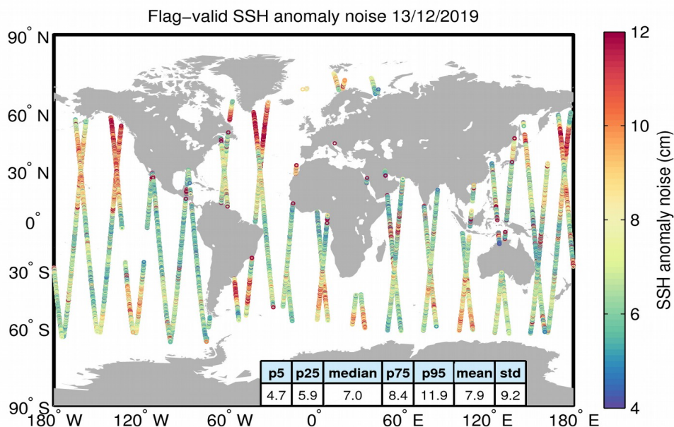
Figure 8. Geographical distribution of flag-valid 20-Hz SSH anomaly measurement noise over oceans and lakes for 13/12/2019. The statistical values shown in the table refer to the SSH anomaly noise and are calculated over all measurements shown in the figure.
