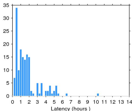
Figure 2. Histogram of the data latency for 13/12/2019. The y-axis denotes the number of files that are made available with a delay of x-hours with respect to the mean time of the records stored in the file.
