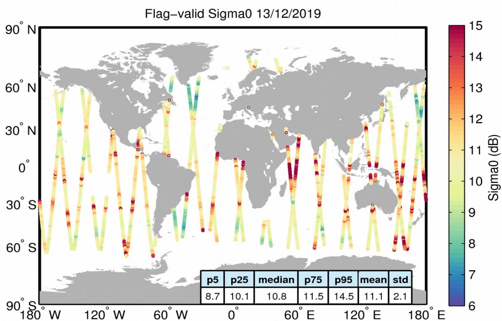
Figure 23. Geographical distribution of flag-valid sigma0 data over oceans and lakes for 13/12/2019. The statistical values shown in the table refer to the sigma0 in dB and are calculated over all measurements shown in the figure.
