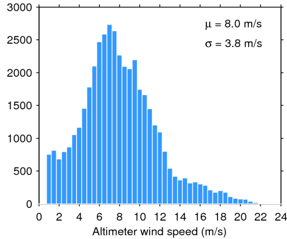
Figure 33. Histogram of flag-valid wind over oceans and lakes for 13/12/2019. The mean ( \mu ) and standard deviation ( \sigma ) are also shown. Note that values larger than 24 m/s are excluded from the histogram for the sake of readability but not from the computation of \mu and \sigma .
