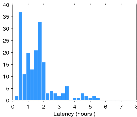
Figure 2. Histogram of the data latency for 12/12/2019. The y-axis denotes the number of files that are made available with a delay of x-hours with respect to the mean time of the records stored in the file.
