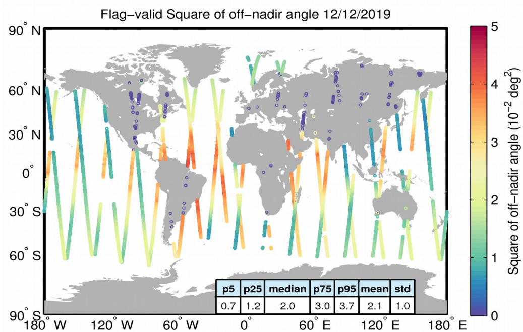
Figure 37. Geographical distribution of flag-valid mispointing data over oceans and lakes for 12/12/2019. The statistical values shown in the table refer to the mispointing in 10^{-2} deg 2 and are calculated over all measurements shown in the figure.
