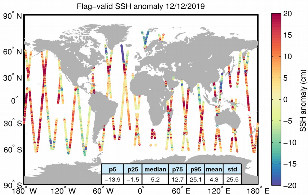
Figure 5. Geographical distribution of flag-valid 1-Hz SSH anomaly data over oceans and lakes for 12/12/2019. The statistical values shown in the table refer to the SSH anomaly in cm and are calculated over all measurements shown in the figure.
