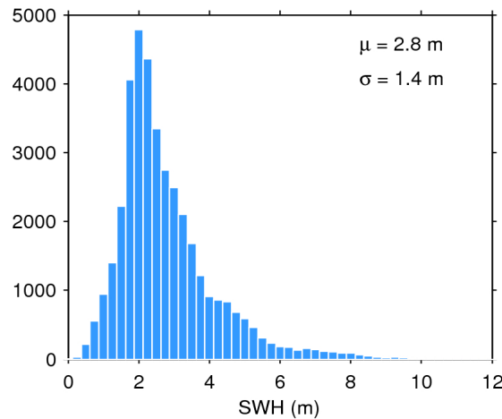
Figure 20. Histogram of science-valid SWH over oceans and lakes for 12/12/2019. The mean ( \mu ) and standard deviation ( \sigma ) are also shown. Note that values larger than 12 m are excluded from the histogram for the sake of readability but not from the computation of \mu and \sigma .
