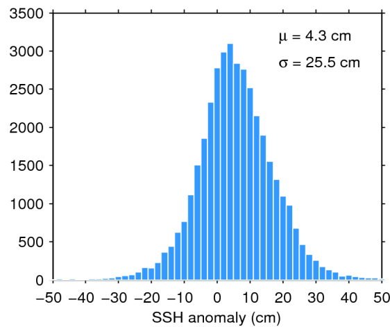
Figure 7. Histogram of flag-valid SSH anomaly over oceans and lakes for 12/12/2019. The mean ( \mu ) and standard deviation ( \sigma ) are also shown. Note that values outside [-50 50] cm are excluded from the histogram for the sake of readability but not from the computation of \mu and \sigma .
