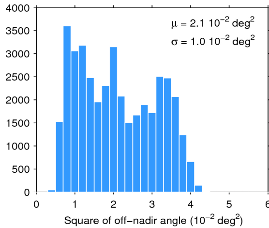
Figure 39. Histogram of flag-valid mispointing over oceans and lakes for 12/12/2019. The mean ( \mu ) and standard deviation ( \sigma ) are also shown. Note that values larger than 6 \cdot 10^{-2} \text{ deg}^2 are excluded from the histogram for the sake of readability but not from the computation of \mu and \sigma .
