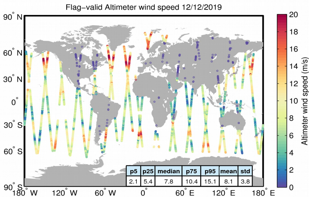
Figure 31. Geographical distribution of flag-valid wind data over oceans and lakes for 12/12/2019. The statistical values shown in the table refer to the wind in m/s and are calculated over all measurements shown in the figure.
