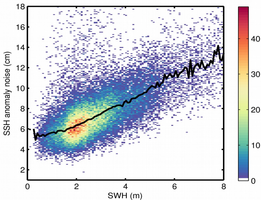
Figure 9. 2D histogram showing flag-valid SSH anomaly noise as a function of SWH for 12/12/2019. The black line denotes the median SSH anomaly noise as a function of SWH.
