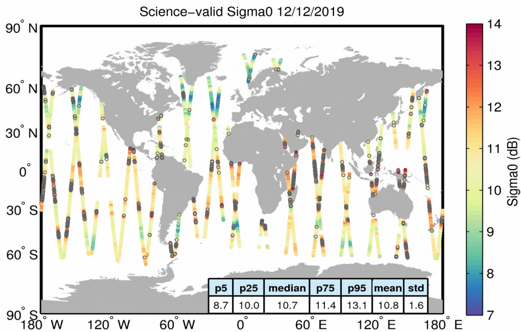
Figure 27. Geographical distribution of science-valid sigma0 data over oceans and lakes for 12/12/2019. The statistical values shown in the table refer to the sigma0 in dB and are calculated over all measurements shown in the figure. Gray circles denote records that have been rejected based on the editing criteria described in Table 4.
