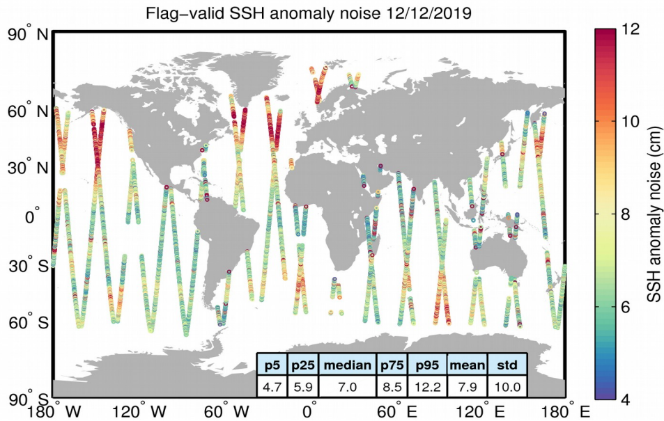
Figure 8. Geographical distribution of flag-valid 20-Hz SSH anomaly measurement noise over oceans and lakes for 12/12/2019. The statistical values shown in the table refer to the SSH anomaly noise and are calculated over all measurements shown in the figure.
