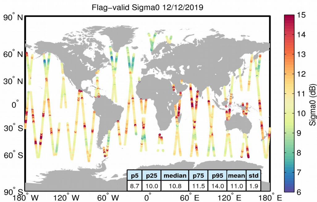
Figure 23. Geographical distribution of flag-valid sigma0 data over oceans and lakes for 12/12/2019. The statistical values shown in the table refer to the sigma0 in dB and are calculated over all measurements shown in the figure.
