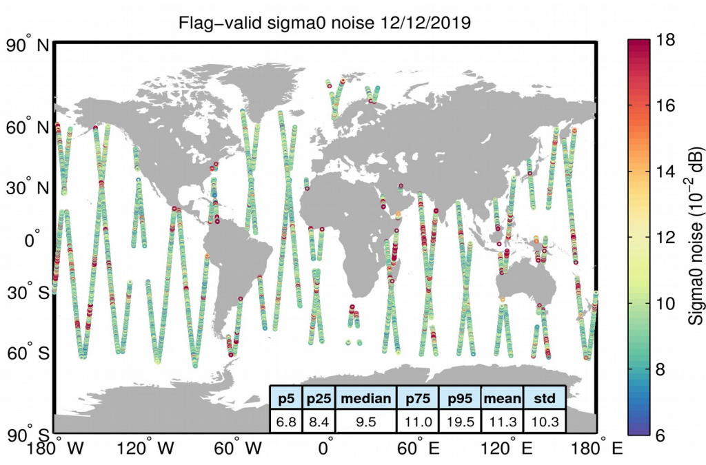
Figure 26. Geographical distribution of flag-valid 20-Hz sigma0 measurement noise over oceans and lakes for 12/12/2019. The statistical values shown in the table refer to the sigma0 noise and are calculated over all measurements shown in the figure.
