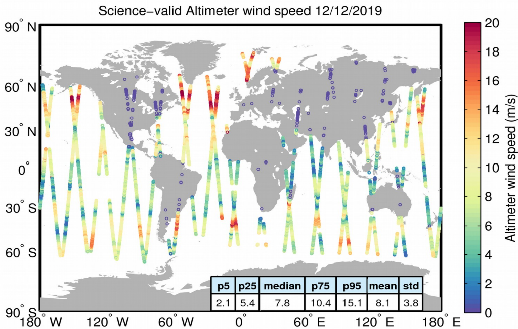
Figure 34. Geographical distribution of science-valid wind data over oceans and lakes for 12/12/2019. The statistical values shown in the table refer to the wind in m/s and are calculated over all measurements shown in the figure. Gray circles denote records that have been rejected based on the editing criteria described in Table 5.
