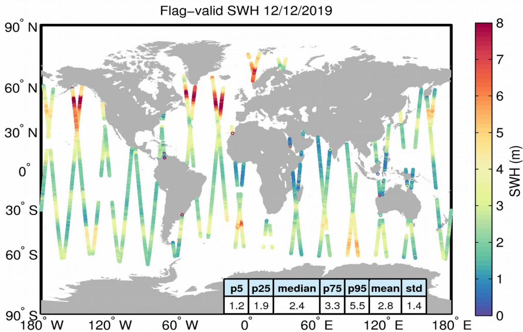
Figure 15. Geographical distribution of flag-valid SWH data over oceans and lakes for 12/12/2019. The statistical values shown in the table refer to the SWH in m and are calculated over all measurements shown in the figure.
