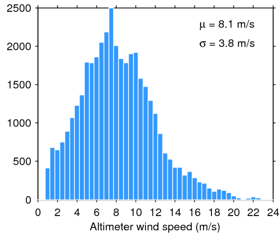
Figure 33. Histogram of flag-valid wind over oceans and lakes for 12/12/2019. The mean ( \mu ) and standard deviation ( \sigma ) are also shown. Note that values larger than 24 m/s are excluded from the histogram for the sake of readability but not from the computation of \mu and \sigma .
