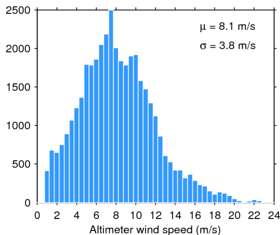
Figure 35. Histogram of science-valid wind over oceans and lakes for 12/12/2019. The mean ( \mu ) and standard deviation ( \sigma ) are also shown. Note that values larger than 24 m/s are excluded from the histogram for the sake of readability but not from the computation of \mu and \sigma .
