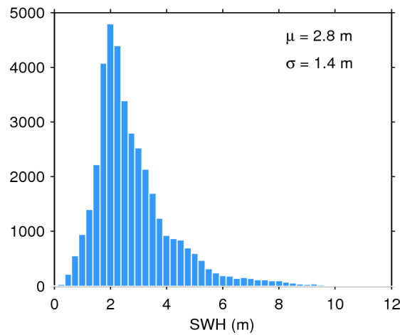
Figure 17. Histogram of flag-valid SWH over oceans and lakes for 12/12/2019. The mean ( \mu ) and standard deviation ( \sigma ) are also shown. Note that values larger than 12 m are excluded from the histogram for the sake of readability but not from the computation of \mu and \sigma .
