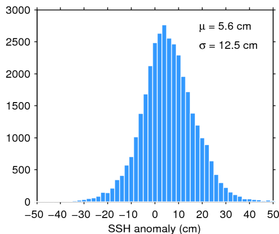
Figure 11. Histogram of science-valid SSH anomaly over oceans and lakes for 12/12/2019. The mean ( \mu ) and standard deviation ( \sigma ) are also shown. Note that values outside [-50 50] cm are excluded from the histogram for the sake of readability but not from the computation of \mu and \sigma .
