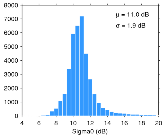
Figure 25. Histogram of flag-valid sigma0 over oceans and lakes for 12/12/2019. The mean ( \mu ) and standard deviation ( \sigma ) are also shown. Note that values outside [4 20] dB are excluded from the histogram for the sake of readability but not from the computation of \mu and \sigma .
