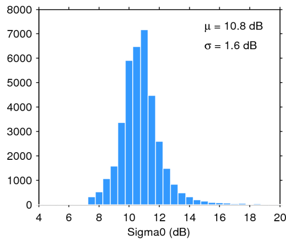
Figure 28. Histogram of science-valid sigma0 over oceans and lakes for 12/12/2019. The mean ( \mu ) and standard deviation ( \sigma ) are also shown. Note that values outside [4 20] dB are excluded from the histogram for the sake of readability but not from the computation of \mu and \sigma .
