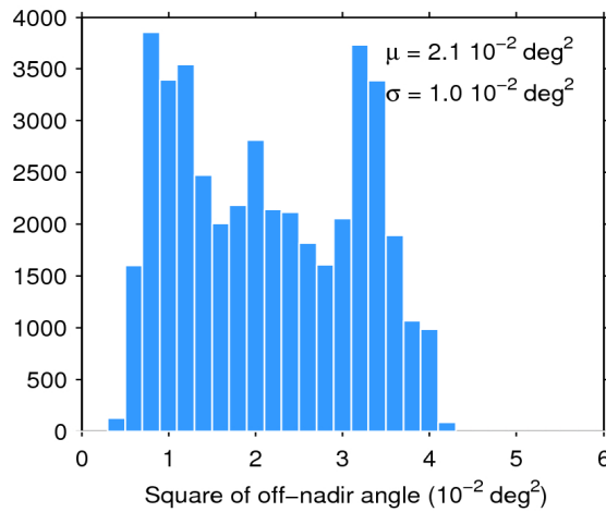
Figure 39. Histogram of flag-valid mispointing over oceans and lakes for 11/12/2019. The mean ( \mu ) and standard deviation ( \sigma ) are also shown. Note that values larger than 6 \cdot 10^{-2} \text{ deg}^2 are excluded from the histogram for the sake of readability but not from the computation of \mu and \sigma .
