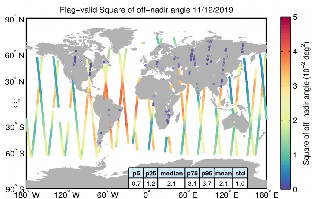
Figure 37. Geographical distribution of flag-valid mispointing data over oceans and lakes for 11/12/2019. The statistical values shown in the table refer to the mispointing in 10^{-2} \text{ deg}^2 and are calculated over all measurements shown in the figure.
