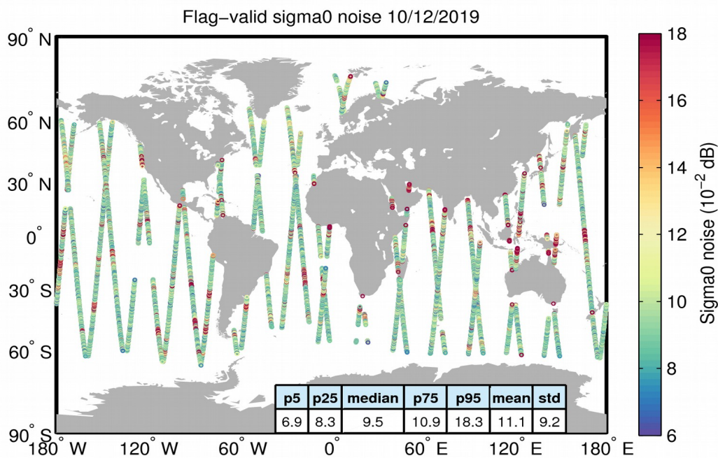
Figure 26. Geographical distribution of flag-valid 20-Hz sigma0 measurement noise over oceans and lakes for 10/12/2019. The statistical values shown in the table refer to the sigma0 noise and are calculated over all measurements shown in the figure.
