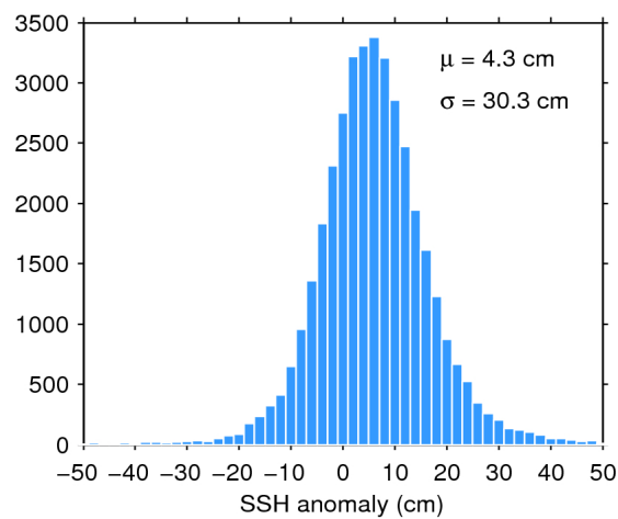
Figure 7. Histogram of flag-valid SSH anomaly over oceans and lakes for 10/12/2019. The mean ( \mu ) and standard deviation ( \sigma ) are also shown. Note that values outside [-50 \ 50] cm are excluded from the histogram for the sake of readability but not from the computation of \mu and \sigma .
