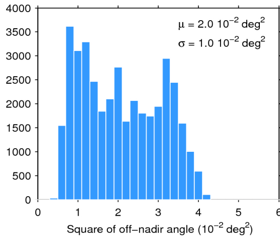
Figure 39. Histogram of flag-valid mispointing over oceans and lakes for 10/12/2019. The mean ( \mu ) and standard deviation ( \sigma ) are also shown. Note that values larger than 6 \cdot 10^{-2} \text{ deg}^2 are excluded from the histogram for the sake of readability but not from the computation of \mu and \sigma .
