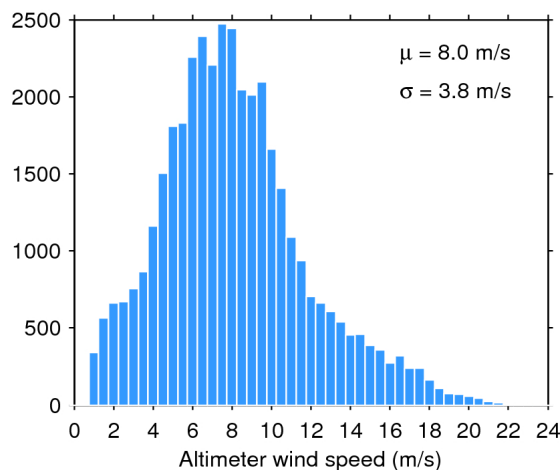
Figure 35. Histogram of science-valid wind over oceans and lakes for 10/12/2019. The mean ( \mu ) and standard deviation ( \sigma ) are also shown. Note that values larger than 24 m/s are excluded from the histogram for the sake of readability but not from the computation of \mu and \sigma .
