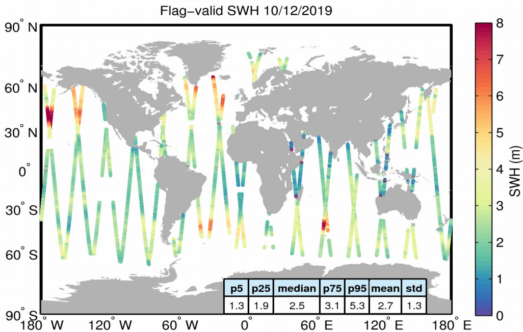
Figure 15. Geographical distribution of flag-valid SWH data over oceans and lakes for 10/12/2019. The statistical values shown in the table refer to the SWH in m and are calculated over all measurements shown in the figure.
