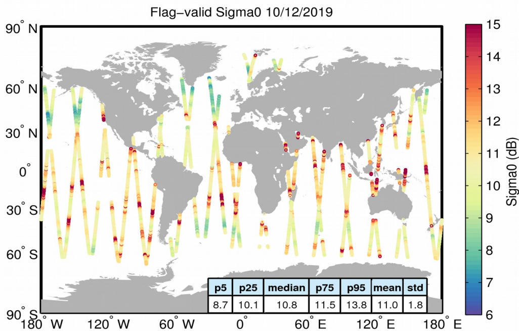
Figure 23. Geographical distribution of flag-valid sigma0 data over oceans and lakes for 10/12/2019. The statistical values shown in the table refer to the sigma0 in dB and are calculated over all measurements shown in the figure.
