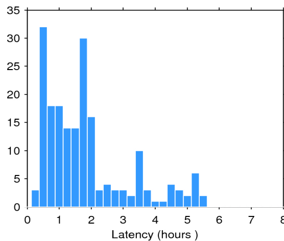
Figure 2. Histogram of the data latency for 10/12/2019. The y-axis denotes the number of files that are made available with a delay of x-hours with respect to the mean time of the records stored in the file.
