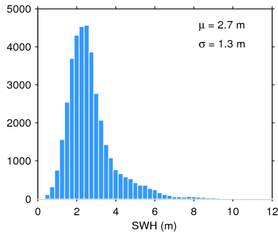
Figure 17. Histogram of flag-valid SWH over oceans and lakes for 10/12/2019. The mean ( \mu ) and standard deviation ( \sigma ) are also shown. Note that values larger than 12 m are excluded from the histogram for the sake of readability but not from the computation of \mu and \sigma .
