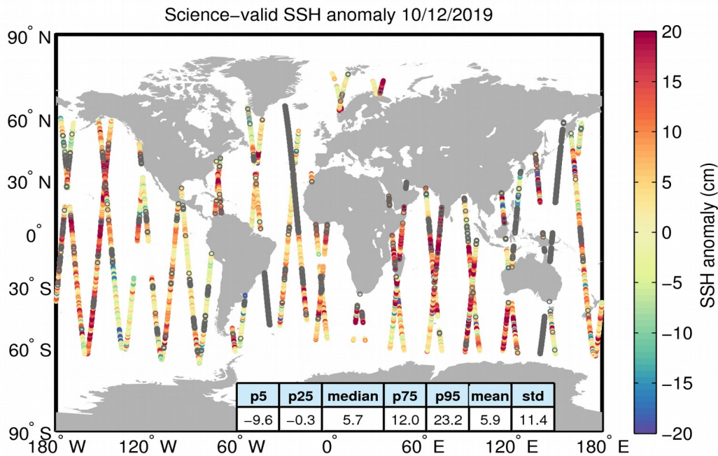
Figure 10. Geographical distribution of science-valid SSH anomaly data over oceans and lakes for 10/12/2019. The statistical values shown in the table refer to the SSH anomaly in cm and are calculated over all measurements shown in the figure. Gray circles denote records that have been rejected based on the editing criteria described in Table 2.
