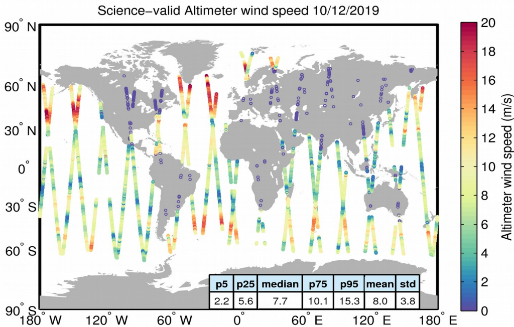
Figure 34. Geographical distribution of science-valid wind data over oceans and lakes for 10/12/2019. The statistical values shown in the table refer to the wind in m/s and are calculated over all measurements shown in the figure. Gray circles denote records that have been rejected based on the editing criteria described in Table 5.
