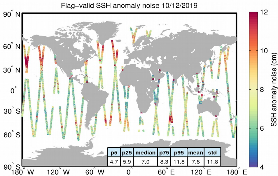
Figure 8. Geographical distribution of flag-valid 20-Hz SSH anomaly measurement noise over oceans and lakes for 10/12/2019. The statistical values shown in the table refer to the SSH anomaly noise and are calculated over all measurements shown in the figure.
