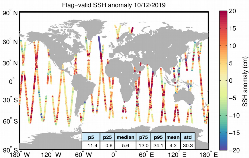
Figure 5. Geographical distribution of flag-valid 1-Hz SSH anomaly data over oceans and lakes for 10/12/2019. The statistical values shown in the table refer to the SSH anomaly in cm and are calculated over all measurements shown in the figure.
