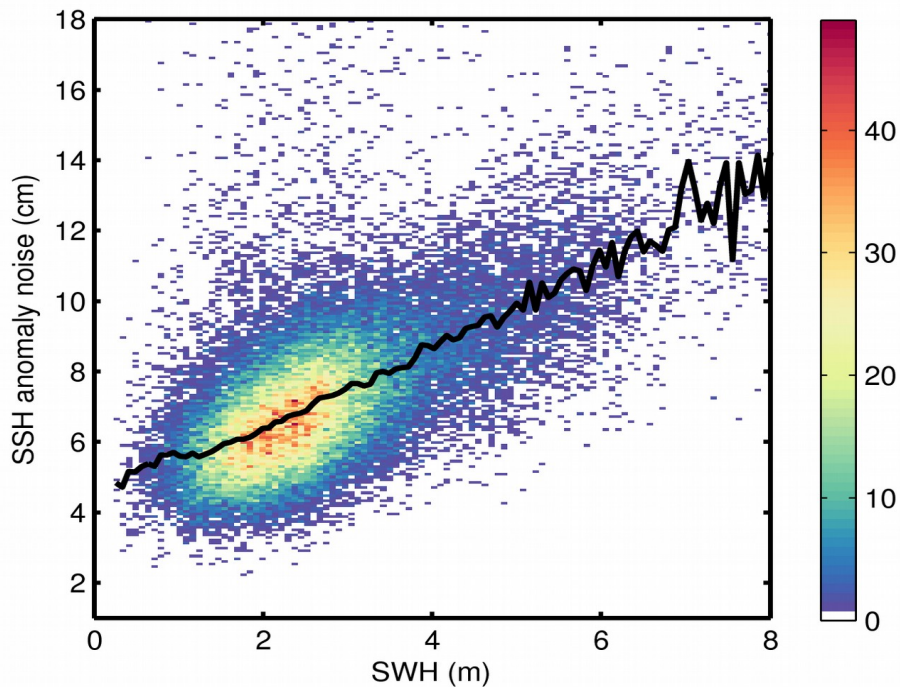
Figure 9. 2D histogram showing flag-valid SSH anomaly noise as a function of SWH for 10/12/2019. The black line denotes the median SSH anomaly noise as a function of SWH.
