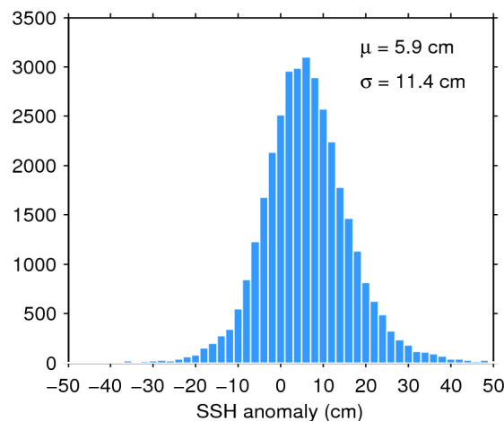
Figure 11. Histogram of science-valid SSH anomaly over oceans and lakes for 10/12/2019. The mean ( \mu ) and standard deviation ( \sigma ) are also shown. Note that values outside [-50 50] cm are excluded from the histogram for the sake of readability but not from the computation of \mu and \sigma .
