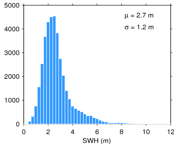
Figure 20. Histogram of science-valid SWH over oceans and lakes for 10/12/2019. The mean ( \mu ) and standard deviation ( \sigma ) are also shown. Note that values larger than 12 m are excluded from the histogram for the sake of readability but not from the computation of \mu and \sigma .
