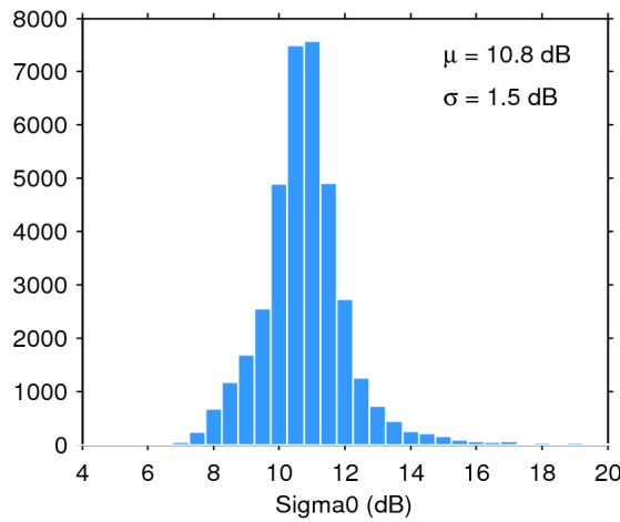
Figure 28. Histogram of science-valid sigma0 over oceans and lakes for 10/12/2019. The mean ( \mu ) and standard deviation ( \sigma ) are also shown. Note that values outside [4 20] dB are excluded from the histogram for the sake of readability but not from the computation of \mu and \sigma .
