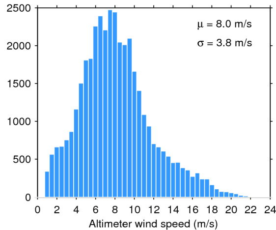
Figure 33. Histogram of flag-valid wind over oceans and lakes for 10/12/2019. The mean ( \mu ) and standard deviation ( \sigma ) are also shown. Note that values larger than 24 m/s are excluded from the histogram for the sake of readability but not from the computation of \mu and \sigma .
