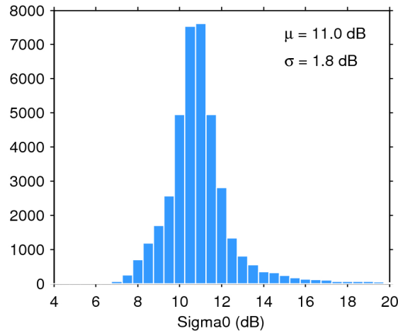
Figure 25. Histogram of flag-valid sigma0 over oceans and lakes for 10/12/2019. The mean ( \mu ) and standard deviation ( \sigma ) are also shown. Note that values outside [4 20] dB are excluded from the histogram for the sake of readability but not from the computation of \mu and \sigma .
