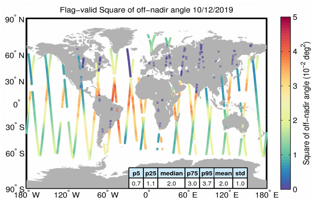
Figure 37. Geographical distribution of flag-valid mispointing data over oceans and lakes for 10/12/2019. The statistical values shown in the table refer to the mispointing in 10^{-2} deg 2 and are calculated over all measurements shown in the figure.
