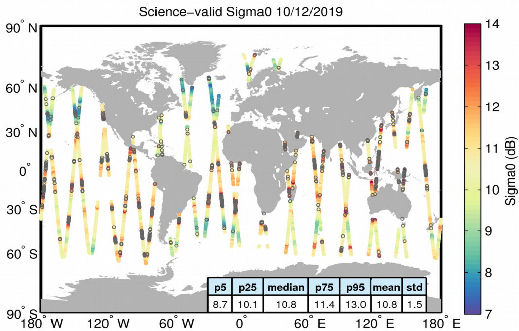
Figure 27. Geographical distribution of science-valid sigma0 data over oceans and lakes for 10/12/2019. The statistical values shown in the table refer to the sigma0 in dB and are calculated over all measurements shown in the figure. Gray circles denote records that have been rejected based on the editing criteria described in Table 4.
