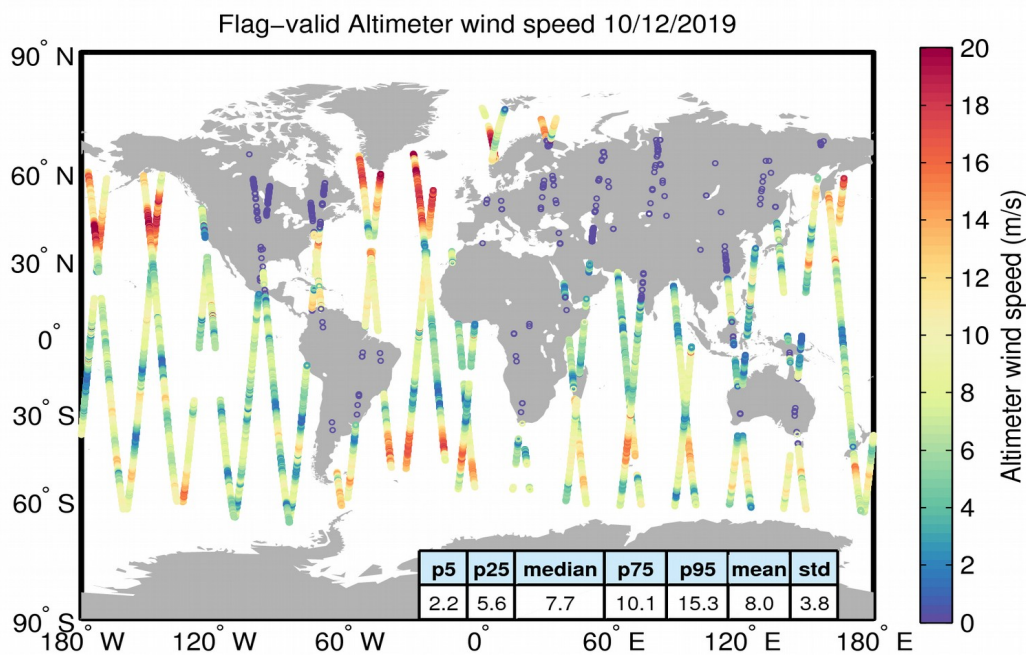
Figure 31. Geographical distribution of flag-valid wind data over oceans and lakes for 10/12/2019. The statistical values shown in the table refer to the wind in m/s and are calculated over all measurements shown in the figure.
