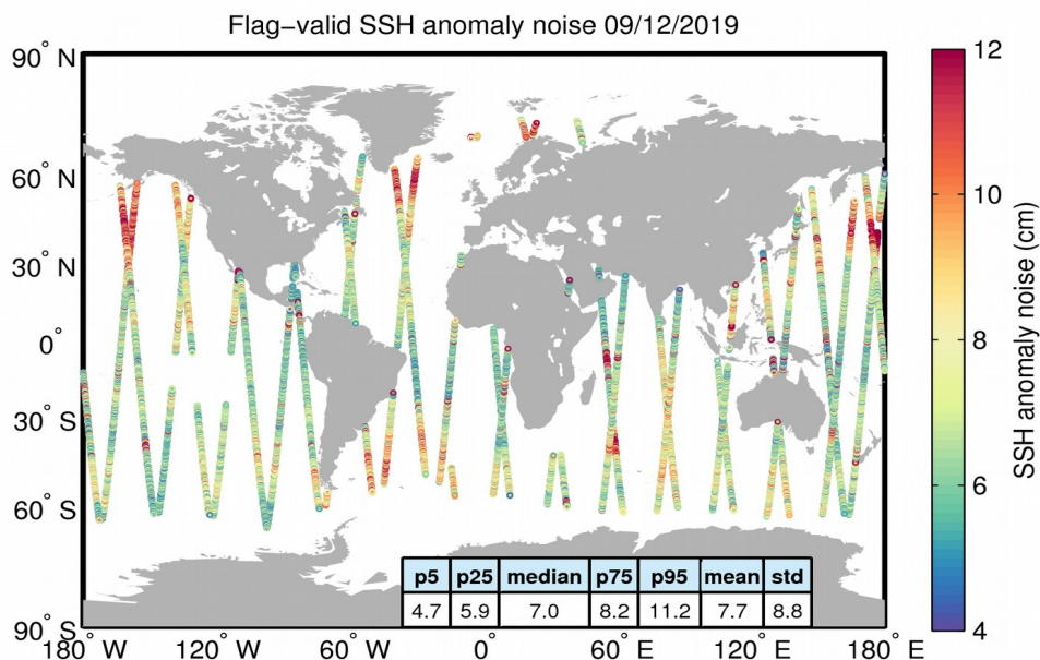
Figure 8. Geographical distribution of flag-valid 20-Hz SSH anomaly measurement noise over oceans and lakes for 09/12/2019. The statistical values shown in the table refer to the SSH anomaly noise and are calculated over all measurements shown in the figure.
