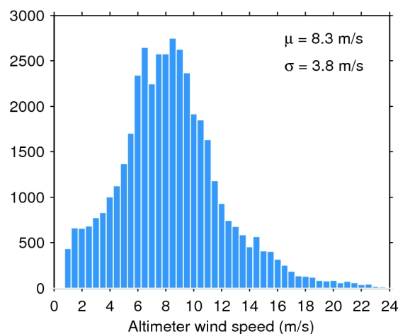
Figure 35. Histogram of science-valid wind over oceans and lakes for 09/12/2019. The mean ( \mu ) and standard deviation ( \sigma ) are also shown. Note that values larger than 24 m/s are excluded from the histogram for the sake of readability but not from the computation of \mu and \sigma .
