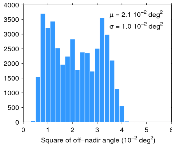
Figure 39. Histogram of flag-valid mispointing over oceans and lakes for 09/12/2019. The mean ( \mu ) and standard deviation ( \sigma ) are also shown. Note that values larger than 6 \cdot 10^{-2} \text{ deg}^2 are excluded from the histogram for the sake of readability but not from the computation of \mu and \sigma .
