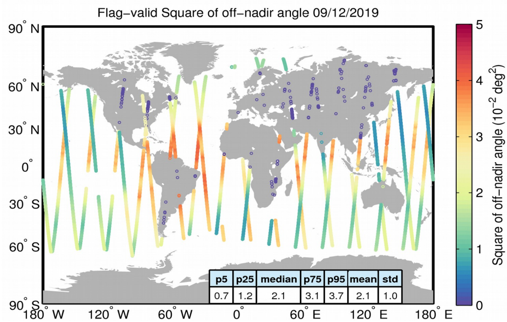
Figure 37. Geographical distribution of flag-valid mispointing data over oceans and lakes for 09/12/2019. The statistical values shown in the table refer to the mispointing in 10^{-2} \text{ deg}^2 and are calculated over all measurements shown in the figure.
