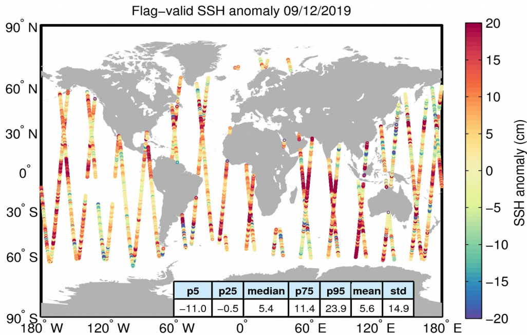
Figure 5. Geographical distribution of flag-valid 1-Hz SSH anomaly data over oceans and lakes for 09/12/2019. The statistical values shown in the table refer to the SSH anomaly in cm and are calculated over all measurements shown in the figure.
