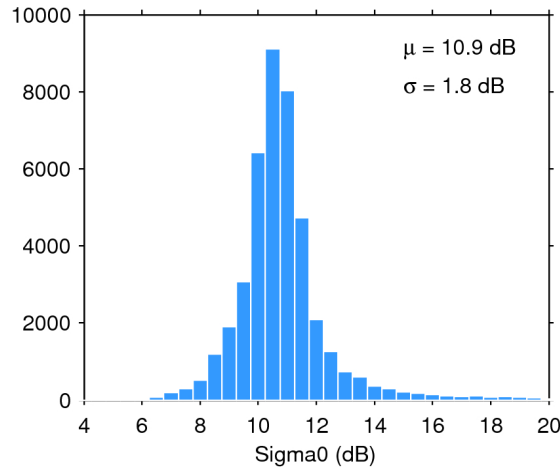
Figure 25. Histogram of flag-valid sigma0 over oceans and lakes for 09/12/2019. The mean ( \mu ) and standard deviation ( \sigma ) are also shown. Note that values outside [4 20] dB are excluded from the histogram for the sake of readability but not from the computation of \mu and \sigma .
