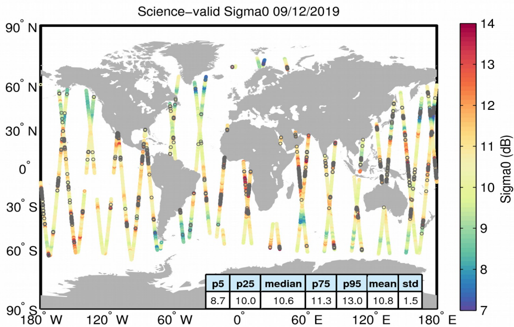
Figure 27. Geographical distribution of science-valid sigma0 data over oceans and lakes for 09/12/2019. The statistical values shown in the table refer to the sigma0 in dB and are calculated over all measurements shown in the figure. Gray circles denote records that have been rejected based on the editing criteria described in Table 4.
