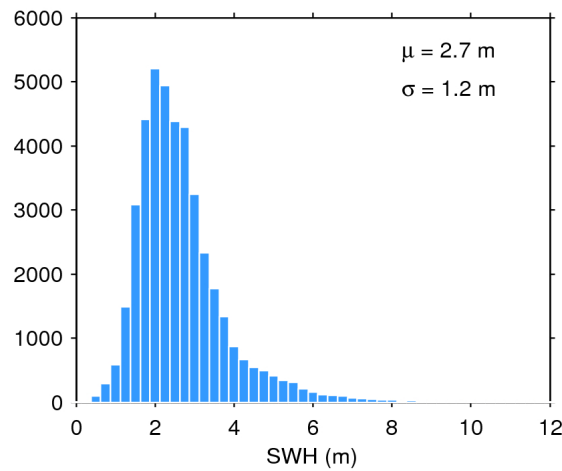
Figure 17. Histogram of flag-valid SWH over oceans and lakes for 09/12/2019. The mean ( \mu ) and standard deviation ( \sigma ) are also shown. Note that values larger than 12 m are excluded from the histogram for the sake of readability but not from the computation of \mu and \sigma .
