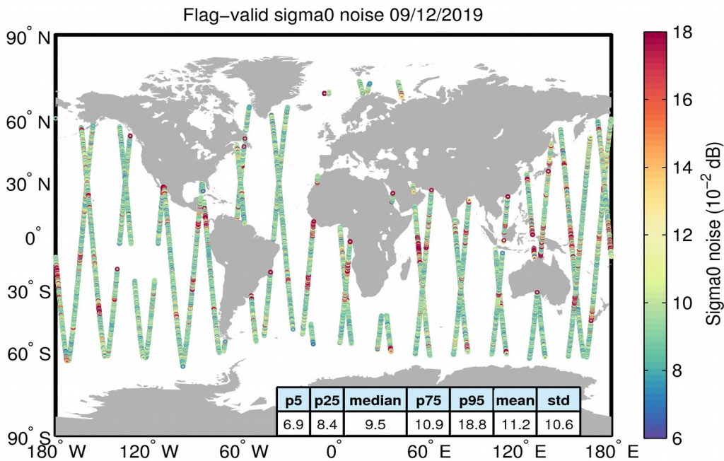
Figure 26. Geographical distribution of flag-valid 20-Hz sigma0 measurement noise over oceans and lakes for 09/12/2019. The statistical values shown in the table refer to the sigma0 noise and are calculated over all measurements shown in the figure.
