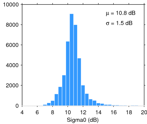
Figure 28. Histogram of science-valid sigma0 over oceans and lakes for 09/12/2019. The mean ( \mu ) and standard deviation ( \sigma ) are also shown. Note that values outside [4 20] dB are excluded from the histogram for the sake of readability but not from the computation of \mu and \sigma .
