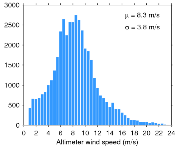
Figure 33. Histogram of flag-valid wind over oceans and lakes for 09/12/2019. The mean ( \mu ) and standard deviation ( \sigma ) are also shown. Note that values larger than 24 m/s are excluded from the histogram for the sake of readability but not from the computation of \mu and \sigma .
