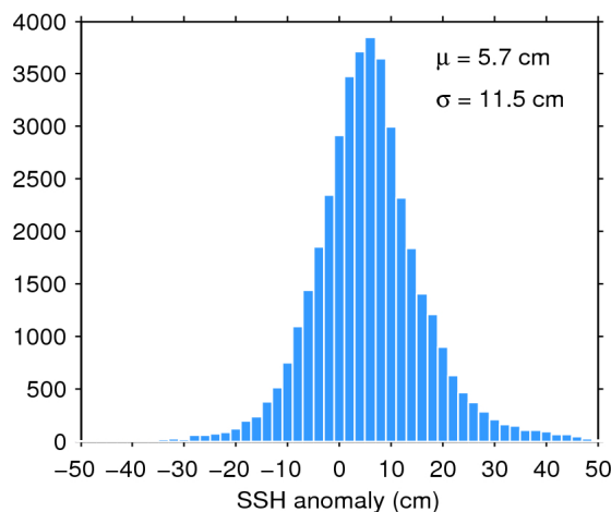
Figure 11. Histogram of science-valid SSH anomaly over oceans and lakes for 09/12/2019. The mean ( \mu ) and standard deviation ( \sigma ) are also shown. Note that values outside [-50 50] cm are excluded from the histogram for the sake of readability but not from the computation of \mu and \sigma .
