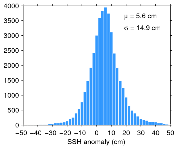
Figure 7. Histogram of flag-valid SSH anomaly over oceans and lakes for 09/12/2019. The mean ( \mu ) and standard deviation ( \sigma ) are also shown. Note that values outside [-50\ 50] cm are excluded from the histogram for the sake of readability but not from the computation of \mu and \sigma .
