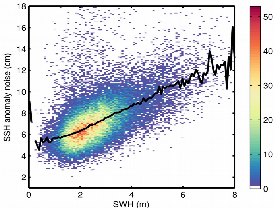
Figure 9. 2D histogram showing flag-valid SSH anomaly noise as a function of SWH for 09/12/2019. The black line denotes the median SSH anomaly noise as a function of SWH.
