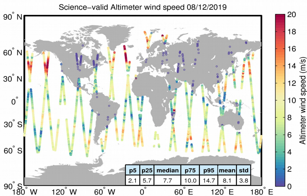
Figure 34. Geographical distribution of science-valid wind data over oceans and lakes for 08/12/2019. The statistical values shown in the table refer to the wind in m/s and are calculated over all measurements shown in the figure. Gray circles denote records that have been rejected based on the editing criteria described in Table 5.
