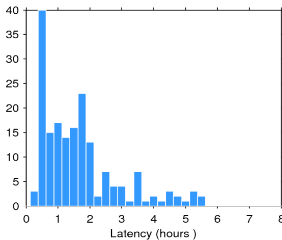
Figure 2. Histogram of the data latency for 08/12/2019. The y-axis denotes the number of files that are made available with a delay of x-hours with respect to the mean time of the records stored in the file.
