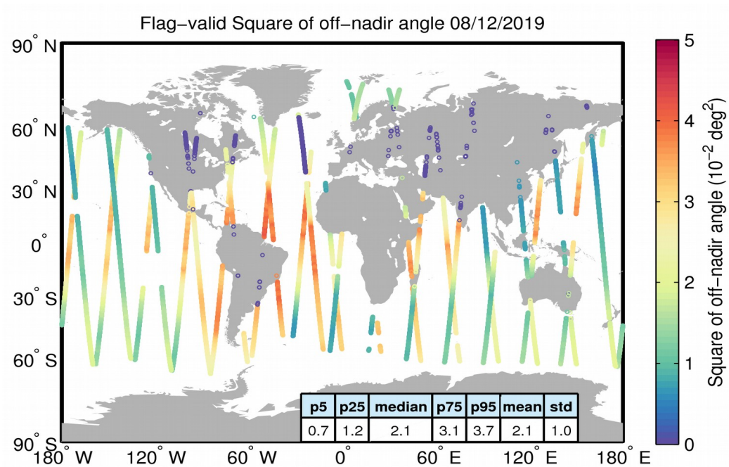
Figure 37. Geographical distribution of flag-valid mispointing data over oceans and lakes for 08/12/2019. The statistical values shown in the table refer to the mispointing in 10^{-2} \text{ deg}^2 and are calculated over all measurements shown in the figure.
