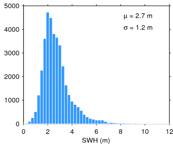
Figure 20. Histogram of science-valid SWH over oceans and lakes for 08/12/2019. The mean ( \mu ) and standard deviation ( \sigma ) are also shown. Note that values larger than 12 m are excluded from the histogram for the sake of readability but not from the computation of \mu and \sigma .
