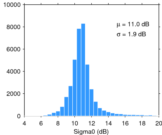
Figure 25. Histogram of flag-valid sigma0 over oceans and lakes for 08/12/2019. The mean ( \mu ) and standard deviation ( \sigma ) are also shown. Note that values outside [4 20] dB are excluded from the histogram for the sake of readability but not from the computation of \mu and \sigma .
