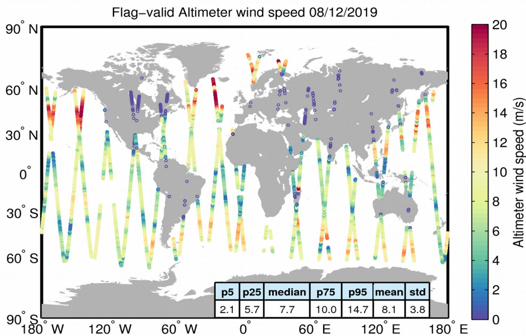
Figure 31. Geographical distribution of flag-valid wind data over oceans and lakes for 08/12/2019. The statistical values shown in the table refer to the wind in m/s and are calculated over all measurements shown in the figure.
