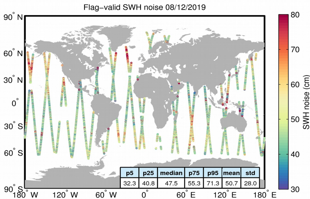
Figure 18. Geographical distribution of flag-valid 20-Hz SWH measurement noise over oceans and lakes for 08/12/2019. The statistical values shown in the figure refer to the SWH noise and are calculated over all measurements shown in the figure.
