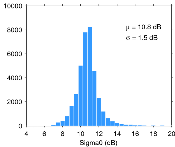
Figure 28. Histogram of science-valid sigma0 over oceans and lakes for 08/12/2019. The mean ( \mu ) and standard deviation ( \sigma ) are also shown. Note that values outside [4 20] dB are excluded from the histogram for the sake of readability but not from the computation of \mu and \sigma .
