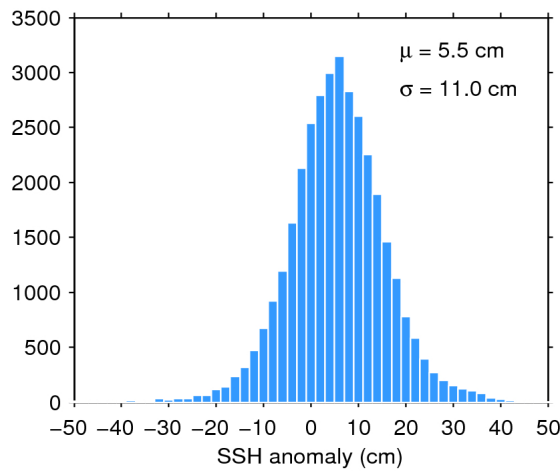
Figure 11. Histogram of science-valid SSH anomaly over oceans and lakes for 08/12/2019. The mean ( \mu ) and standard deviation ( \sigma ) are also shown. Note that values outside [-50 50] cm are excluded from the histogram for the sake of readability but not from the computation of \mu and \sigma .
