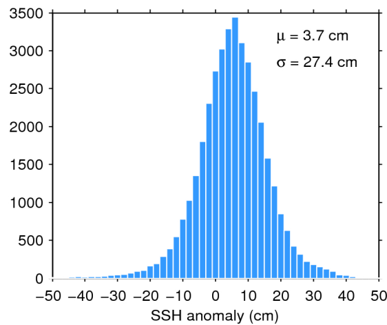
Figure 7. Histogram of flag-valid SSH anomaly over oceans and lakes for 08/12/2019. The mean ( \mu ) and standard deviation ( \sigma ) are also shown. Note that values outside [-50\ 50] cm are excluded from the histogram for the sake of readability but not from the computation of \mu and \sigma .
