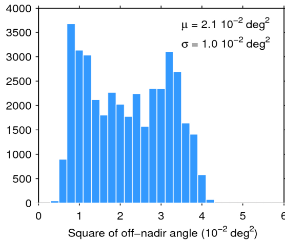
Figure 39. Histogram of flag-valid mispointing over oceans and lakes for 08/12/2019. The mean ( \mu ) and standard deviation ( \sigma ) are also shown. Note that values larger than 6 \cdot 10^{-2} \text{ deg}^2 are excluded from the histogram for the sake of readability but not from the computation of \mu and \sigma .
