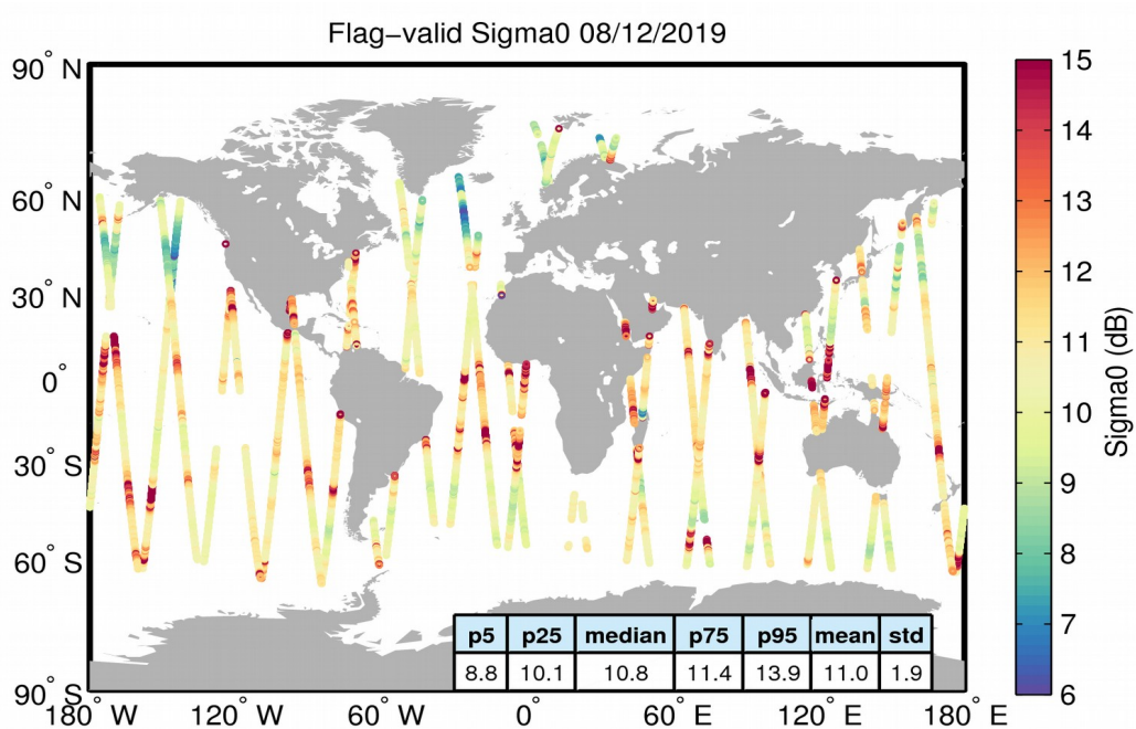
Figure 23. Geographical distribution of flag-valid sigma0 data over oceans and lakes for 08/12/2019. The statistical values shown in the table refer to the sigma0 in dB and are calculated over all measurements shown in the figure.
