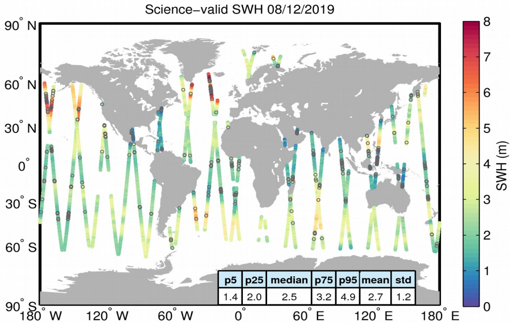
Figure 19. Geographical distribution of science-valid SWH data over oceans and lakes for 08/12/2019. The statistical values shown in the table refer to the SWH in m and are calculated over all measurements shown in the figure. Gray circles denote records that have been rejected based on the editing criteria described in Table 3.
