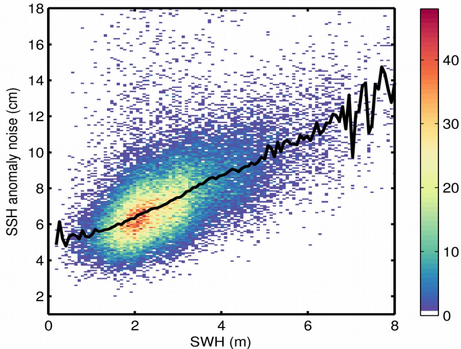
Figure 9. 2D histogram showing flag-valid SSH anomaly noise as a function of SWH for 08/12/2019. The black line denotes the median SSH anomaly noise as a function of SWH.
