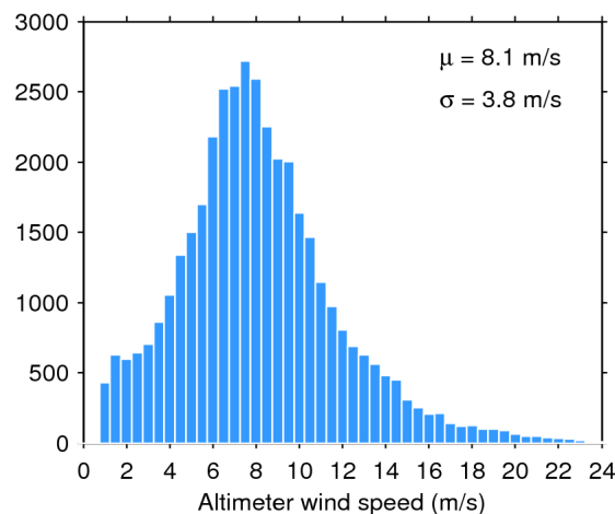
Figure 35. Histogram of science-valid wind over oceans and lakes for 08/12/2019. The mean ( \mu ) and standard deviation ( \sigma ) are also shown. Note that values larger than 24 m/s are excluded from the histogram for the sake of readability but not from the computation of \mu and \sigma .
