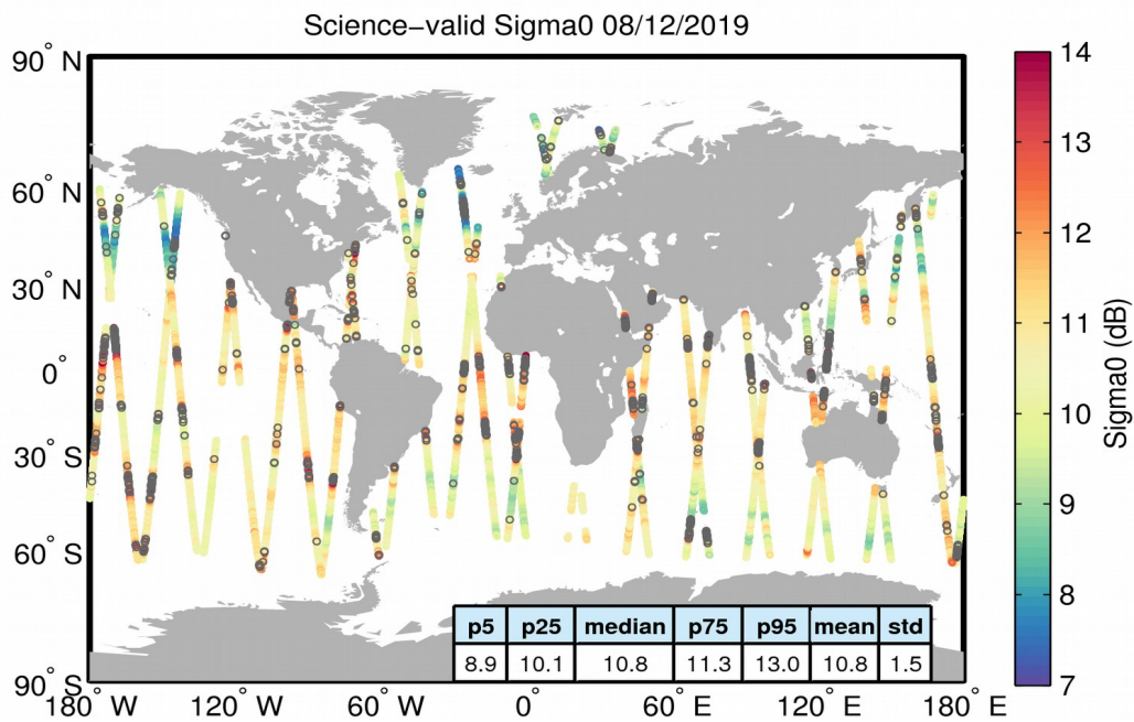
Figure 27. Geographical distribution of science-valid sigma0 data over oceans and lakes for 08/12/2019. The statistical values shown in the table refer to the sigma0 in dB and are calculated over all measurements shown in the figure. Gray circles denote records that have been rejected based on the editing criteria described in Table 4.
