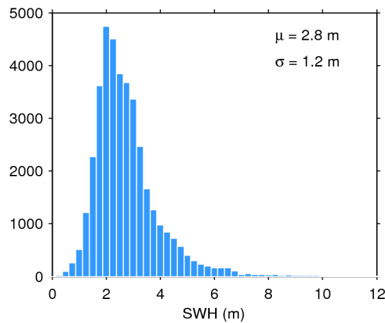
Figure 17. Histogram of flag-valid SWH over oceans and lakes for 08/12/2019. The mean ( \mu ) and standard deviation ( \sigma ) are also shown. Note that values larger than 12 m are excluded from the histogram for the sake of readability but not from the computation of \mu and \sigma .
