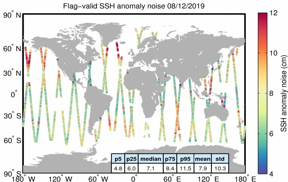
Figure 8. Geographical distribution of flag-valid 20-Hz SSH anomaly measurement noise over oceans and lakes for 08/12/2019. The statistical values shown in the table refer to the SSH anomaly noise and are calculated over all measurements shown in the figure.
