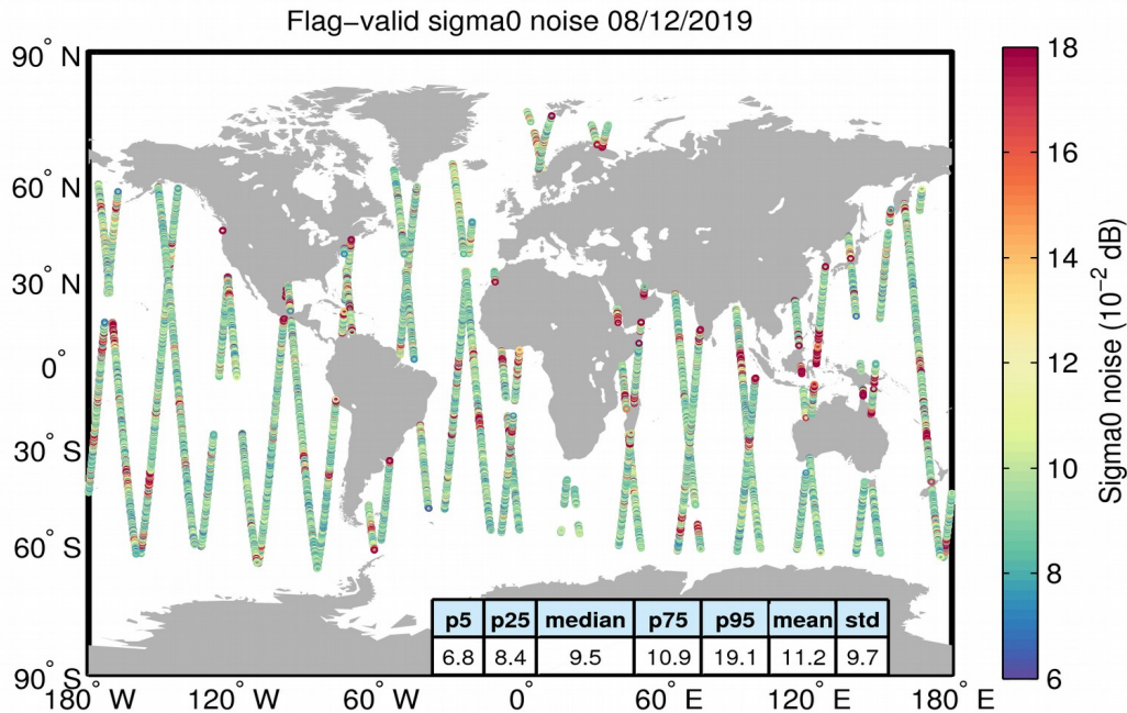
Figure 26. Geographical distribution of flag-valid 20-Hz sigma0 measurement noise over oceans and lakes for 08/12/2019. The statistical values shown in the table refer to the sigma0 noise and are calculated over all measurements shown in the figure.
