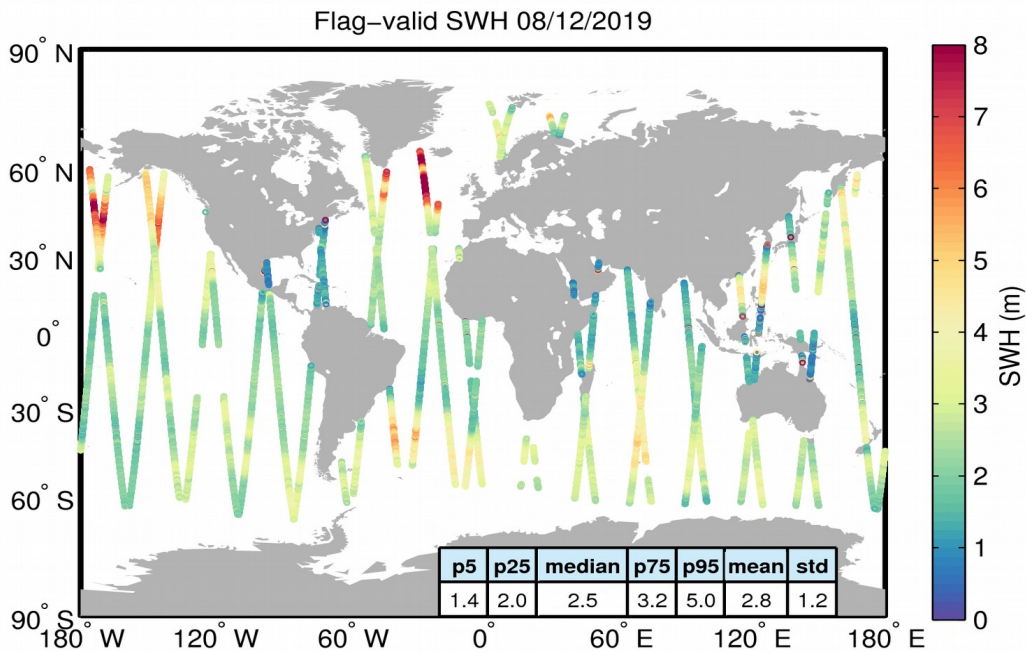
Figure 15. Geographical distribution of flag-valid SWH data over oceans and lakes for 08/12/2019. The statistical values shown in the table refer to the SWH in m and are calculated over all measurements shown in the figure.
