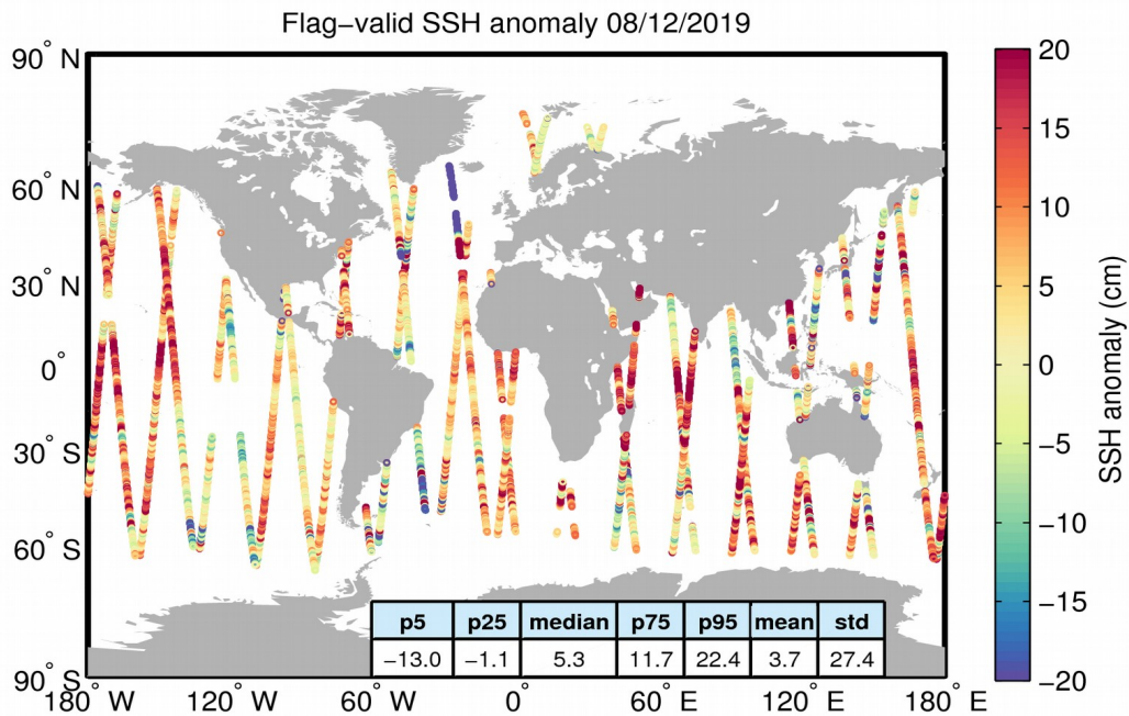
Figure 5. Geographical distribution of flag-valid 1-Hz SSH anomaly data over oceans and lakes for 08/12/2019. The statistical values shown in the table refer to the SSH anomaly in cm and are calculated over all measurements shown in the figure.
