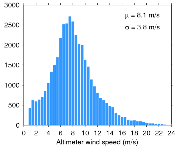
Figure 33. Histogram of flag-valid wind over oceans and lakes for 08/12/2019. The mean ( \mu ) and standard deviation ( \sigma ) are also shown. Note that values larger than 24 m/s are excluded from the histogram for the sake of readability but not from the computation of \mu and \sigma .
