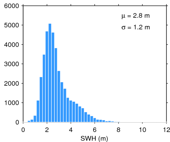
Figure 20. Histogram of science-valid SWH over oceans and lakes for 07/12/2019. The mean ( \mu ) and standard deviation ( \sigma ) are also shown. Note that values larger than 12 m are excluded from the histogram for the sake of readability but not from the computation of \mu and \sigma .
