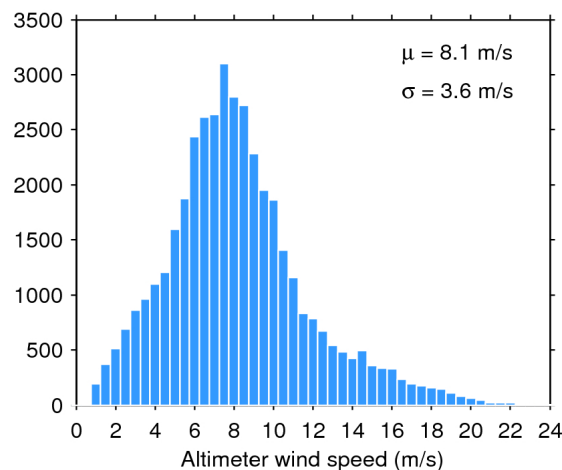
Figure 35. Histogram of science-valid wind over oceans and lakes for 07/12/2019. The mean ( \mu ) and standard deviation ( \sigma ) are also shown. Note that values larger than 24 m/s are excluded from the histogram for the sake of readability but not from the computation of \mu and \sigma .
