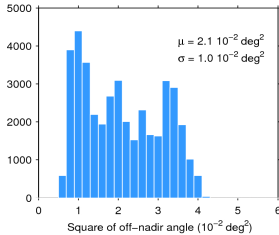
Figure 39. Histogram of flag-valid mispointing over oceans and lakes for 07/12/2019. The mean ( \mu ) and standard deviation ( \sigma ) are also shown. Note that values larger than 6 \cdot 10^{-2} \text{ deg}^2 are excluded from the histogram for the sake of readability but not from the computation of \mu and \sigma .
