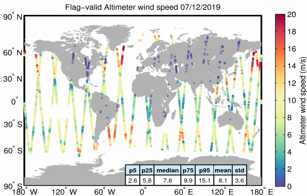
Figure 31. Geographical distribution of flag-valid wind data over oceans and lakes for 07/12/2019. The statistical values shown in the table refer to the wind in m/s and are calculated over all measurements shown in the figure.
