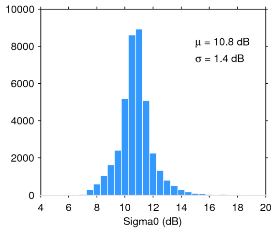
Figure 28. Histogram of science-valid sigma0 over oceans and lakes for 07/12/2019. The mean ( \mu ) and standard deviation ( \sigma ) are also shown. Note that values outside [4 20] dB are excluded from the histogram for the sake of readability but not from the computation of \mu and \sigma .
