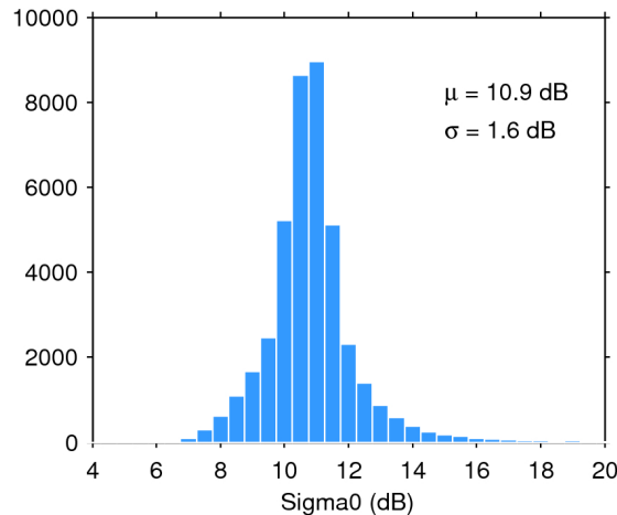
Figure 25. Histogram of flag-valid sigma0 over oceans and lakes for 07/12/2019. The mean ( \mu ) and standard deviation ( \sigma ) are also shown. Note that values outside [4 20] dB are excluded from the histogram for the sake of readability but not from the computation of \mu and \sigma .
