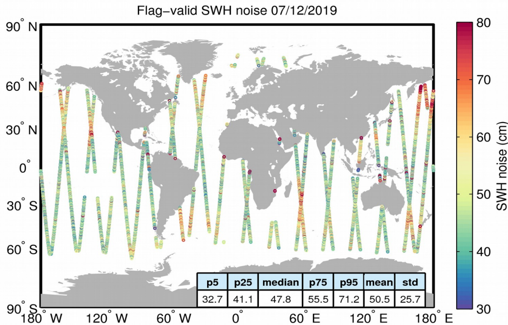
Figure 18. Geographical distribution of flag-valid 20-Hz SWH measurement noise over oceans and lakes for 07/12/2019. The statistical values shown in the figure refer to the SWH noise and are calculated over all measurements shown in the figure.
