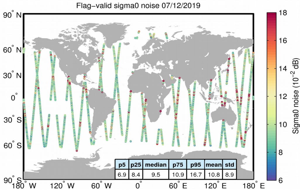
Figure 26. Geographical distribution of flag-valid 20-Hz sigma0 measurement noise over oceans and lakes for 07/12/2019. The statistical values shown in the table refer to the sigma0 noise and are calculated over all measurements shown in the figure.
