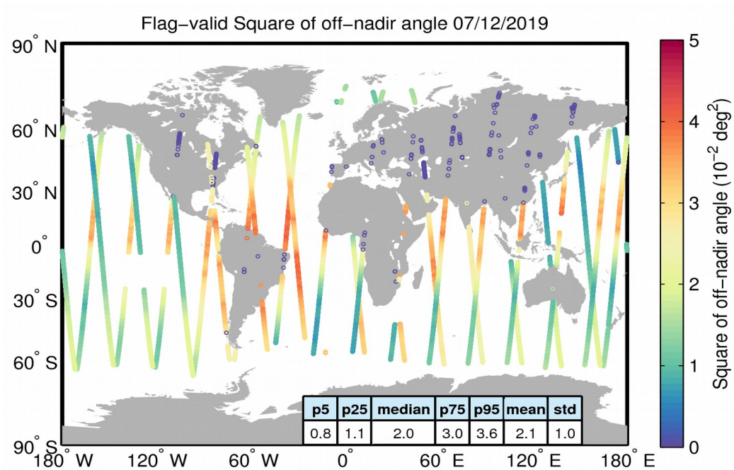
Figure 37. Geographical distribution of flag-valid mispointing data over oceans and lakes for 07/12/2019. The statistical values shown in the table refer to the mispointing in 10^{-2} \text{ deg}^2 and are calculated over all measurements shown in the figure.
