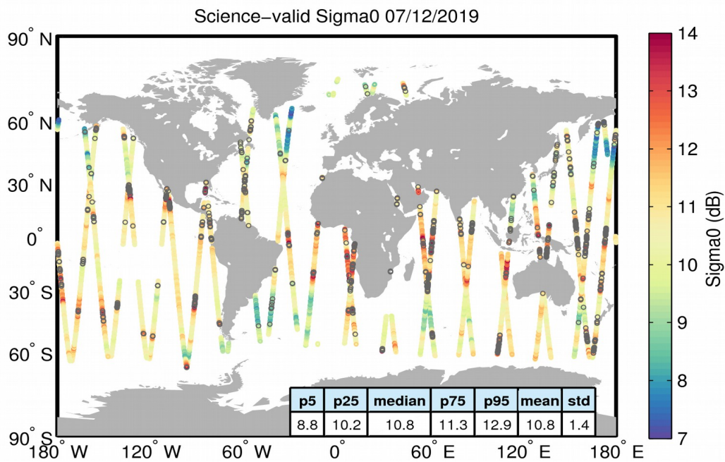
Figure 27. Geographical distribution of science-valid sigma0 data over oceans and lakes for 07/12/2019. The statistical values shown in the table refer to the sigma0 in dB and are calculated over all measurements shown in the figure. Gray circles denote records that have been rejected based on the editing criteria described in Table 4.
