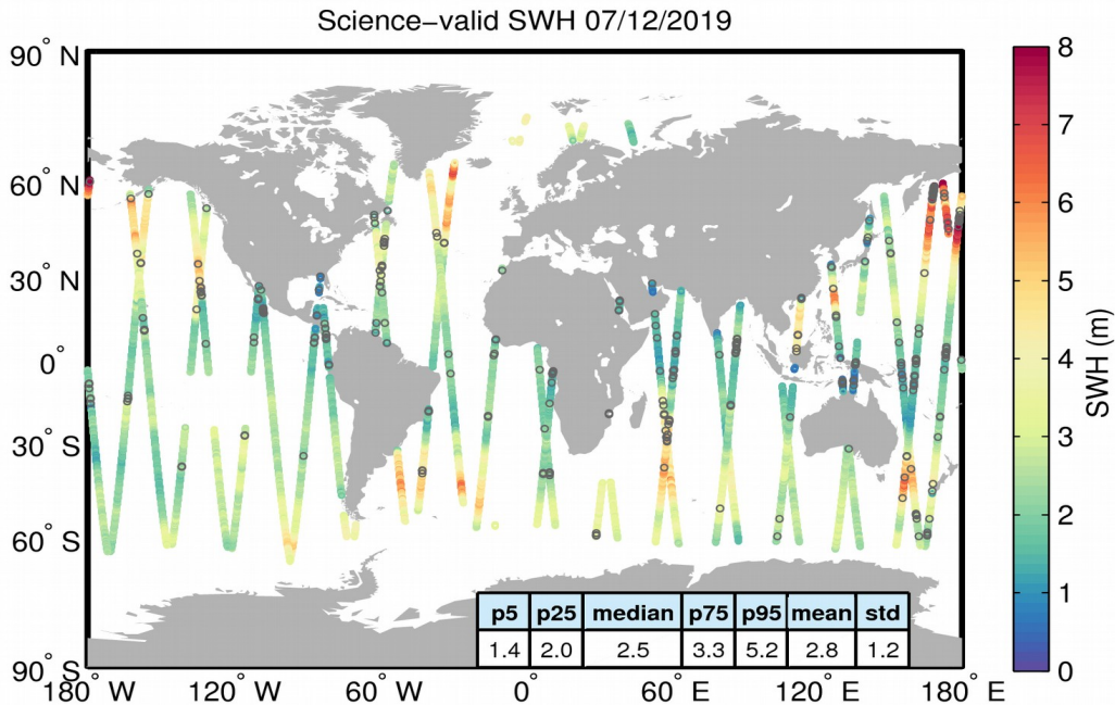
Figure 19. Geographical distribution of science-valid SWH data over oceans and lakes for 07/12/2019. The statistical values shown in the table refer to the SWH in m and are calculated over all measurements shown in the figure. Gray circles denote records that have been rejected based on the editing criteria described in Table 3.
