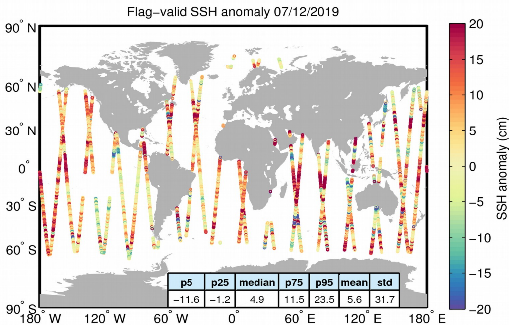
Figure 5. Geographical distribution of flag-valid 1-Hz SSH anomaly data over oceans and lakes for 07/12/2019. The statistical values shown in the table refer to the SSH anomaly in cm and are calculated over all measurements shown in the figure.
