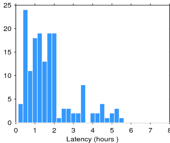
Figure 2. Histogram of the data latency for 07/12/2019. The y-axis denotes the number of files that are made available with a delay of x-hours with respect to the mean time of the records stored in the file.
