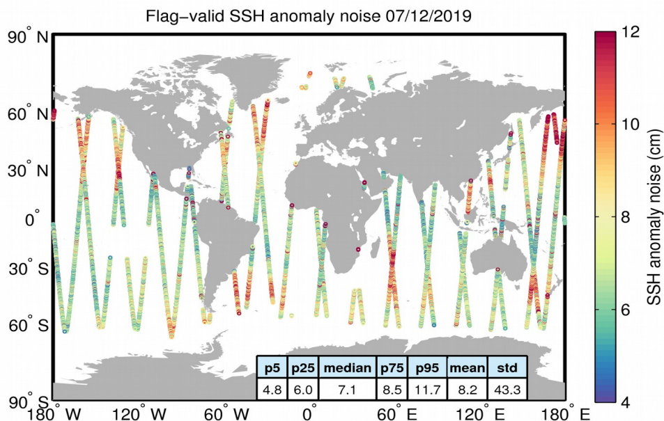
Figure 8. Geographical distribution of flag-valid 20-Hz SSH anomaly measurement noise over oceans and lakes for 07/12/2019. The statistical values shown in the table refer to the SSH anomaly noise and are calculated over all measurements shown in the figure.
