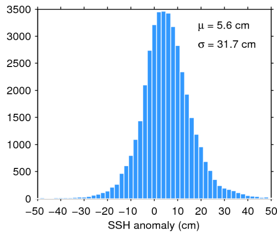
Figure 7. Histogram of flag-valid SSH anomaly over oceans and lakes for 07/12/2019. The mean ( \mu ) and standard deviation ( \sigma ) are also shown. Note that values outside [-50\ 50] cm are excluded from the histogram for the sake of readability but not from the computation of \mu and \sigma .
