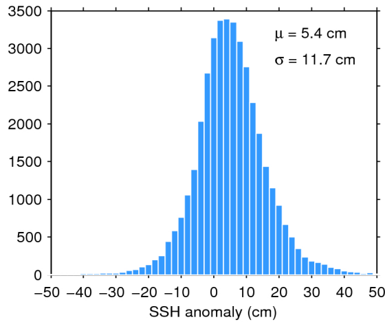
Figure 11. Histogram of science-valid SSH anomaly over oceans and lakes for 07/12/2019. The mean ( \mu ) and standard deviation ( \sigma ) are also shown. Note that values outside [-50 50] cm are excluded from the histogram for the sake of readability but not from the computation of \mu and \sigma .
