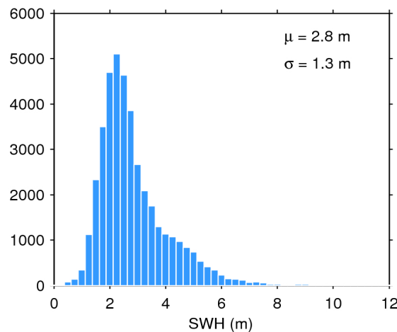
Figure 17. Histogram of flag-valid SWH over oceans and lakes for 07/12/2019. The mean ( \mu ) and standard deviation ( \sigma ) are also shown. Note that values larger than 12 m are excluded from the histogram for the sake of readability but not from the computation of \mu and \sigma .
