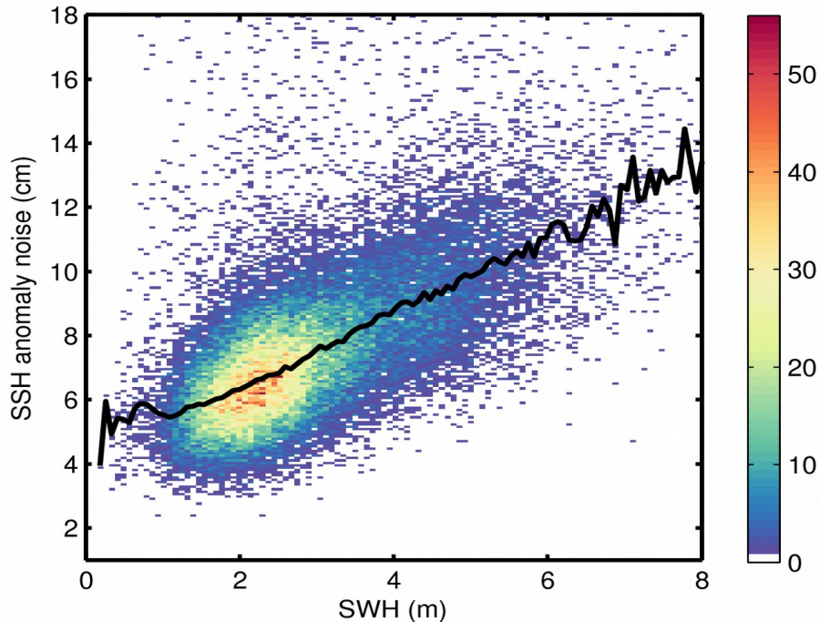
Figure 9. 2D histogram showing flag-valid SSH anomaly noise as a function of SWH for 07/12/2019. The black line denotes the median SSH anomaly noise as a function of SWH.
