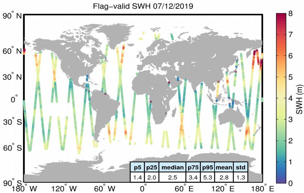
Figure 15. Geographical distribution of flag-valid SWH data over oceans and lakes for 07/12/2019. The statistical values shown in the table refer to the SWH in m and are calculated over all measurements shown in the figure.
