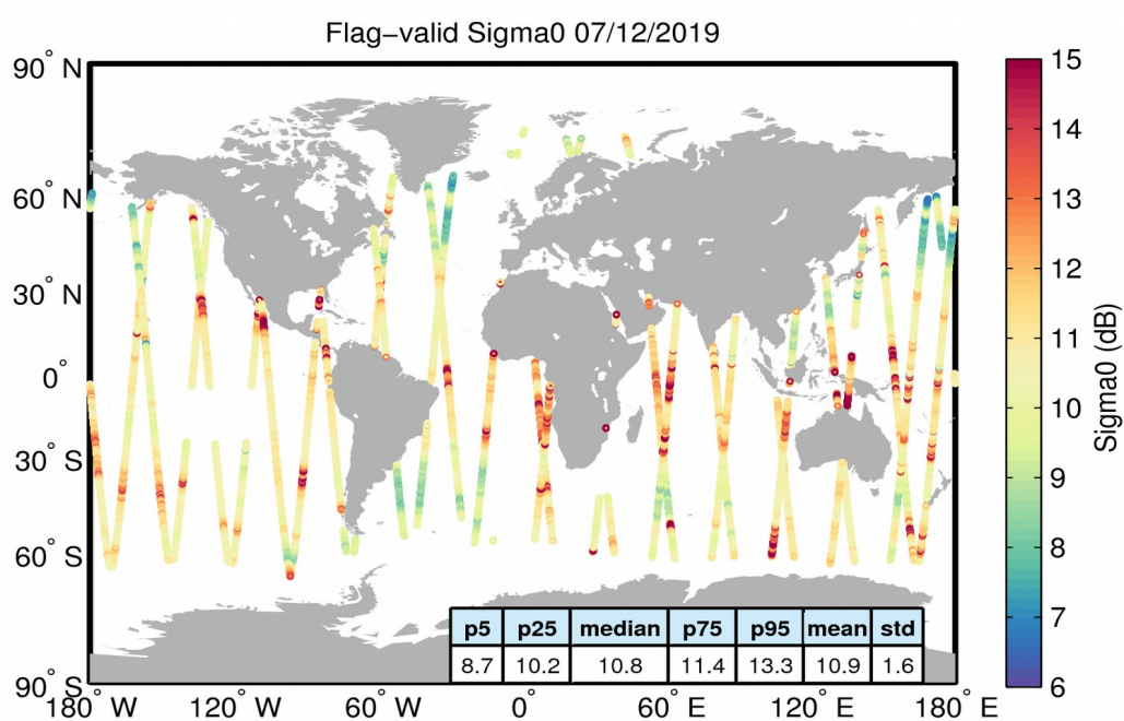
Figure 23. Geographical distribution of flag-valid sigma0 data over oceans and lakes for 07/12/2019. The statistical values shown in the table refer to the sigma0 in dB and are calculated over all measurements shown in the figure.
