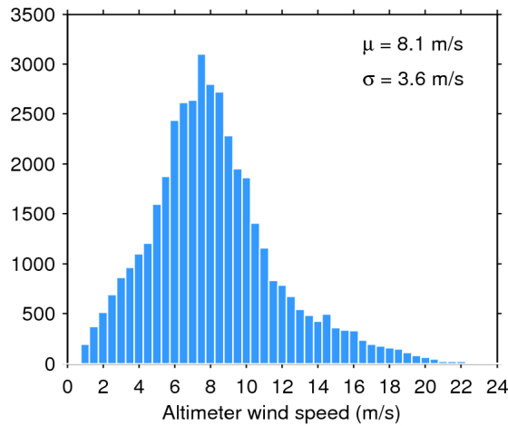
Figure 33. Histogram of flag-valid wind over oceans and lakes for 07/12/2019. The mean ( \mu ) and standard deviation ( \sigma ) are also shown. Note that values larger than 24 m/s are excluded from the histogram for the sake of readability but not from the computation of \mu and \sigma .
