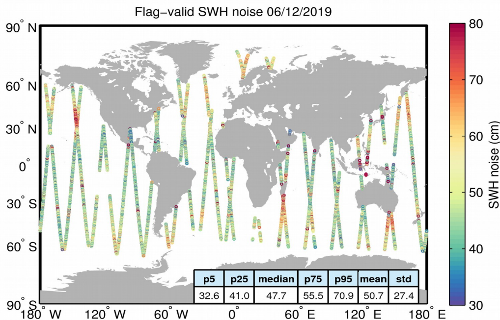
Figure 18. Geographical distribution of flag-valid 20-Hz SWH measurement noise over oceans and lakes for 06/12/2019. The statistical values shown in the figure refer to the SWH noise and are calculated over all measurements shown in the figure.
