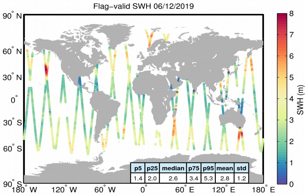
Figure 15. Geographical distribution of flag-valid SWH data over oceans and lakes for 06/12/2019. The statistical values shown in the table refer to the SWH in m and are calculated over all measurements shown in the figure.
