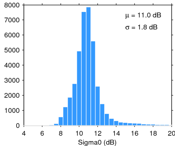
Figure 25. Histogram of flag-valid sigma0 over oceans and lakes for 06/12/2019. The mean ( \mu ) and standard deviation ( \sigma ) are also shown. Note that values outside [4 20] dB are excluded from the histogram for the sake of readability but not from the computation of \mu and \sigma .
