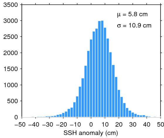
Figure 11. Histogram of science-valid SSH anomaly over oceans and lakes for 06/12/2019. The mean ( \mu ) and standard deviation ( \sigma ) are also shown. Note that values outside [-50 50] cm are excluded from the histogram for the sake of readability but not from the computation of \mu and \sigma .
