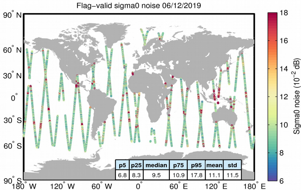
Figure 26. Geographical distribution of flag-valid 20-Hz sigma0 measurement noise over oceans and lakes for 06/12/2019. The statistical values shown in the table refer to the sigma0 noise and are calculated over all measurements shown in the figure.
