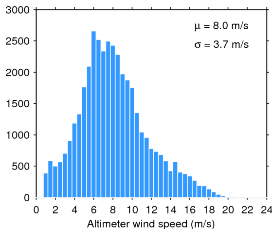
Figure 35. Histogram of science-valid wind over oceans and lakes for 06/12/2019. The mean ( \mu ) and standard deviation ( \sigma ) are also shown. Note that values larger than 24 m/s are excluded from the histogram for the sake of readability but not from the computation of \mu and \sigma .
