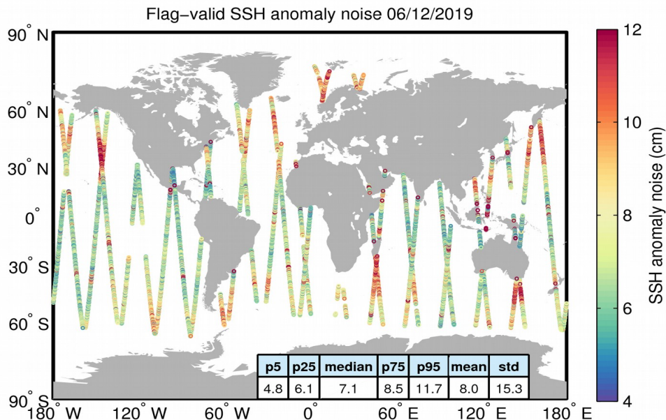
Figure 8. Geographical distribution of flag-valid 20-Hz SSH anomaly measurement noise over oceans and lakes for 06/12/2019. The statistical values shown in the table refer to the SSH anomaly noise and are calculated over all measurements shown in the figure.
