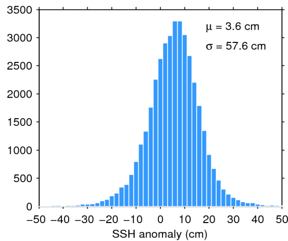
Figure 7. Histogram of flag-valid SSH anomaly over oceans and lakes for 06/12/2019. The mean ( \mu ) and standard deviation ( \sigma ) are also shown. Note that values outside [-50\ 50] cm are excluded from the histogram for the sake of readability but not from the computation of \mu and \sigma .
