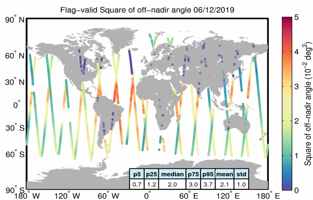
Figure 37. Geographical distribution of flag-valid mispointing data over oceans and lakes for 06/12/2019. The statistical values shown in the table refer to the mispointing in 10^{-2} \text{ deg}^2 and are calculated over all measurements shown in the figure.
