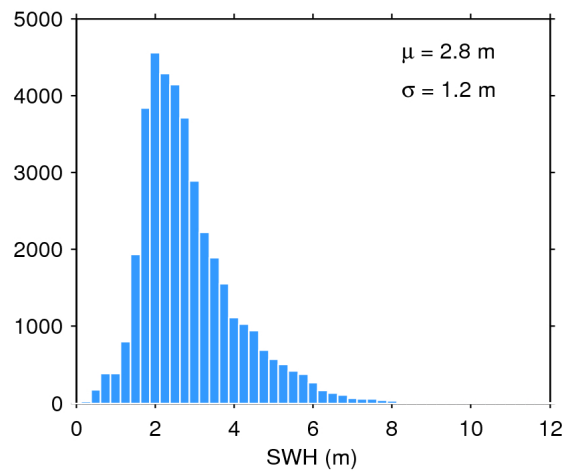
Figure 17. Histogram of flag-valid SWH over oceans and lakes for 06/12/2019. The mean ( \mu ) and standard deviation ( \sigma ) are also shown. Note that values larger than 12 m are excluded from the histogram for the sake of readability but not from the computation of \mu and \sigma .
