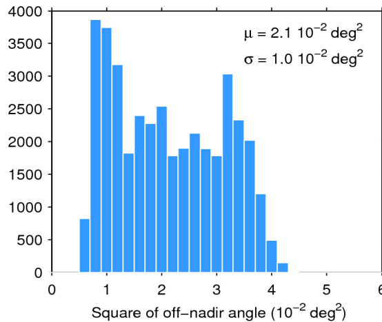
Figure 39. Histogram of flag-valid mispointing over oceans and lakes for 06/12/2019. The mean ( \mu ) and standard deviation ( \sigma ) are also shown. Note that values larger than 6 \cdot 10^{-2} \text{ deg}^2 are excluded from the histogram for the sake of readability but not from the computation of \mu and \sigma .
