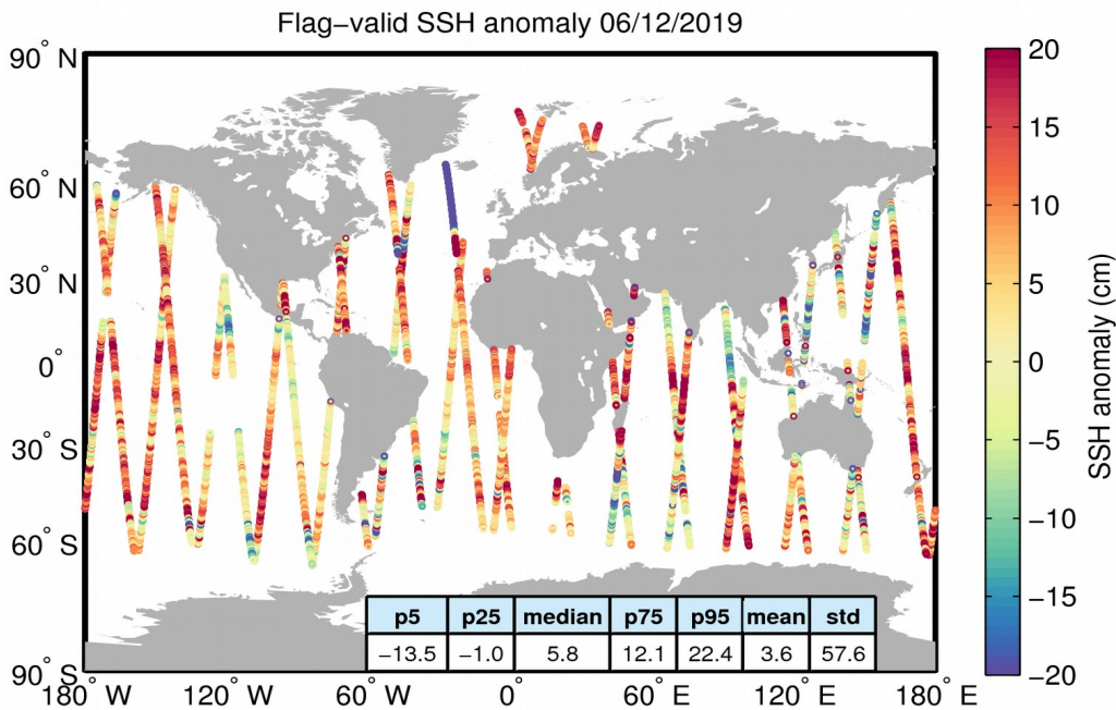
Figure 5. Geographical distribution of flag-valid 1-Hz SSH anomaly data over oceans and lakes for 06/12/2019. The statistical values shown in the table refer to the SSH anomaly in cm and are calculated over all measurements shown in the figure.
