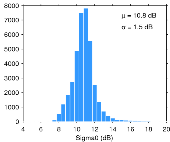
Figure 28. Histogram of science-valid sigma0 over oceans and lakes for 06/12/2019. The mean ( \mu ) and standard deviation ( \sigma ) are also shown. Note that values outside [4 20] dB are excluded from the histogram for the sake of readability but not from the computation of \mu and \sigma .
