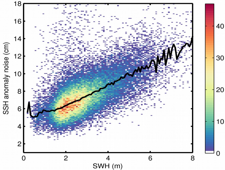
Figure 9. 2D histogram showing flag-valid SSH anomaly noise as a function of SWH for 06/12/2019. The black line denotes the median SSH anomaly noise as a function of SWH.
