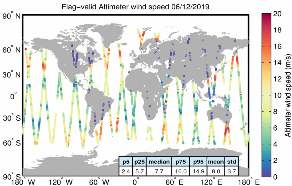
Figure 31. Geographical distribution of flag-valid wind data over oceans and lakes for 06/12/2019. The statistical values shown in the table refer to the wind in m/s and are calculated over all measurements shown in the figure.
