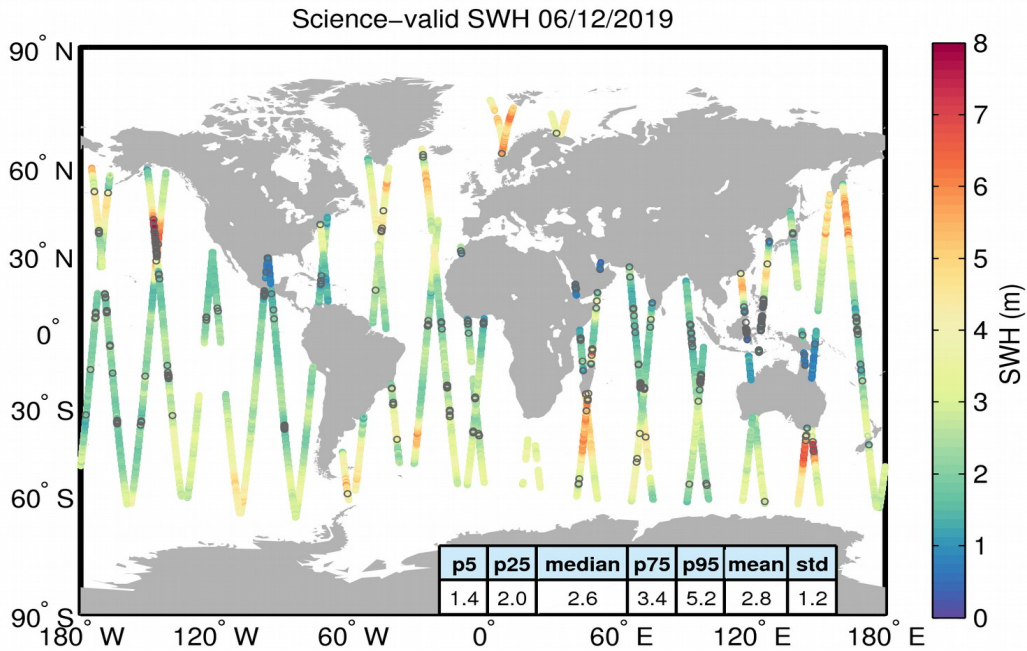
Figure 19. Geographical distribution of science-valid SWH data over oceans and lakes for 06/12/2019. The statistical values shown in the table refer to the SWH in m and are calculated over all measurements shown in the figure. Gray circles denote records that have been rejected based on the editing criteria described in Table 3.
