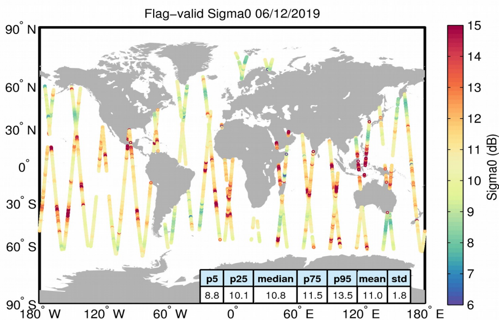
Figure 23. Geographical distribution of flag-valid sigma0 data over oceans and lakes for 06/12/2019. The statistical values shown in the table refer to the sigma0 in dB and are calculated over all measurements shown in the figure.
