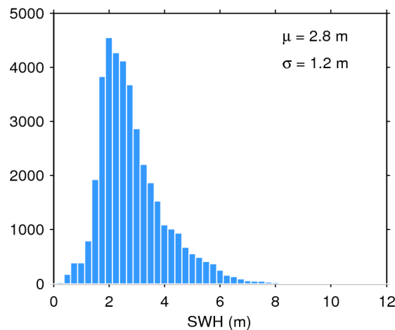
Figure 20. Histogram of science-valid SWH over oceans and lakes for 06/12/2019. The mean ( \mu ) and standard deviation ( \sigma ) are also shown. Note that values larger than 12 m are excluded from the histogram for the sake of readability but not from the computation of \mu and \sigma .
