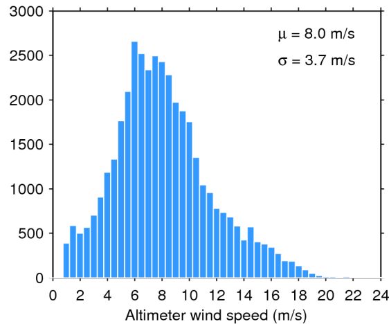
Figure 33. Histogram of flag-valid wind over oceans and lakes for 06/12/2019. The mean ( \mu ) and standard deviation ( \sigma ) are also shown. Note that values larger than 24 m/s are excluded from the histogram for the sake of readability but not from the computation of \mu and \sigma .
