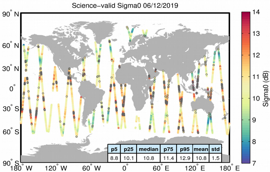
Figure 27. Geographical distribution of science-valid sigma0 data over oceans and lakes for 06/12/2019. The statistical values shown in the table refer to the sigma0 in dB and are calculated over all measurements shown in the figure. Gray circles denote records that have been rejected based on the editing criteria described in Table 4.
