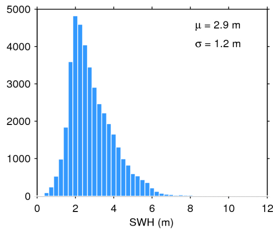
Figure 17. Histogram of flag-valid SWH over oceans and lakes for 05/12/2019. The mean ( \mu ) and standard deviation ( \sigma ) are also shown. Note that values larger than 12 m are excluded from the histogram for the sake of readability but not from the computation of \mu and \sigma .
