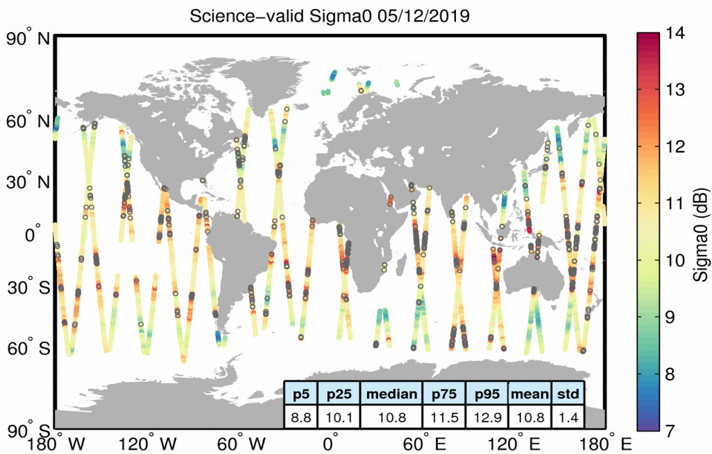
Figure 27. Geographical distribution of science-valid sigma0 data over oceans and lakes for 05/12/2019. The statistical values shown in the table refer to the sigma0 in dB and are calculated over all measurements shown in the figure. Gray circles denote records that have been rejected based on the editing criteria described in Table 4.
