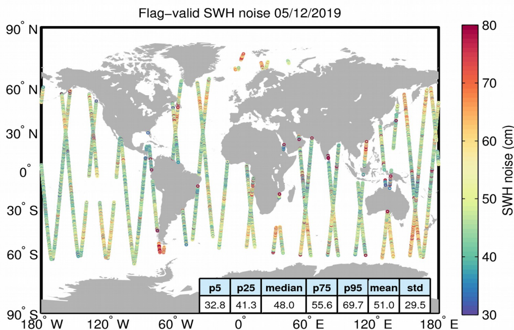
Figure 18. Geographical distribution of flag-valid 20-Hz SWH measurement noise over oceans and lakes for 05/12/2019. The statistical values shown in the figure refer to the SWH noise and are calculated over all measurements shown in the figure.
