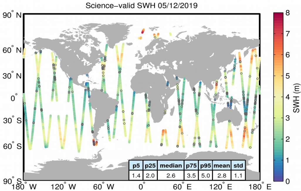
Figure 19. Geographical distribution of science-valid SWH data over oceans and lakes for 05/12/2019. The statistical values shown in the table refer to the SWH in m and are calculated over all measurements shown in the figure. Gray circles denote records that have been rejected based on the editing criteria described in Table 3.
