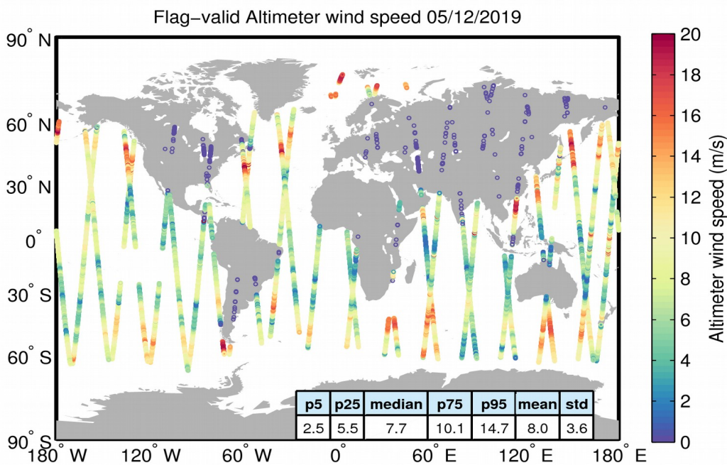
Figure 31. Geographical distribution of flag-valid wind data over oceans and lakes for 05/12/2019. The statistical values shown in the table refer to the wind in m/s and are calculated over all measurements shown in the figure.
