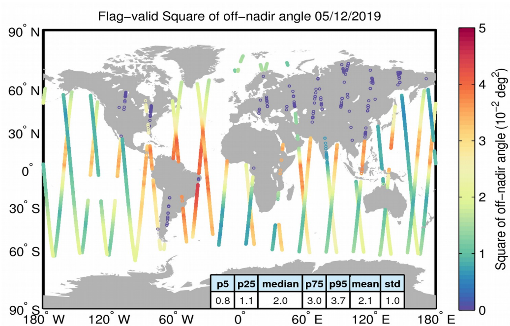
Figure 37. Geographical distribution of flag-valid mispointing data over oceans and lakes for 05/12/2019. The statistical values shown in the table refer to the mispointing in 10^{-2} deg 2 and are calculated over all measurements shown in the figure.
