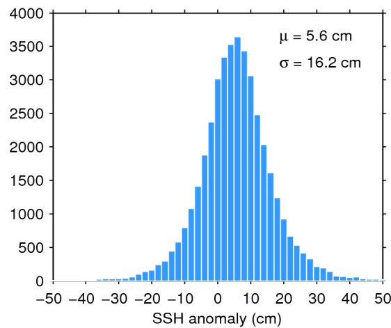
Figure 7. Histogram of flag-valid SSH anomaly over oceans and lakes for 05/12/2019. The mean ( \mu ) and standard deviation ( \sigma ) are also shown. Note that values outside [-50\ 50] cm are excluded from the histogram for the sake of readability but not from the computation of \mu and \sigma .
