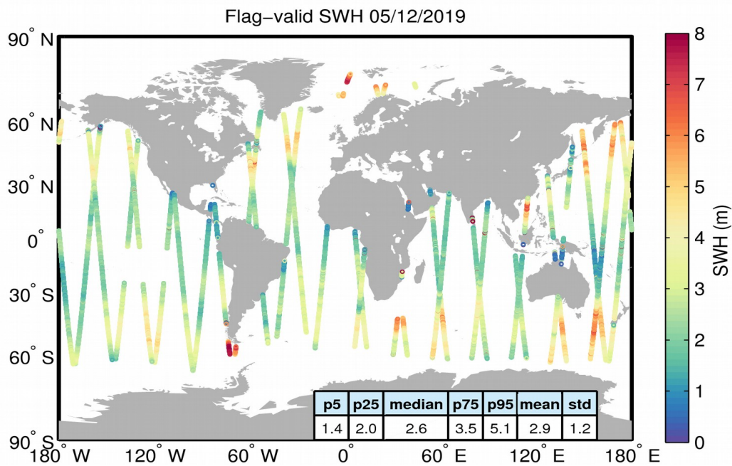
Figure 15. Geographical distribution of flag-valid SWH data over oceans and lakes for 05/12/2019. The statistical values shown in the table refer to the SWH in m and are calculated over all measurements shown in the figure.
