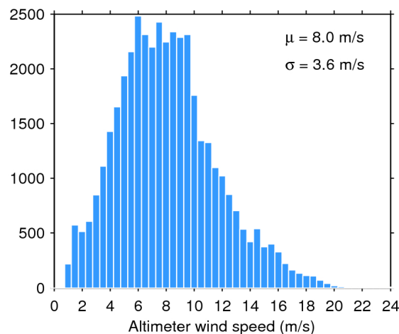
Figure 35. Histogram of science-valid wind over oceans and lakes for 05/12/2019. The mean ( \mu ) and standard deviation ( \sigma ) are also shown. Note that values larger than 24 m/s are excluded from the histogram for the sake of readability but not from the computation of \mu and \sigma .
