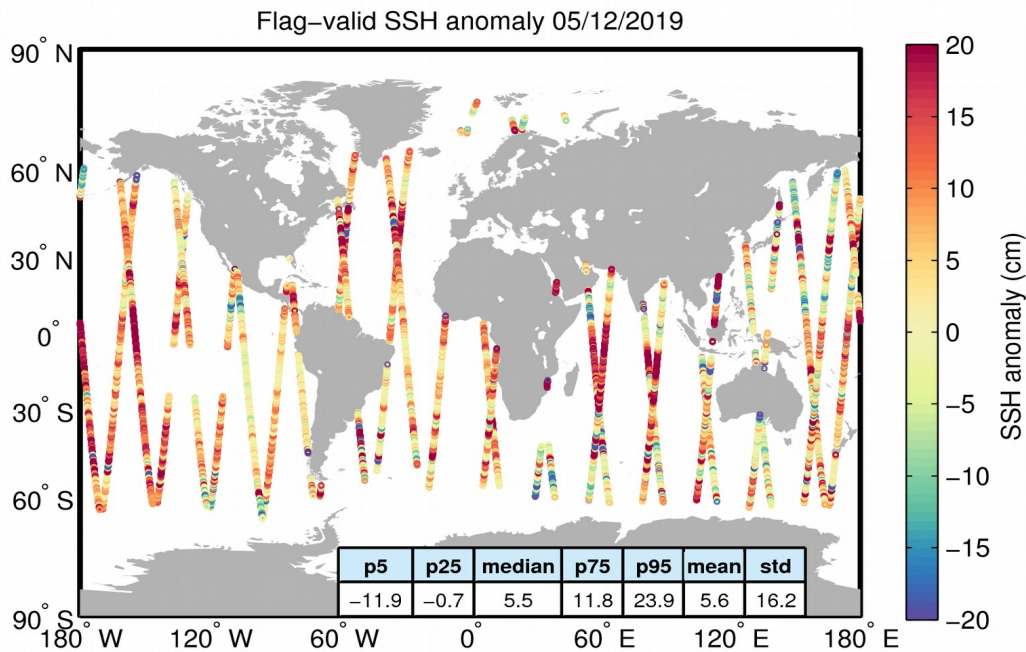
Figure 5. Geographical distribution of flag-valid 1-Hz SSH anomaly data over oceans and lakes for 05/12/2019. The statistical values shown in the table refer to the SSH anomaly in cm and are calculated over all measurements shown in the figure.
