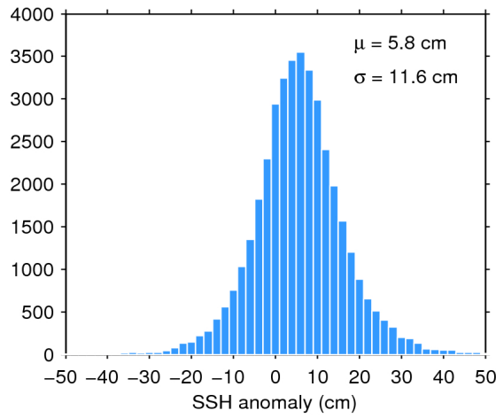
Figure 11. Histogram of science-valid SSH anomaly over oceans and lakes for 05/12/2019. The mean ( \mu ) and standard deviation ( \sigma ) are also shown. Note that values outside [-50 50] cm are excluded from the histogram for the sake of readability but not from the computation of \mu and \sigma .
