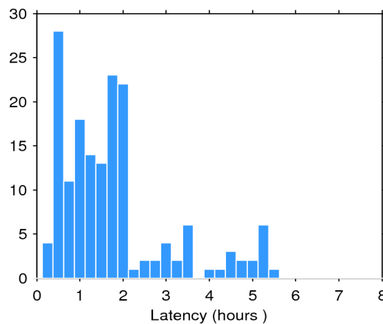
Figure 2. Histogram of the data latency for 05/12/2019. The y-axis denotes the number of files that are made available with a delay of x-hours with respect to the mean time of the records stored in the file.
