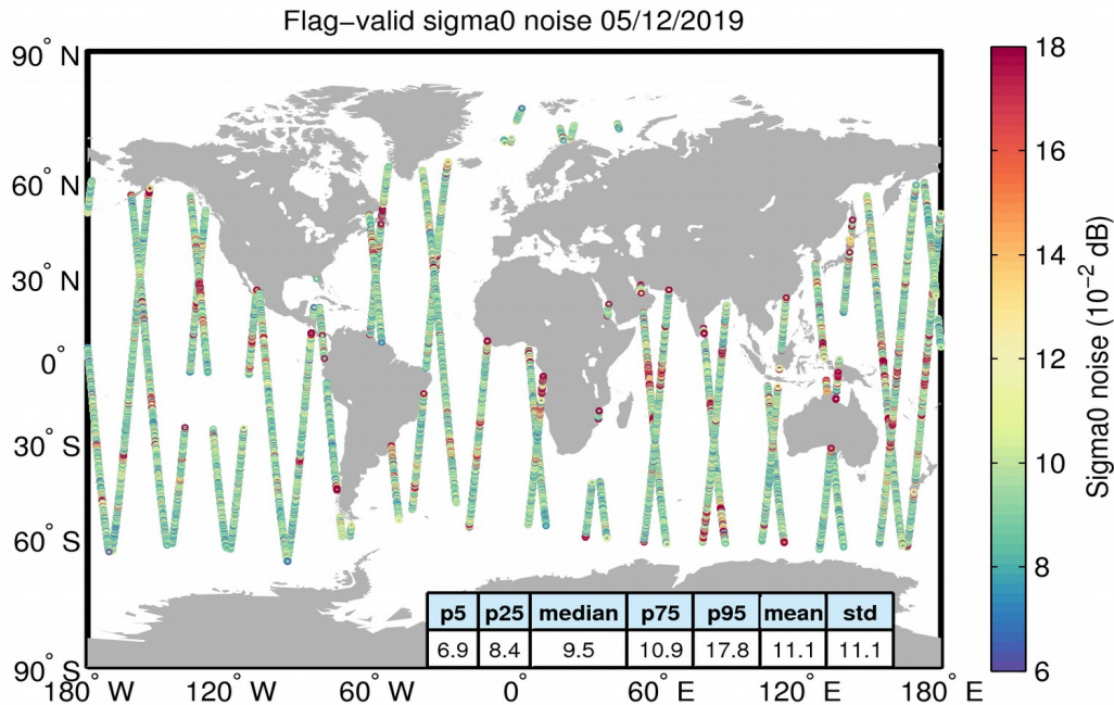
Figure 26. Geographical distribution of flag-valid 20-Hz sigma0 measurement noise over oceans and lakes for 05/12/2019. The statistical values shown in the table refer to the sigma0 noise and are calculated over all measurements shown in the figure.
