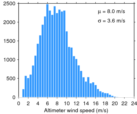
Figure 33. Histogram of flag-valid wind over oceans and lakes for 05/12/2019. The mean ( \mu ) and standard deviation ( \sigma ) are also shown. Note that values larger than 24 m/s are excluded from the histogram for the sake of readability but not from the computation of \mu and \sigma .
