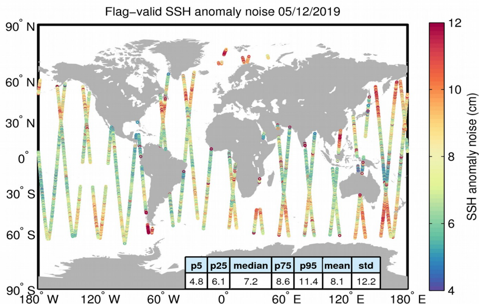
Figure 8. Geographical distribution of flag-valid 20-Hz SSH anomaly measurement noise over oceans and lakes for 05/12/2019. The statistical values shown in the table refer to the SSH anomaly noise and are calculated over all measurements shown in the figure.
