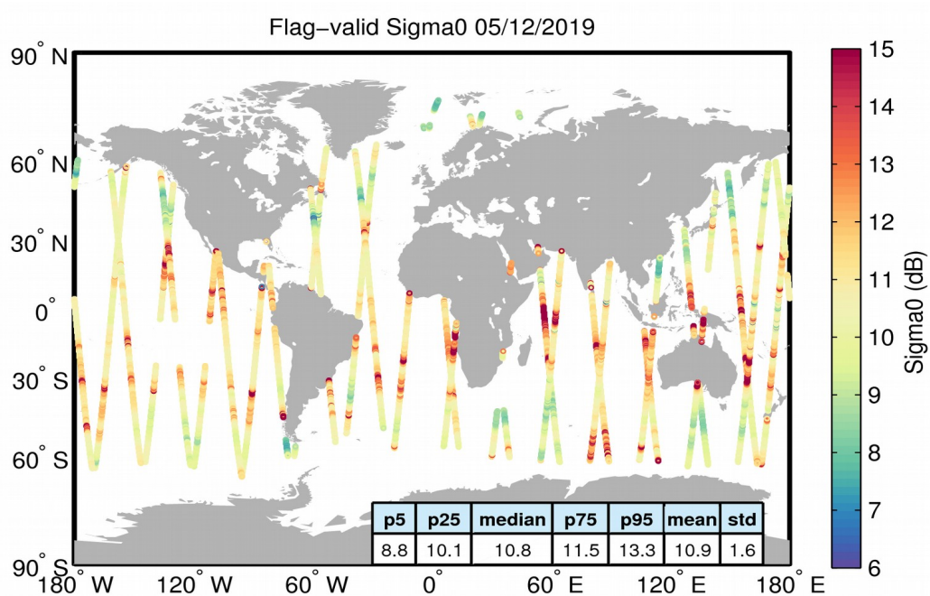
Figure 23. Geographical distribution of flag-valid sigma0 data over oceans and lakes for 05/12/2019. The statistical values shown in the table refer to the sigma0 in dB and are calculated over all measurements shown in the figure.
