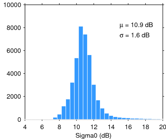
Figure 25. Histogram of flag-valid sigma0 over oceans and lakes for 05/12/2019. The mean ( \mu ) and standard deviation ( \sigma ) are also shown. Note that values outside [4 20] dB are excluded from the histogram for the sake of readability but not from the computation of \mu and \sigma .
