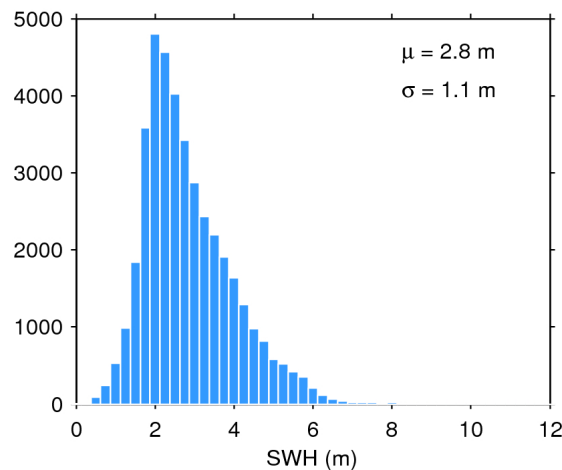
Figure 20. Histogram of science-valid SWH over oceans and lakes for 05/12/2019. The mean ( \mu ) and standard deviation ( \sigma ) are also shown. Note that values larger than 12 m are excluded from the histogram for the sake of readability but not from the computation of \mu and \sigma .
