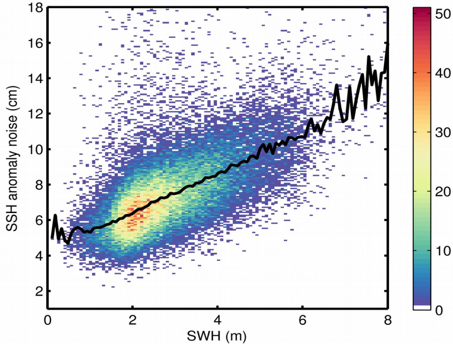
Figure 9. 2D histogram showing flag-valid SSH anomaly noise as a function of SWH for 05/12/2019. The black line denotes the median SSH anomaly noise as a function of SWH.
