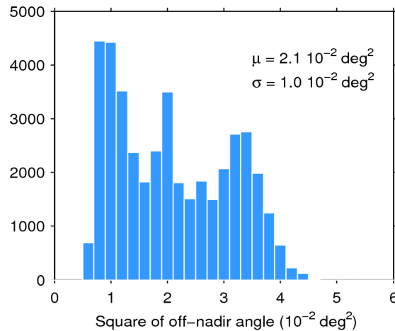
Figure 39. Histogram of flag-valid mispointing over oceans and lakes for 05/12/2019. The mean ( \mu ) and standard deviation ( \sigma ) are also shown. Note that values larger than 6 \cdot 10^{-2} \text{ deg}^2 are excluded from the histogram for the sake of readability but not from the computation of \mu and \sigma .
