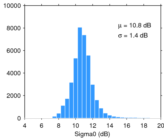
Figure 28. Histogram of science-valid sigma0 over oceans and lakes for 05/12/2019. The mean ( \mu ) and standard deviation ( \sigma ) are also shown. Note that values outside [4 20] dB are excluded from the histogram for the sake of readability but not from the computation of \mu and \sigma .
