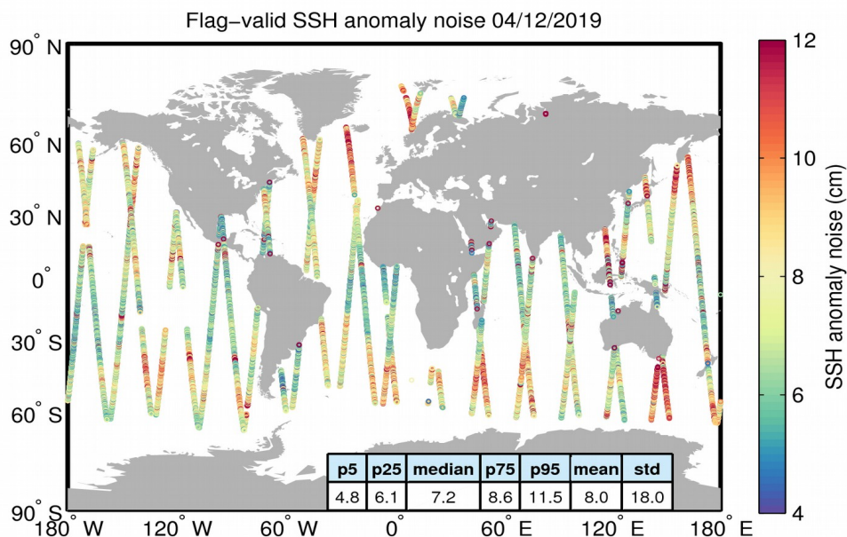
Figure 8. Geographical distribution of flag-valid 20-Hz SSH anomaly measurement noise over oceans and lakes for 04/12/2019. The statistical values shown in the table refer to the SSH anomaly noise and are calculated over all measurements shown in the figure.
