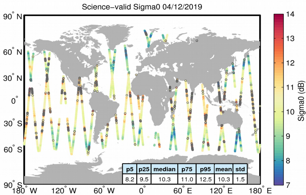
Figure 27. Geographical distribution of science-valid sigma0 data over oceans and lakes for 04/12/2019. The statistical values shown in the table refer to the sigma0 in dB and are calculated over all measurements shown in the figure. Gray circles denote records that have been rejected based on the editing criteria described in Table 4.
