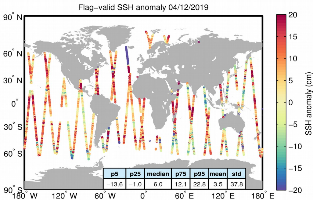
Figure 5. Geographical distribution of flag-valid 1-Hz SSH anomaly data over oceans and lakes for 04/12/2019. The statistical values shown in the table refer to the SSH anomaly in cm and are calculated over all measurements shown in the figure.
