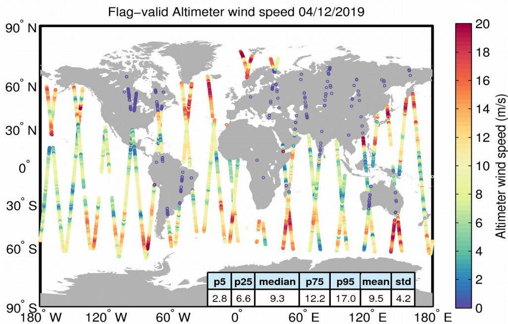
Figure 31. Geographical distribution of flag-valid wind data over oceans and lakes for 04/12/2019. The statistical values shown in the table refer to the wind in m/s and are calculated over all measurements shown in the figure.
