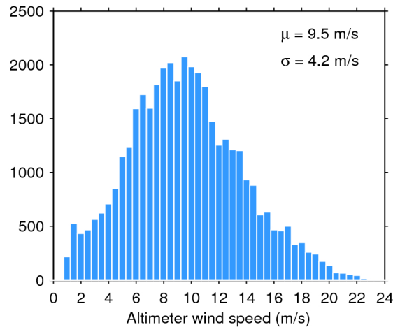
Figure 33. Histogram of flag-valid wind over oceans and lakes for 04/12/2019. The mean ( \mu ) and standard deviation ( \sigma ) are also shown. Note that values larger than 24 m/s are excluded from the histogram for the sake of readability but not from the computation of \mu and \sigma .
