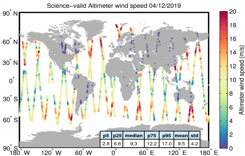
Figure 34. Geographical distribution of science-valid wind data over oceans and lakes for 04/12/2019. The statistical values shown in the table refer to the wind in m/s and are calculated over all measurements shown in the figure. Gray circles denote records that have been rejected based on the editing criteria described in Table 5.
