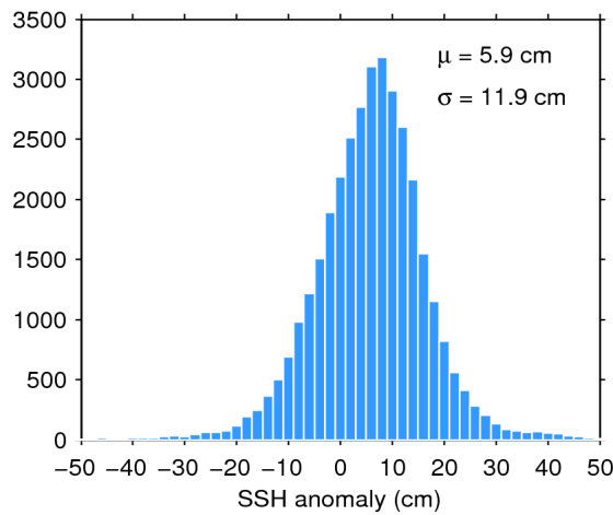
Figure 11. Histogram of science-valid SSH anomaly over oceans and lakes for 04/12/2019. The mean ( \mu ) and standard deviation ( \sigma ) are also shown. Note that values outside [-50 50] cm are excluded from the histogram for the sake of readability but not from the computation of \mu and \sigma .
