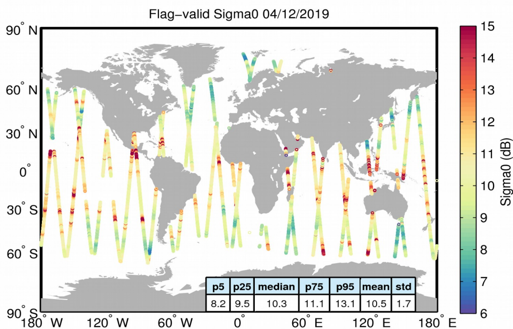
Figure 23. Geographical distribution of flag-valid sigma0 data over oceans and lakes for 04/12/2019. The statistical values shown in the table refer to the sigma0 in dB and are calculated over all measurements shown in the figure.
