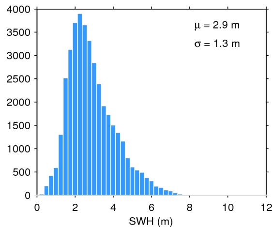
Figure 17. Histogram of flag-valid SWH over oceans and lakes for 04/12/2019. The mean ( \mu ) and standard deviation ( \sigma ) are also shown. Note that values larger than 12 m are excluded from the histogram for the sake of readability but not from the computation of \mu and \sigma .
