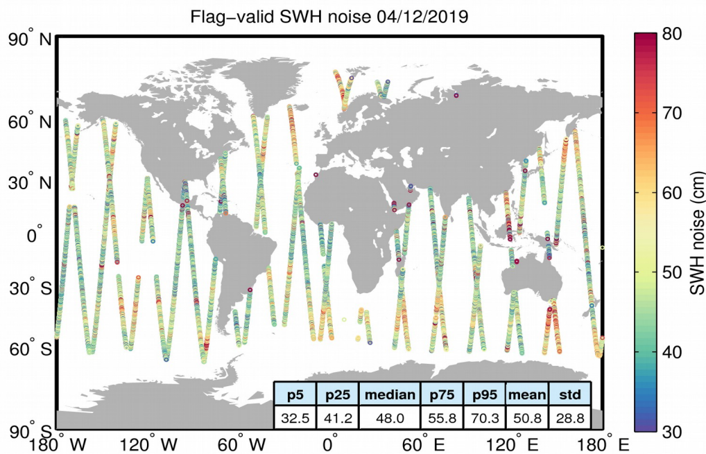
Figure 18. Geographical distribution of flag-valid 20-Hz SWH measurement noise over oceans and lakes for 04/12/2019. The statistical values shown in the figure refer to the SWH noise and are calculated over all measurements shown in the figure.
