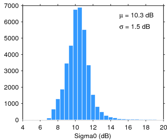
Figure 28. Histogram of science-valid sigma0 over oceans and lakes for 04/12/2019. The mean ( \mu ) and standard deviation ( \sigma ) are also shown. Note that values outside [4 20] dB are excluded from the histogram for the sake of readability but not from the computation of \mu and \sigma .
