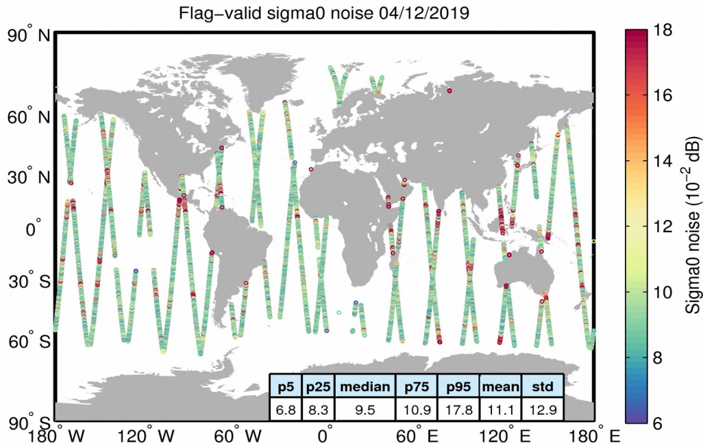
Figure 26. Geographical distribution of flag-valid 20-Hz sigma0 measurement noise over oceans and lakes for 04/12/2019. The statistical values shown in the table refer to the sigma0 noise and are calculated over all measurements shown in the figure.
