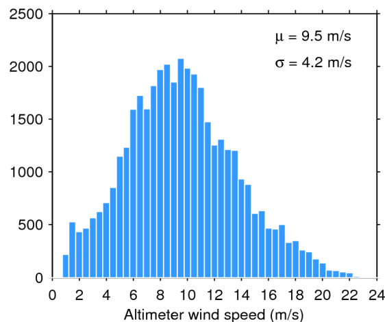
Figure 35. Histogram of science-valid wind over oceans and lakes for 04/12/2019. The mean ( \mu ) and standard deviation ( \sigma ) are also shown. Note that values larger than 24 m/s are excluded from the histogram for the sake of readability but not from the computation of \mu and \sigma .
