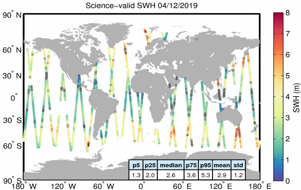
Figure 19. Geographical distribution of science-valid SWH data over oceans and lakes for 04/12/2019. The statistical values shown in the table refer to the SWH in m and are calculated over all measurements shown in the figure. Gray circles denote records that have been rejected based on the editing criteria described in Table 3.
