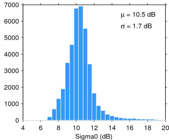
Figure 25. Histogram of flag-valid sigma0 over oceans and lakes for 04/12/2019. The mean ( \mu ) and standard deviation ( \sigma ) are also shown. Note that values outside [4 20] dB are excluded from the histogram for the sake of readability but not from the computation of \mu and \sigma .
