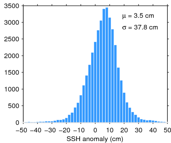
Figure 7. Histogram of flag-valid SSH anomaly over oceans and lakes for 04/12/2019. The mean ( \mu ) and standard deviation ( \sigma ) are also shown. Note that values outside [-50\ 50] cm are excluded from the histogram for the sake of readability but not from the computation of \mu and \sigma .
