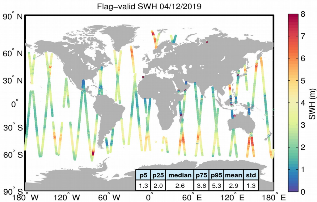
Figure 15. Geographical distribution of flag-valid SWH data over oceans and lakes for 04/12/2019. The statistical values shown in the table refer to the SWH in m and are calculated over all measurements shown in the figure.
