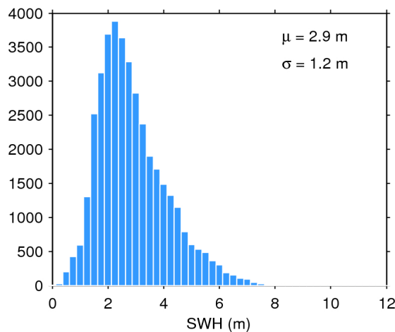
Figure 20. Histogram of science-valid SWH over oceans and lakes for 04/12/2019. The mean ( \mu ) and standard deviation ( \sigma ) are also shown. Note that values larger than 12 m are excluded from the histogram for the sake of readability but not from the computation of \mu and \sigma .
