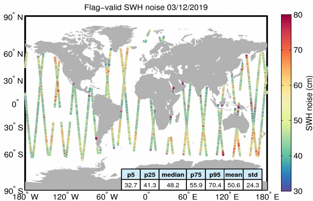
Figure 18. Geographical distribution of flag-valid 20-Hz SWH measurement noise over oceans and lakes for 03/12/2019. The statistical values shown in the table refer to the SWH noise and are calculated over all measurements shown in the figure.
