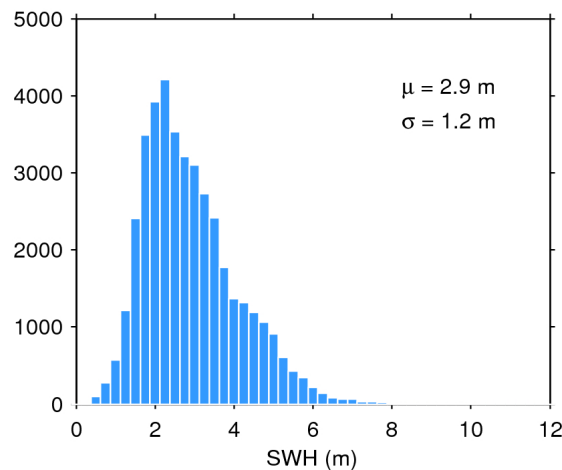
Figure 20. Histogram of science-valid SWH over oceans and lakes for 03/12/2019. The mean ( \mu ) and standard deviation ( \sigma ) are also shown. Note that values larger than 12 m are excluded from the histogram for the sake of readability but not from the computation of \mu and \sigma .
