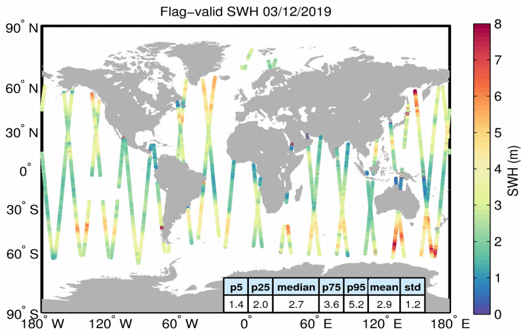
Figure 15. Geographical distribution of flag-valid SWH data over oceans and lakes for 03/12/2019. The statistical values shown in the table refer to the SWH in m and are calculated over all measurements shown in the figure.
