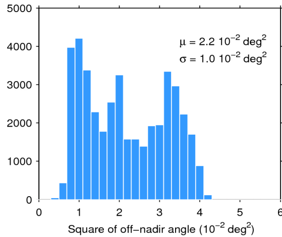
Figure 39. Histogram of flag-valid mispointing over oceans and lakes for 03/12/2019. The mean ( \mu ) and standard deviation ( \sigma ) are also shown. Note that values larger than 6 \cdot 10^{-2} \text{ deg}^2 are excluded from the histogram for the sake of readability but not from the computation of \mu and \sigma .
