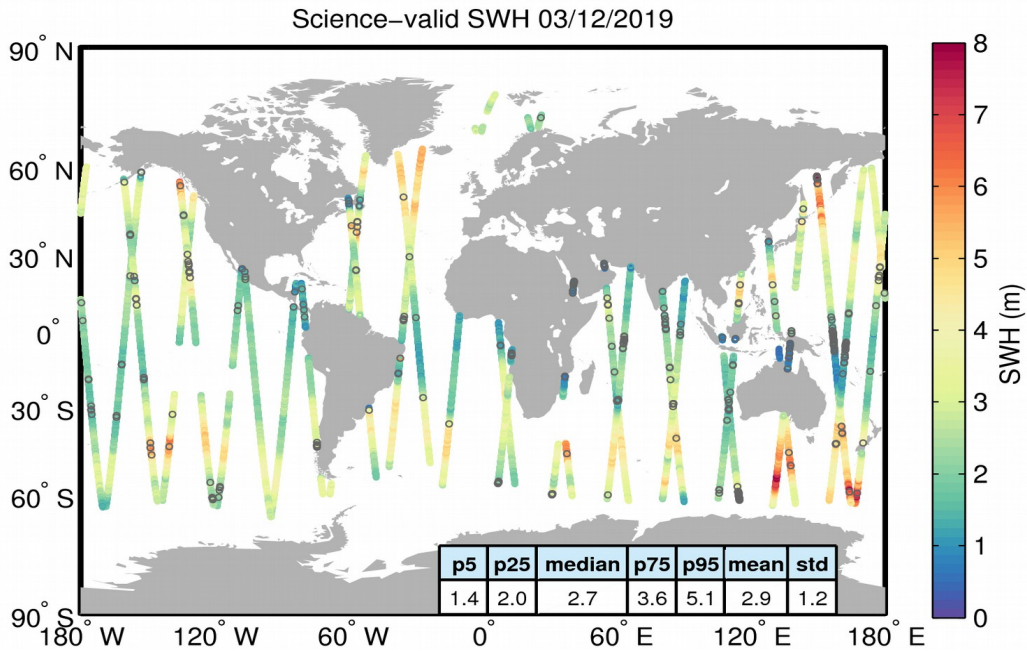
Figure 19. Geographical distribution of science-valid SWH data over oceans and lakes for 03/12/2019. The statistical values shown in the table refer to the SWH in m and are calculated over all measurements shown in the figure. Gray circles denote records that have been rejected based on the editing criteria described in Table 3.
