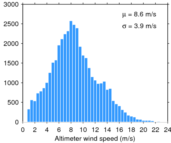
Figure 33. Histogram of flag-valid wind over oceans and lakes for 03/12/2019. The mean ( \mu ) and standard deviation ( \sigma ) are also shown. Note that values larger than 24 m/s are excluded from the histogram for the sake of readability but not from the computation of \mu and \sigma .
