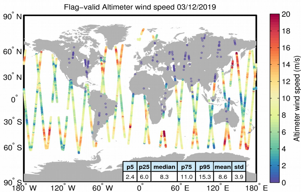
Figure 31. Geographical distribution of flag-valid wind data over oceans and lakes for 03/12/2019. The statistical values shown in the table refer to the wind in m/s and are calculated over all measurements shown in the figure.
