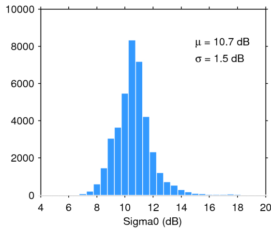
Figure 28. Histogram of science-valid sigma0 over oceans and lakes for 03/12/2019. The mean ( \mu ) and standard deviation ( \sigma ) are also shown. Note that values outside [4 20] dB are excluded from the histogram for the sake of readability but not from the computation of \mu and \sigma .
