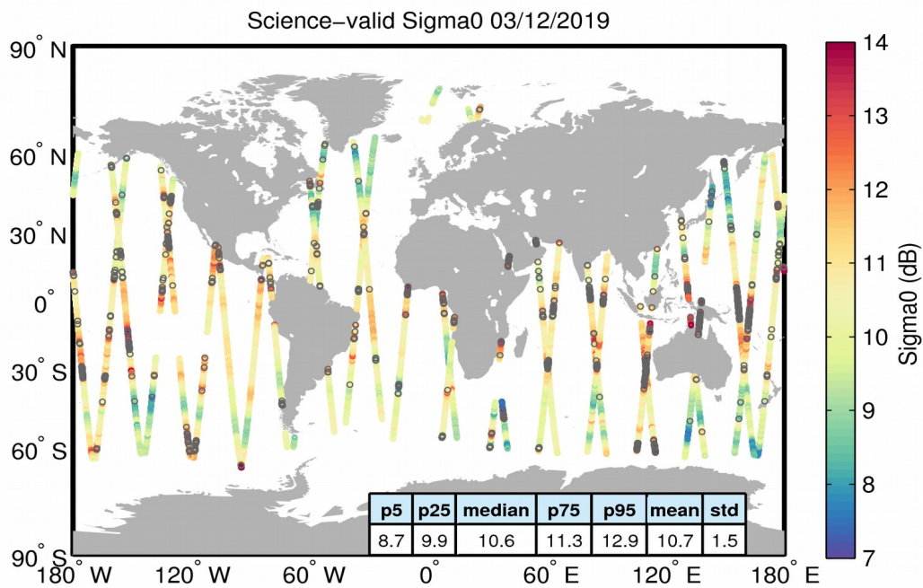
Figure 27. Geographical distribution of science-valid sigma0 data over oceans and lakes for 03/12/2019. The statistical values shown in the table refer to the sigma0 in dB and are calculated over all measurements shown in the figure. Gray circles denote records that have been rejected based on the editing criteria described in Table 4.
