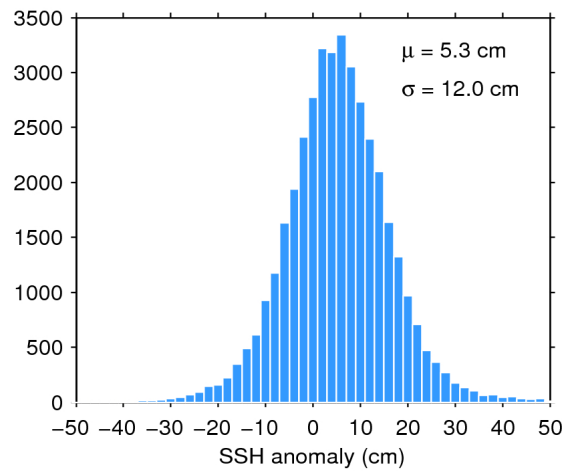
Figure 11. Histogram of science-valid SSH anomaly over oceans and lakes for 03/12/2019. The mean ( \mu ) and standard deviation ( \sigma ) are also shown. Note that values outside [-50 50] cm are excluded from the histogram for the sake of readability but not from the computation of \mu and \sigma .
