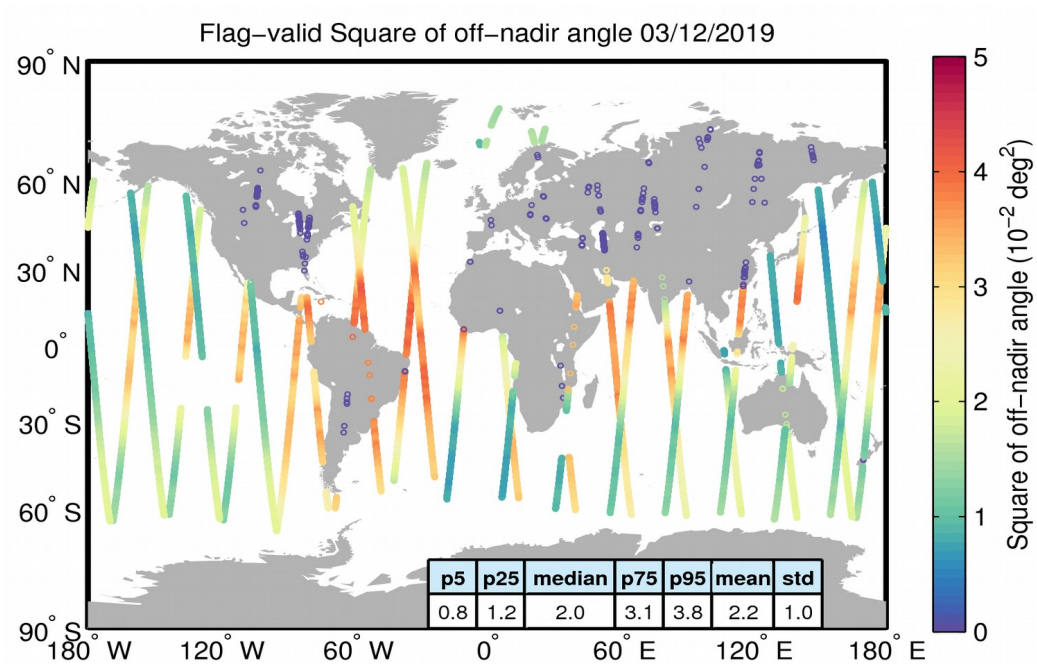
Figure 37. Geographical distribution of flag-valid mispointing data over oceans and lakes for 03/12/2019. The statistical values shown in the table refer to the mispointing in 10^{-2} \text{deg}^2 and are calculated over all measurements shown in the figure.
