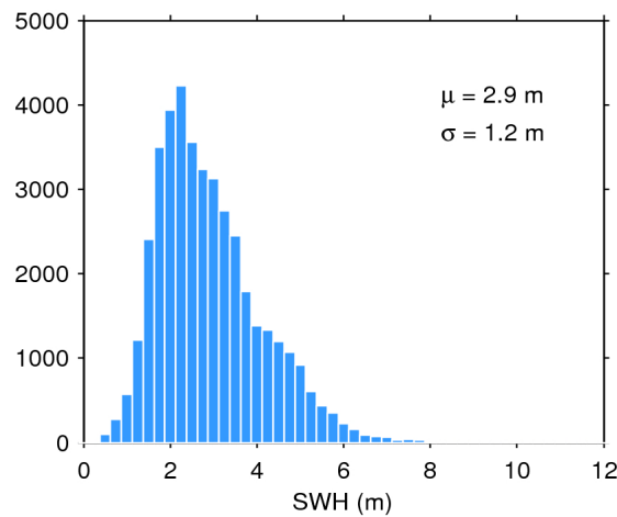
Figure 17. Histogram of flag-valid SWH over oceans and lakes for 03/12/2019. The mean ( \mu ) and standard deviation ( \sigma ) are also shown. Note that values larger than 12 m are excluded from the histogram for the sake of readability but not from the computation of \mu and \sigma .
