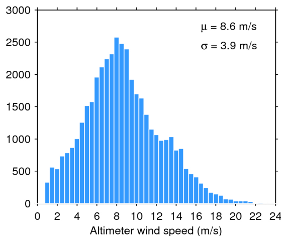
Figure 35. Histogram of science-valid wind over oceans and lakes for 03/12/2019. The mean ( \mu ) and standard deviation ( \sigma ) are also shown. Note that values larger than 24 m/s are excluded from the histogram for the sake of readability but not from the computation of \mu and \sigma .
