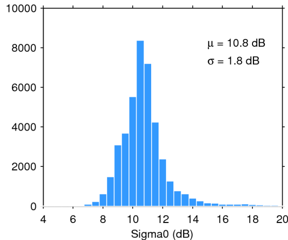
Figure 25. Histogram of flag-valid sigma0 over oceans and lakes for 03/12/2019. The mean ( \mu ) and standard deviation ( \sigma ) are also shown. Note that values outside [4 20] dB are excluded from the histogram for the sake of readability but not from the computation of \mu and \sigma .
