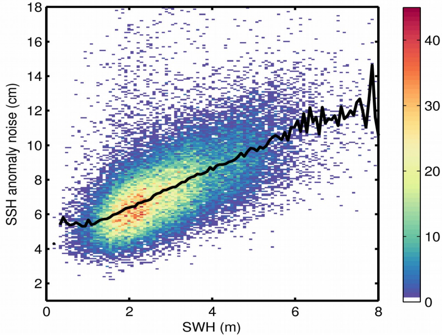
Figure 9. 2D histogram showing flag-valid SSH anomaly noise as a function of SWH for 03/12/2019. The black line denotes the median SSH anomaly noise as a function of SWH.
