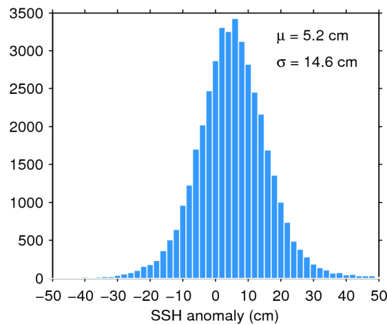
Figure 7. Histogram of flag-valid SSH anomaly over oceans and lakes for 03/12/2019. The mean ( \mu ) and standard deviation ( \sigma ) are also shown. Note that values outside [-50\ 50] cm are excluded from the histogram for the sake of readability but not from the computation of \mu and \sigma .
