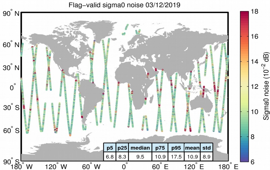
Figure 26. Geographical distribution of flag-valid 20-Hz sigma0 measurement noise over oceans and lakes for 03/12/2019. The statistical values shown in the table refer to the sigma0 noise and are calculated over all measurements shown in the figure.
