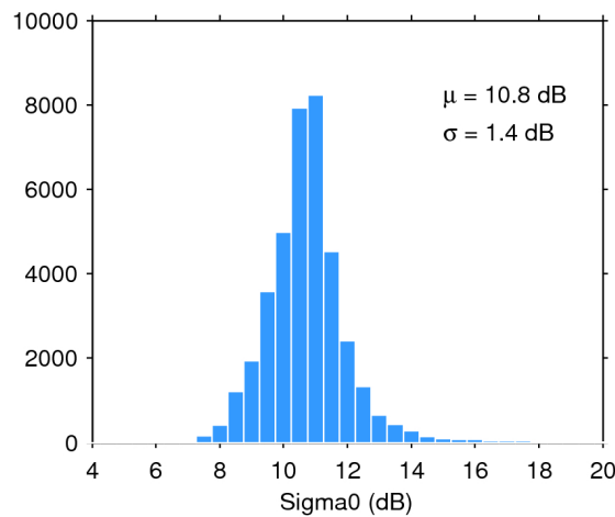
Figure 28. Histogram of science-valid sigma0 over oceans and lakes for 02/12/2019. The mean ( \mu ) and standard deviation ( \sigma ) are also shown. Note that values outside [4 20] dB are excluded from the histogram for the sake of readability but not from the computation of \mu and \sigma .
