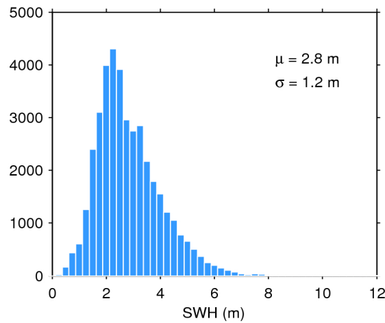
Figure 17. Histogram of flag-valid SWH over oceans and lakes for 02/12/2019. The mean ( \mu ) and standard deviation ( \sigma ) are also shown. Note that values larger than 12 m are excluded from the histogram for the sake of readability but not from the computation of \mu and \sigma .
