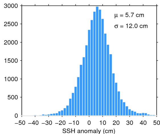
Figure 11. Histogram of science-valid SSH anomaly over oceans and lakes for 02/12/2019. The mean ( \mu ) and standard deviation ( \sigma ) are also shown. Note that values outside [-50 50] cm are excluded from the histogram for the sake of readability but not from the computation of \mu and \sigma .
