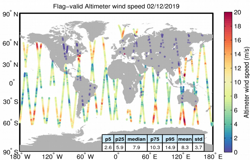
Figure 31. Geographical distribution of flag-valid wind data over oceans and lakes for 02/12/2019. The statistical values shown in the table refer to the wind in m/s and are calculated over all measurements shown in the figure.
