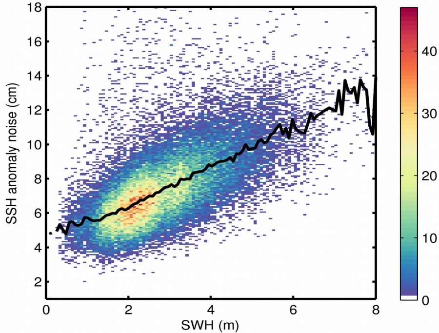
Figure 9. 2D histogram showing flag-valid SSH anomaly noise as a function of SWH for 02/12/2019. The black line denotes the median SSH anomaly noise as a function of SWH.
