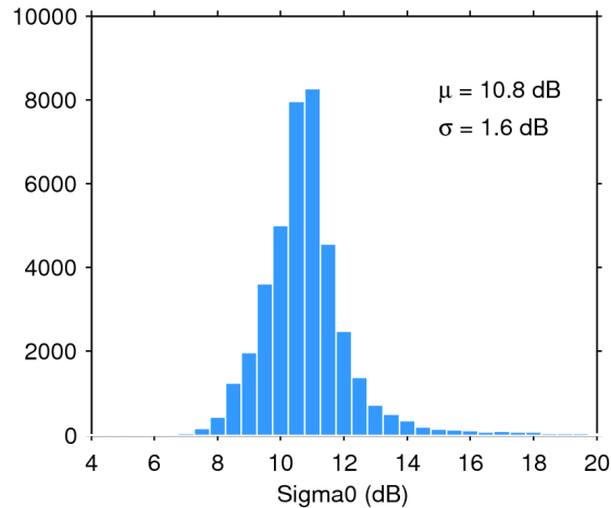
Figure 25. Histogram of flag-valid sigma0 over oceans and lakes for 02/12/2019. The mean ( \mu ) and standard deviation ( \sigma ) are also shown. Note that values outside [4 20] dB are excluded from the histogram for the sake of readability but not from the computation of \mu and \sigma .
