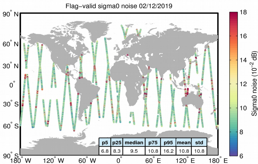
Figure 26. Geographical distribution of flag-valid 20-Hz sigma0 measurement noise over oceans and lakes for 02/12/2019. The statistical values shown in the figure refer to the sigma0 noise and are calculated over all measurements shown in the figure.
