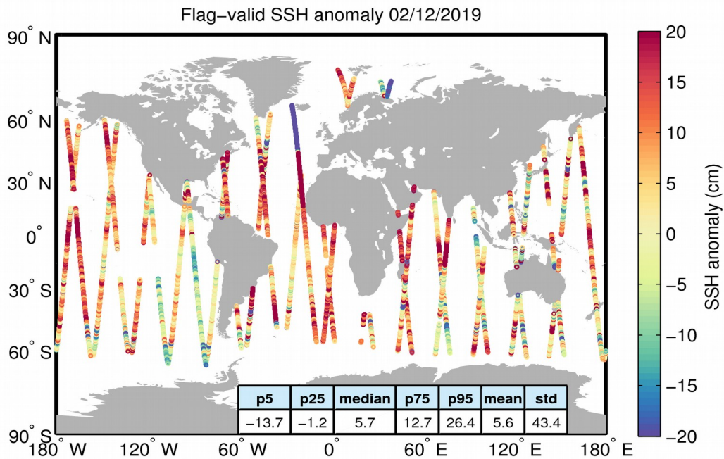
Figure 5. Geographical distribution of flag-valid 1-Hz SSH anomaly data over oceans and lakes for 02/12/2019. The statistical values shown in the table refer to the SSH anomaly in cm and are calculated over all measurements shown in the figure.
