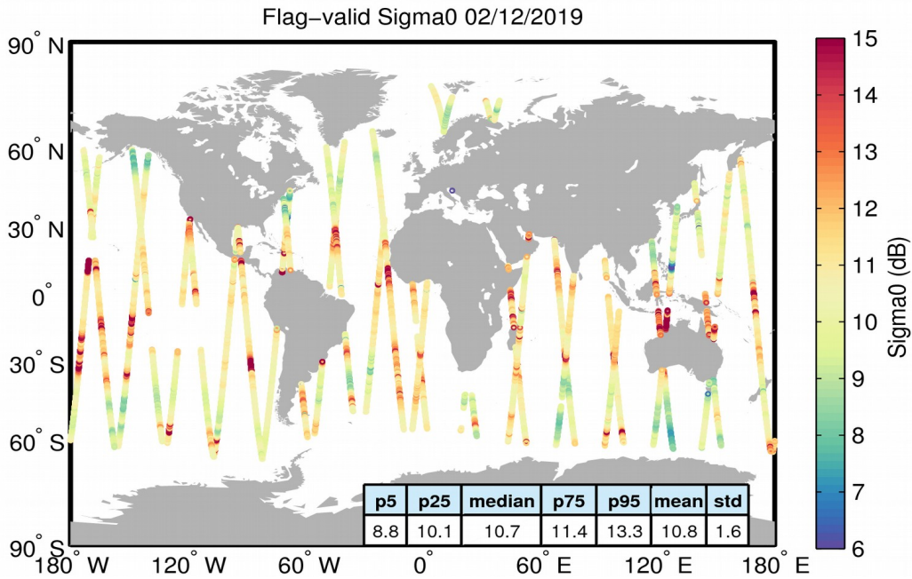
Figure 23. Geographical distribution of flag-valid sigma0 data over oceans and lakes for 02/12/2019. The statistical values shown in the table refer to the sigma0 in dB and are calculated over all measurements shown in the figure.
