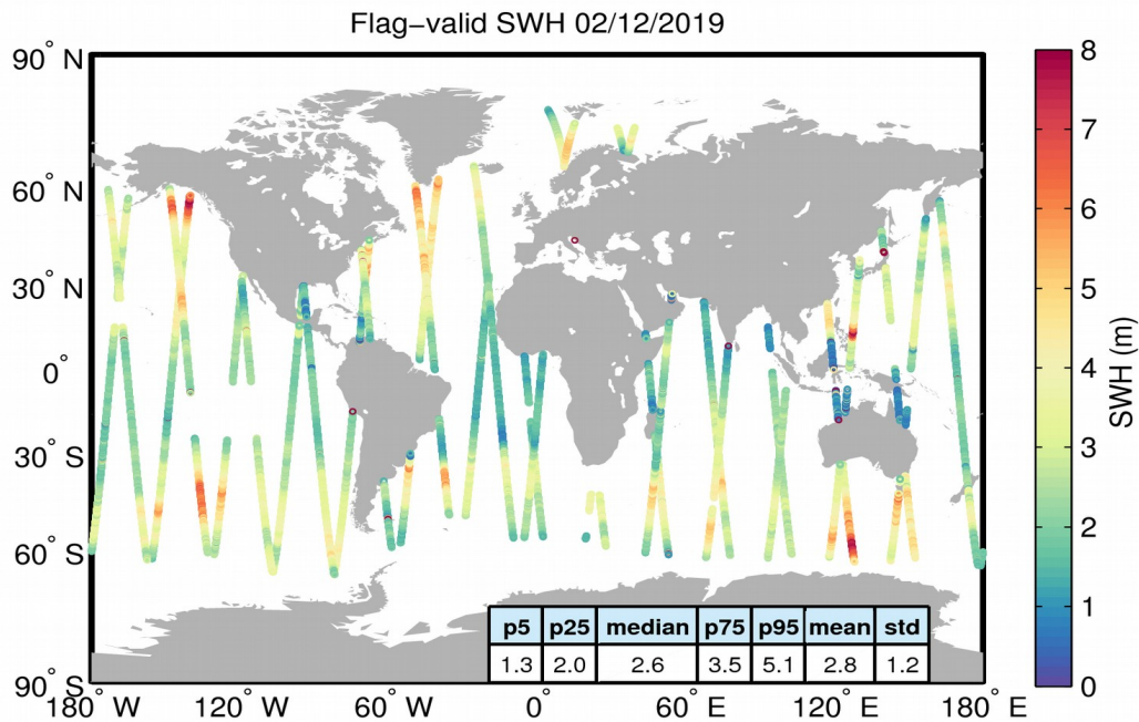
Figure 15. Geographical distribution of flag-valid SWH data over oceans and lakes for 02/12/2019. The statistical values shown in the table refer to the SWH in m and are calculated over all measurements shown in the figure.
