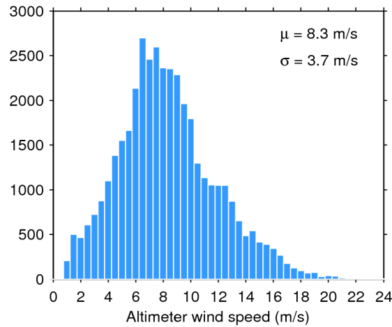
Figure 33. Histogram of flag-valid wind over oceans and lakes for 02/12/2019. The mean ( \mu ) and standard deviation ( \sigma ) are also shown. Note that values larger than 24 m/s are excluded from the histogram for the sake of readability but not from the computation of \mu and \sigma .
