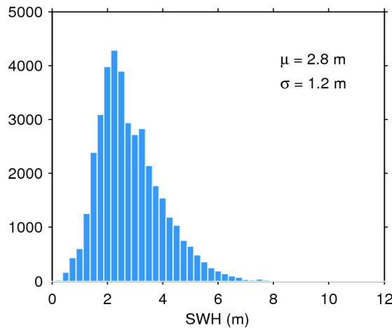
Figure 20. Histogram of science-valid SWH over oceans and lakes for 02/12/2019. The mean ( \mu ) and standard deviation ( \sigma ) are also shown. Note that values larger than 12 m are excluded from the histogram for the sake of readability but not from the computation of \mu and \sigma .
