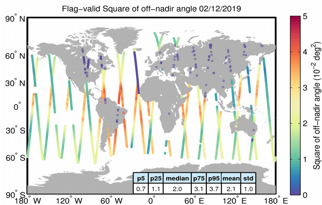
Figure 37. Geographical distribution of flag-valid mispointing data over oceans and lakes for 02/12/2019. The statistical values shown in the table refer to the mispointing in 10^{-2} deg 2 and are calculated over all measurements shown in the figure.
