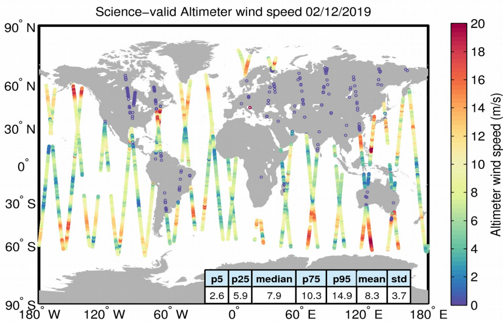
Figure 34. Geographical distribution of science-valid wind data over oceans and lakes for 02/12/2019. The statistical values shown in the table refer to the wind in m/s and are calculated over all measurements shown in the figure. Gray circles denote records that have been rejected based on the editing criteria described in Table 5.
