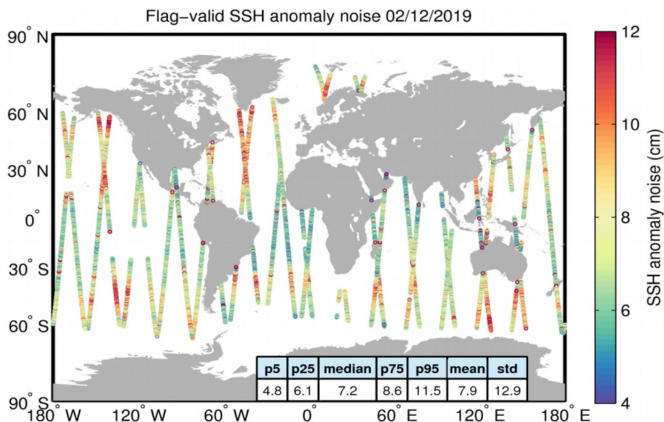
Figure 8. Geographical distribution of flag-valid 20-Hz SSH anomaly measurement noise over oceans and lakes for 02/12/2019. The statistical values shown in the table refer to the SSH anomaly noise and are calculated over all measurements shown in the figure.
