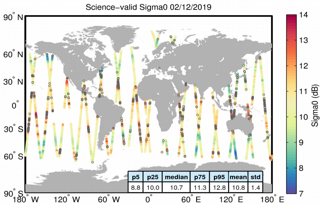
Figure 27. Geographical distribution of science-valid sigma0 data over oceans and lakes for 02/12/2019. The statistical values shown in the table refer to the sigma0 in dB and are calculated over all measurements shown in the figure. Gray circles denote records that have been rejected based on the editing criteria described in Table 4.
