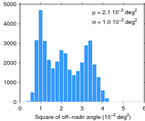
Figure 39. Histogram of flag-valid mispointing over oceans and lakes for 02/12/2019. The mean ( \mu ) and standard deviation ( \sigma ) are also shown. Note that values larger than 6 \cdot 10^{-2} \text{ deg}^2 are excluded from the histogram for the sake of readability but not from the computation of \mu and \sigma .
