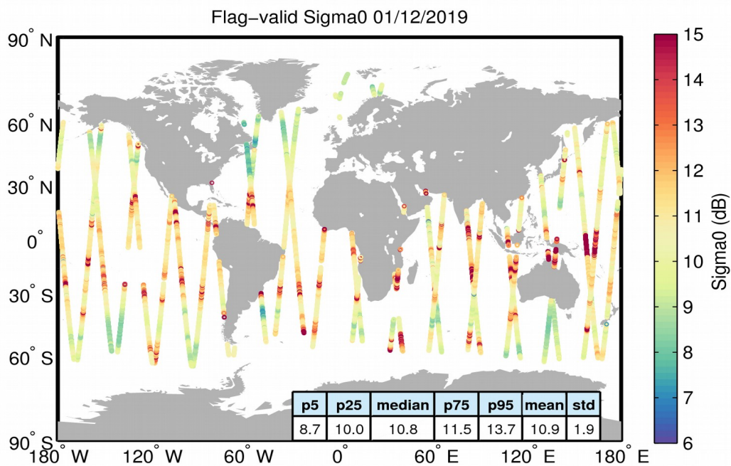
Figure 23. Geographical distribution of flag-valid sigma0 data over oceans and lakes for 01/12/2019. The statistical values shown in the table refer to the sigma0 in dB and are calculated over all measurements shown in the figure.
