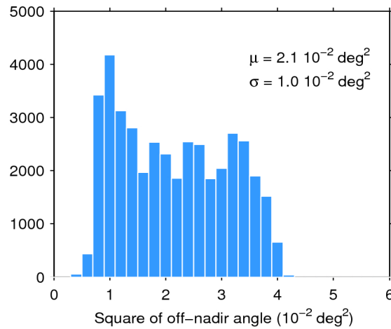
Figure 39. Histogram of flag-valid mispointing over oceans and lakes for 01/12/2019. The mean ( \mu ) and standard deviation ( \sigma ) are also shown. Note that values larger than 6 \cdot 10^{-2} \text{ deg}^2 are excluded from the histogram for the sake of readability but not from the computation of \mu and \sigma .
