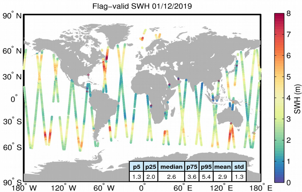
Figure 15. Geographical distribution of flag-valid SWH data over oceans and lakes for 01/12/2019. The statistical values shown in the table refer to the SWH in m and are calculated over all measurements shown in the figure.
