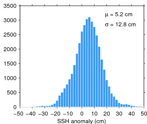
Figure 11. Histogram of science-valid SSH anomaly over oceans and lakes for 01/12/2019. The mean ( \mu ) and standard deviation ( \sigma ) are also shown. Note that values outside [-50 50] cm are excluded from the histogram for the sake of readability but not from the computation of \mu and \sigma .
