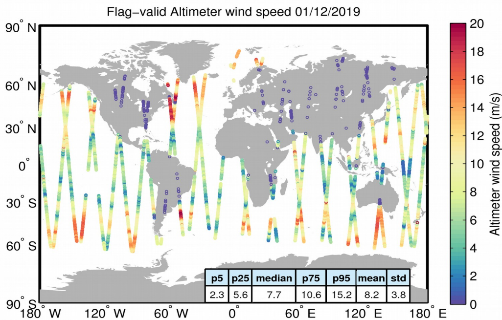
Figure 31. Geographical distribution of flag-valid wind data over oceans and lakes for 01/12/2019. The statistical values shown in the table refer to the wind in m/s and are calculated over all measurements shown in the figure.
