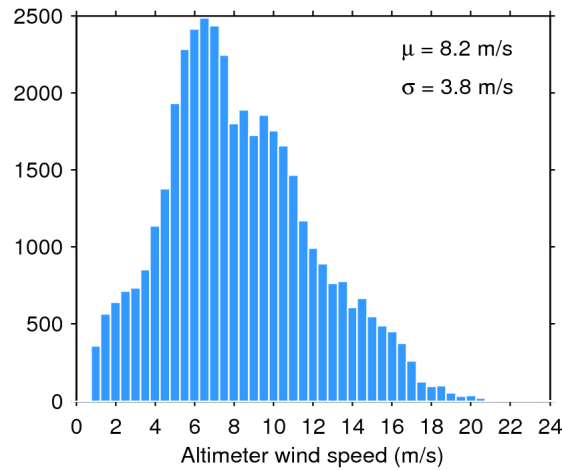
Figure 33. Histogram of flag-valid wind over oceans and lakes for 01/12/2019. The mean ( \mu ) and standard deviation ( \sigma ) are also shown. Note that values larger than 24 m/s are excluded from the histogram for the sake of readability but not from the computation of \mu and \sigma .
