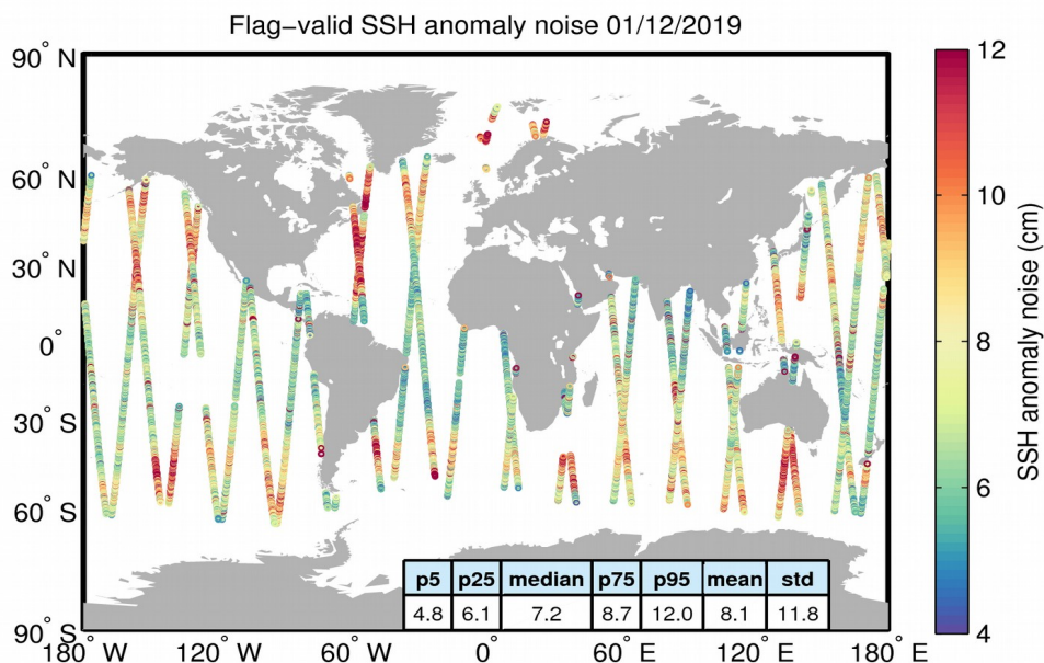
Figure 8. Geographical distribution of flag-valid 20-Hz SSH anomaly measurement noise over oceans and lakes for 01/12/2019. The statistical values shown in the table refer to the SSH anomaly noise and are calculated over all measurements shown in the figure.
