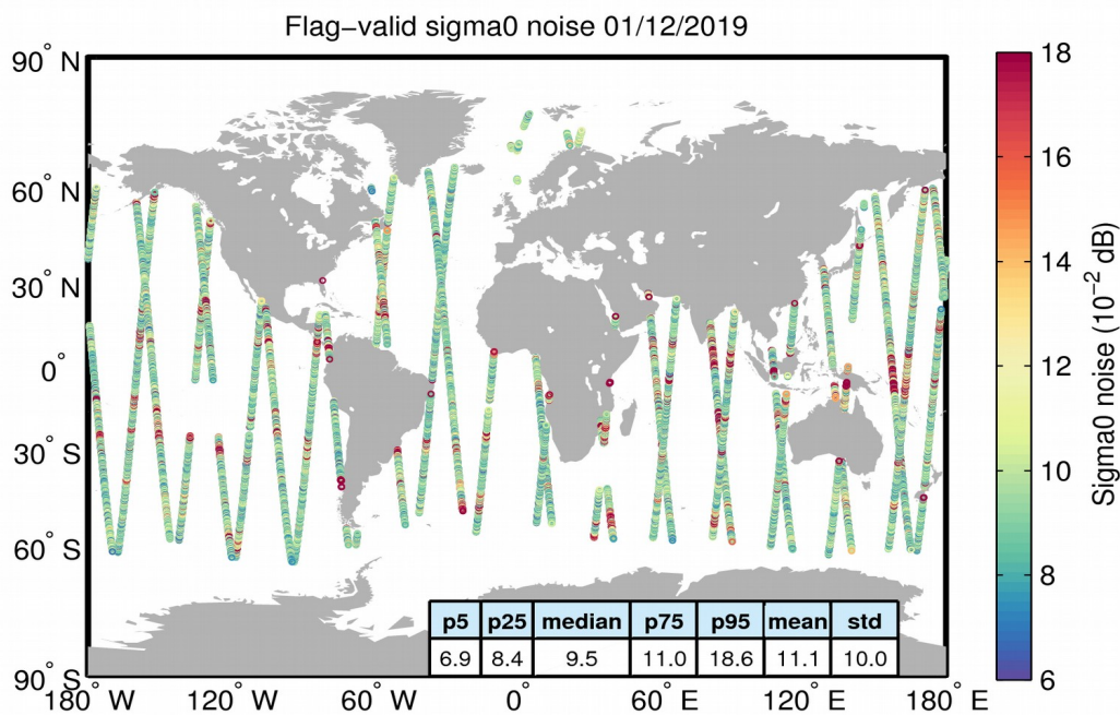
Figure 26. Geographical distribution of flag-valid 20-Hz sigma0 measurement noise over oceans and lakes for 01/12/2019. The statistical values shown in the table refer to the sigma0 noise and are calculated over all measurements shown in the figure.
