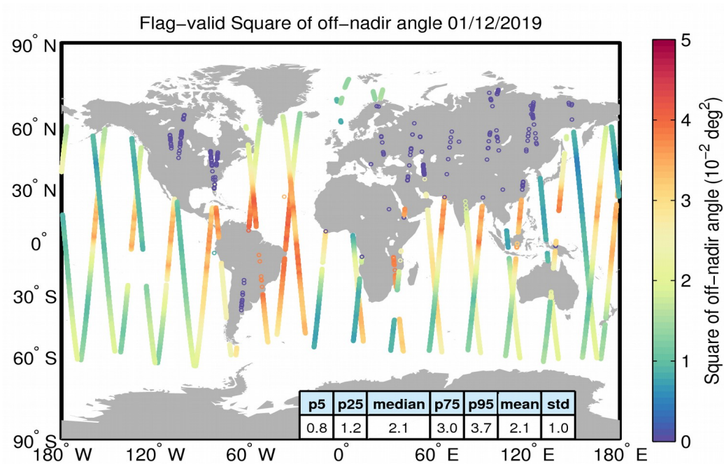
Figure 37. Geographical distribution of flag-valid mispointing data over oceans and lakes for 01/12/2019. The statistical values shown in the table refer to the mispointing in 10^{-2} \text{deg}^2 and are calculated over all measurements shown in the figure.
