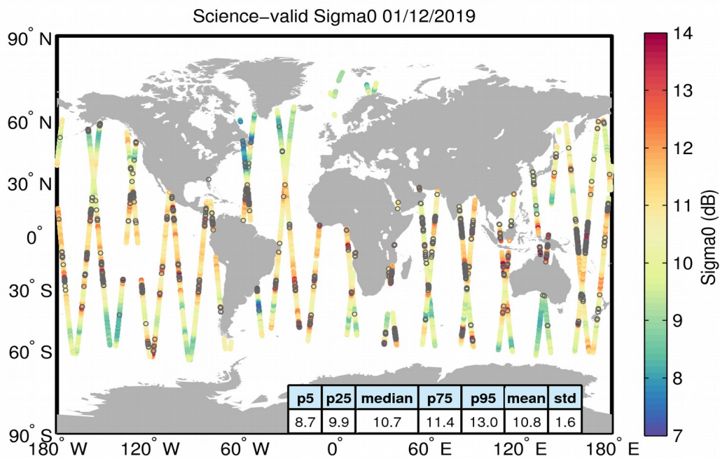
Figure 27. Geographical distribution of science-valid sigma0 data over oceans and lakes for 01/12/2019. The statistical values shown in the table refer to the sigma0 in dB and are calculated over all measurements shown in the figure. Gray circles denote records that have been rejected based on the editing criteria described in Table 4.
