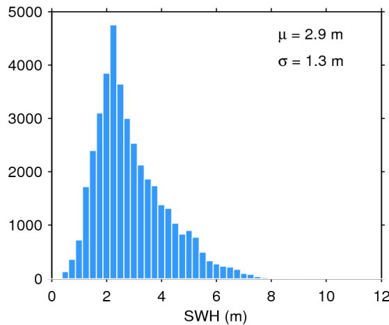
Figure 20. Histogram of science-valid SWH over oceans and lakes for 01/12/2019. The mean ( \mu ) and standard deviation ( \sigma ) are also shown. Note that values larger than 12 m are excluded from the histogram for the sake of readability but not from the computation of \mu and \sigma .
