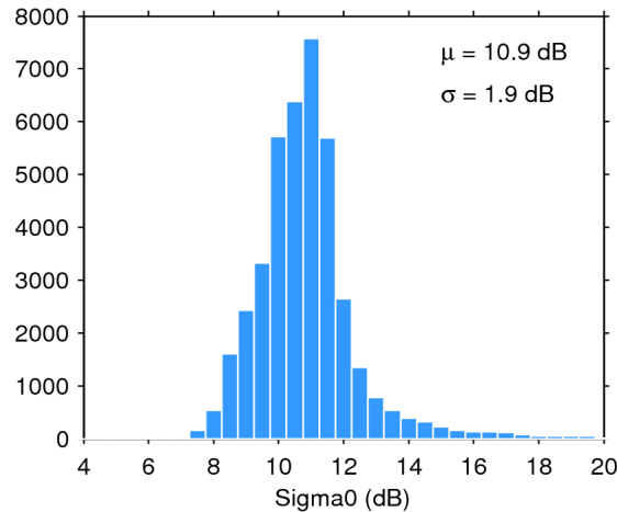
Figure 25. Histogram of flag-valid sigma0 over oceans and lakes for 01/12/2019. The mean ( \mu ) and standard deviation ( \sigma ) are also shown. Note that values outside [4 20] dB are excluded from the histogram for the sake of readability but not from the computation of \mu and \sigma .
