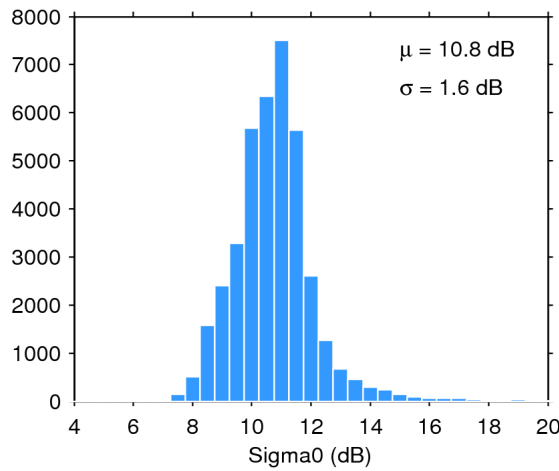
Figure 28. Histogram of science-valid sigma0 over oceans and lakes for 01/12/2019. The mean ( \mu ) and standard deviation ( \sigma ) are also shown. Note that values outside [4 20] dB are excluded from the histogram for the sake of readability but not from the computation of \mu and \sigma .
