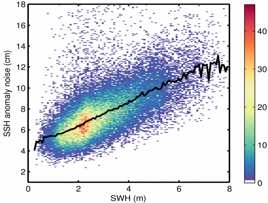
Figure 9. 2D histogram showing flag-valid SSH anomaly noise as a function of SWH for 01/12/2019. The black line denotes the median SSH anomaly noise as a function of SWH.
