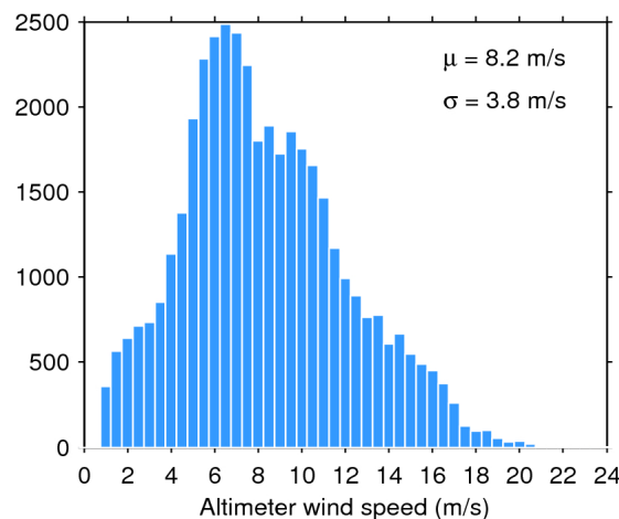
Figure 35. Histogram of science-valid wind over oceans and lakes for 01/12/2019. The mean ( \mu ) and standard deviation ( \sigma ) are also shown. Note that values larger than 24 m/s are excluded from the histogram for the sake of readability but not from the computation of \mu and \sigma .
