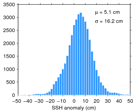
Figure 7. Histogram of flag-valid SSH anomaly over oceans and lakes for 01/12/2019. The mean ( \mu ) and standard deviation ( \sigma ) are also shown. Note that values outside [-50\ 50] cm are excluded from the histogram for the sake of readability but not from the computation of \mu and \sigma .
