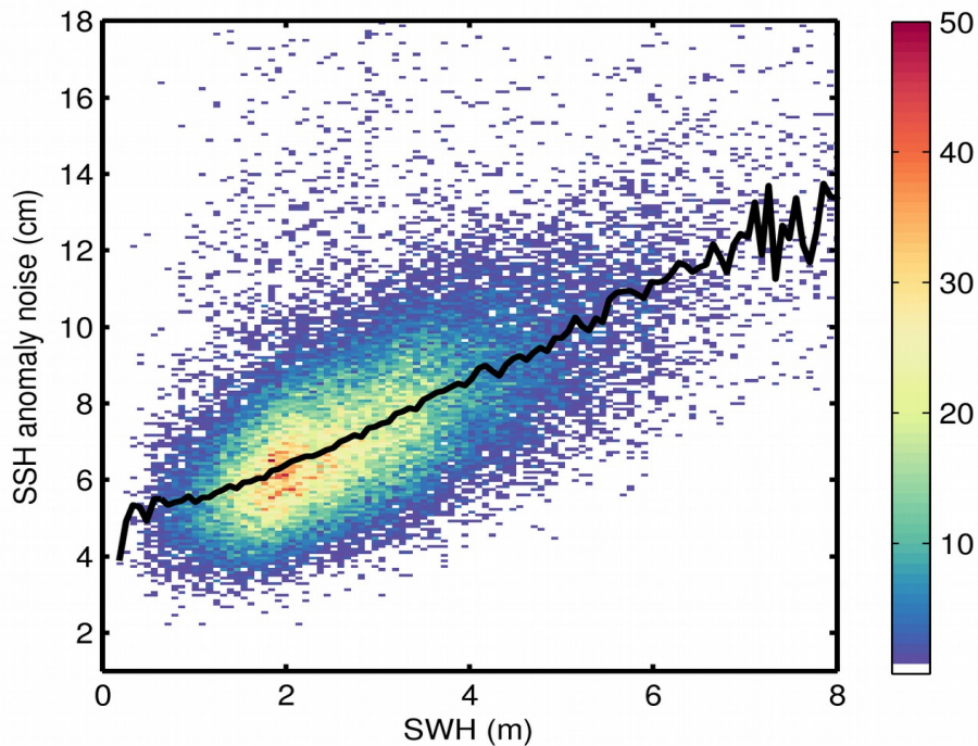
Figure 9. 2D histogram showing flag-valid SSH anomaly noise as a function of SWH for 25/11/2019. The black line denotes the median SSH anomaly noise as a function of SWH.
