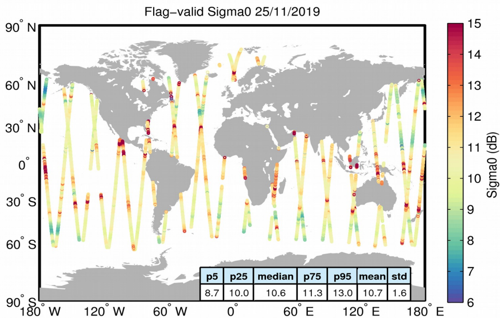
Figure 23. Geographical distribution of flag-valid sigma0 data over oceans and lakes for 25/11/2019. The statistical values shown in the table refer to the sigma0 in dB and are calculated over all measurements shown in the figure.
