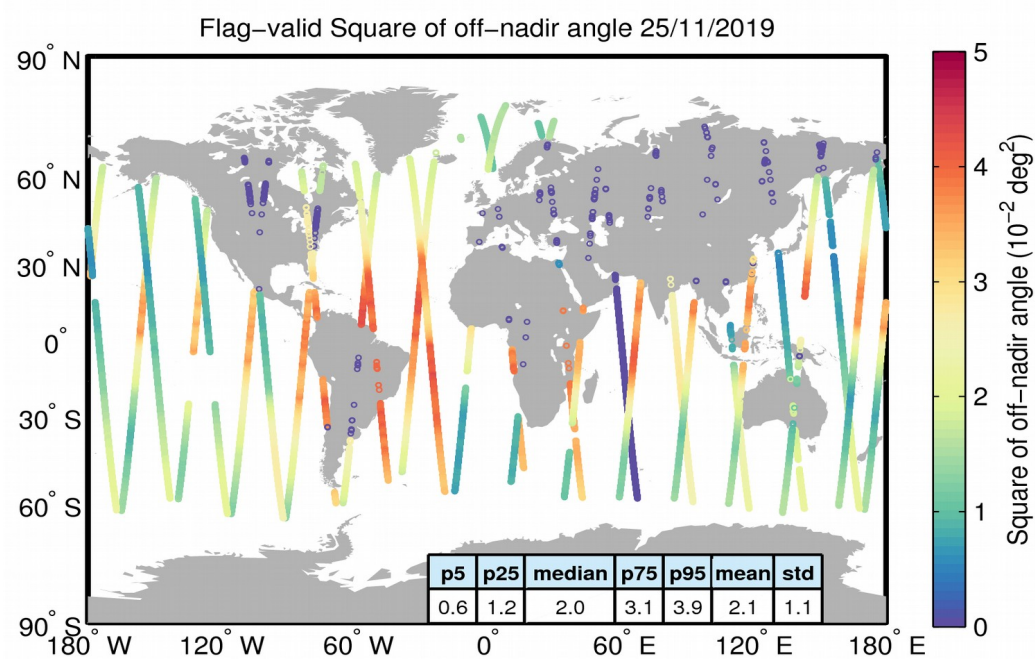
Figure 37. Geographical distribution of flag-valid mispointing data over oceans and lakes for 25/11/2019. The statistical values shown in the table refer to the mispointing in 10^{-2} deg 2 and are calculated over all measurements shown in the figure.
