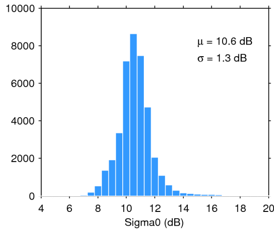
Figure 28. Histogram of science-valid sigma0 over oceans and lakes for 25/11/2019. The mean ( \mu ) and standard deviation ( \sigma ) are also shown. Note that values outside [4 20] dB are excluded from the histogram for the sake of readability but not from the computation of \mu and \sigma .
