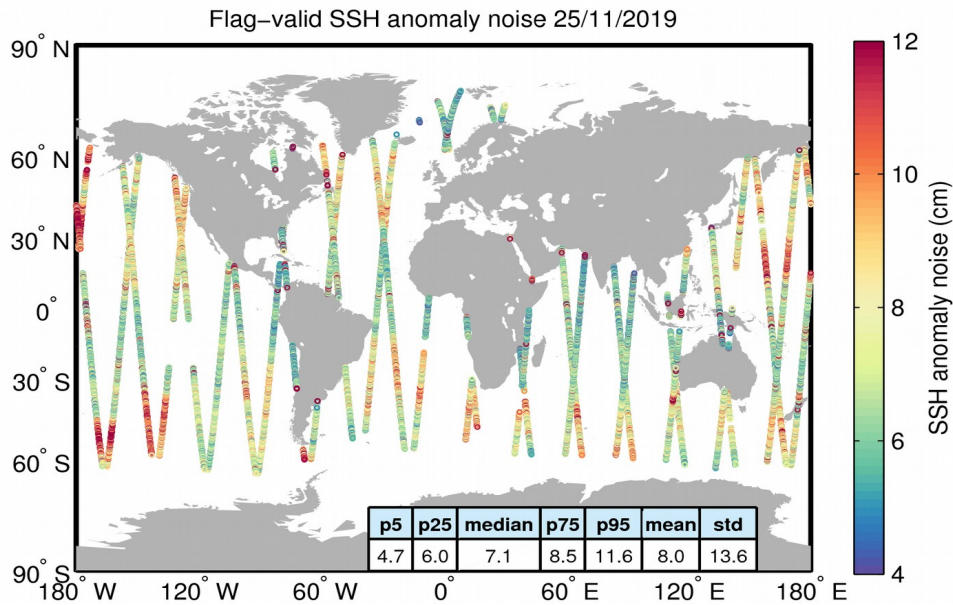
Figure 8. Geographical distribution of flag-valid 20-Hz SSH anomaly measurement noise over oceans and lakes for 25/11/2019. The statistical values shown in the table refer to the SSH anomaly noise and are calculated over all measurements shown in the figure.
