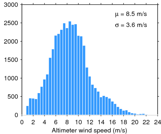
Figure 33. Histogram of flag-valid wind over oceans and lakes for 25/11/2019. The mean ( \mu ) and standard deviation ( \sigma ) are also shown. Note that values larger than 24 m/s are excluded from the histogram for the sake of readability but not from the computation of \mu and \sigma .
