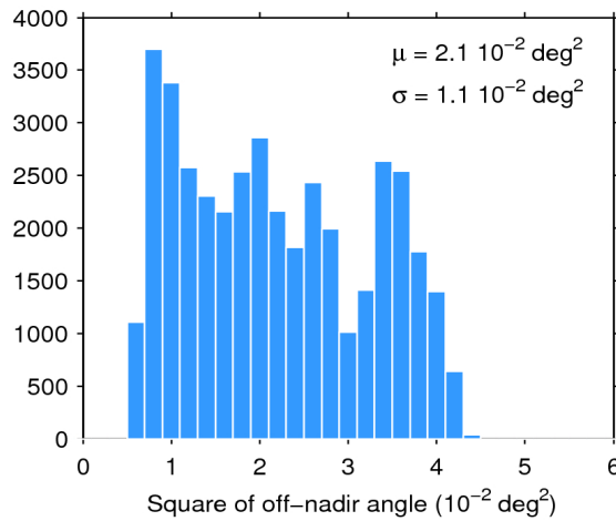
Figure 39. Histogram of flag-valid mispointing over oceans and lakes for 25/11/2019. The mean ( \mu ) and standard deviation ( \sigma ) are also shown. Note that values larger than 6 \cdot 10^{-2} \text{ deg}^2 are excluded from the histogram for the sake of readability but not from the computation of \mu and \sigma .
