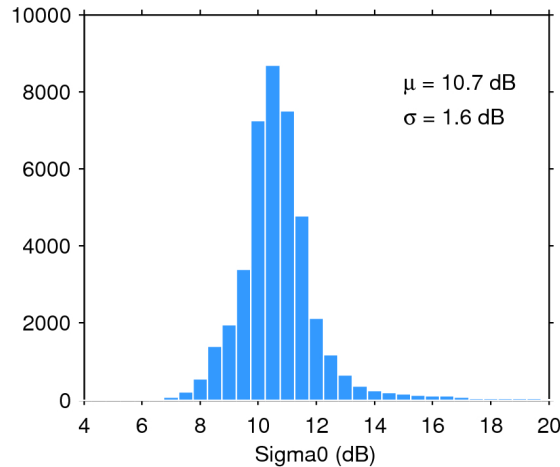
Figure 25. Histogram of flag-valid sigma0 over oceans and lakes for 25/11/2019. The mean ( \mu ) and standard deviation ( \sigma ) are also shown. Note that values outside [4 20] dB are excluded from the histogram for the sake of readability but not from the computation of \mu and \sigma .
