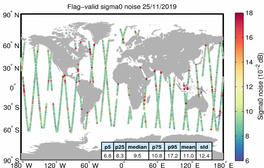
Figure 26. Geographical distribution of flag-valid 20-Hz sigma0 measurement noise over oceans and lakes for 25/11/2019. The statistical values shown in the table refer to the sigma0 noise and are calculated over all measurements shown in the figure.
