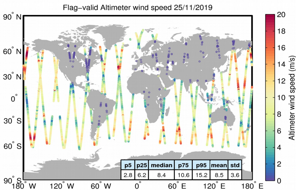
Figure 31. Geographical distribution of flag-valid wind data over oceans and lakes for 25/11/2019. The statistical values shown in the table refer to the wind in m/s and are calculated over all measurements shown in the figure.
