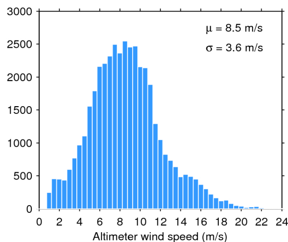
Figure 35. Histogram of science-valid wind over oceans and lakes for 25/11/2019. The mean ( \mu ) and standard deviation ( \sigma ) are also shown. Note that values larger than 24 m/s are excluded from the histogram for the sake of readability but not from the computation of \mu and \sigma .
