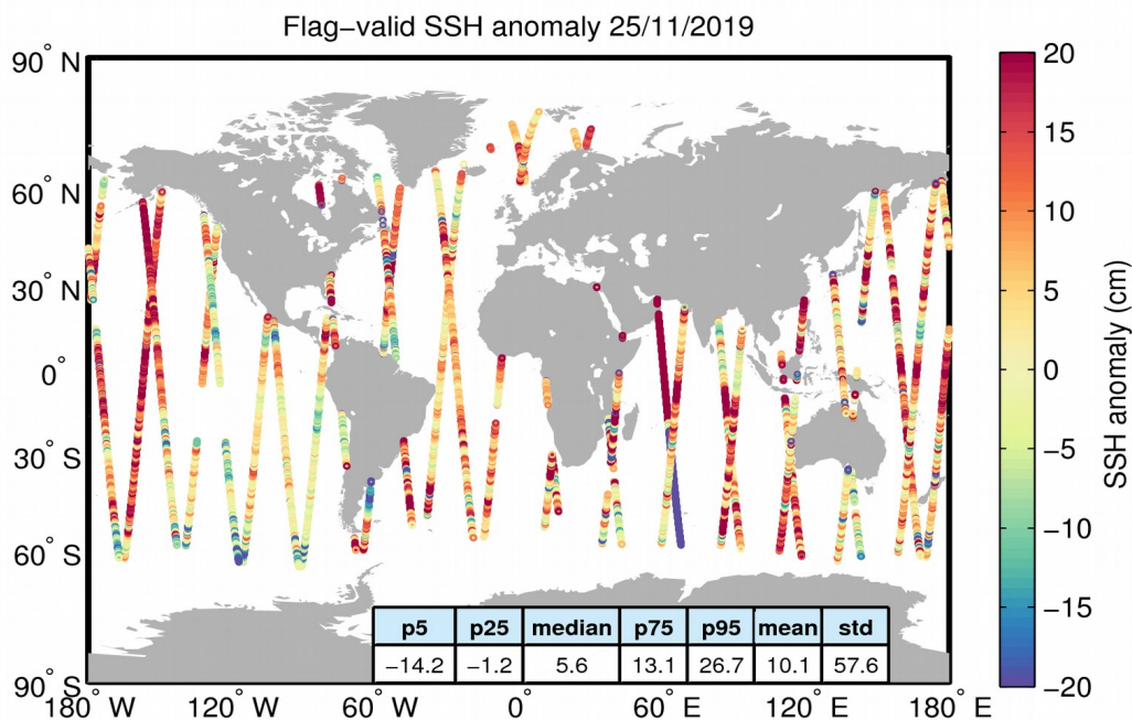
Figure 5. Geographical distribution of flag-valid 1-Hz SSH anomaly data over oceans and lakes for 25/11/2019. The statistical values shown in the table refer to the SSH anomaly in cm and are calculated over all measurements shown in the figure.
