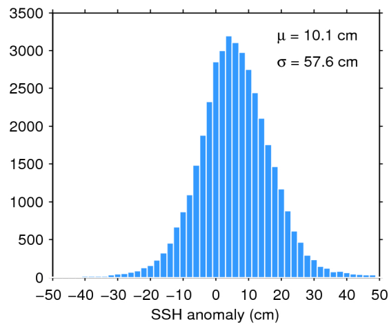
Figure 7. Histogram of flag-valid SSH anomaly over oceans and lakes for 25/11/2019. The mean ( \mu ) and standard deviation ( \sigma ) are also shown. Note that values outside [-50 50] cm are excluded from the histogram for the sake of readability but not from the computation of \mu and \sigma .
