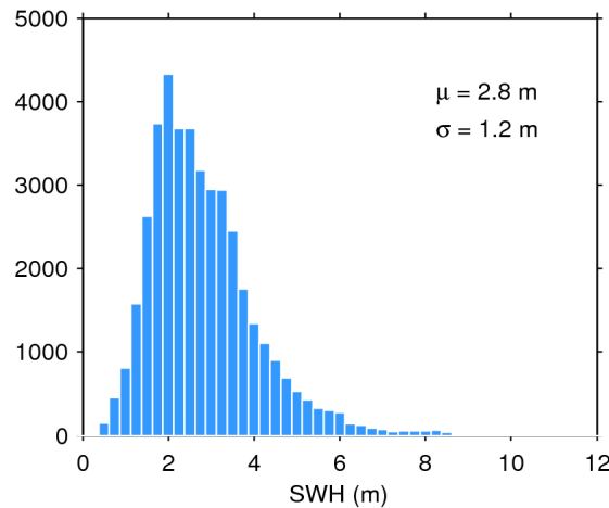
Figure 20. Histogram of science-valid SWH over oceans and lakes for 25/11/2019. The mean ( \mu ) and standard deviation ( \sigma ) are also shown. Note that values larger than 12 m are excluded from the histogram for the sake of readability but not from the computation of \mu and \sigma .
