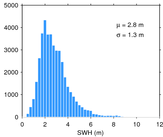
Figure 17. Histogram of flag-valid SWH over oceans and lakes for 25/11/2019. The mean ( \mu ) and standard deviation ( \sigma ) are also shown. Note that values larger than 12 m are excluded from the histogram for the sake of readability but not from the computation of \mu and \sigma .
