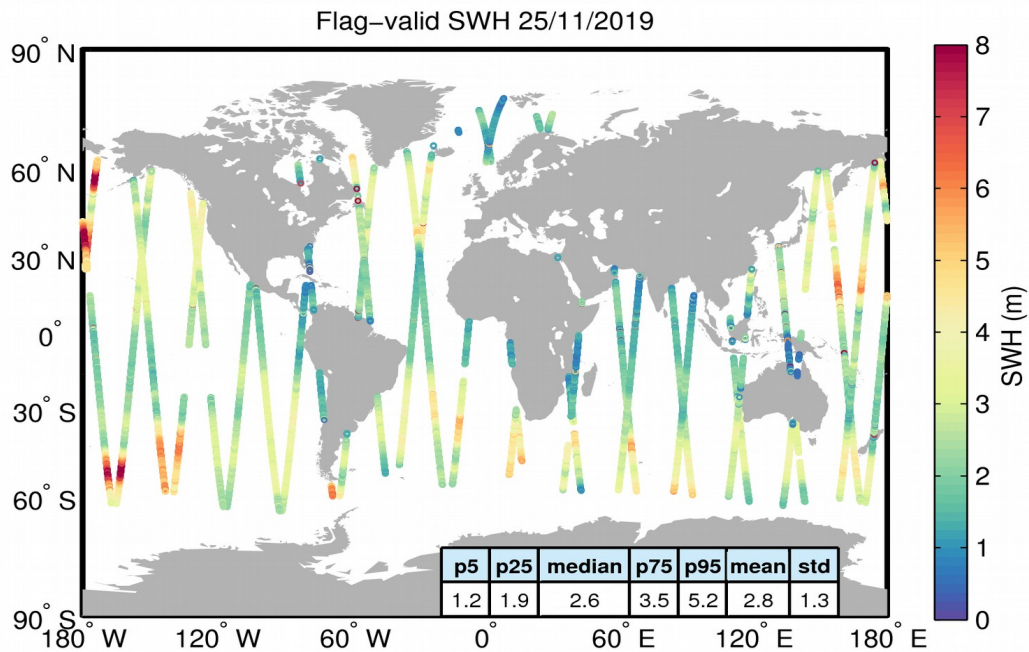
Figure 15. Geographical distribution of flag-valid SWH data over oceans and lakes for 25/11/2019. The statistical values shown in the table refer to the SWH in m and are calculated over all measurements shown in the figure.
