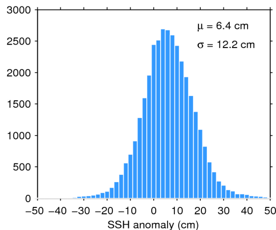
Figure 11. Histogram of science-valid SSH anomaly over oceans and lakes for 25/11/2019. The mean ( \mu ) and standard deviation ( \sigma ) are also shown. Note that values outside [-50 50] cm are excluded from the histogram for the sake of readability but not from the computation of \mu and \sigma .
