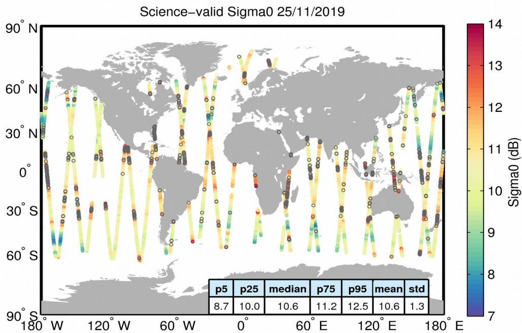
Figure 27. Geographical distribution of science-valid sigma0 data over oceans and lakes for 25/11/2019. The statistical values shown in the table refer to the sigma0 in dB and are calculated over all measurements shown in the figure. Gray circles denote records that have been rejected based on the editing criteria described in Table 4.
