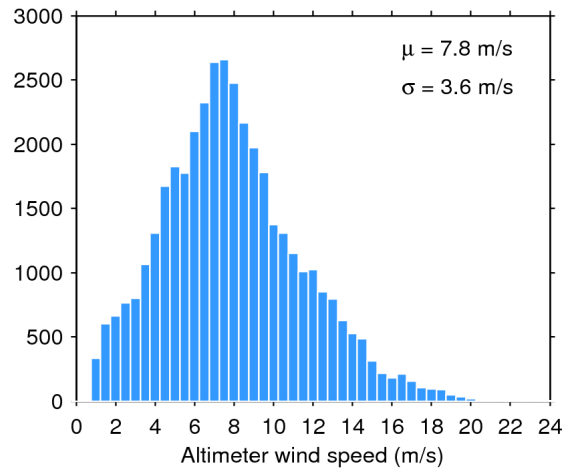
Figure 33. Histogram of flag-valid wind over oceans and lakes for 15/11/2019. The mean ( \mu ) and standard deviation ( \sigma ) are also shown. Note that values larger than 24 m/s are excluded from the histogram for the sake of readability but not from the computation of \mu and \sigma .
