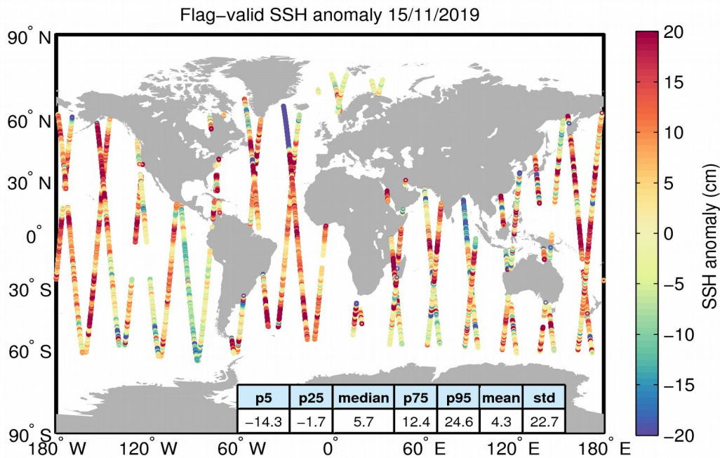
Figure 5. Geographical distribution of flag-valid 1-Hz SSH anomaly data over oceans and lakes for 15/11/2019. The statistical values shown in the table refer to the SSH anomaly in cm and are calculated over all measurements shown in the figure.
