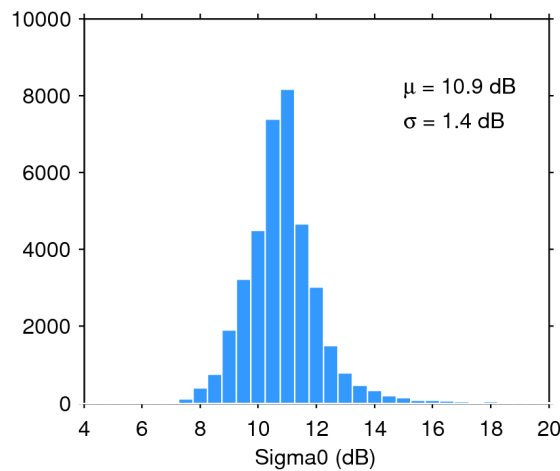
Figure 28. Histogram of science-valid sigma0 over oceans and lakes for 15/11/2019. The mean ( \mu ) and standard deviation ( \sigma ) are also shown. Note that values outside [4 20] dB are excluded from the histogram for the sake of readability but not from the computation of \mu and \sigma .
