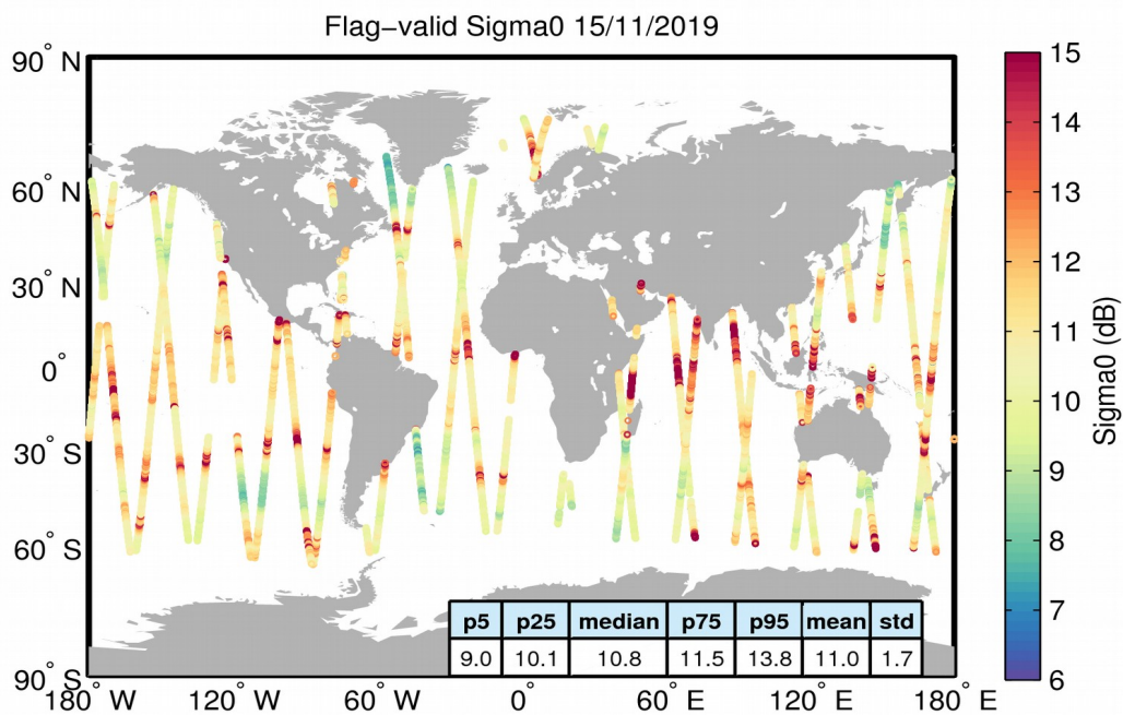
Figure 23. Geographical distribution of flag-valid sigma0 data over oceans and lakes for 15/11/2019. The statistical values shown in the table refer to the sigma0 in dB and are calculated over all measurements shown in the figure.
