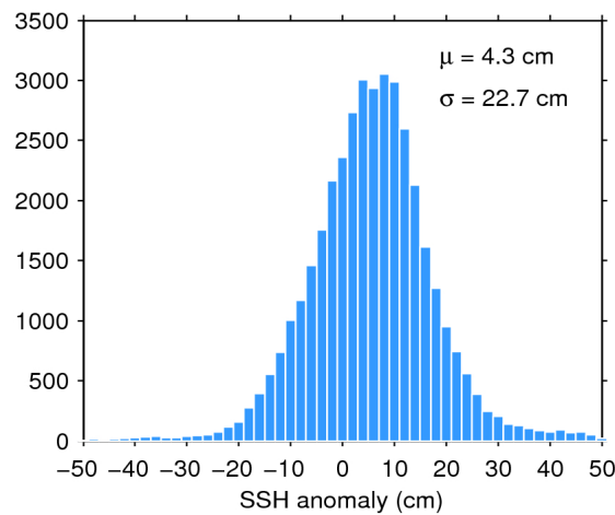
Figure 7. Histogram of flag-valid SSH anomaly over oceans and lakes for 15/11/2019. The mean ( \mu ) and standard deviation ( \sigma ) are also shown. Note that values outside [-50 50] cm are excluded from the histogram for the sake of readability but not from the computation of \mu and \sigma .
