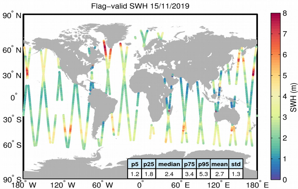
Figure 15. Geographical distribution of flag-valid SWH data over oceans and lakes for 15/11/2019. The statistical values shown in the table refer to the SWH in m and are calculated over all measurements shown in the figure.
