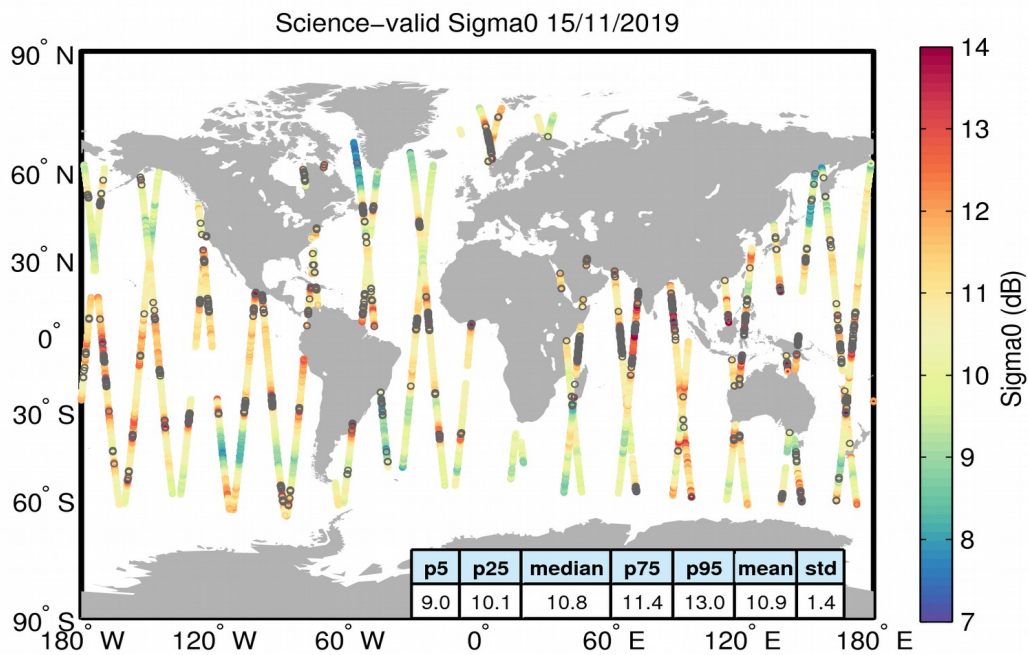
Figure 27. Geographical distribution of science-valid sigma0 data over oceans and lakes for 15/11/2019. The statistical values shown in the table refer to the sigma0 in dB and are calculated over all measurements shown in the figure. Gray circles denote records that have been rejected based on the editing criteria described in Table 4.
