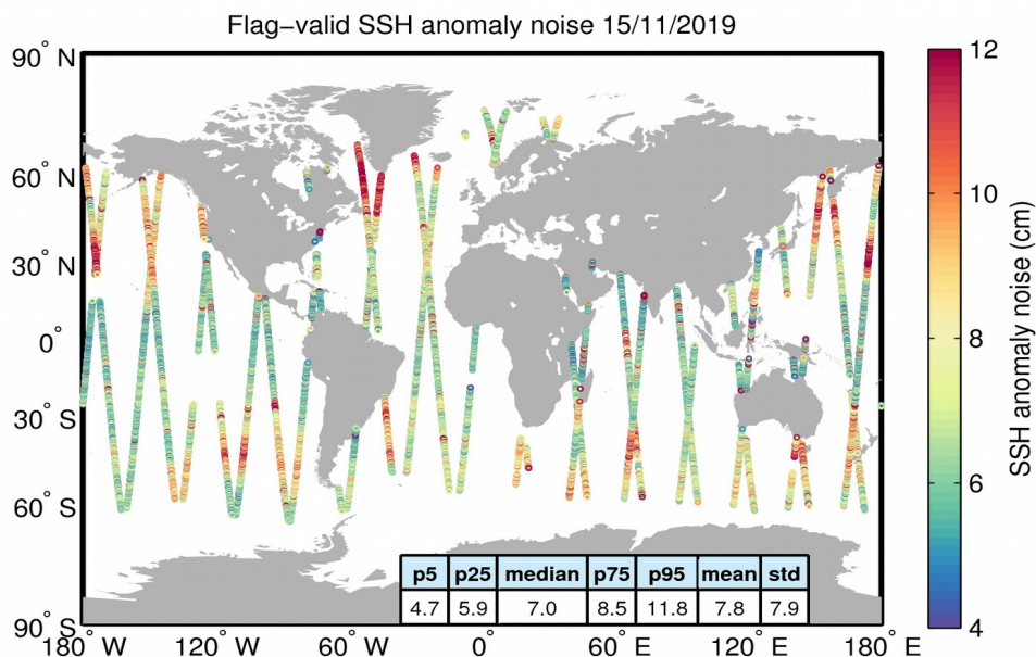
Figure 8. Geographical distribution of flag-valid 20-Hz SSH anomaly measurement noise over oceans and lakes for 15/11/2019. The statistical values shown in the table refer to the SSH anomaly noise and are calculated over all measurements shown in the figure.
