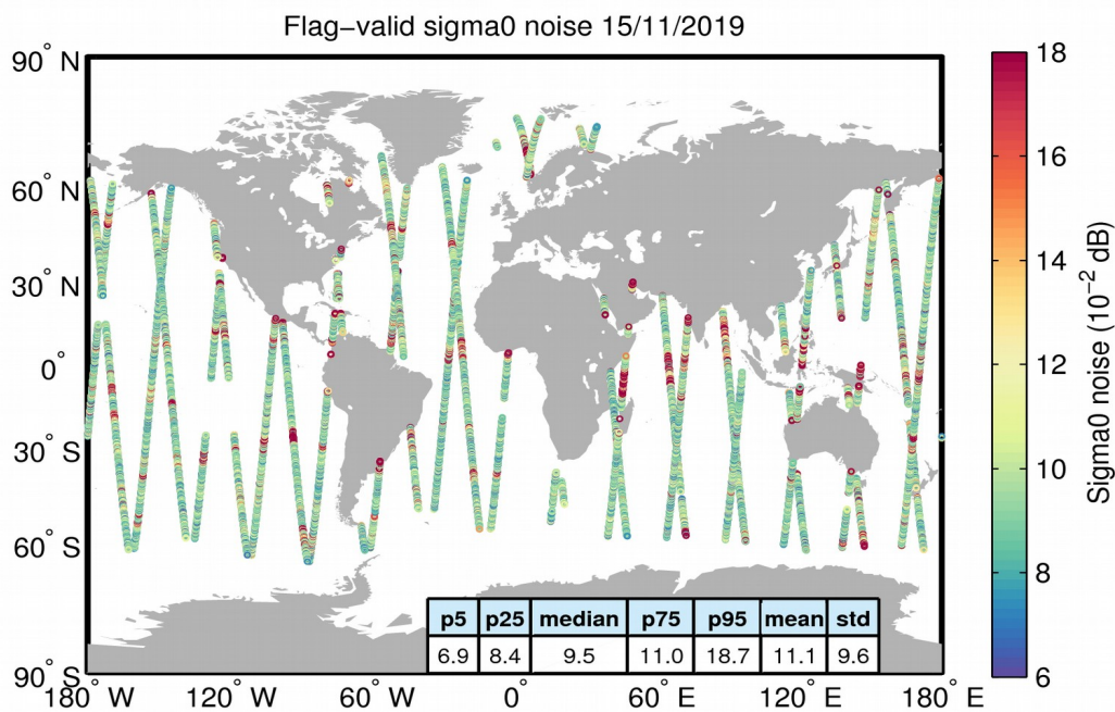
Figure 26. Geographical distribution of flag-valid 20-Hz sigma0 measurement noise over oceans and lakes for 15/11/2019. The statistical values shown in the table refer to the sigma0 noise and are calculated over all measurements shown in the figure.
