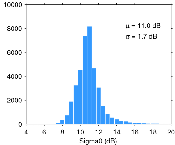
Figure 25. Histogram of flag-valid sigma0 over oceans and lakes for 15/11/2019. The mean ( \mu ) and standard deviation ( \sigma ) are also shown. Note that values outside [4 20] dB are excluded from the histogram for the sake of readability but not from the computation of \mu and \sigma .
