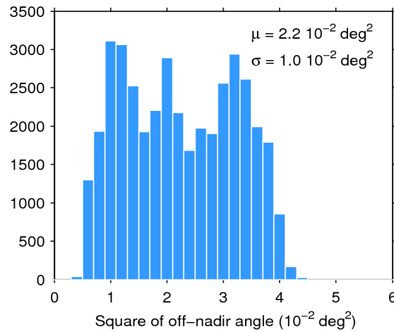
Figure 39. Histogram of flag-valid mispointing over oceans and lakes for 15/11/2019. The mean ( \mu ) and standard deviation ( \sigma ) are also shown. Note that values larger than 6 \cdot 10^{-2} \text{ deg}^2 are excluded from the histogram for the sake of readability but not from the computation of \mu and \sigma .
