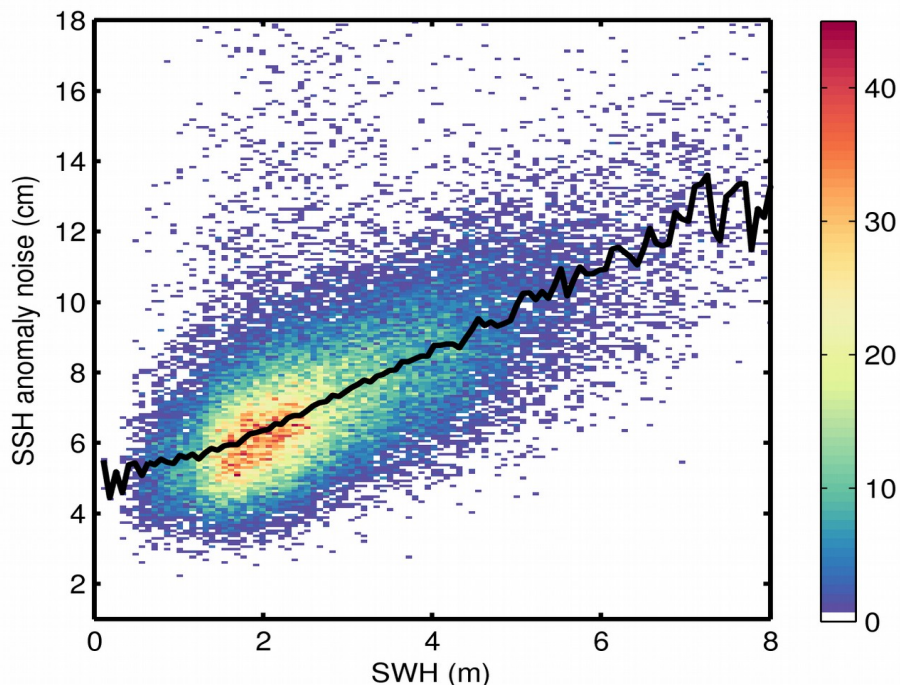
Figure 9. 2D histogram showing flag-valid SSH anomaly noise as a function of SWH for 15/11/2019. The black line denotes the median SSH anomaly noise as a function of SWH.
