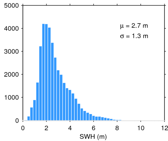
Figure 17. Histogram of flag-valid SWH over oceans and lakes for 15/11/2019. The mean ( \mu ) and standard deviation ( \sigma ) are also shown. Note that values larger than 12 m are excluded from the histogram for the sake of readability but not from the computation of \mu and \sigma .
