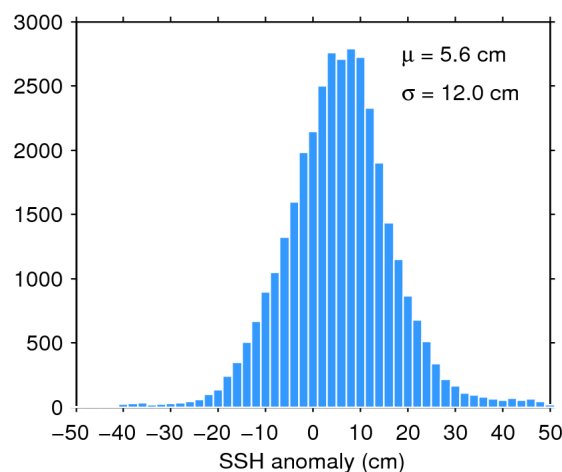
Figure 11. Histogram of science-valid SSH anomaly over oceans and lakes for 15/11/2019. The mean ( \mu ) and standard deviation ( \sigma ) are also shown. Note that values outside [-50 50] cm are excluded from the histogram for the sake of readability but not from the computation of \mu and \sigma .
