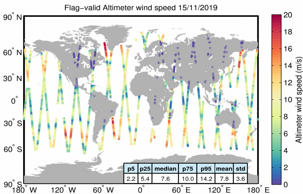
Figure 31. Geographical distribution of flag-valid wind data over oceans and lakes for 15/11/2019. The statistical values shown in the table refer to the wind in m/s and are calculated over all measurements shown in the figure.
