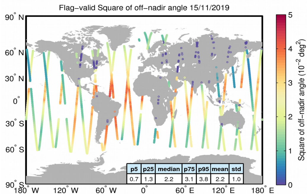
Figure 37. Geographical distribution of flag-valid mispointing data over oceans and lakes for 15/11/2019. The statistical values shown in the table refer to the mispointing in 10^{-2} deg 2 and are calculated over all measurements shown in the figure.
