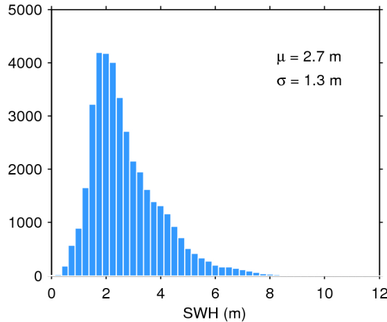
Figure 20. Histogram of science-valid SWH over oceans and lakes for 15/11/2019. The mean ( \mu ) and standard deviation ( \sigma ) are also shown. Note that values larger than 12 m are excluded from the histogram for the sake of readability but not from the computation of \mu and \sigma .
