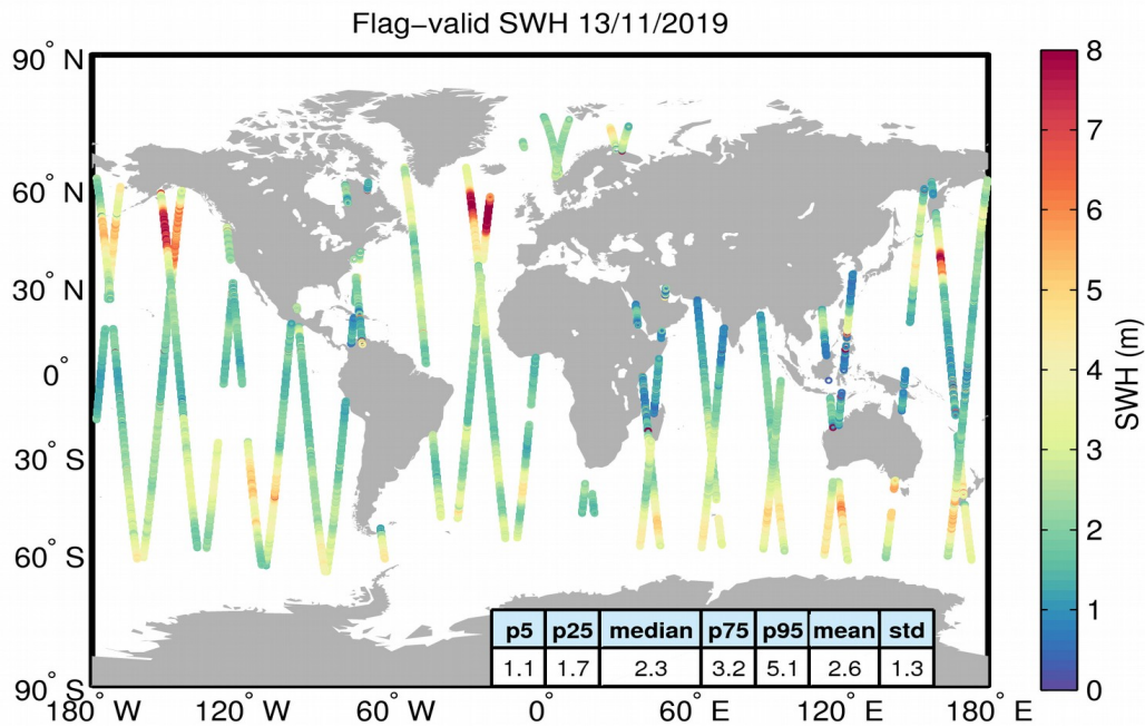
Figure 15. Geographical distribution of flag-valid SWH data over oceans and lakes for 13/11/2019. The statistical values shown in the table refer to the SWH in m and are calculated over all measurements shown in the figure.
