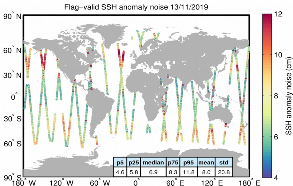
Figure 8. Geographical distribution of flag-valid 20-Hz SSH anomaly measurement noise over oceans and lakes for 13/11/2019. The statistical values shown in the table refer to the SSH anomaly noise and are calculated over all measurements shown in the figure.
