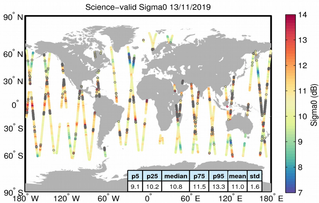
Figure 27. Geographical distribution of science-valid sigma0 data over oceans and lakes for 13/11/2019. The statistical values shown in the table refer to the sigma0 in dB and are calculated over all measurements shown in the figure. Gray circles denote records that have been rejected based on the editing criteria described in Table 4.
