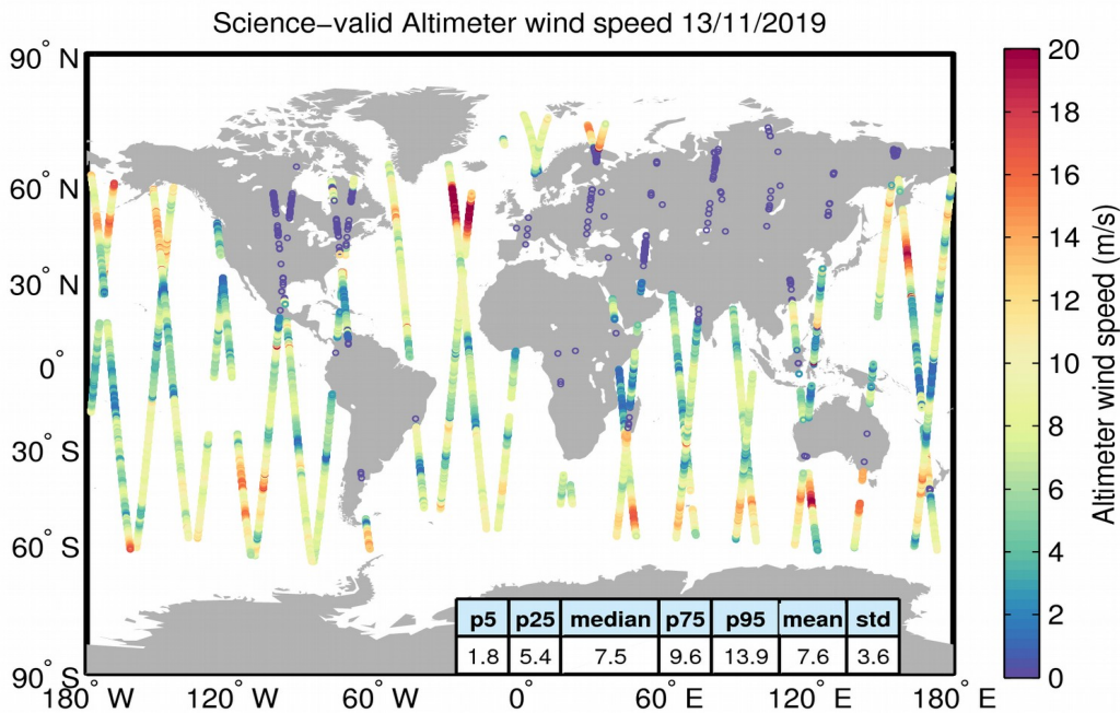
Figure 34. Geographical distribution of science-valid wind data over oceans and lakes for 13/11/2019. The statistical values shown in the table refer to the wind in m/s and are calculated over all measurements shown in the figure. Gray circles denote records that have been rejected based on the editing criteria described in Table 5.
