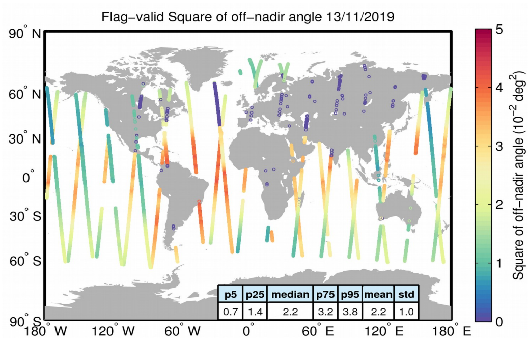
Figure 37. Geographical distribution of flag-valid mispointing data over oceans and lakes for 13/11/2019. The statistical values shown in the table refer to the mispointing in 10^{-2} deg 2 and are calculated over all measurements shown in the figure.
