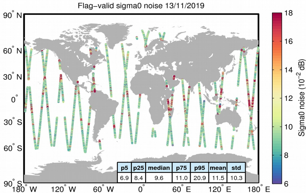
Figure 26. Geographical distribution of flag-valid 20-Hz sigma0 measurement noise over oceans and lakes for 13/11/2019. The statistical values shown in the table refer to the sigma0 noise and are calculated over all measurements shown in the figure.
