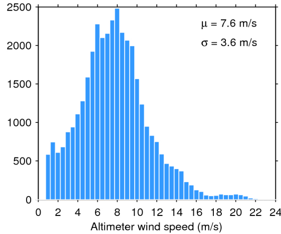
Figure 33. Histogram of flag-valid wind over oceans and lakes for 13/11/2019. The mean ( \mu ) and standard deviation ( \sigma ) are also shown. Note that values larger than 24 m/s are excluded from the histogram for the sake of readability but not from the computation of \mu and \sigma .
