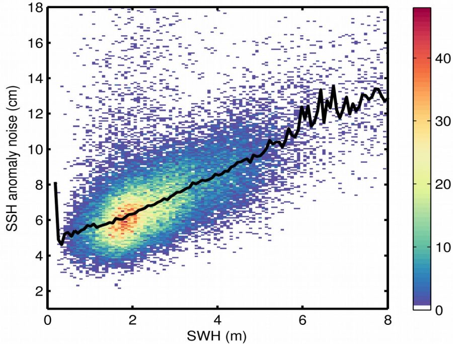
Figure 9. 2D histogram showing flag-valid SSH anomaly noise as a function of SWH for 13/11/2019. The black line denotes the median SSH anomaly noise as a function of SWH.
