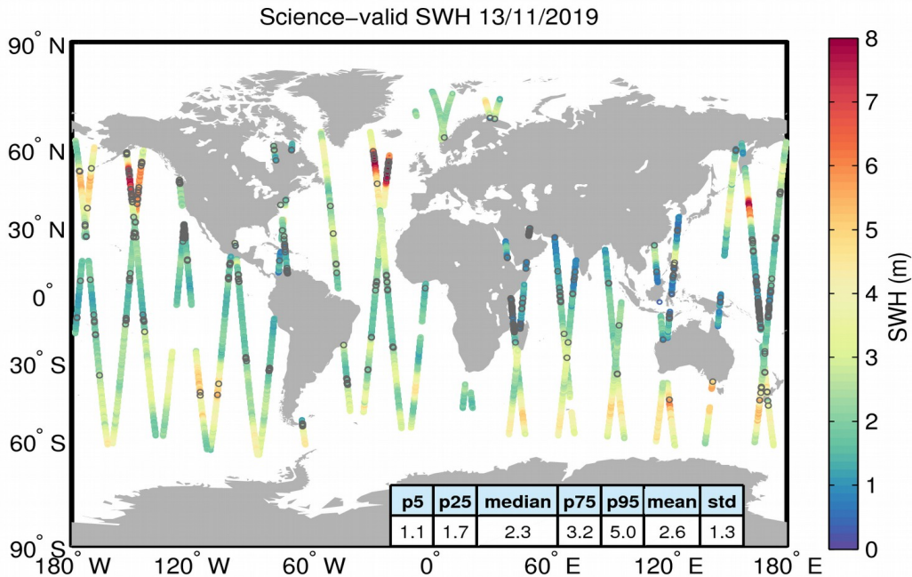
Figure 19. Geographical distribution of science-valid SWH data over oceans and lakes for 13/11/2019. The statistical values shown in the table refer to the SWH in m and are calculated over all measurements shown in the figure. Gray circles denote records that have been rejected based on the editing criteria described in Table 3.
