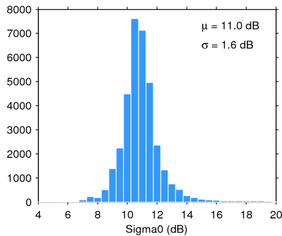
Figure 28. Histogram of science-valid sigma0 over oceans and lakes for 13/11/2019. The mean ( \mu ) and standard deviation ( \sigma ) are also shown. Note that values outside [4 20] dB are excluded from the histogram for the sake of readability but not from the computation of \mu and \sigma .
