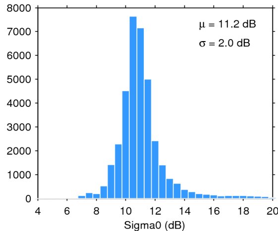
Figure 25. Histogram of flag-valid sigma0 over oceans and lakes for 13/11/2019. The mean ( \mu ) and standard deviation ( \sigma ) are also shown. Note that values outside [4 20] dB are excluded from the histogram for the sake of readability but not from the computation of \mu and \sigma .
