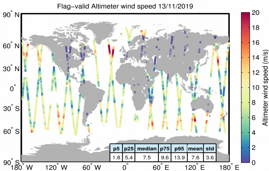
Figure 31. Geographical distribution of flag-valid wind data over oceans and lakes for 13/11/2019. The statistical values shown in the table refer to the wind in m/s and are calculated over all measurements shown in the figure.
