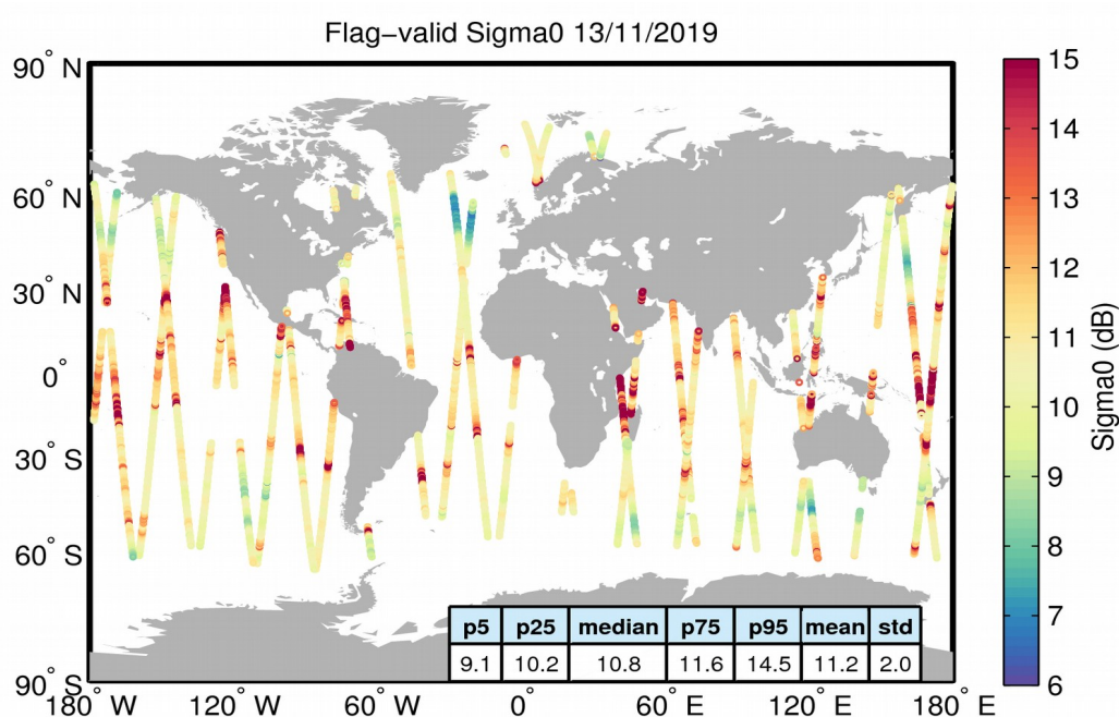
Figure 23. Geographical distribution of flag-valid sigma0 data over oceans and lakes for 13/11/2019. The statistical values shown in the table refer to the sigma0 in dB and are calculated over all measurements shown in the figure.
