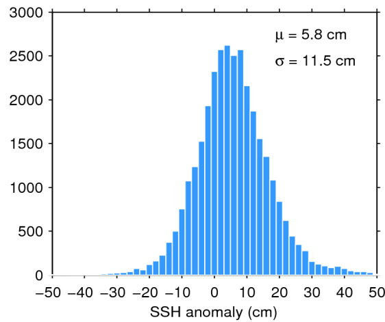
Figure 11. Histogram of science-valid SSH anomaly over oceans and lakes for 13/11/2019. The mean ( \mu ) and standard deviation ( \sigma ) are also shown. Note that values outside [-50 50] cm are excluded from the histogram for the sake of readability but not from the computation of \mu and \sigma .
