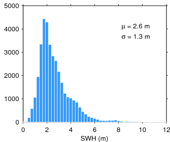
Figure 17. Histogram of flag-valid SWH over oceans and lakes for 13/11/2019. The mean ( \mu ) and standard deviation ( \sigma ) are also shown. Note that values larger than 12 m are excluded from the histogram for the sake of readability but not from the computation of \mu and \sigma .
