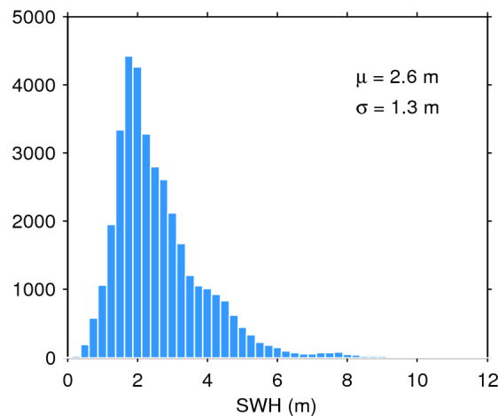
Figure 20. Histogram of science-valid SWH over oceans and lakes for 13/11/2019. The mean ( \mu ) and standard deviation ( \sigma ) are also shown. Note that values larger than 12 m are excluded from the histogram for the sake of readability but not from the computation of \mu and \sigma .
