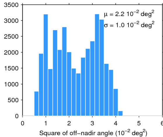
Figure 39. Histogram of flag-valid mispointing over oceans and lakes for 13/11/2019. The mean ( \mu ) and standard deviation ( \sigma ) are also shown. Note that values larger than 6 \cdot 10^{-2} \text{ deg}^2 are excluded from the histogram for the sake of readability but not from the computation of \mu and \sigma .
