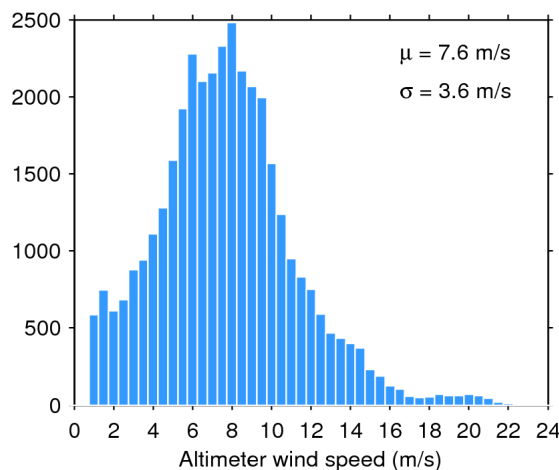
Figure 35. Histogram of science-valid wind over oceans and lakes for 13/11/2019. The mean ( \mu ) and standard deviation ( \sigma ) are also shown. Note that values larger than 24 m/s are excluded from the histogram for the sake of readability but not from the computation of \mu and \sigma .
