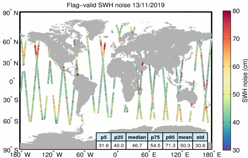
Figure 18. Geographical distribution of flag-valid 20-Hz SWH measurement noise over oceans and lakes for 13/11/2019. The statistical values shown in the figure refer to the SWH noise and are calculated over all measurements shown in the figure.
