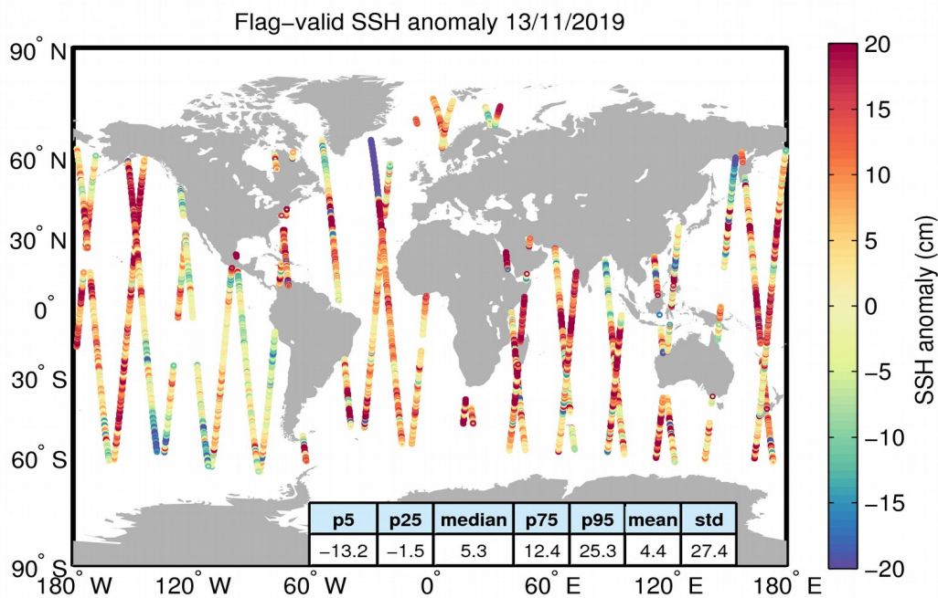
Figure 5. Geographical distribution of flag-valid 1-Hz SSH anomaly data over oceans and lakes for 13/11/2019. The statistical values shown in the table refer to the SSH anomaly in cm and are calculated over all measurements shown in the figure.
