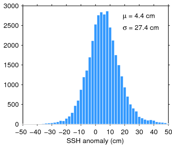
Figure 7. Histogram of flag-valid SSH anomaly over oceans and lakes for 13/11/2019. The mean ( \mu ) and standard deviation ( \sigma ) are also shown. Note that values outside [-50\ 50] cm are excluded from the histogram for the sake of readability but not from the computation of \mu and \sigma .
