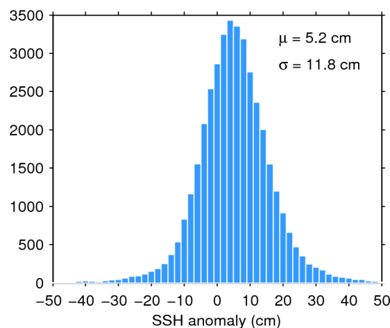
Figure 11. Histogram of science-valid SSH anomaly over oceans and lakes for 12/11/2019. The mean ( \mu ) and standard deviation ( \sigma ) are also shown. Note that values outside [-50 50] cm are excluded from the histogram for the sake of readability but not from the computation of \mu and \sigma .
