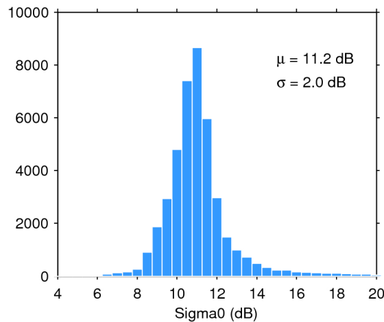
Figure 25. Histogram of flag-valid sigma0 over oceans and lakes for 12/11/2019. The mean ( \mu ) and standard deviation ( \sigma ) are also shown. Note that values outside [4 20] dB are excluded from the histogram for the sake of readability but not from the computation of \mu and \sigma .
