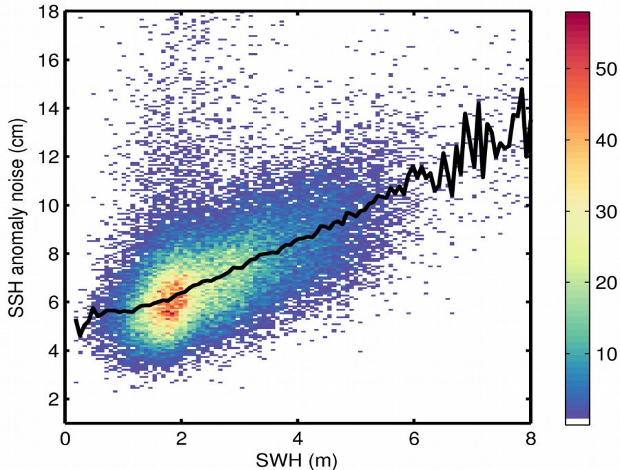
Figure 9. 2D histogram showing flag-valid SSH anomaly noise as a function of SWH for 12/11/2019. The black line denotes the median SSH anomaly noise as a function of SWH.
