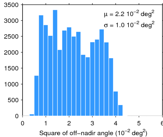
Figure 39. Histogram of flag-valid mispointing over oceans and lakes for 12/11/2019. The mean ( \mu ) and standard deviation ( \sigma ) are also shown. Note that values larger than 6 \cdot 10^{-2} \text{ deg}^2 are excluded from the histogram for the sake of readability but not from the computation of \mu and \sigma .
