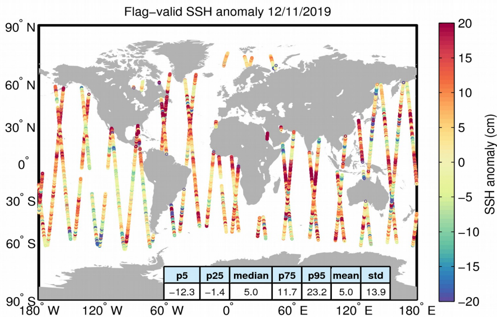
Figure 5. Geographical distribution of flag-valid 1-Hz SSH anomaly data over oceans and lakes for 12/11/2019. The statistical values shown in the table refer to the SSH anomaly in cm and are calculated over all measurements shown in the figure.
