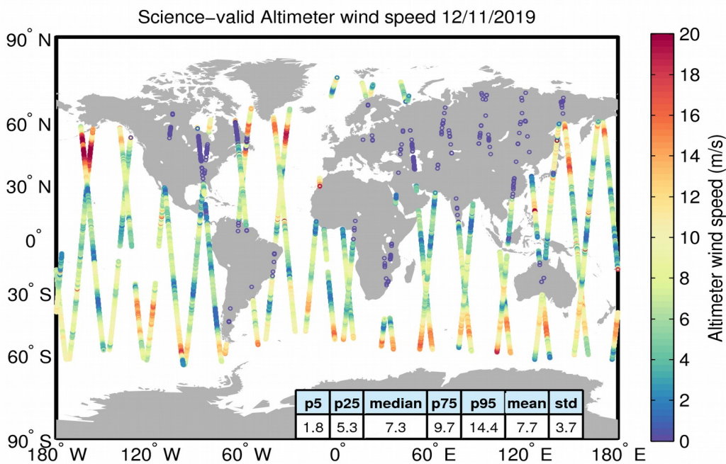
Figure 34. Geographical distribution of science-valid wind data over oceans and lakes for 12/11/2019. The statistical values shown in the table refer to the wind in m/s and are calculated over all measurements shown in the figure. Gray circles denote records that have been rejected based on the editing criteria described in Table 5.
