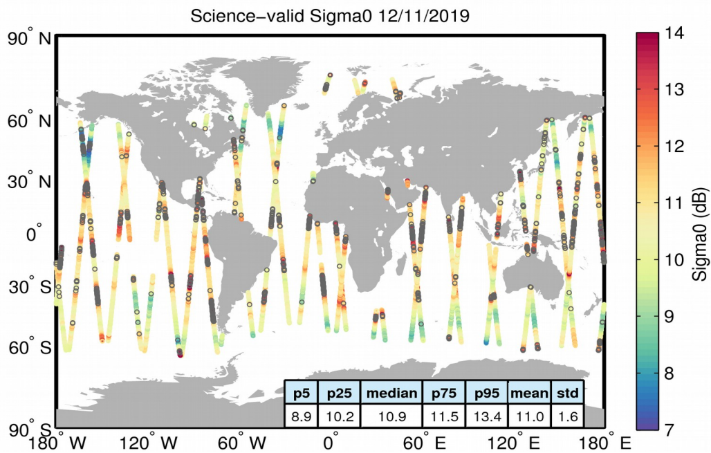
Figure 27. Geographical distribution of science-valid sigma0 data over oceans and lakes for 12/11/2019. The statistical values shown in the table refer to the sigma0 in dB and are calculated over all measurements shown in the figure. Gray circles denote records that have been rejected based on the editing criteria described in Table 4.
