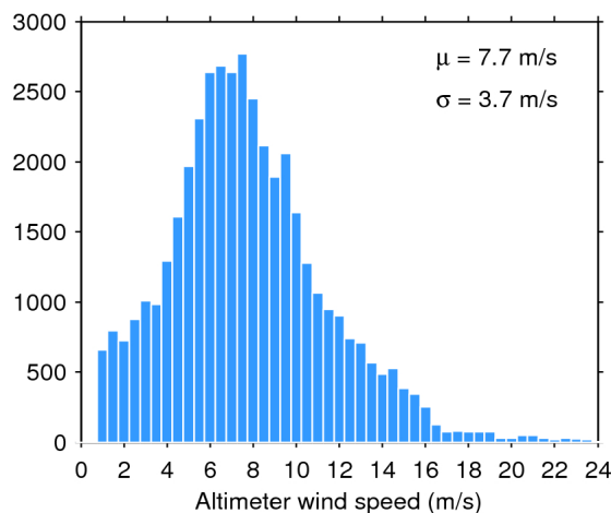
Figure 35. Histogram of science-valid wind over oceans and lakes for 12/11/2019. The mean ( \mu ) and standard deviation ( \sigma ) are also shown. Note that values larger than 24 m/s are excluded from the histogram for the sake of readability but not from the computation of \mu and \sigma .
