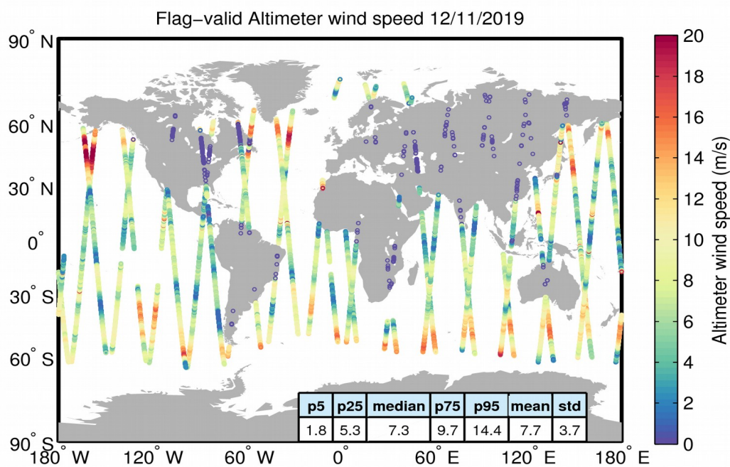
Figure 31. Geographical distribution of flag-valid wind data over oceans and lakes for 12/11/2019. The statistical values shown in the table refer to the wind in m/s and are calculated over all measurements shown in the figure.
