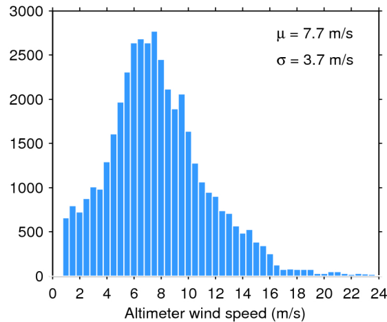
Figure 33. Histogram of flag-valid wind over oceans and lakes for 12/11/2019. The mean ( \mu ) and standard deviation ( \sigma ) are also shown. Note that values larger than 24 m/s are excluded from the histogram for the sake of readability but not from the computation of \mu and \sigma .
