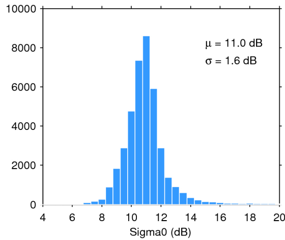
Figure 28. Histogram of science-valid sigma0 over oceans and lakes for 12/11/2019. The mean ( \mu ) and standard deviation ( \sigma ) are also shown. Note that values outside [4 20] dB are excluded from the histogram for the sake of readability but not from the computation of \mu and \sigma .
