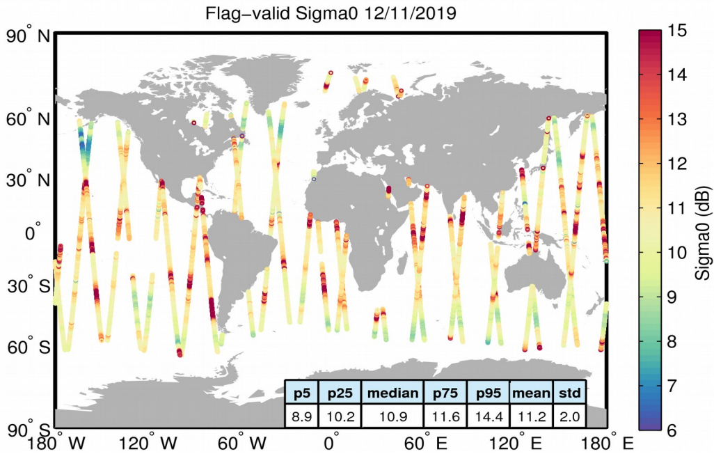
Figure 23. Geographical distribution of flag-valid sigma0 data over oceans and lakes for 12/11/2019. The statistical values shown in the table refer to the sigma0 in dB and are calculated over all measurements shown in the figure.
