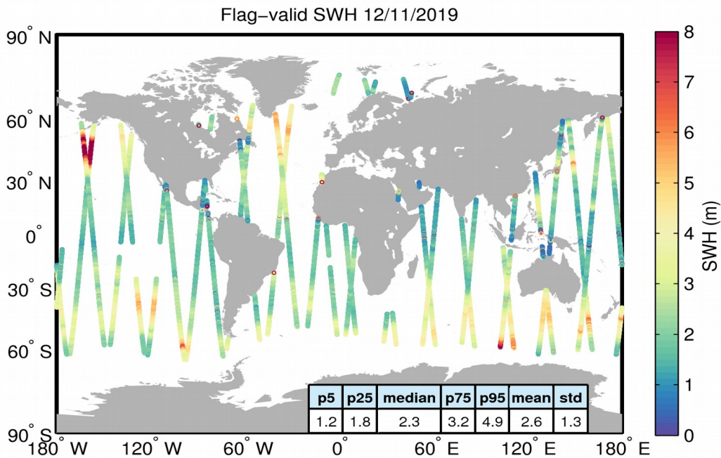
Figure 15. Geographical distribution of flag-valid SWH data over oceans and lakes for 12/11/2019. The statistical values shown in the table refer to the SWH in m and are calculated over all measurements shown in the figure.
