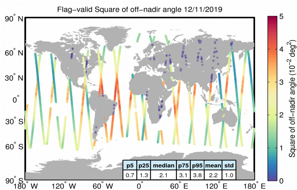
Figure 37. Geographical distribution of flag-valid mispointing data over oceans and lakes for 12/11/2019. The statistical values shown in the table refer to the mispointing in 10^{-2} \text{ deg}^2 and are calculated over all measurements shown in the figure.
