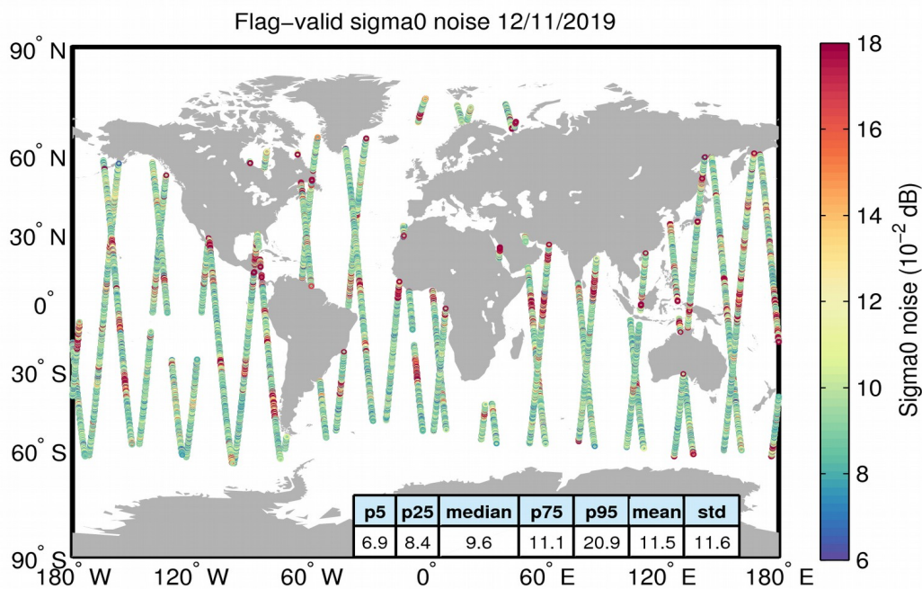
Figure 26. Geographical distribution of flag-valid 20-Hz sigma0 measurement noise over oceans and lakes for 12/11/2019. The statistical values shown in the table refer to the sigma0 noise and are calculated over all measurements shown in the figure.
