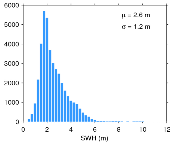
Figure 20. Histogram of science-valid SWH over oceans and lakes for 12/11/2019. The mean ( \mu ) and standard deviation ( \sigma ) are also shown. Note that values larger than 12 m are excluded from the histogram for the sake of readability but not from the computation of \mu and \sigma .
