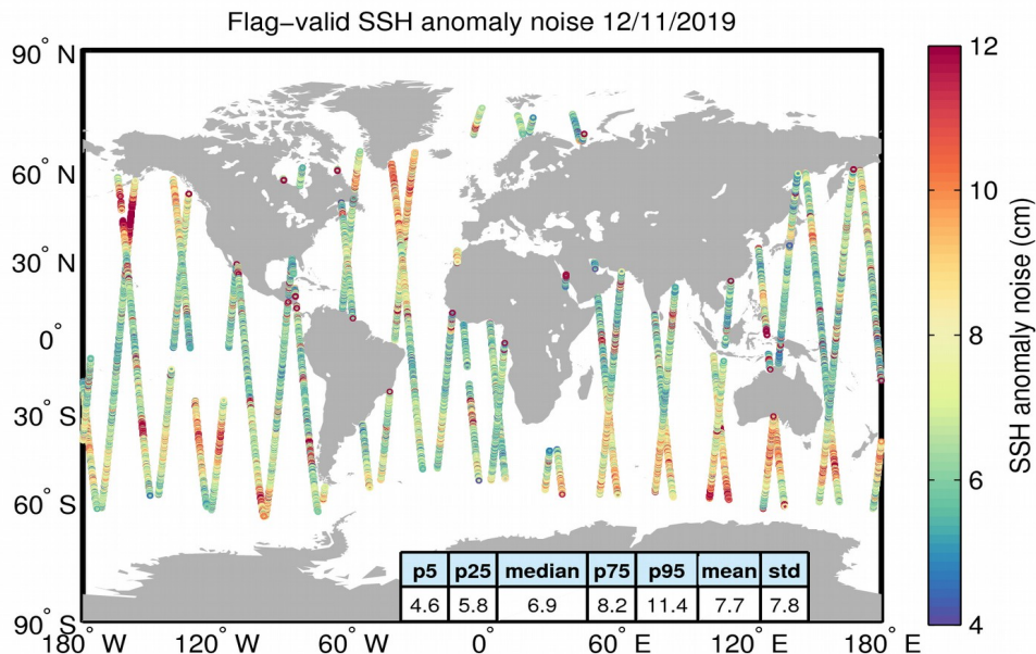
Figure 8. Geographical distribution of flag-valid 20-Hz SSH anomaly measurement noise over oceans and lakes for 12/11/2019. The statistical values shown in the table refer to the SSH anomaly noise and are calculated over all measurements shown in the figure.
