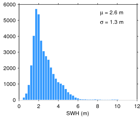
Figure 17. Histogram of flag-valid SWH over oceans and lakes for 12/11/2019. The mean ( \mu ) and standard deviation ( \sigma ) are also shown. Note that values larger than 12 m are excluded from the histogram for the sake of readability but not from the computation of \mu and \sigma .
