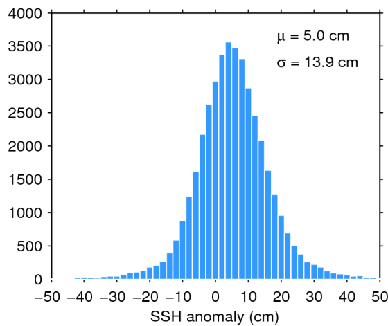
Figure 7. Histogram of flag-valid SSH anomaly over oceans and lakes for 12/11/2019. The mean ( \mu ) and standard deviation ( \sigma ) are also shown. Note that values outside [-50\ 50] cm are excluded from the histogram for the sake of readability but not from the computation of \mu and \sigma .
