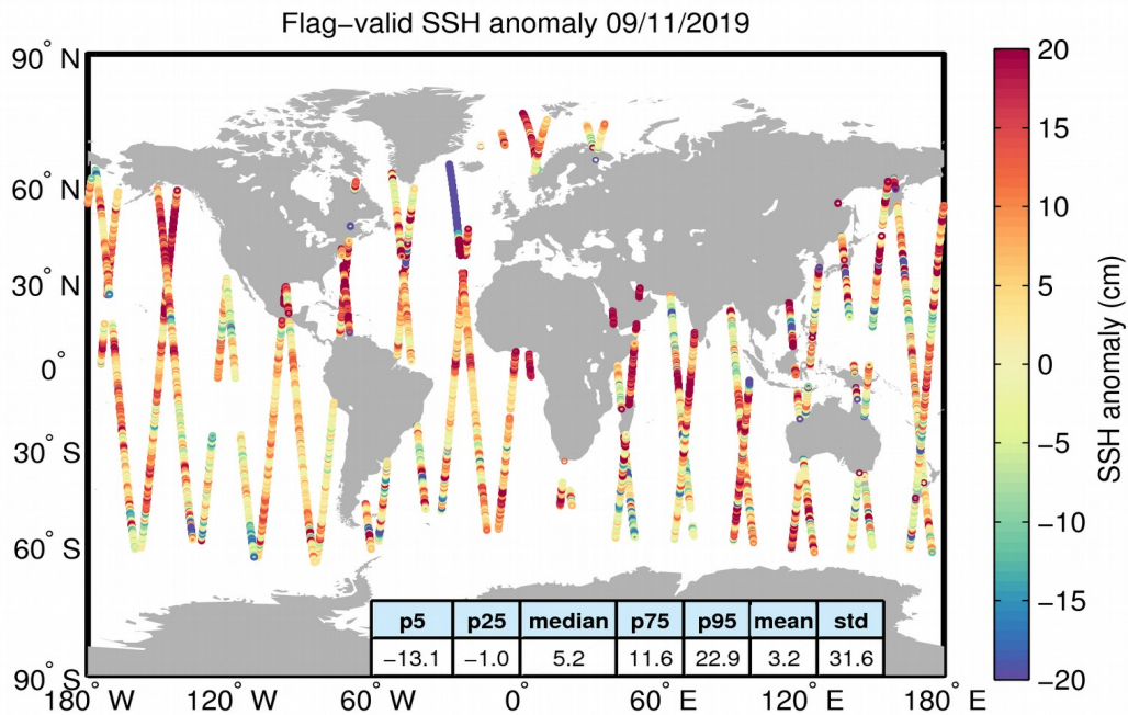
Figure 5. Geographical distribution of flag-valid 1-Hz SSH anomaly data over oceans and lakes for 09/11/2019. The statistical values shown in the table refer to the SSH anomaly in cm and are calculated over all measurements shown in the figure.
