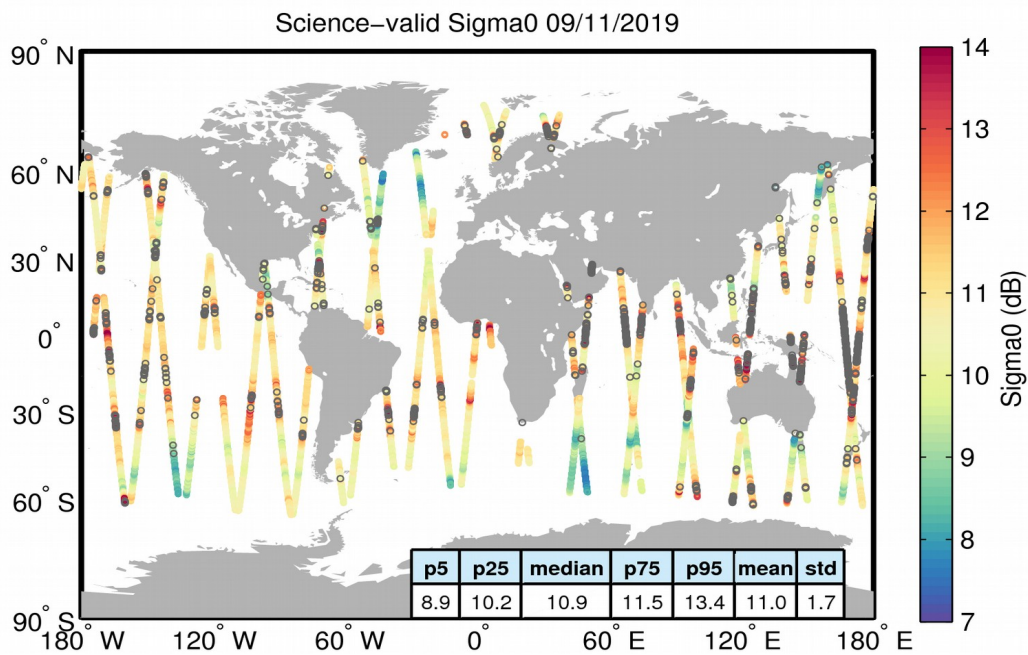
Figure 27. Geographical distribution of science-valid sigma0 data over oceans and lakes for 09/11/2019. The statistical values shown in the table refer to the sigma0 in dB and are calculated over all measurements shown in the figure. Gray circles denote records that have been rejected based on the editing criteria described in Table 4.
