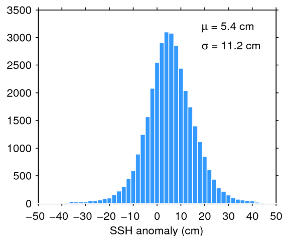
Figure 11. Histogram of science-valid SSH anomaly over oceans and lakes for 09/11/2019. The mean ( \mu ) and standard deviation ( \sigma ) are also shown. Note that values outside [-50 50] cm are excluded from the histogram for the sake of readability but not from the computation of \mu and \sigma .
