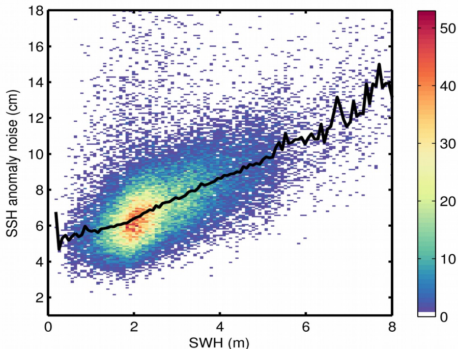
Figure 9. 2D histogram showing flag-valid SSH anomaly noise as a function of SWH for 09/11/2019. The black line denotes the median SSH anomaly noise as a function of SWH.
