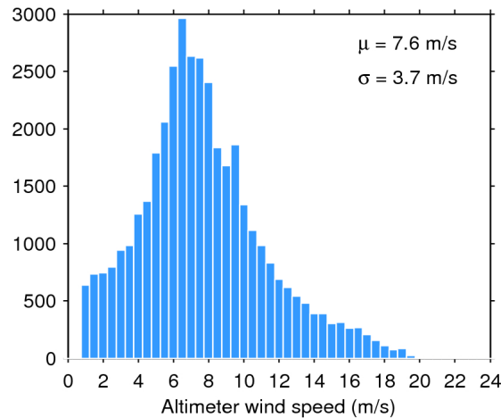
Figure 33. Histogram of flag-valid wind over oceans and lakes for 09/11/2019. The mean ( \mu ) and standard deviation ( \sigma ) are also shown. Note that values larger than 24 m/s are excluded from the histogram for the sake of readability but not from the computation of \mu and \sigma .
