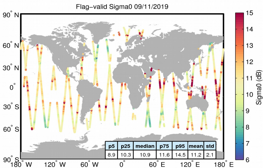
Figure 23. Geographical distribution of flag-valid sigma0 data over oceans and lakes for 09/11/2019. The statistical values shown in the table refer to the sigma0 in dB and are calculated over all measurements shown in the figure.
