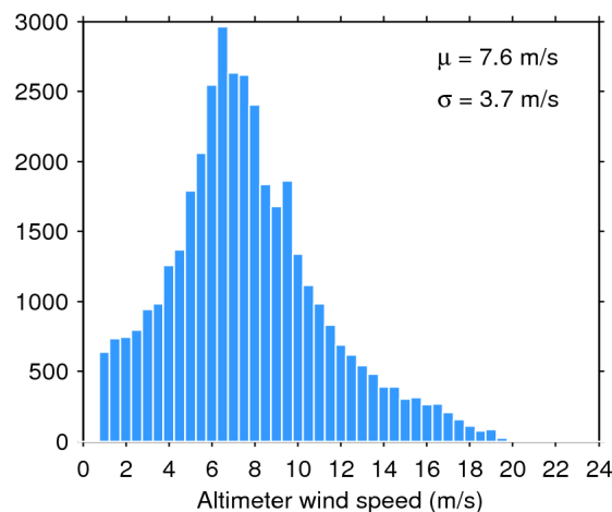
Figure 35. Histogram of science-valid wind over oceans and lakes for 09/11/2019. The mean ( \mu ) and standard deviation ( \sigma ) are also shown. Note that values larger than 24 m/s are excluded from the histogram for the sake of readability but not from the computation of \mu and \sigma .
