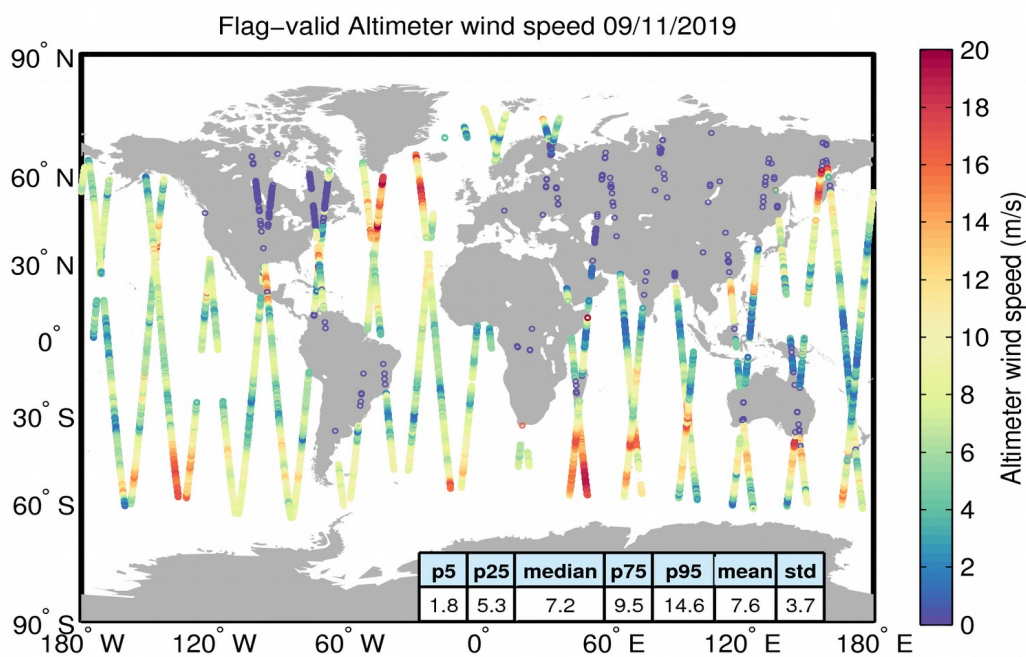
Figure 31. Geographical distribution of flag-valid wind data over oceans and lakes for 09/11/2019. The statistical values shown in the table refer to the wind in m/s and are calculated over all measurements shown in the figure.
