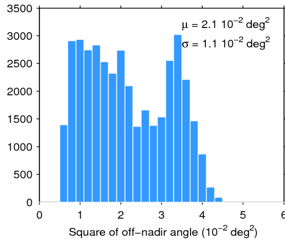
Figure 39. Histogram of flag-valid mispointing over oceans and lakes for 09/11/2019. The mean ( \mu ) and standard deviation ( \sigma ) are also shown. Note that values larger than 6 \cdot 10^{-2} \text{ deg}^2 are excluded from the histogram for the sake of readability but not from the computation of \mu and \sigma .
