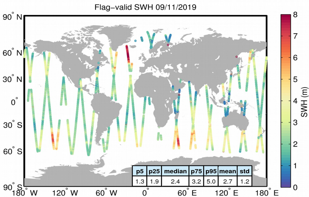
Figure 15. Geographical distribution of flag-valid SWH data over oceans and lakes for 09/11/2019. The statistical values shown in the table refer to the SWH in m and are calculated over all measurements shown in the figure.
