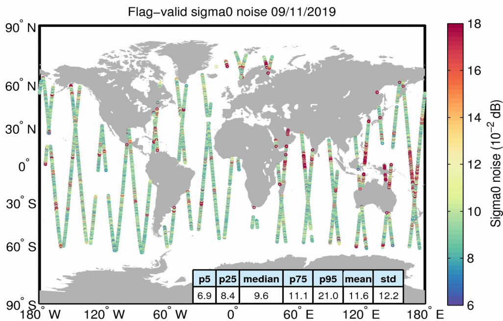
Figure 26. Geographical distribution of flag-valid 20-Hz sigma0 measurement noise over oceans and lakes for 09/11/2019. The statistical values shown in the table refer to the sigma0 noise and are calculated over all measurements shown in the figure.
