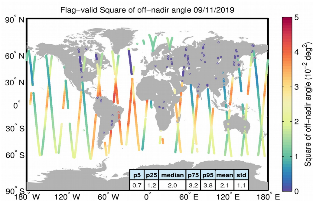
Figure 37. Geographical distribution of flag-valid mispointing data over oceans and lakes for 09/11/2019. The statistical values shown in the table refer to the mispointing in 10^{-2} \text{ deg}^2 and are calculated over all measurements shown in the figure.
