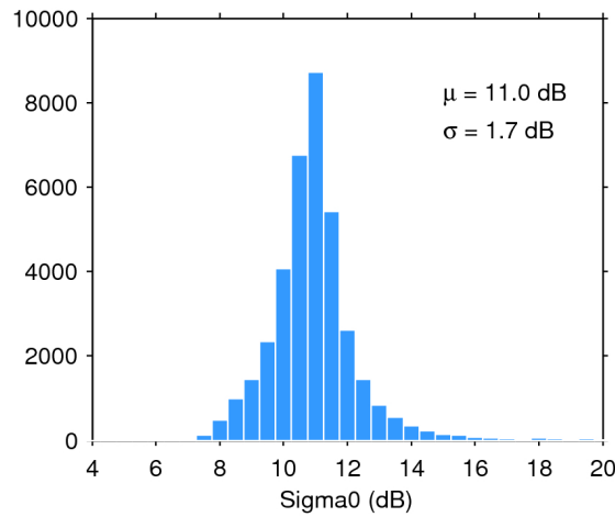
Figure 28. Histogram of science-valid sigma0 over oceans and lakes for 09/11/2019. The mean ( \mu ) and standard deviation ( \sigma ) are also shown. Note that values outside [4 20] dB are excluded from the histogram for the sake of readability but not from the computation of \mu and \sigma .
