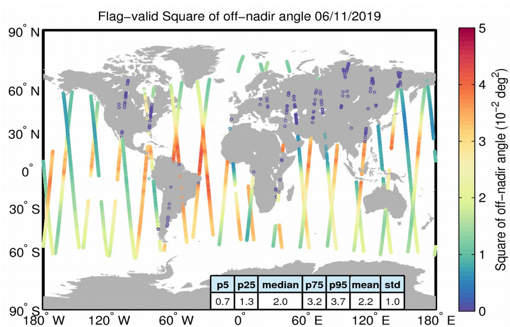
Figure 37. Geographical distribution of flag-valid mispointing data over oceans and lakes for 06/11/2019. The statistical values shown in the table refer to the mispointing in 10^{-2} \text{deg}^2 and are calculated over all measurements shown in the figure.
