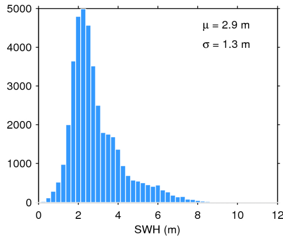
Figure 20. Histogram of science-valid SWH over oceans and lakes for 06/11/2019. The mean ( \mu ) and standard deviation ( \sigma ) are also shown. Note that values larger than 12 m are excluded from the histogram for the sake of readability but not from the computation of \mu and \sigma .
