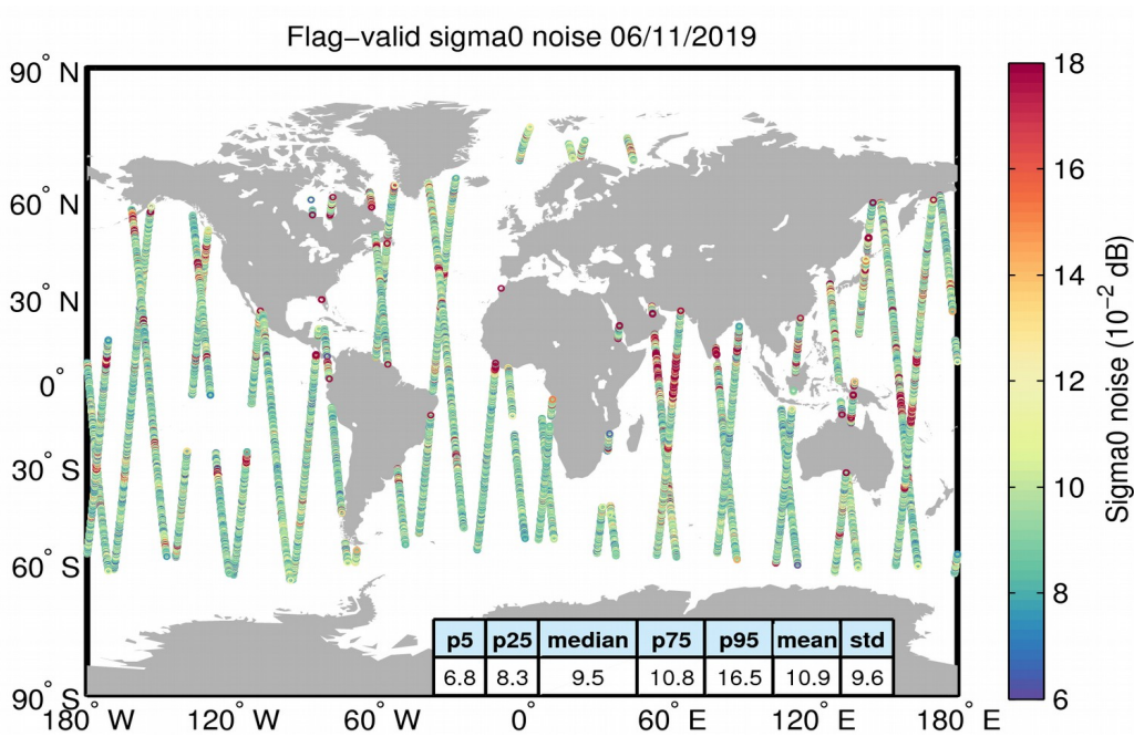
Figure 26. Geographical distribution of flag-valid 20-Hz sigma0 measurement noise over oceans and lakes for 06/11/2019. The statistical values shown in the table refer to the sigma0 noise and are calculated over all measurements shown in the figure.
