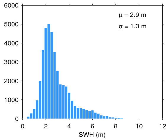
Figure 17. Histogram of flag-valid SWH over oceans and lakes for 06/11/2019. The mean ( \mu ) and standard deviation ( \sigma ) are also shown. Note that values larger than 12 m are excluded from the histogram for the sake of readability but not from the computation of \mu and \sigma .
