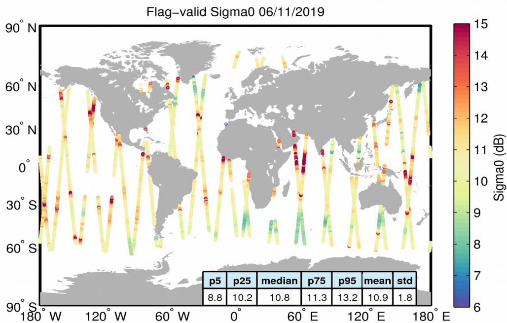
Figure 23. Geographical distribution of flag-valid sigma0 data over oceans and lakes for 06/11/2019. The statistical values shown in the table refer to the sigma0 in dB and are calculated over all measurements shown in the figure.
