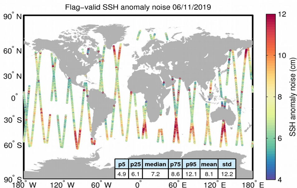
Figure 8. Geographical distribution of flag-valid 20-Hz SSH anomaly measurement noise over oceans and lakes for 06/11/2019. The statistical values shown in the table refer to the SSH anomaly noise and are calculated over all measurements shown in the figure.
