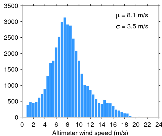
Figure 35. Histogram of science-valid wind over oceans and lakes for 06/11/2019. The mean ( \mu ) and standard deviation ( \sigma ) are also shown. Note that values larger than 24 m/s are excluded from the histogram for the sake of readability but not from the computation of \mu and \sigma .
