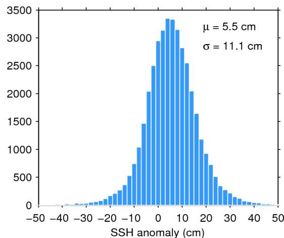
Figure 11. Histogram of science-valid SSH anomaly over oceans and lakes for 06/11/2019. The mean ( \mu ) and standard deviation ( \sigma ) are also shown. Note that values outside [-50 50] cm are excluded from the histogram for the sake of readability but not from the computation of \mu and \sigma .
