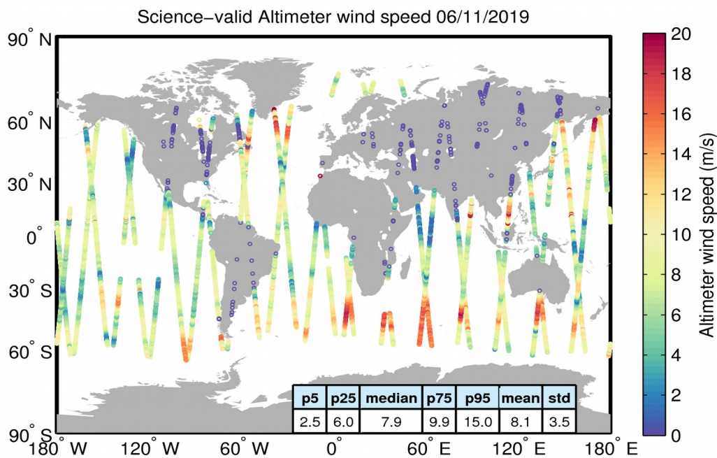
Figure 34. Geographical distribution of science-valid wind data over oceans and lakes for 06/11/2019. The statistical values shown in the table refer to the wind in m/s and are calculated over all measurements shown in the figure. Gray circles denote records that have been rejected based on the editing criteria described in Table 5.
