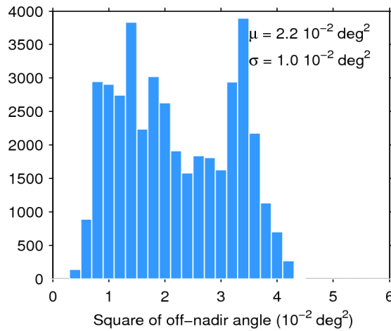
Figure 39. Histogram of flag-valid mispointing over oceans and lakes for 06/11/2019. The mean ( \mu ) and standard deviation ( \sigma ) are also shown. Note that values larger than 6 \cdot 10^{-2} \text{ deg}^2 are excluded from the histogram for the sake of readability but not from the computation of \mu and \sigma .
