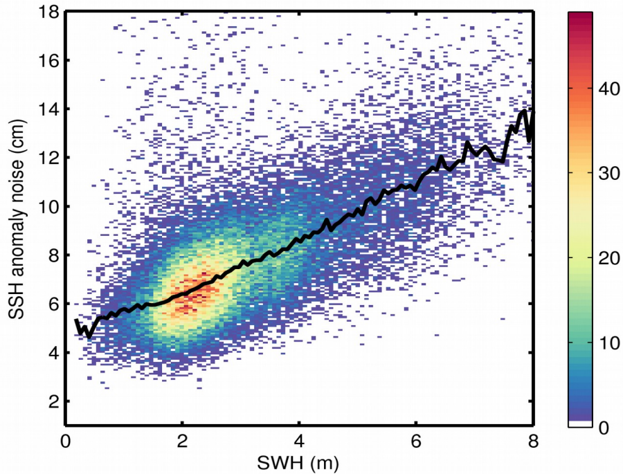
Figure 9. 2D histogram showing flag-valid SSH anomaly noise as a function of SWH for 06/11/2019. The black line denotes the median SSH anomaly noise as a function of SWH.
