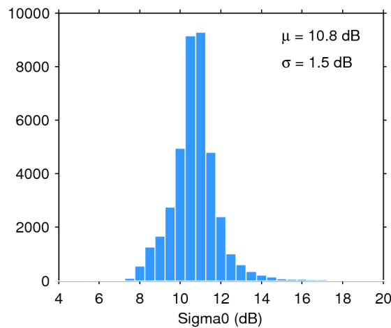
Figure 28. Histogram of science-valid sigma0 over oceans and lakes for 06/11/2019. The mean ( \mu ) and standard deviation ( \sigma ) are also shown. Note that values outside [4 20] dB are excluded from the histogram for the sake of readability but not from the computation of \mu and \sigma .
