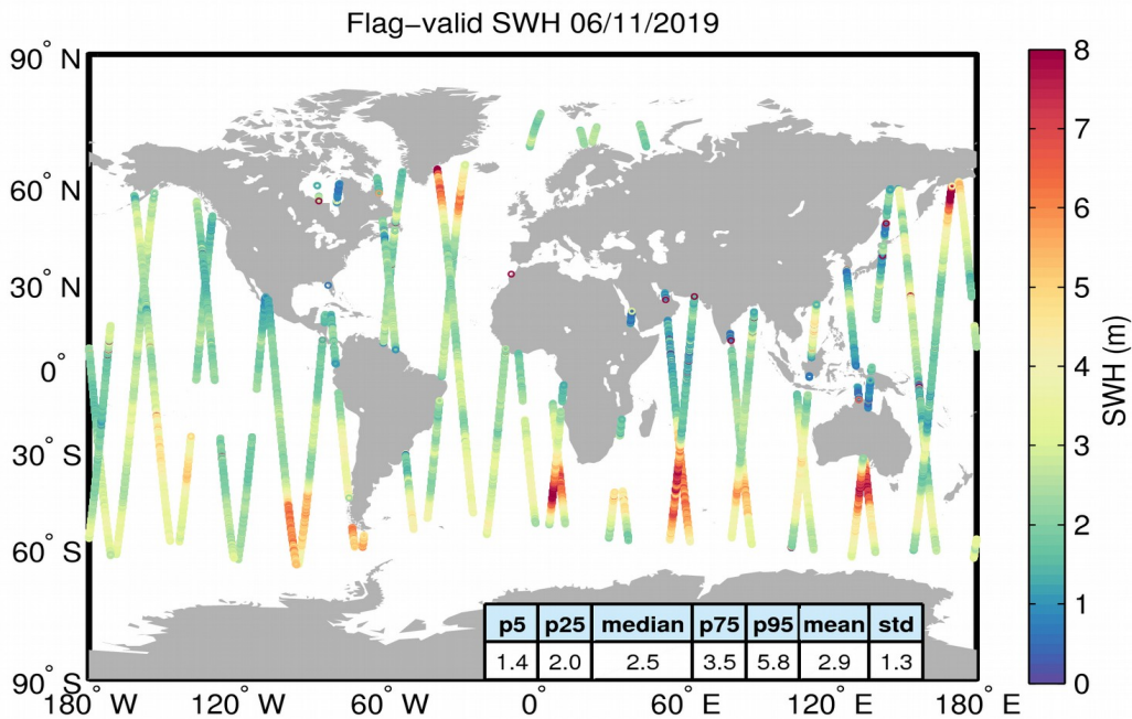
Figure 15. Geographical distribution of flag-valid SWH data over oceans and lakes for 06/11/2019. The statistical values shown in the table refer to the SWH in m and are calculated over all measurements shown in the figure.
