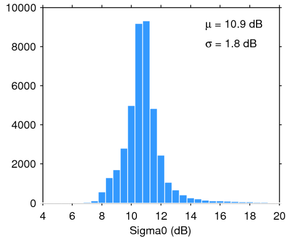
Figure 25. Histogram of flag-valid sigma0 over oceans and lakes for 06/11/2019. The mean ( \mu ) and standard deviation ( \sigma ) are also shown. Note that values outside [4 20] dB are excluded from the histogram for the sake of readability but not from the computation of \mu and \sigma .
