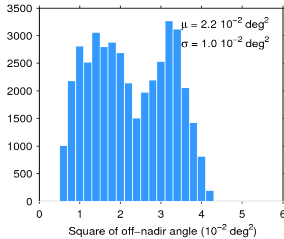
Figure 39. Histogram of flag-valid mispointing over oceans and lakes for 04/11/2019. The mean ( \mu ) and standard deviation ( \sigma ) are also shown. Note that values larger than 6 \cdot 10^{-2} \text{ deg}^2 are excluded from the histogram for the sake of readability but not from the computation of \mu and \sigma .
