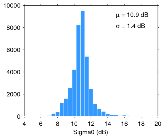
Figure 28. Histogram of science-valid sigma0 over oceans and lakes for 04/11/2019. The mean ( \mu ) and standard deviation ( \sigma ) are also shown. Note that values outside [4 20] dB are excluded from the histogram for the sake of readability but not from the computation of \mu and \sigma .
