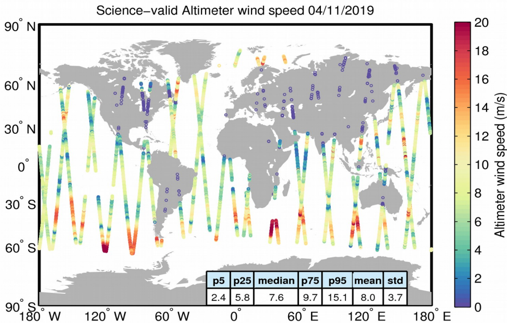
Figure 34. Geographical distribution of science-valid wind data over oceans and lakes for 04/11/2019. The statistical values shown in the table refer to the wind in m/s and are calculated over all measurements shown in the figure. Gray circles denote records that have been rejected based on the editing criteria described in Table 5.
