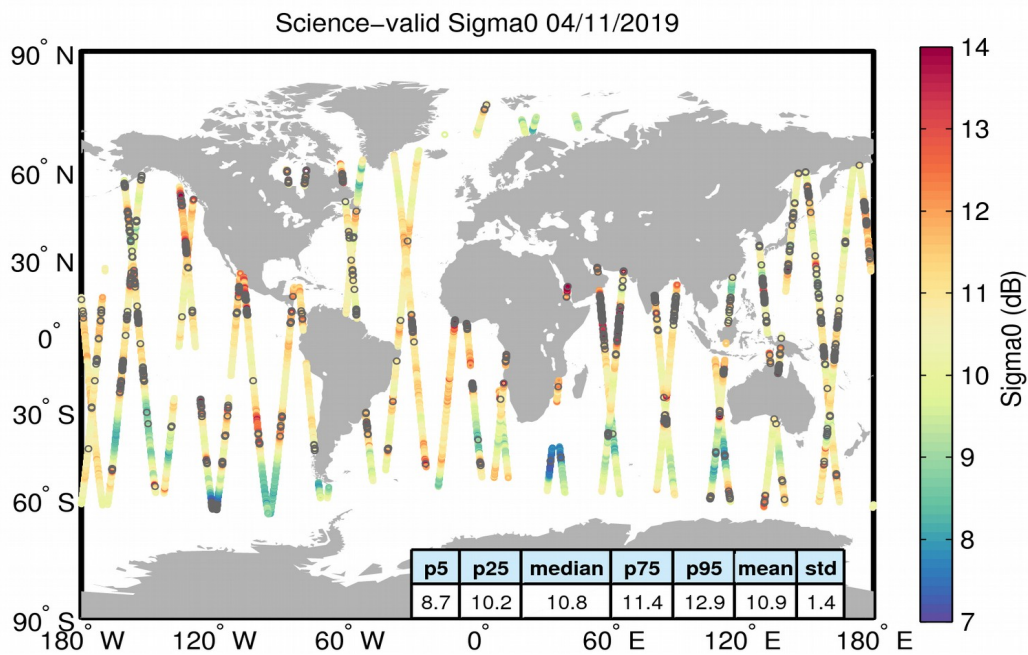
Figure 27. Geographical distribution of science-valid sigma0 data over oceans and lakes for 04/11/2019. The statistical values shown in the table refer to the sigma0 in dB and are calculated over all measurements shown in the figure. Gray circles denote records that have been rejected based on the editing criteria described in Table 4.
