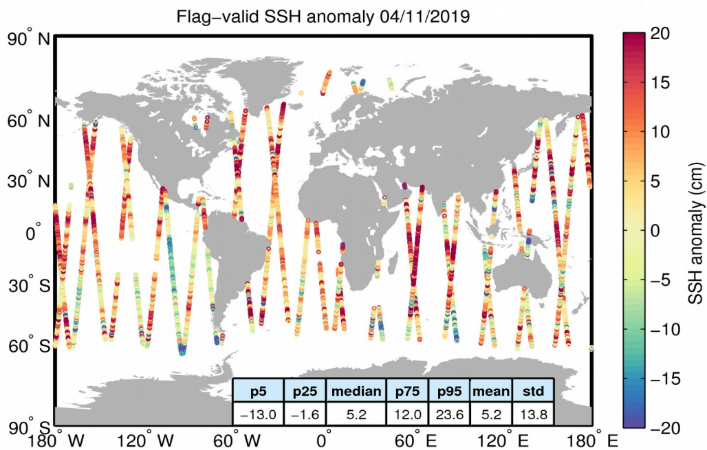
Figure 5. Geographical distribution of flag-valid 1-Hz SSH anomaly data over oceans and lakes for 04/11/2019. The statistical values shown in the table refer to the SSH anomaly in cm and are calculated over all measurements shown in the figure.
