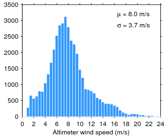
Figure 33. Histogram of flag-valid wind over oceans and lakes for 04/11/2019. The mean ( \mu ) and standard deviation ( \sigma ) are also shown. Note that values larger than 24 m/s are excluded from the histogram for the sake of readability but not from the computation of \mu and \sigma .
