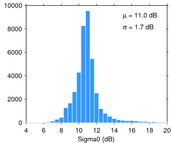
Figure 25. Histogram of flag-valid sigma0 over oceans and lakes for 04/11/2019. The mean ( \mu ) and standard deviation ( \sigma ) are also shown. Note that values outside [4 20] dB are excluded from the histogram for the sake of readability but not from the computation of \mu and \sigma .
