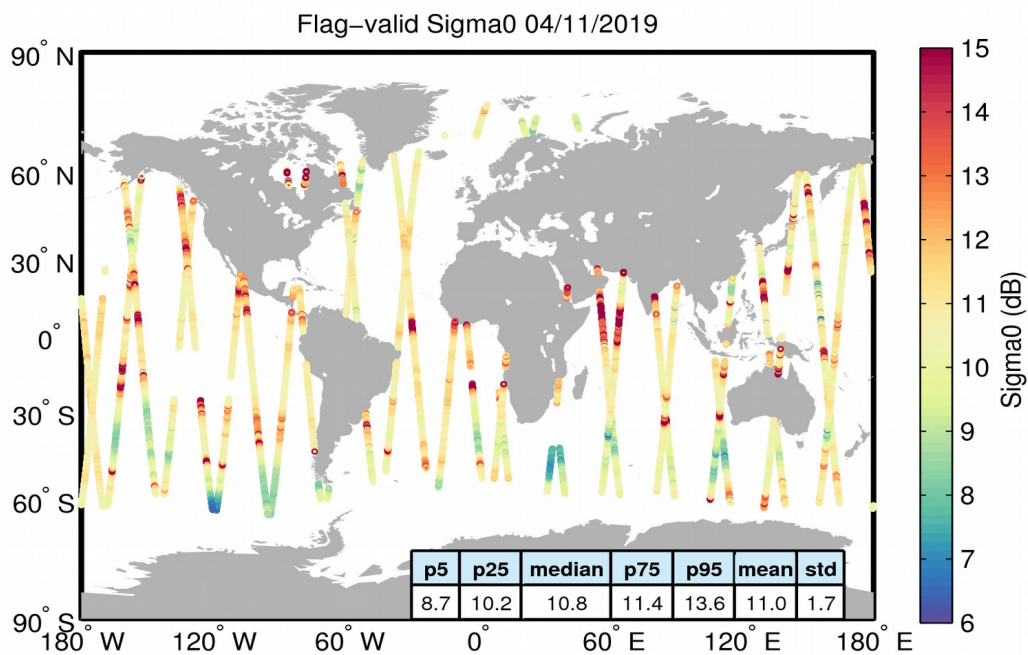
Figure 23. Geographical distribution of flag-valid sigma0 data over oceans and lakes for 04/11/2019. The statistical values shown in the table refer to the sigma0 in dB and are calculated over all measurements shown in the figure.
