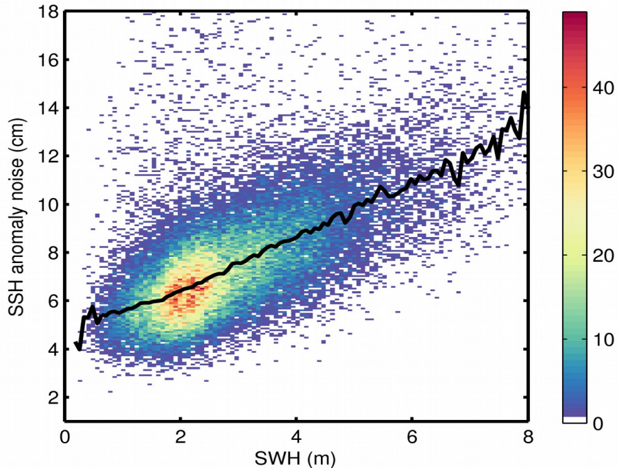
Figure 9. 2D histogram showing flag-valid SSH anomaly noise as a function of SWH for 04/11/2019. The black line denotes the median SSH anomaly noise as a function of SWH.
