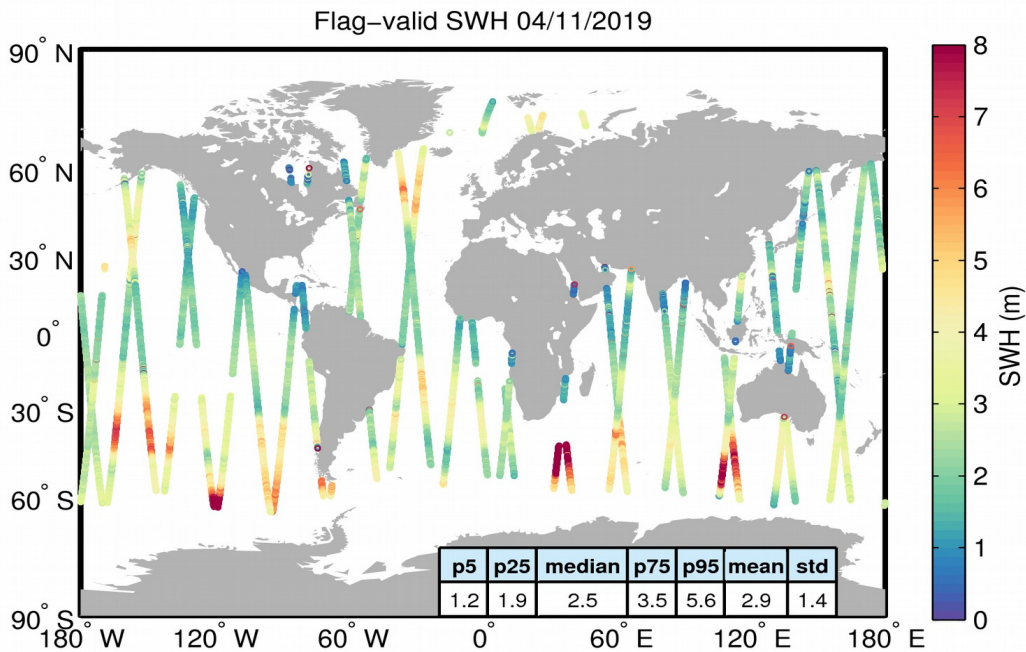
Figure 15. Geographical distribution of flag-valid SWH data over oceans and lakes for 04/11/2019. The statistical values shown in the table refer to the SWH in m and are calculated over all measurements shown in the figure.
