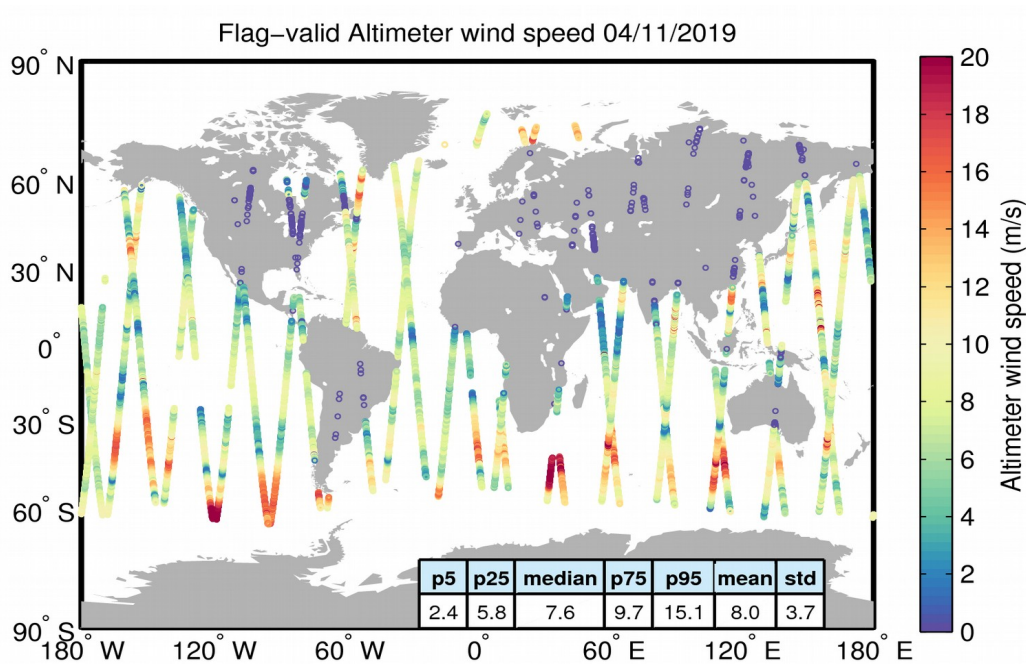
Figure 31. Geographical distribution of flag-valid wind data over oceans and lakes for 04/11/2019. The statistical values shown in the figure refer to the wind in m/s and are calculated over all measurements shown in the figure.
