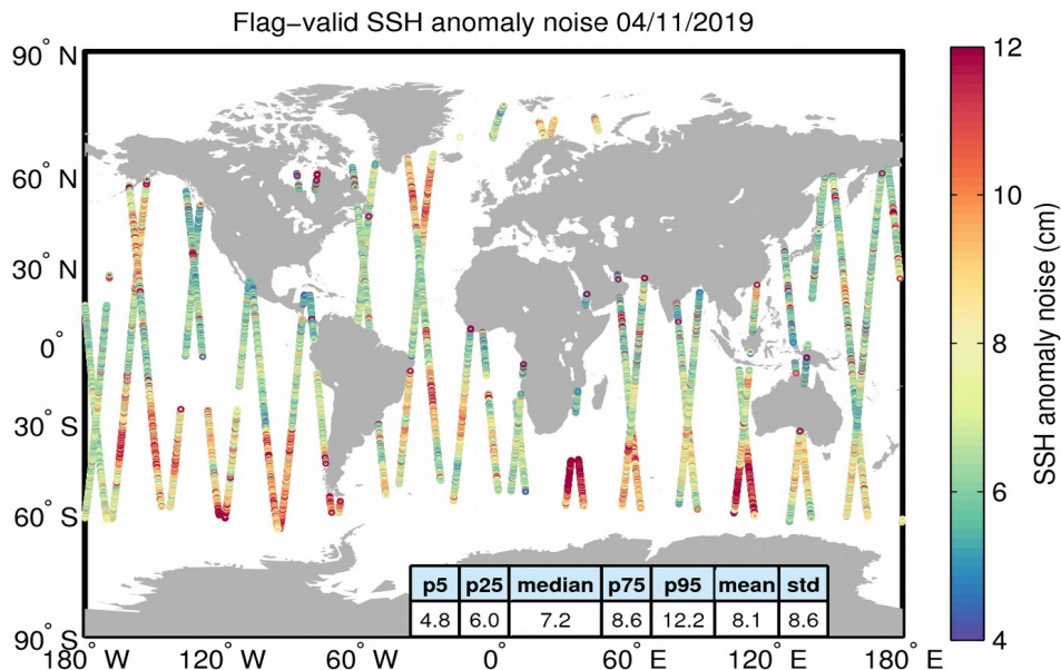
Figure 8. Geographical distribution of flag-valid 20-Hz SSH anomaly measurement noise over oceans and lakes for 04/11/2019. The statistical values shown in the table refer to the SSH anomaly noise and are calculated over all measurements shown in the figure.
