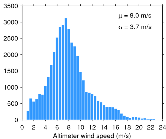
Figure 35. Histogram of science-valid wind over oceans and lakes for 04/11/2019. The mean ( \mu ) and standard deviation ( \sigma ) are also shown. Note that values larger than 24 m/s are excluded from the histogram for the sake of readability but not from the computation of \mu and \sigma .
