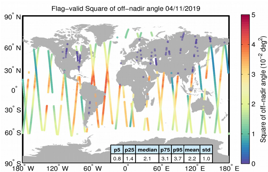
Figure 37. Geographical distribution of flag-valid mispointing data over oceans and lakes for 04/11/2019. The statistical values shown in the table refer to the mispointing in 10^{-2} \text{ deg}^2 and are calculated over all measurements shown in the figure.
