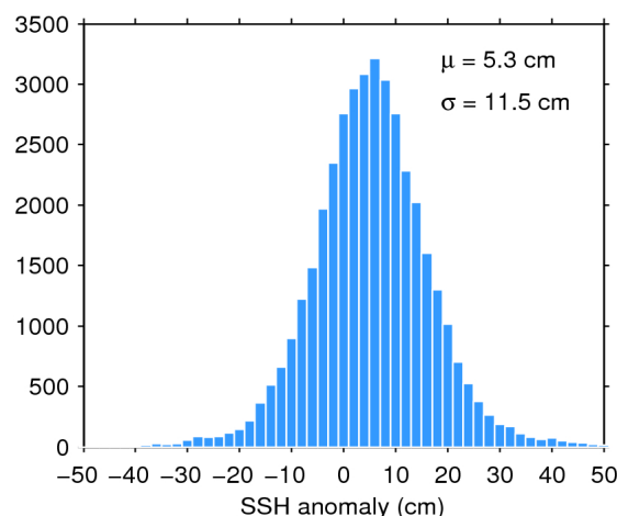
Figure 11. Histogram of science-valid SSH anomaly over oceans and lakes for 04/11/2019. The mean ( \mu ) and standard deviation ( \sigma ) are also shown. Note that values outside [-50 50] cm are excluded from the histogram for the sake of readability but not from the computation of \mu and \sigma .
