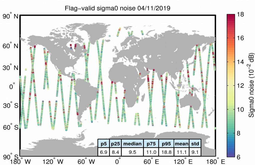
Figure 26. Geographical distribution of flag-valid 20-Hz sigma0 measurement noise over oceans and lakes for 04/11/2019. The statistical values shown in the table refer to the sigma0 noise and are calculated over all measurements shown in the figure.
