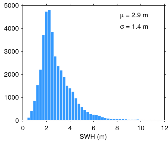
Figure 17. Histogram of flag-valid SWH over oceans and lakes for 04/11/2019. The mean ( \mu ) and standard deviation ( \sigma ) are also shown. Note that values larger than 12 m are excluded from the histogram for the sake of readability but not from the computation of \mu and \sigma .
