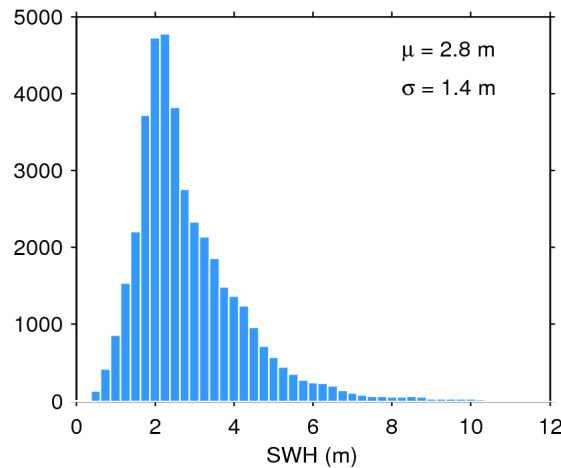
Figure 20. Histogram of science-valid SWH over oceans and lakes for 04/11/2019. The mean ( \mu ) and standard deviation ( \sigma ) are also shown. Note that values larger than 12 m are excluded from the histogram for the sake of readability but not from the computation of \mu and \sigma .
