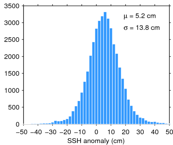
Figure 7. Histogram of flag-valid SSH anomaly over oceans and lakes for 04/11/2019. The mean ( \mu ) and standard deviation ( \sigma ) are also shown. Note that values outside [-50 50] cm are excluded from the histogram for the sake of readability but not from the computation of \mu and \sigma .
