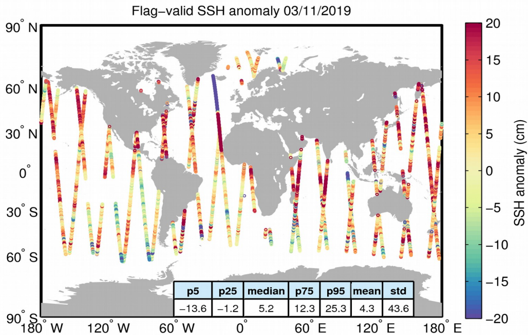
Figure 5. Geographical distribution of flag-valid 1-Hz SSH anomaly data over oceans and lakes for 03/11/2019. The statistical values shown in the table refer to the SSH anomaly in cm and are calculated over all measurements shown in the figure.
