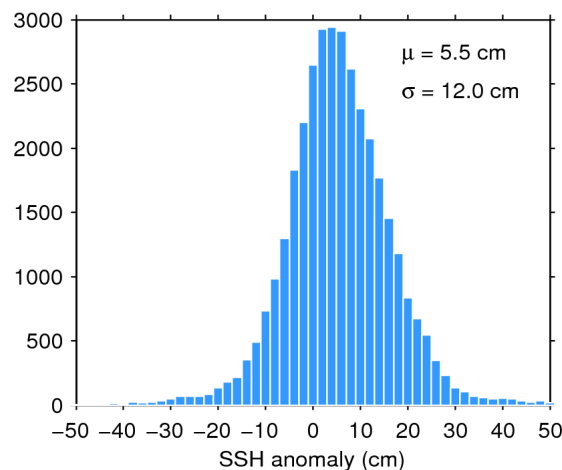
Figure 11. Histogram of science-valid SSH anomaly over oceans and lakes for 03/11/2019. The mean ( \mu ) and standard deviation ( \sigma ) are also shown. Note that values outside [-50 50] cm are excluded from the histogram for the sake of readability but not from the computation of \mu and \sigma .
