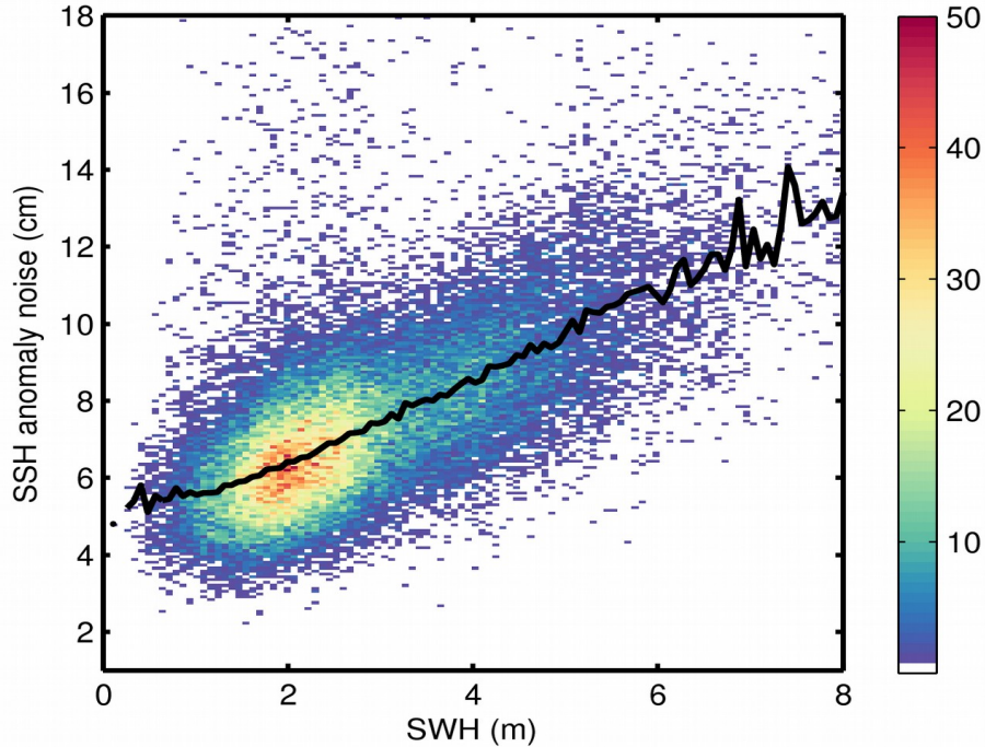
Figure 9. 2D histogram showing flag-valid SSH anomaly noise as a function of SWH for 03/11/2019. The black line denotes the median SSH anomaly noise as a function of SWH.
