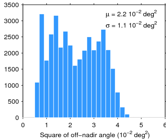
Figure 39. Histogram of flag-valid mispointing over oceans and lakes for 03/11/2019. The mean ( \mu ) and standard deviation ( \sigma ) are also shown. Note that values larger than 6 \cdot 10^{-2} \text{ deg}^2 are excluded from the histogram for the sake of readability but not from the computation of \mu and \sigma .
