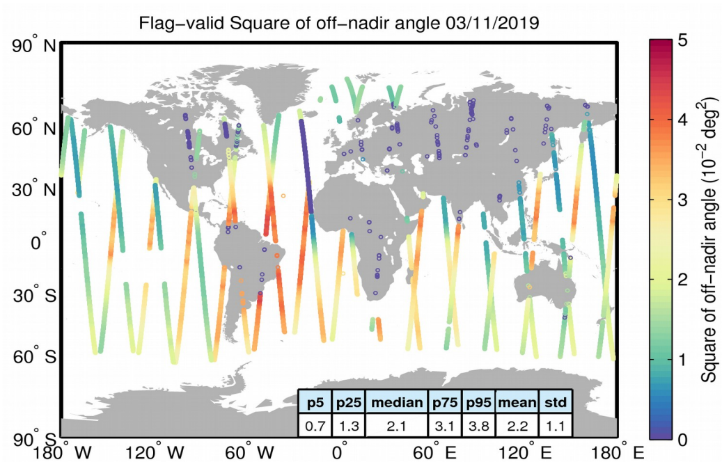
Figure 37. Geographical distribution of flag-valid mispointing data over oceans and lakes for 03/11/2019. The statistical values shown in the table refer to the mispointing in 10^{-2} \text{ deg}^2 and are calculated over all measurements shown in the figure.
