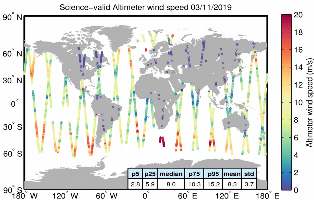
Figure 34. Geographical distribution of science-valid wind data over oceans and lakes for 03/11/2019. The statistical values shown in the table refer to the wind in m/s and are calculated over all measurements shown in the figure. Gray circles denote records that have been rejected based on the editing criteria described in Table 5.
