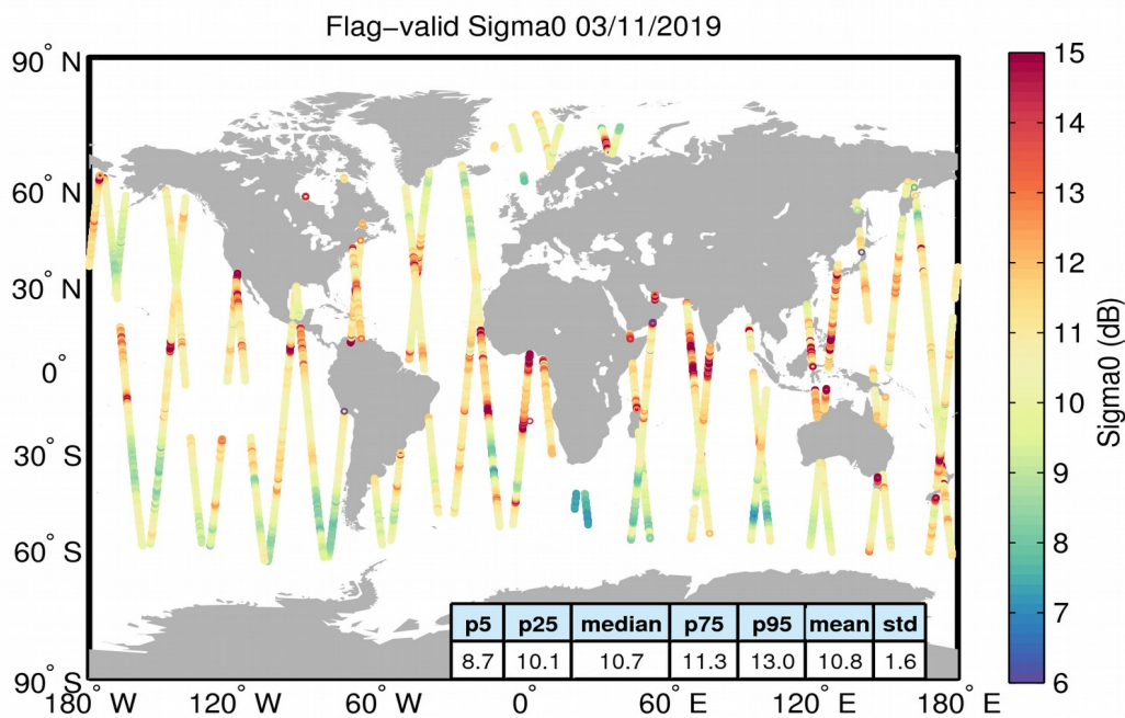
Figure 23. Geographical distribution of flag-valid sigma0 data over oceans and lakes for 03/11/2019. The statistical values shown in the table refer to the sigma0 in dB and are calculated over all measurements shown in the figure.
