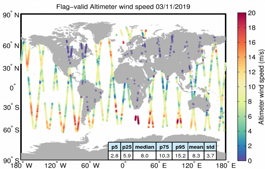
Figure 31. Geographical distribution of flag-valid wind data over oceans and lakes for 03/11/2019. The statistical values shown in the table refer to the wind in m/s and are calculated over all measurements shown in the figure.
