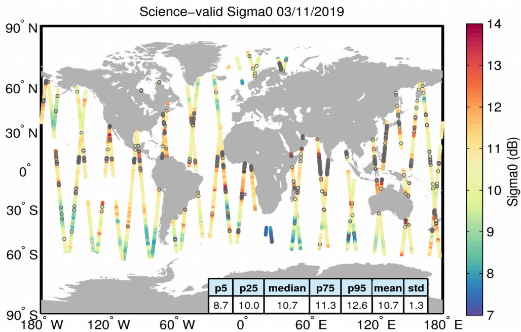
Figure 27. Geographical distribution of science-valid sigma0 data over oceans and lakes for 03/11/2019. The statistical values shown in the table refer to the sigma0 in dB and are calculated over all measurements shown in the figure. Gray circles denote records that have been rejected based on the editing criteria described in Table 4.
