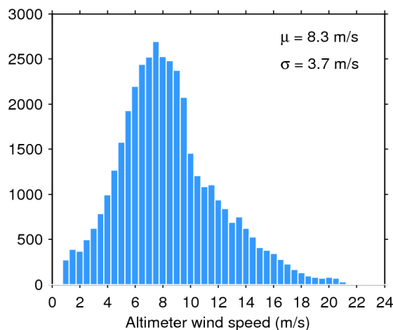
Figure 35. Histogram of science-valid wind over oceans and lakes for 03/11/2019. The mean ( \mu ) and standard deviation ( \sigma ) are also shown. Note that values larger than 24 m/s are excluded from the histogram for the sake of readability but not from the computation of \mu and \sigma .
