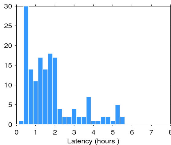
Figure 2. Histogram of the data latency for 03/11/2019. The y-axis denotes the number of files that are made available with a delay of x-hours with respect to the mean time of the records stored in the file.
