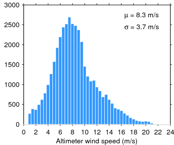
Figure 33. Histogram of flag-valid wind over oceans and lakes for 03/11/2019. The mean ( \mu ) and standard deviation ( \sigma ) are also shown. Note that values larger than 24 m/s are excluded from the histogram for the sake of readability but not from the computation of \mu and \sigma .
