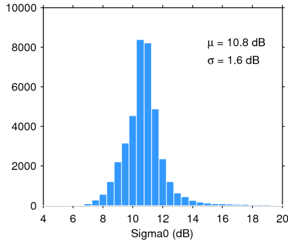
Figure 25. Histogram of flag-valid sigma0 over oceans and lakes for 03/11/2019. The mean ( \mu ) and standard deviation ( \sigma ) are also shown. Note that values outside [4 20] dB are excluded from the histogram for the sake of readability but not from the computation of \mu and \sigma .
