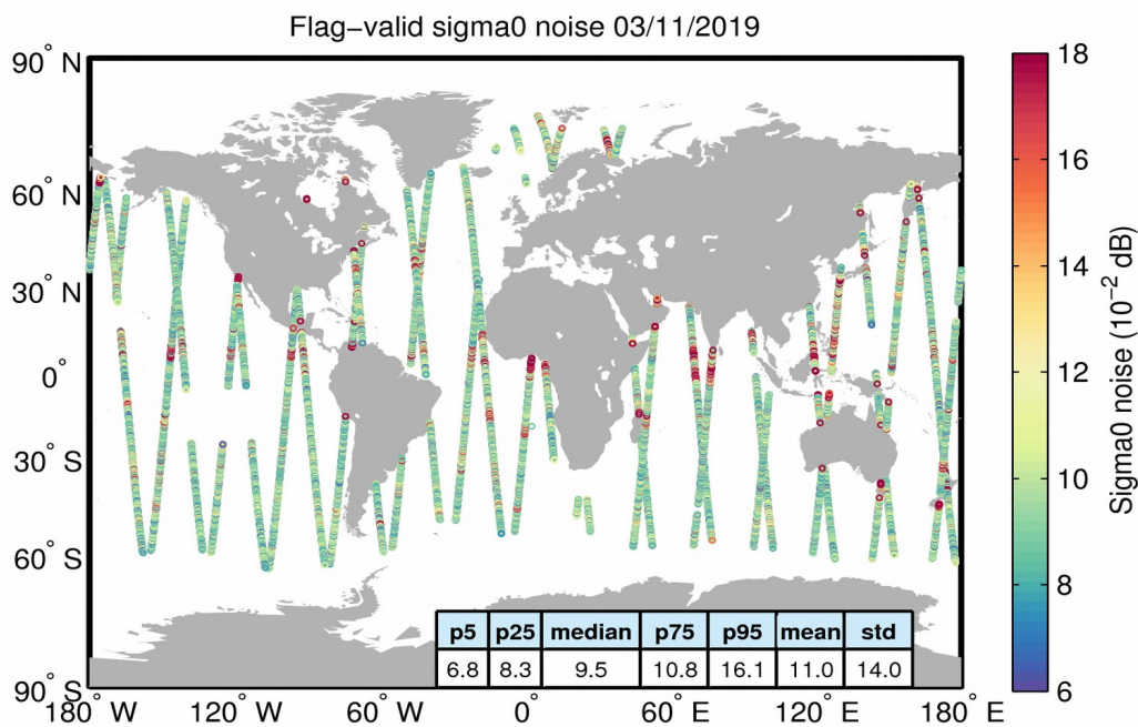
Figure 26. Geographical distribution of flag-valid 20-Hz sigma0 measurement noise over oceans and lakes for 03/11/2019. The statistical values shown in the table refer to the sigma0 noise and are calculated over all measurements shown in the figure.
