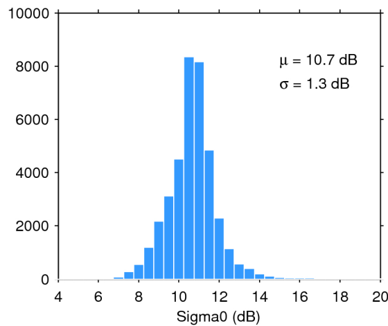
Figure 28. Histogram of science-valid sigma0 over oceans and lakes for 03/11/2019. The mean ( \mu ) and standard deviation ( \sigma ) are also shown. Note that values outside [4 20] dB are excluded from the histogram for the sake of readability but not from the computation of \mu and \sigma .
