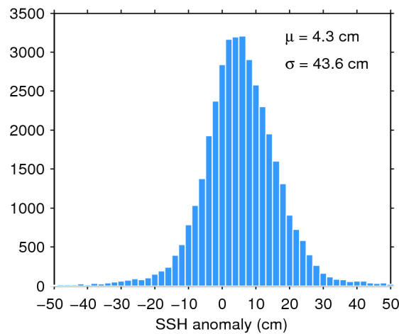
Figure 7. Histogram of flag-valid SSH anomaly over oceans and lakes for 03/11/2019. The mean ( \mu ) and standard deviation ( \sigma ) are also shown. Note that values outside [-50\ 50] cm are excluded from the histogram for the sake of readability but not from the computation of \mu and \sigma .
