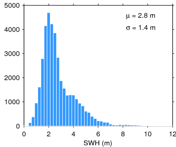
Figure 20. Histogram of science-valid SWH over oceans and lakes for 03/11/2019. The mean ( \mu ) and standard deviation ( \sigma ) are also shown. Note that values larger than 12 m are excluded from the histogram for the sake of readability but not from the computation of \mu and \sigma .
