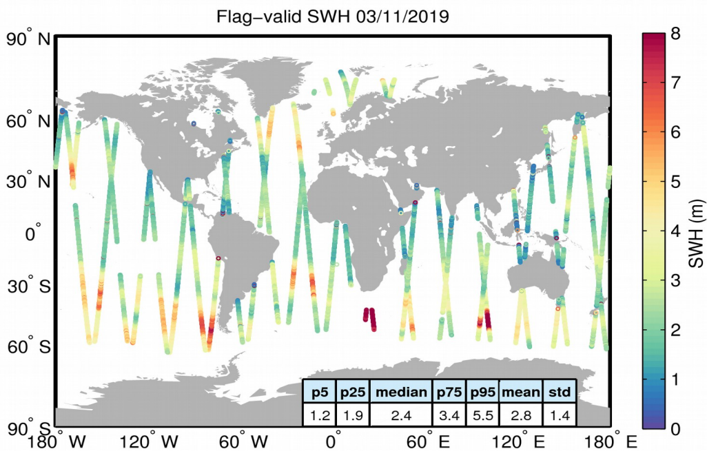
Figure 15. Geographical distribution of flag-valid SWH data over oceans and lakes for 03/11/2019. The statistical values shown in the table refer to the SWH in m and are calculated over all measurements shown in the figure.
