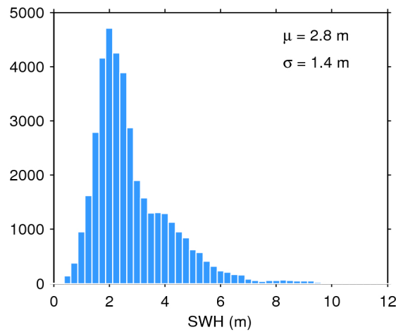
Figure 17. Histogram of flag-valid SWH over oceans and lakes for 03/11/2019. The mean ( \mu ) and standard deviation ( \sigma ) are also shown. Note that values larger than 12 m are excluded from the histogram for the sake of readability but not from the computation of \mu and \sigma .
