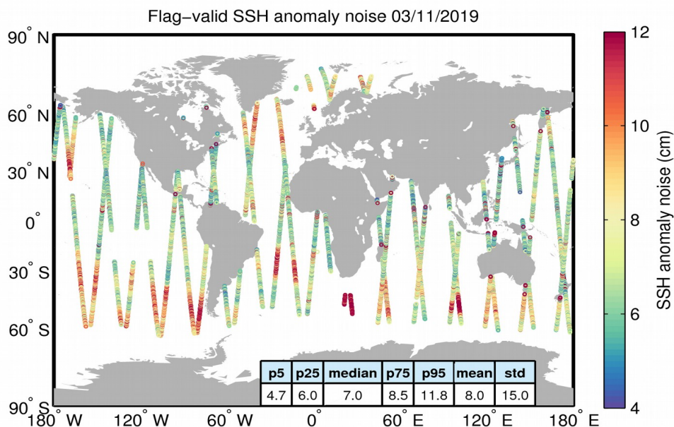
Figure 8. Geographical distribution of flag-valid 20-Hz SSH anomaly measurement noise over oceans and lakes for 03/11/2019. The statistical values shown in the table refer to the SSH anomaly noise and are calculated over all measurements shown in the figure.
