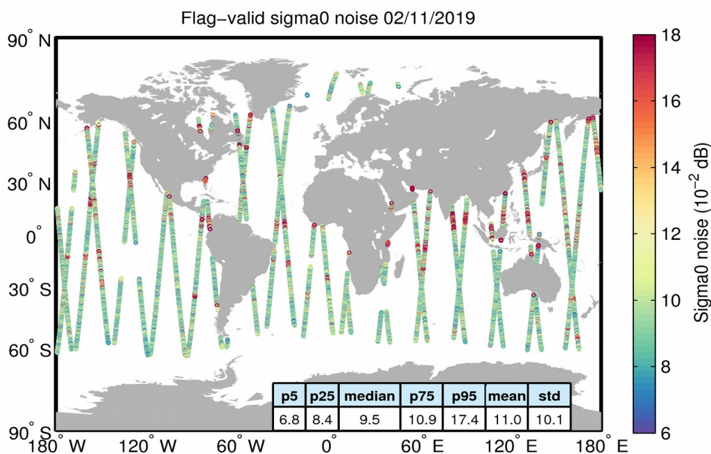
Figure 26. Geographical distribution of flag-valid 20-Hz sigma0 measurement noise over oceans and lakes for 02/11/2019. The statistical values shown in the table refer to the sigma0 noise and are calculated over all measurements shown in the figure.
