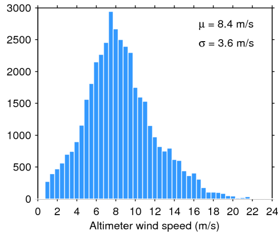
Figure 33. Histogram of flag-valid wind over oceans and lakes for 02/11/2019. The mean ( \mu ) and standard deviation ( \sigma ) are also shown. Note that values larger than 24 m/s are excluded from the histogram for the sake of readability but not from the computation of \mu and \sigma .
