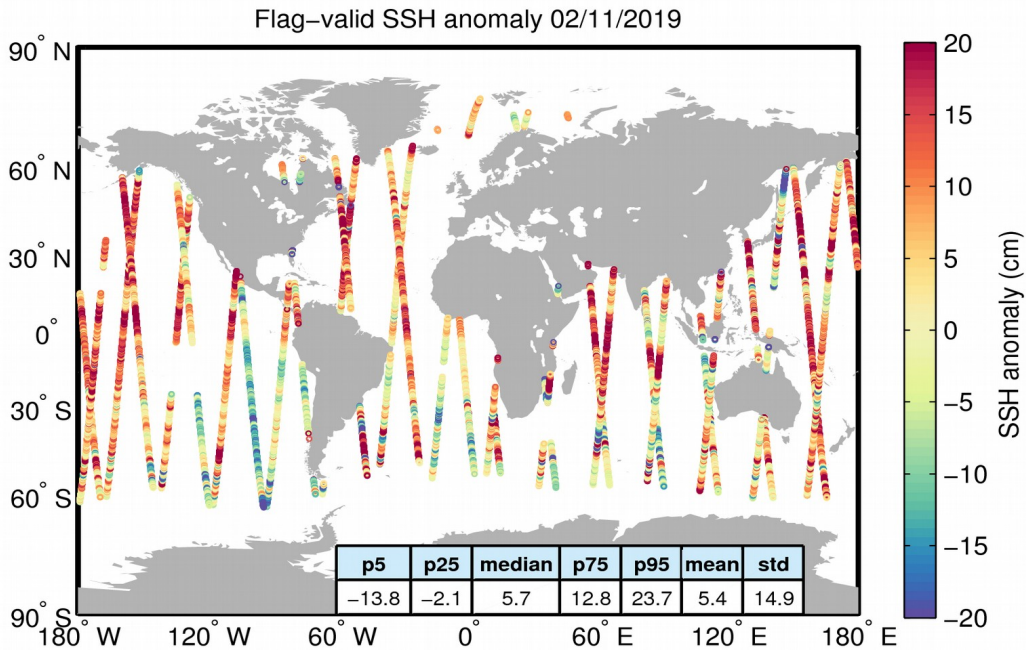
Figure 5. Geographical distribution of flag-valid 1-Hz SSH anomaly data over oceans and lakes for 02/11/2019. The statistical values shown in the table refer to the SSH anomaly in cm and are calculated over all measurements shown in the figure.
