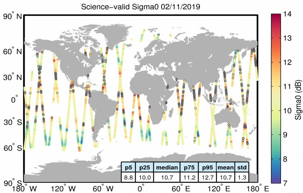
Figure 27. Geographical distribution of science-valid sigma0 data over oceans and lakes for 02/11/2019. The statistical values shown in the table refer to the sigma0 in dB and are calculated over all measurements shown in the figure. Gray circles denote records that have been rejected based on the editing criteria described in Table 4.
