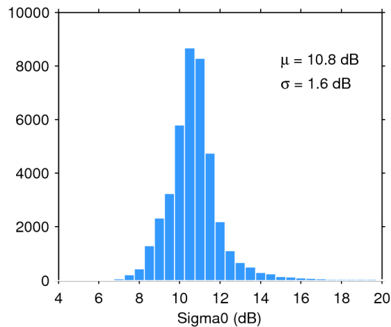
Figure 25. Histogram of flag-valid sigma0 over oceans and lakes for 02/11/2019. The mean ( \mu ) and standard deviation ( \sigma ) are also shown. Note that values outside [4 20] dB are excluded from the histogram for the sake of readability but not from the computation of \mu and \sigma .
