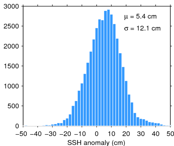
Figure 11. Histogram of science-valid SSH anomaly over oceans and lakes for 02/11/2019. The mean ( \mu ) and standard deviation ( \sigma ) are also shown. Note that values outside [-50 50] cm are excluded from the histogram for the sake of readability but not from the computation of \mu and \sigma .
