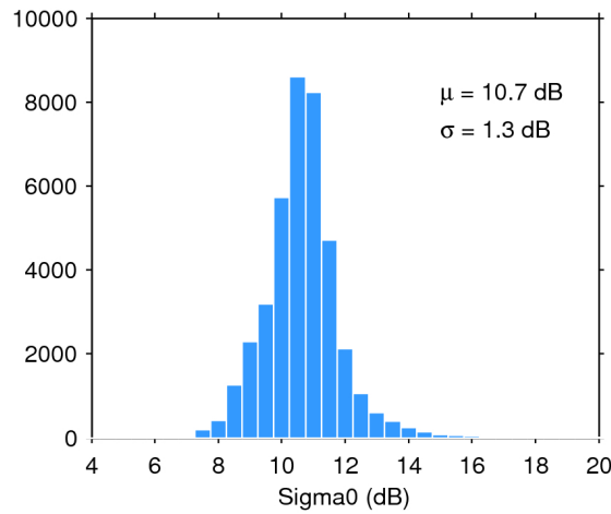
Figure 28. Histogram of science-valid sigma0 over oceans and lakes for 02/11/2019. The mean ( \mu ) and standard deviation ( \sigma ) are also shown. Note that values outside [4 20] dB are excluded from the histogram for the sake of readability but not from the computation of \mu and \sigma .
