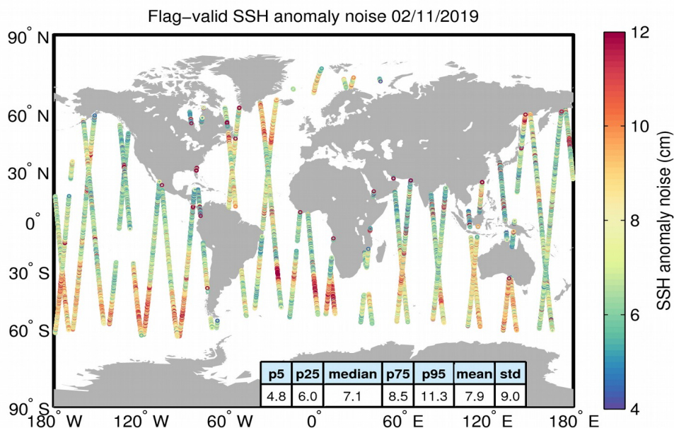
Figure 8. Geographical distribution of flag-valid 20-Hz SSH anomaly measurement noise over oceans and lakes for 02/11/2019. The statistical values shown in the table refer to the SSH anomaly noise and are calculated over all measurements shown in the figure.
