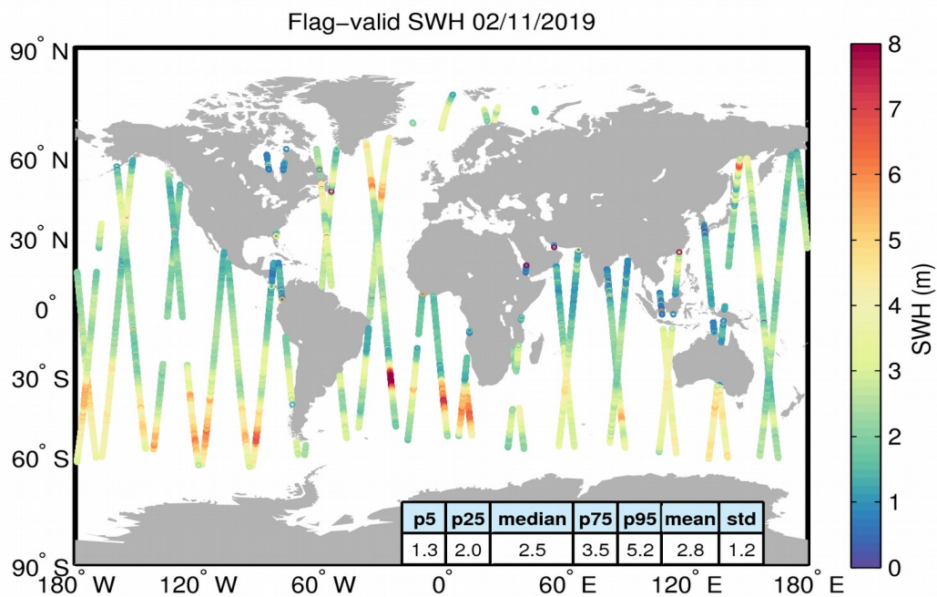
Figure 15. Geographical distribution of flag-valid SWH data over oceans and lakes for 02/11/2019. The statistical values shown in the table refer to the SWH in m and are calculated over all measurements shown in the figure.
