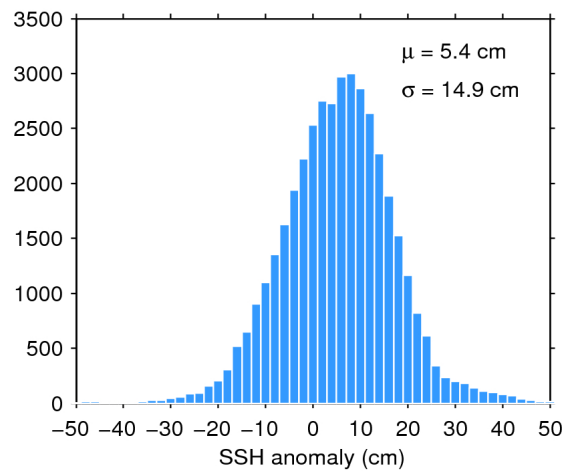
Figure 7. Histogram of flag-valid SSH anomaly over oceans and lakes for 02/11/2019. The mean ( \mu ) and standard deviation ( \sigma ) are also shown. Note that values outside [-50 50] cm are excluded from the histogram for the sake of readability but not from the computation of \mu and \sigma .
