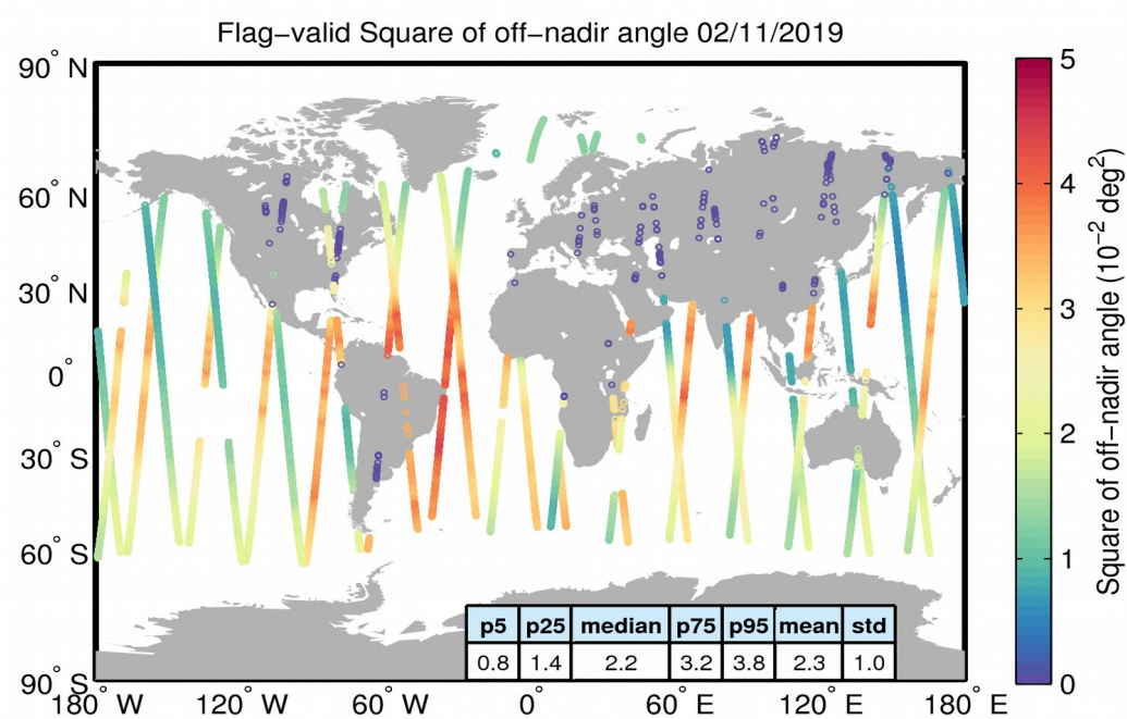
Figure 37. Geographical distribution of flag-valid mispointing data over oceans and lakes for 02/11/2019. The statistical values shown in the table refer to the mispointing in 10^{-2} \text{ deg}^2 and are calculated over all measurements shown in the figure.
