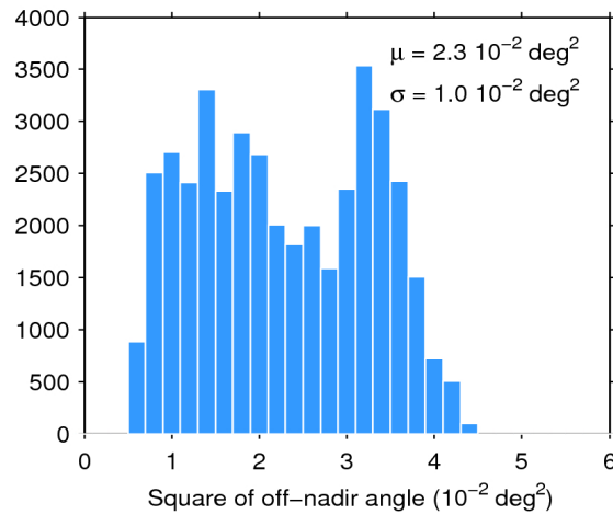
Figure 39. Histogram of flag-valid mispointing over oceans and lakes for 02/11/2019. The mean ( \mu ) and standard deviation ( \sigma ) are also shown. Note that values larger than 6 \cdot 10^{-2} \text{ deg}^2 are excluded from the histogram for the sake of readability but not from the computation of \mu and \sigma .
