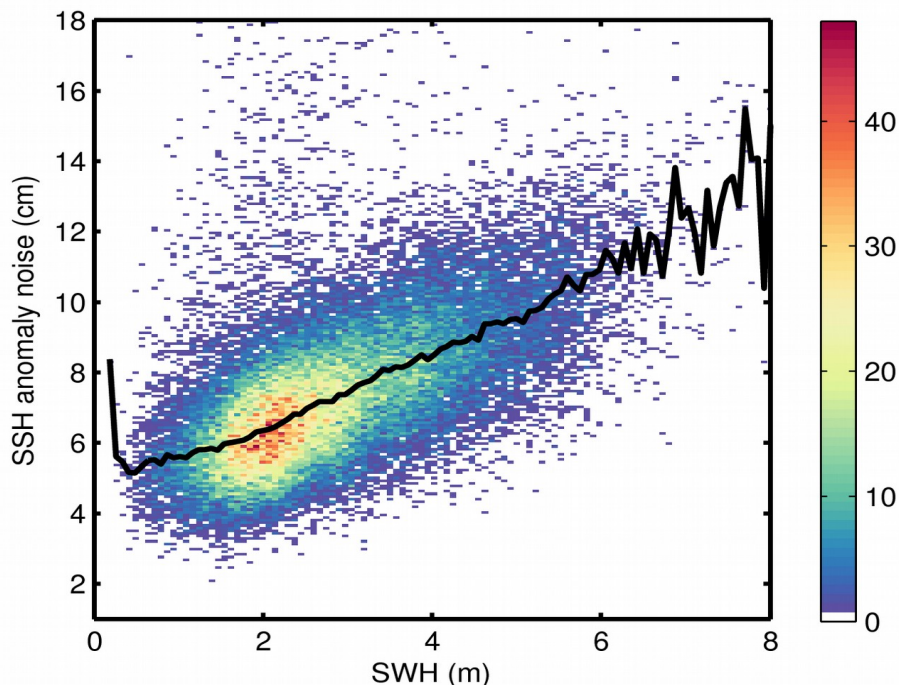
Figure 9. 2D histogram showing flag-valid SSH anomaly noise as a function of SWH for 02/11/2019. The black line denotes the median SSH anomaly noise as a function of SWH.
