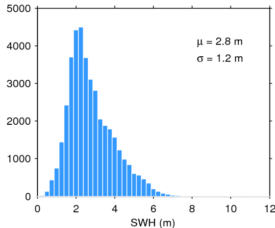
Figure 20. Histogram of science-valid SWH over oceans and lakes for 02/11/2019. The mean ( \mu ) and standard deviation ( \sigma ) are also shown. Note that values larger than 12 m are excluded from the histogram for the sake of readability but not from the computation of \mu and \sigma .
