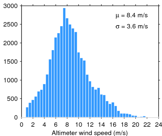
Figure 35. Histogram of science-valid wind over oceans and lakes for 02/11/2019. The mean ( \mu ) and standard deviation ( \sigma ) are also shown. Note that values larger than 24 m/s are excluded from the histogram for the sake of readability but not from the computation of \mu and \sigma .
