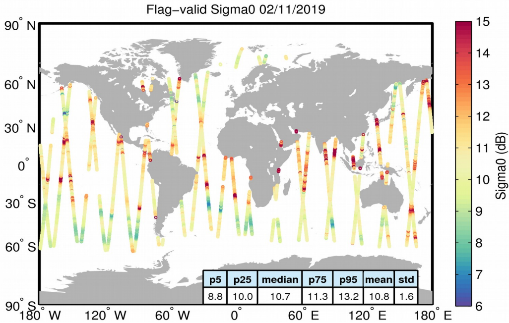
Figure 23. Geographical distribution of flag-valid sigma0 data over oceans and lakes for 02/11/2019. The statistical values shown in the table refer to the sigma0 in dB and are calculated over all measurements shown in the figure.
