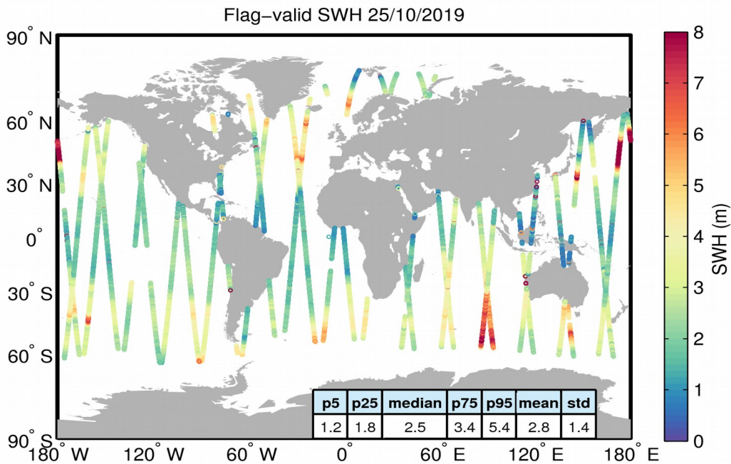
Figure 15. Geographical distribution of flag-valid SWH data over oceans and lakes for 25/10/2019. The statistical values shown in the table refer to the SWH in m and are calculated over all measurements shown in the figure.
