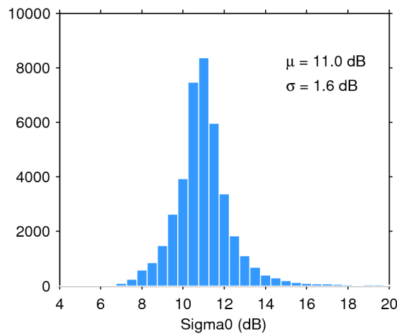
Figure 28. Histogram of science-valid sigma0 over oceans and lakes for 25/10/2019. The mean ( \mu ) and standard deviation ( \sigma ) are also shown. Note that values outside [4 20] dB are excluded from the histogram for the sake of readability but not from the computation of \mu and \sigma .
