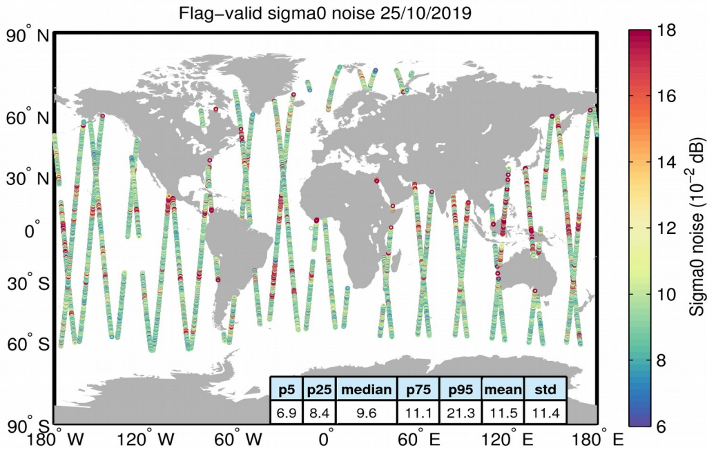
Figure 26. Geographical distribution of flag-valid 20-Hz sigma0 measurement noise over oceans and lakes for 25/10/2019. The statistical values shown in the table refer to the sigma0 noise and are calculated over all measurements shown in the figure.
