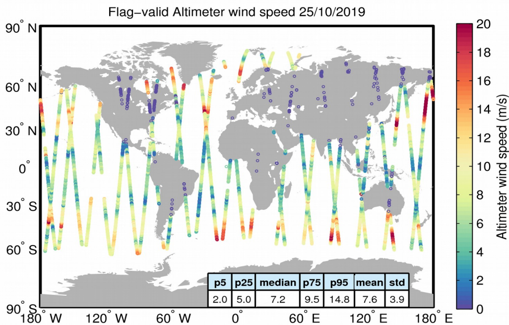
Figure 31. Geographical distribution of flag-valid wind data over oceans and lakes for 25/10/2019. The statistical values shown in the table refer to the wind in m/s and are calculated over all measurements shown in the figure.
