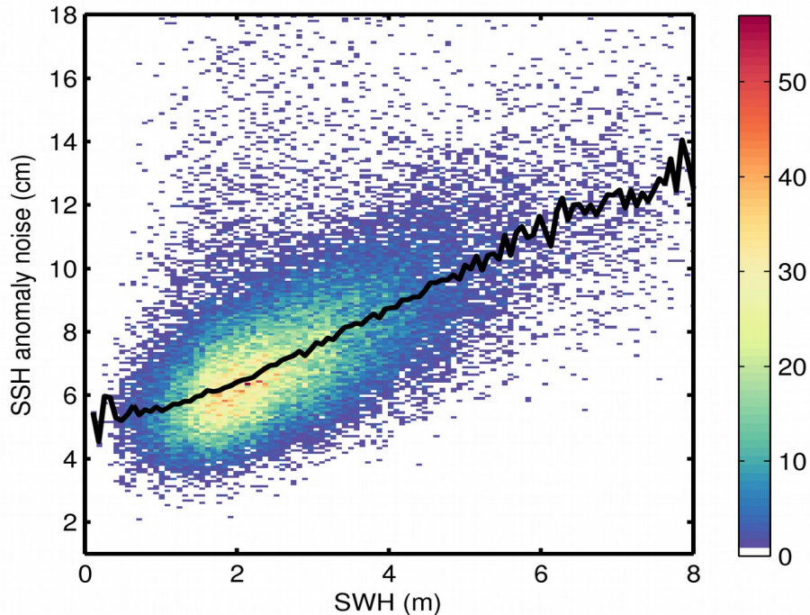
Figure 9. 2D histogram showing flag-valid SSH anomaly noise as a function of SWH for 25/10/2019. The black line denotes the median SSH anomaly noise as a function of SWH.
