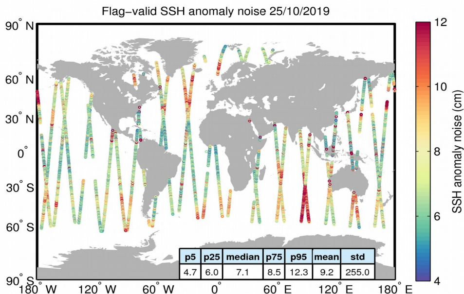
Figure 8. Geographical distribution of flag-valid 20-Hz SSH anomaly measurement noise over oceans and lakes for 25/10/2019. The statistical values shown in the table refer to the SSH anomaly noise and are calculated over all measurements shown in the figure.
