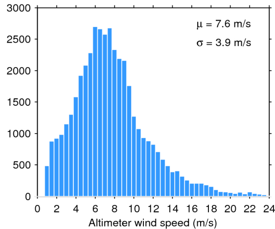
Figure 33. Histogram of flag-valid wind over oceans and lakes for 25/10/2019. The mean ( \mu ) and standard deviation ( \sigma ) are also shown. Note that values larger than 24 m/s are excluded from the histogram for the sake of readability but not from the computation of \mu and \sigma .
