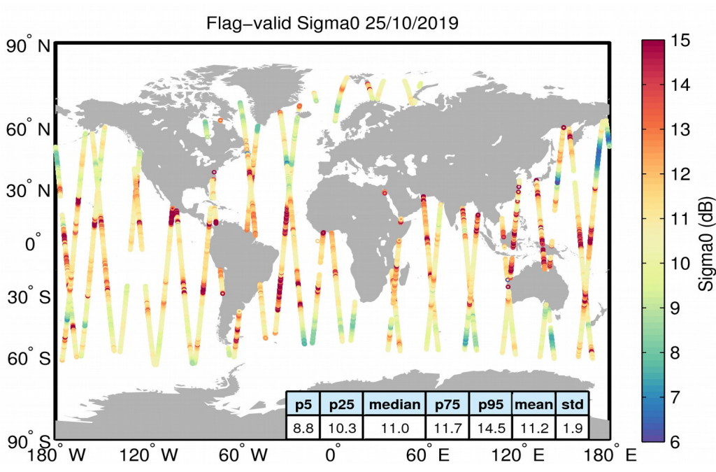
Figure 23. Geographical distribution of flag-valid sigma0 data over oceans and lakes for 25/10/2019. The statistical values shown in the table refer to the sigma0 in dB and are calculated over all measurements shown in the figure.
