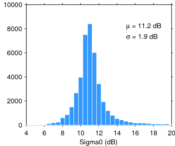
Figure 25. Histogram of flag-valid sigma0 over oceans and lakes for 25/10/2019. The mean ( \mu ) and standard deviation ( \sigma ) are also shown. Note that values outside [4 20] dB are excluded from the histogram for the sake of readability but not from the computation of \mu and \sigma .
