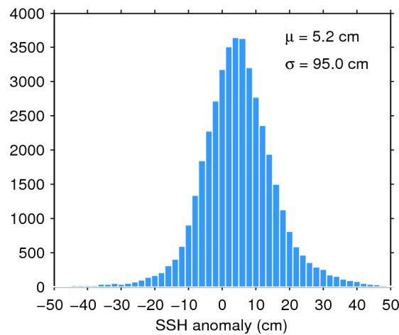
Figure 7. Histogram of flag-valid SSH anomaly over oceans and lakes for 25/10/2019. The mean ( \mu ) and standard deviation ( \sigma ) are also shown. Note that values outside [-50\ 50] cm are excluded from the histogram for the sake of readability but not from the computation of \mu and \sigma .
