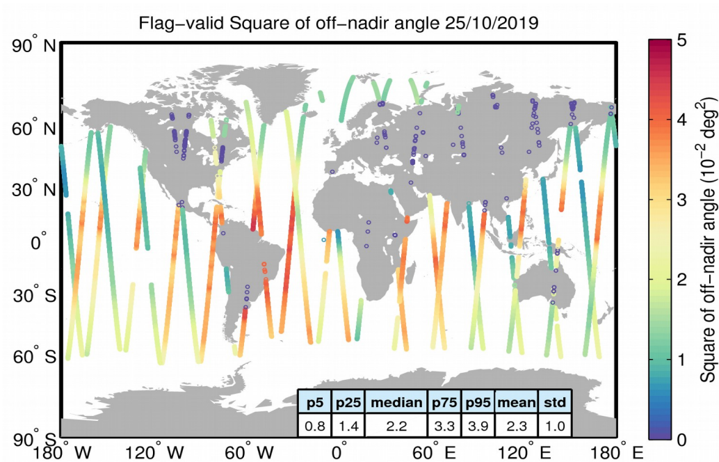
Figure 37. Geographical distribution of flag-valid mispointing data over oceans and lakes for 25/10/2019. The statistical values shown in the table refer to the mispointing in 10^{-2} \text{ deg}^2 and are calculated over all measurements shown in the figure.
