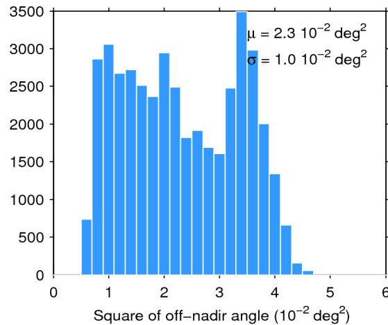
Figure 39. Histogram of flag-valid mispointing over oceans and lakes for 25/10/2019. The mean ( \mu ) and standard deviation ( \sigma ) are also shown. Note that values larger than 6 \cdot 10^{-2} \text{ deg}^2 are excluded from the histogram for the sake of readability but not from the computation of \mu and \sigma .
