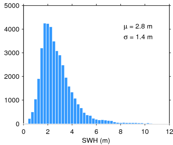
Figure 17. Histogram of flag-valid SWH over oceans and lakes for 25/10/2019. The mean ( \mu ) and standard deviation ( \sigma ) are also shown. Note that values larger than 12 m are excluded from the histogram for the sake of readability but not from the computation of \mu and \sigma .
