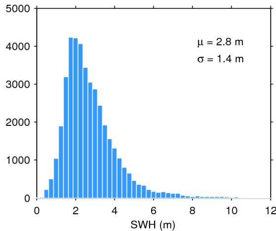
Figure 20. Histogram of science-valid SWH over oceans and lakes for 25/10/2019. The mean ( \mu ) and standard deviation ( \sigma ) are also shown. Note that values larger than 12 m are excluded from the histogram for the sake of readability but not from the computation of \mu and \sigma .
