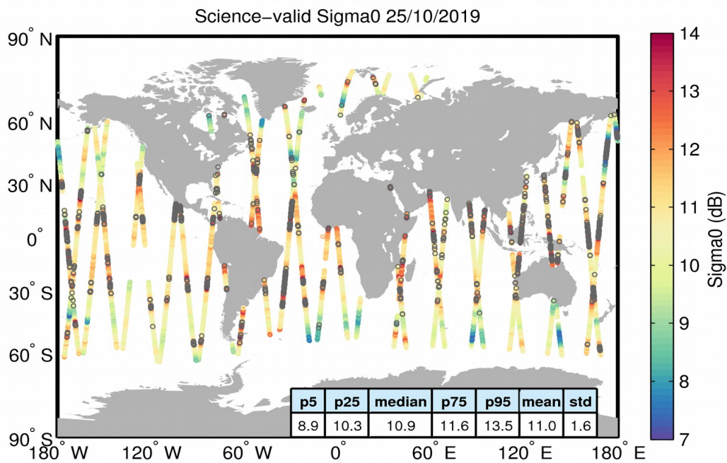
Figure 27. Geographical distribution of science-valid sigma0 data over oceans and lakes for 25/10/2019. The statistical values shown in the table refer to the sigma0 in dB and are calculated over all measurements shown in the figure. Gray circles denote records that have been rejected based on the editing criteria described in Table 4.
