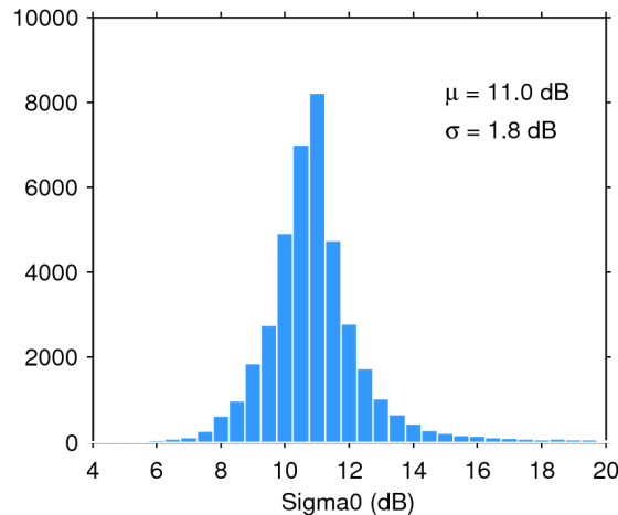
Figure 25. Histogram of flag-valid sigma0 over oceans and lakes for 24/10/2019. The mean ( \mu ) and standard deviation ( \sigma ) are also shown. Note that values outside [4 20] dB are excluded from the histogram for the sake of readability but not from the computation of \mu and \sigma .
