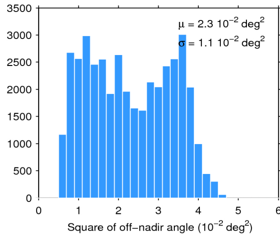
Figure 39. Histogram of flag-valid mispointing over oceans and lakes for 24/10/2019. The mean ( \mu ) and standard deviation ( \sigma ) are also shown. Note that values larger than 6 \cdot 10^{-2} \text{ deg}^2 are excluded from the histogram for the sake of readability but not from the computation of \mu and \sigma .
