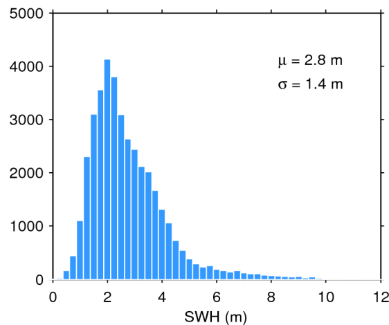
Figure 20. Histogram of science-valid SWH over oceans and lakes for 24/10/2019. The mean ( \mu ) and standard deviation ( \sigma ) are also shown. Note that values larger than 12 m are excluded from the histogram for the sake of readability but not from the computation of \mu and \sigma .
