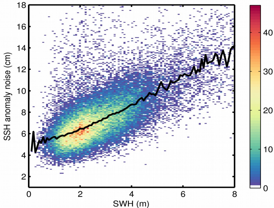
Figure 9. 2D histogram showing flag-valid SSH anomaly noise as a function of SWH for 24/10/2019. The black line denotes the median SSH anomaly noise as a function of SWH.
