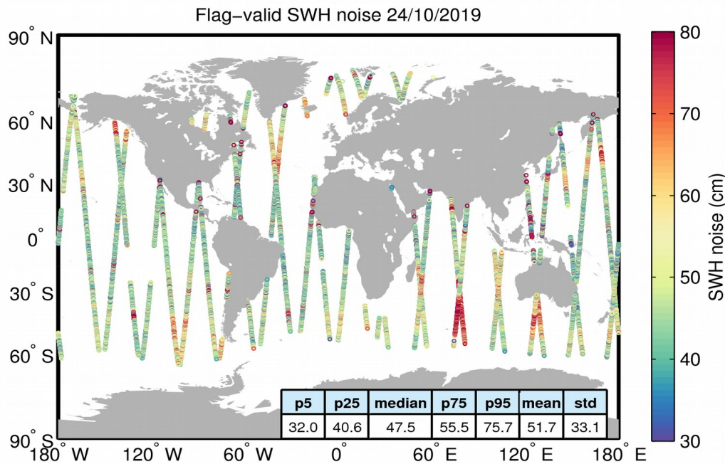
Figure 18. Geographical distribution of flag-valid 20-Hz SWH measurement noise over oceans and lakes for 24/10/2019. The statistical values shown in the figure refer to the SWH noise and are calculated over all measurements shown in the figure.
