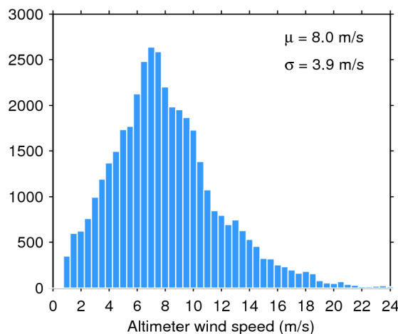
Figure 35. Histogram of science-valid wind over oceans and lakes for 24/10/2019. The mean ( \mu ) and standard deviation ( \sigma ) are also shown. Note that values larger than 24 m/s are excluded from the histogram for the sake of readability but not from the computation of \mu and \sigma .
