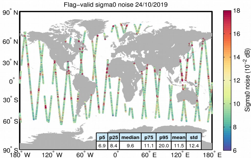
Figure 26. Geographical distribution of flag-valid 20-Hz sigma0 measurement noise over oceans and lakes for 24/10/2019. The statistical values shown in the table refer to the sigma0 noise and are calculated over all measurements shown in the figure.
