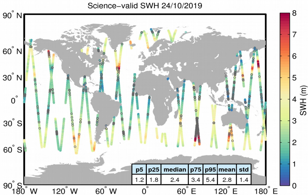
Figure 19. Geographical distribution of science-valid SWH data over oceans and lakes for 24/10/2019. The statistical values shown in the table refer to the SWH in m and are calculated over all measurements shown in the figure. Gray circles denote records that have been rejected based on the editing criteria described in Table 3.
