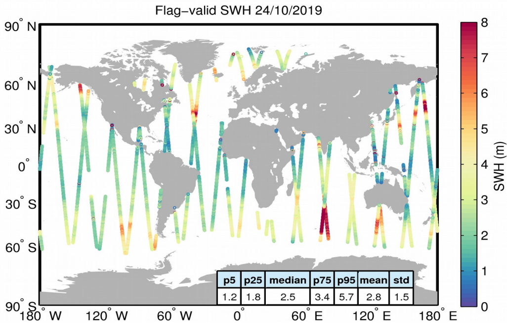
Figure 15. Geographical distribution of flag-valid SWH data over oceans and lakes for 24/10/2019. The statistical values shown in the table refer to the SWH in m and are calculated over all measurements shown in the figure.
