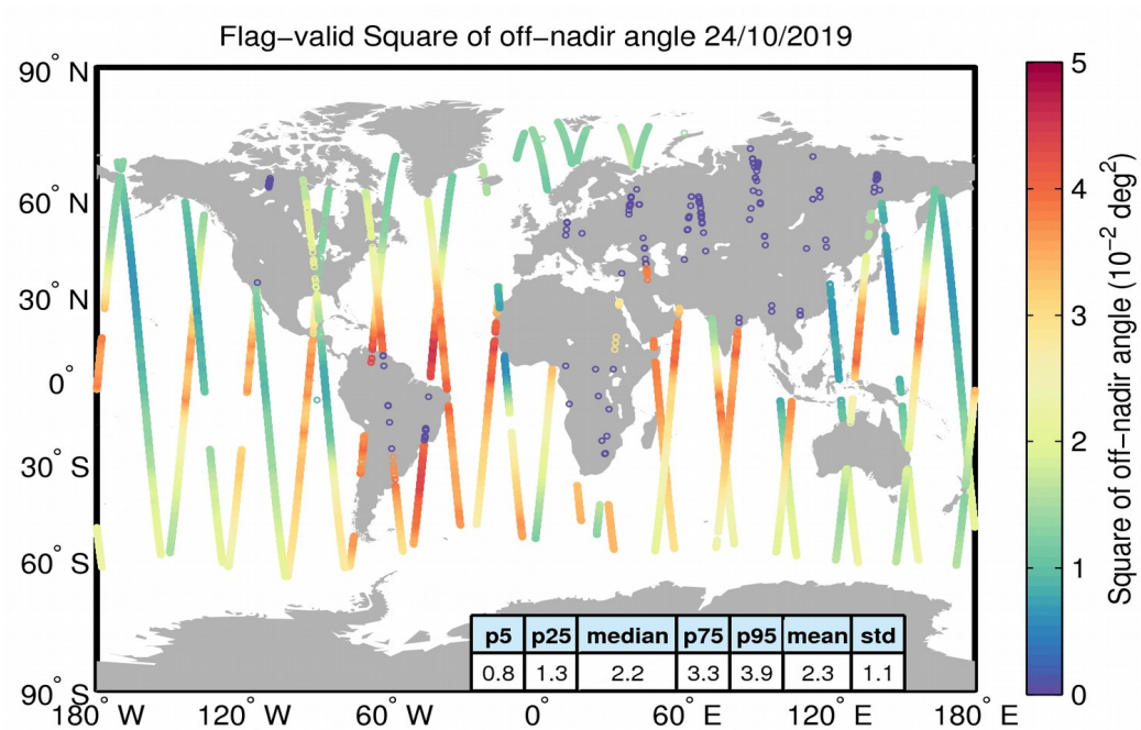
Figure 37. Geographical distribution of flag-valid mispointing data over oceans and lakes for 24/10/2019. The statistical values shown in the table refer to the mispointing in 10^{-2} \text{ deg}^2 and are calculated over all measurements shown in the figure.
