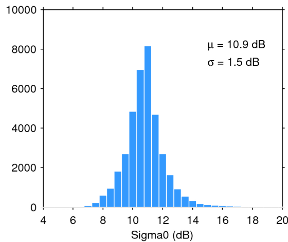
Figure 28. Histogram of science-valid sigma0 over oceans and lakes for 24/10/2019. The mean ( \mu ) and standard deviation ( \sigma ) are also shown. Note that values outside [4 20] dB are excluded from the histogram for the sake of readability but not from the computation of \mu and \sigma .
