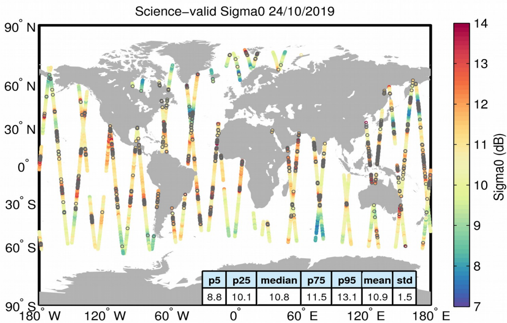
Figure 27. Geographical distribution of science-valid sigma0 data over oceans and lakes for 24/10/2019. The statistical values shown in the table refer to the sigma0 in dB and are calculated over all measurements shown in the figure. Gray circles denote records that have been rejected based on the editing criteria described in Table 4.
