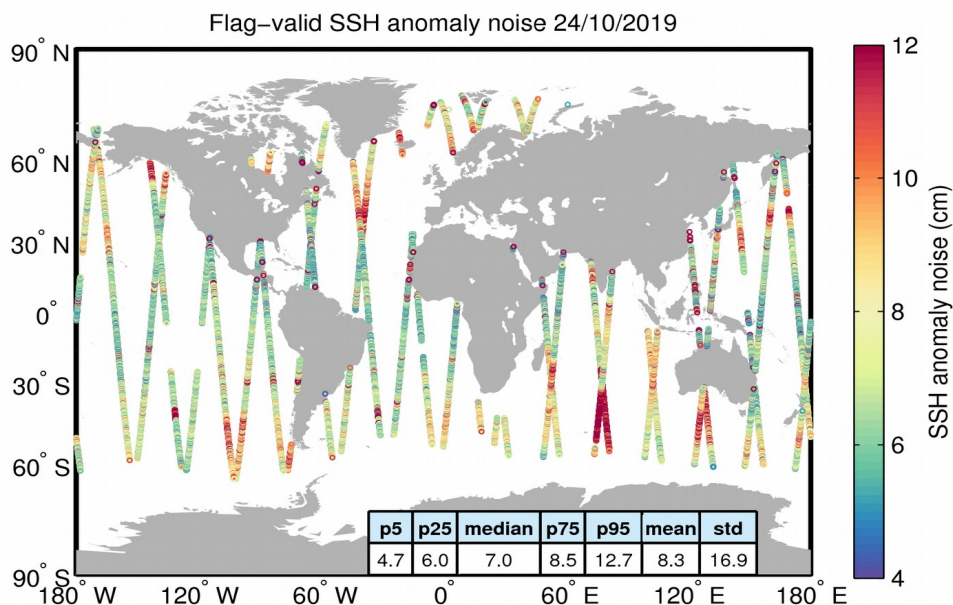
Figure 8. Geographical distribution of flag-valid 20-Hz SSH anomaly measurement noise over oceans and lakes for 24/10/2019. The statistical values shown in the table refer to the SSH anomaly noise and are calculated over all measurements shown in the figure.
