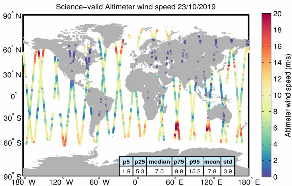
Figure 34. Geographical distribution of science-valid wind data over oceans and lakes for 23/10/2019. The statistical values shown in the table refer to the wind in m/s and are calculated over all measurements shown in the figure. Gray circles denote records that have been rejected based on the editing criteria described in Table 5.
