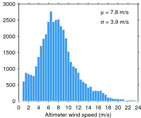
Figure 33. Histogram of flag-valid wind over oceans and lakes for 23/10/2019. The mean ( \mu ) and standard deviation ( \sigma ) are also shown. Note that values larger than 24 m/s are excluded from the histogram for the sake of readability but not from the computation of \mu and \sigma .
