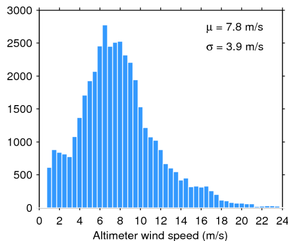
Figure 35. Histogram of science-valid wind over oceans and lakes for 23/10/2019. The mean ( \mu ) and standard deviation ( \sigma ) are also shown. Note that values larger than 24 m/s are excluded from the histogram for the sake of readability but not from the computation of \mu and \sigma .
