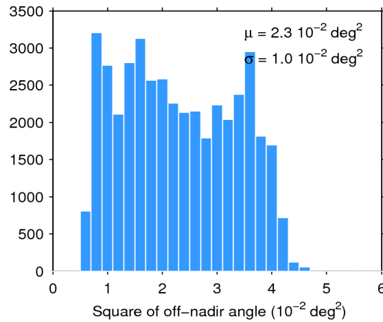
Figure 39. Histogram of flag-valid mispointing over oceans and lakes for 23/10/2019. The mean ( \mu ) and standard deviation ( \sigma ) are also shown. Note that values larger than 6 \cdot 10^{-2} \text{ deg}^2 are excluded from the histogram for the sake of readability but not from the computation of \mu and \sigma .
