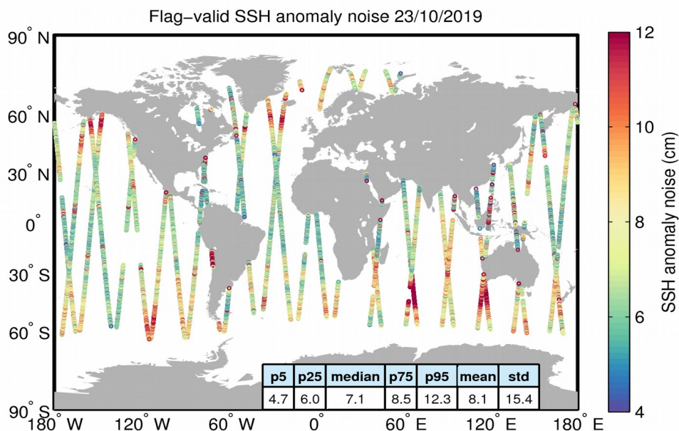
Figure 8. Geographical distribution of flag-valid 20-Hz SSH anomaly measurement noise over oceans and lakes for 23/10/2019. The statistical values shown in the table refer to the SSH anomaly noise and are calculated over all measurements shown in the figure.
