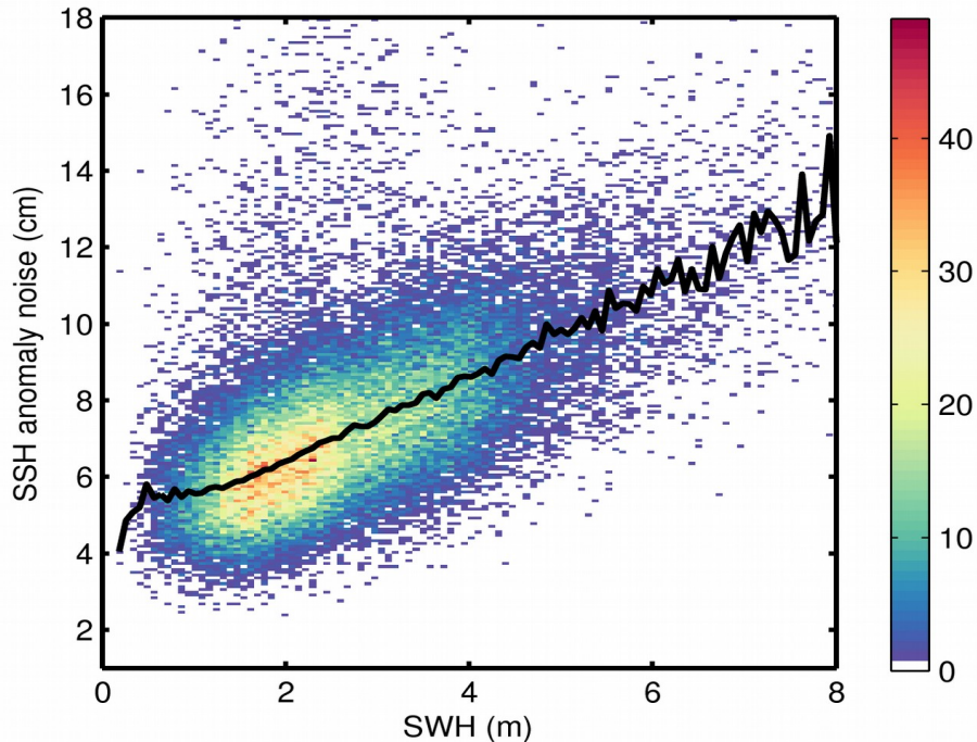
Figure 9. 2D histogram showing flag-valid SSH anomaly noise as a function of SWH for 23/10/2019. The black line denotes the median SSH anomaly noise as a function of SWH.
