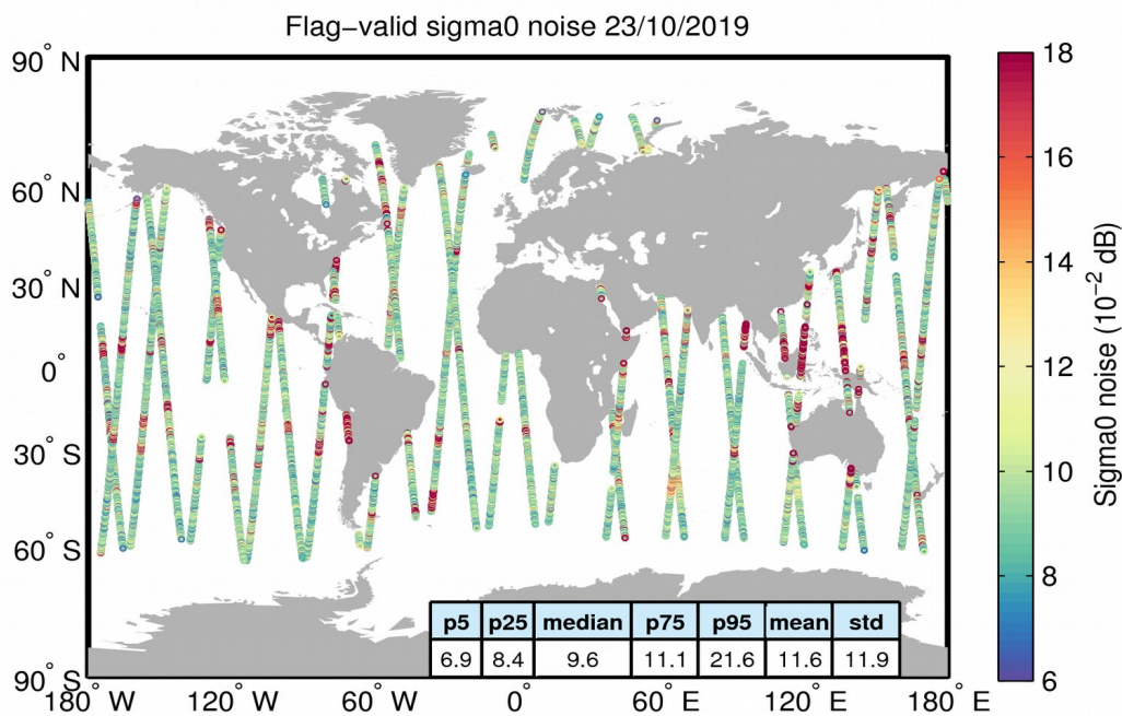
Figure 26. Geographical distribution of flag-valid 20-Hz sigma0 measurement noise over oceans and lakes for 23/10/2019. The statistical values shown in the table refer to the sigma0 noise and are calculated over all measurements shown in the figure.
