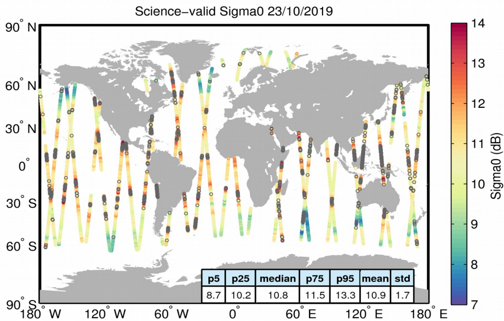
Figure 27. Geographical distribution of science-valid sigma0 data over oceans and lakes for 23/10/2019. The statistical values shown in the table refer to the sigma0 in dB and are calculated over all measurements shown in the figure. Gray circles denote records that have been rejected based on the editing criteria described in Table 4.
