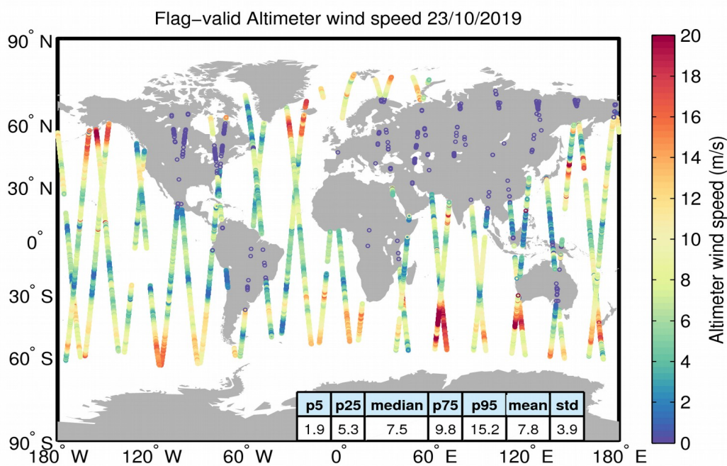
Figure 31. Geographical distribution of flag-valid wind data over oceans and lakes for 23/10/2019. The statistical values shown in the table refer to the wind in m/s and are calculated over all measurements shown in the figure.
