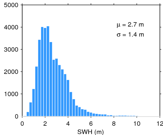
Figure 20. Histogram of science-valid SWH over oceans and lakes for 23/10/2019. The mean ( \mu ) and standard deviation ( \sigma ) are also shown. Note that values larger than 12 m are excluded from the histogram for the sake of readability but not from the computation of \mu and \sigma .
