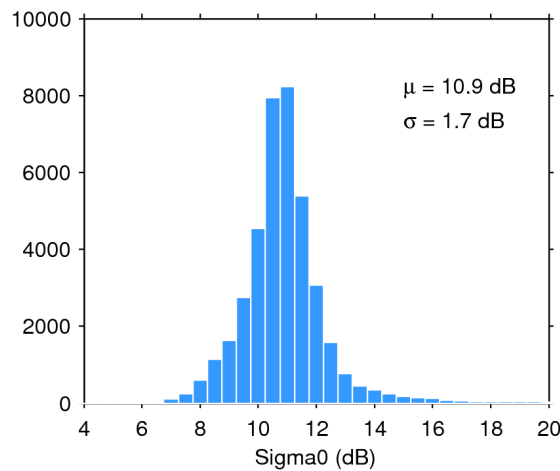
Figure 28. Histogram of science-valid sigma0 over oceans and lakes for 23/10/2019. The mean ( \mu ) and standard deviation ( \sigma ) are also shown. Note that values outside [4 20] dB are excluded from the histogram for the sake of readability but not from the computation of \mu and \sigma .
