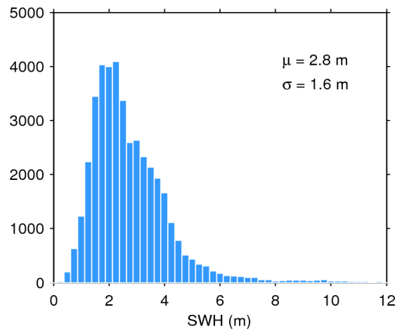
Figure 17. Histogram of flag-valid SWH over oceans and lakes for 23/10/2019. The mean ( \mu ) and standard deviation ( \sigma ) are also shown. Note that values larger than 12 m are excluded from the histogram for the sake of readability but not from the computation of \mu and \sigma .
