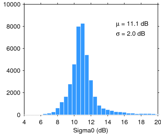
Figure 25. Histogram of flag-valid sigma0 over oceans and lakes for 23/10/2019. The mean ( \mu ) and standard deviation ( \sigma ) are also shown. Note that values outside [4 20] dB are excluded from the histogram for the sake of readability but not from the computation of \mu and \sigma .
