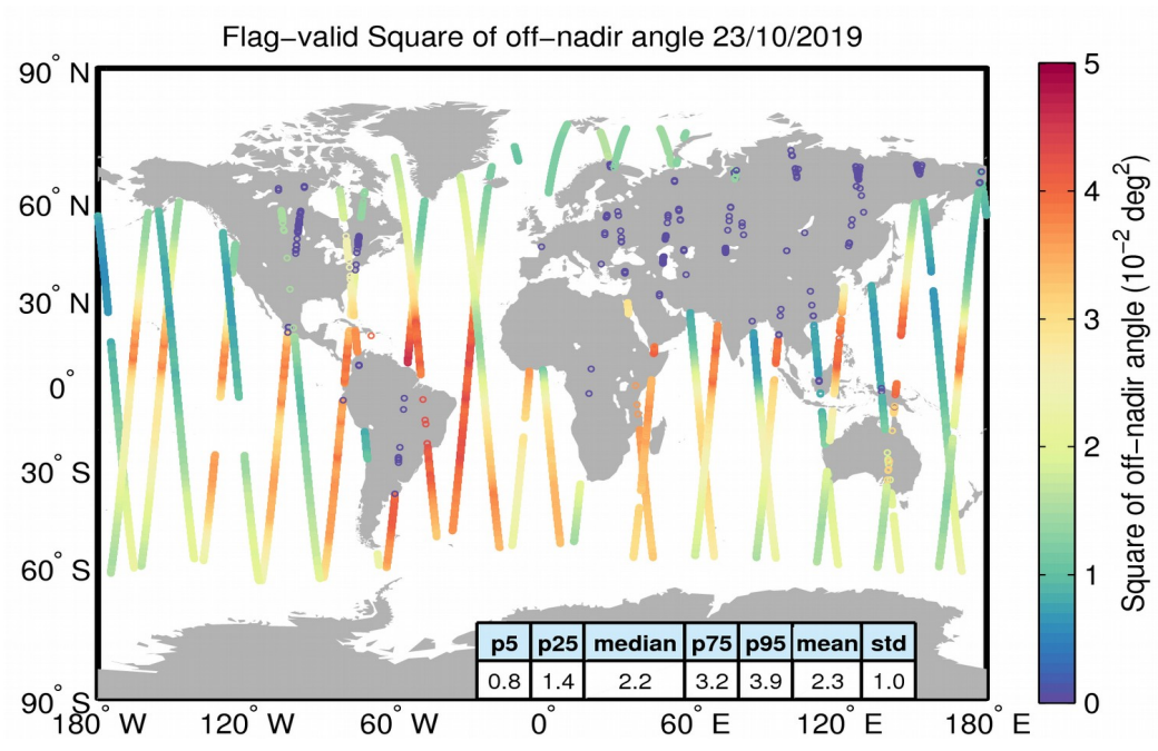
Figure 37. Geographical distribution of flag-valid mispointing data over oceans and lakes for 23/10/2019. The statistical values shown in the table refer to the mispointing in 10^{-2} \text{ deg}^2 and are calculated over all measurements shown in the figure.
