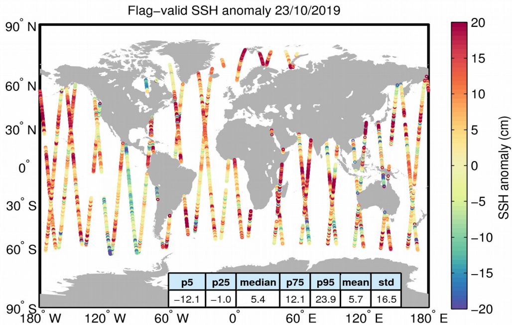
Figure 5. Geographical distribution of flag-valid 1-Hz SSH anomaly data over oceans and lakes for 23/10/2019. The statistical values shown in the table refer to the SSH anomaly in cm and are calculated over all measurements shown in the figure.
