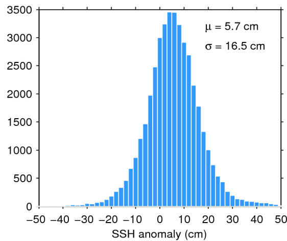
Figure 7. Histogram of flag-valid SSH anomaly over oceans and lakes for 23/10/2019. The mean ( \mu ) and standard deviation ( \sigma ) are also shown. Note that values outside [-50\ 50] cm are excluded from the histogram for the sake of readability but not from the computation of \mu and \sigma .
