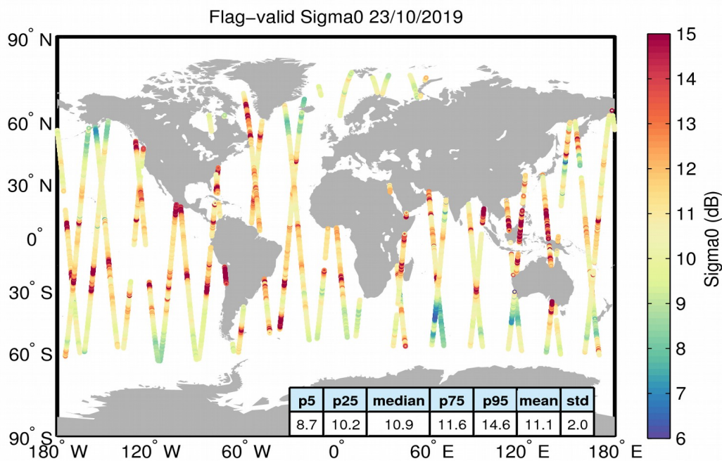
Figure 23. Geographical distribution of flag-valid sigma0 data over oceans and lakes for 23/10/2019. The statistical values shown in the table refer to the sigma0 in dB and are calculated over all measurements shown in the figure.
