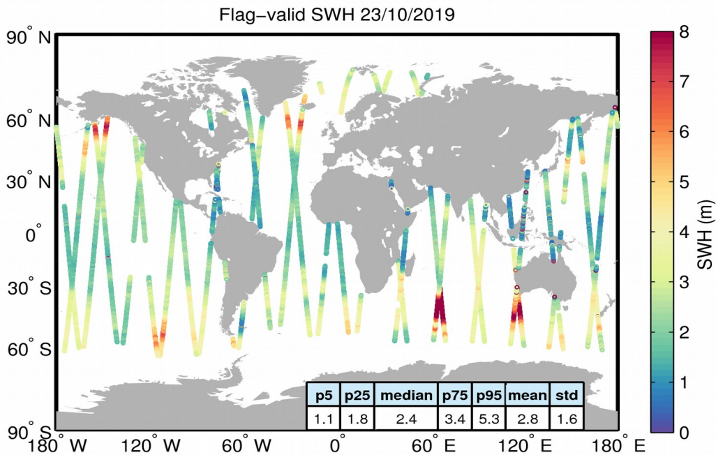
Figure 15. Geographical distribution of flag-valid SWH data over oceans and lakes for 23/10/2019. The statistical values shown in the table refer to the SWH in m and are calculated over all measurements shown in the figure.
