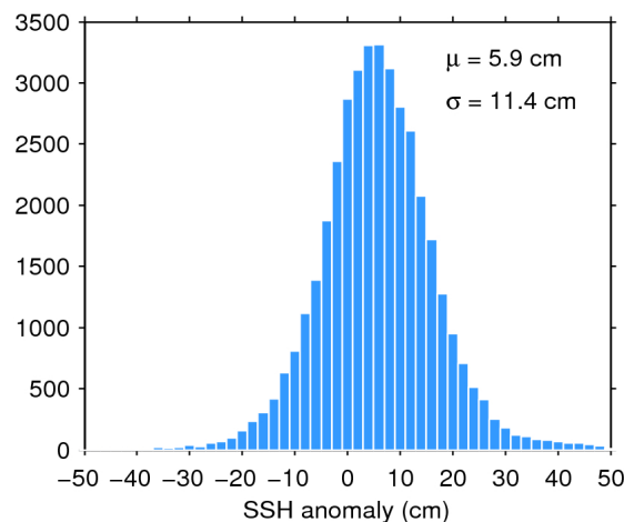
Figure 11. Histogram of science-valid SSH anomaly over oceans and lakes for 23/10/2019. The mean ( \mu ) and standard deviation ( \sigma ) are also shown. Note that values outside [-50 50] cm are excluded from the histogram for the sake of readability but not from the computation of \mu and \sigma .
