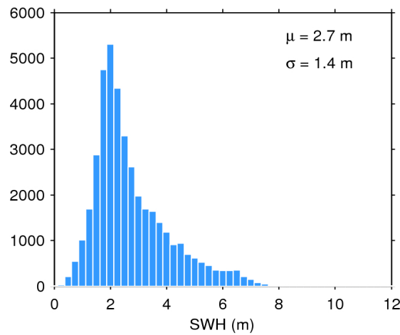
Figure 17. Histogram of flag-valid SWH over oceans and lakes for 21/10/2019. The mean ( \mu ) and standard deviation ( \sigma ) are also shown. Note that values larger than 12 m are excluded from the histogram for the sake of readability but not from the computation of \mu and \sigma .
