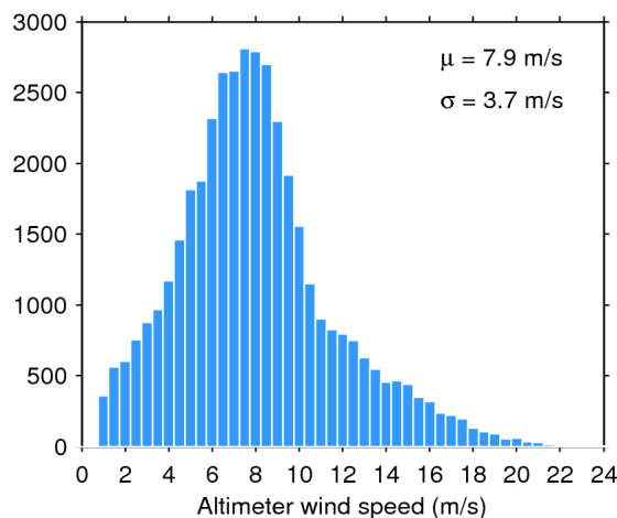
Figure 35. Histogram of science-valid wind over oceans and lakes for 21/10/2019. The mean ( \mu ) and standard deviation ( \sigma ) are also shown. Note that values larger than 24 m/s are excluded from the histogram for the sake of readability but not from the computation of \mu and \sigma .
