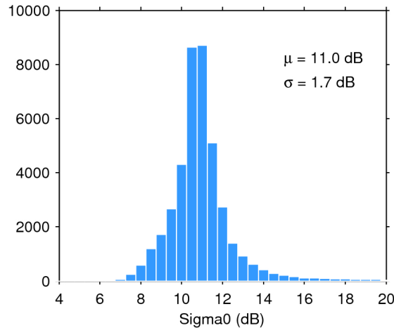
Figure 25. Histogram of flag-valid sigma0 over oceans and lakes for 21/10/2019. The mean ( \mu ) and standard deviation ( \sigma ) are also shown. Note that values outside [4 20] dB are excluded from the histogram for the sake of readability but not from the computation of \mu and \sigma .
