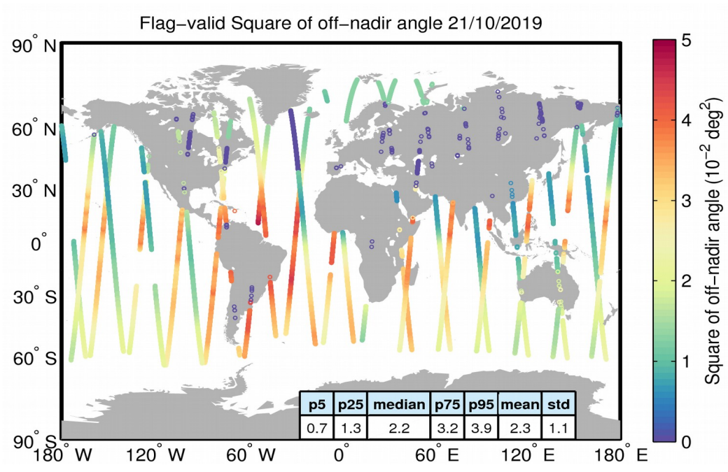
Figure 37. Geographical distribution of flag-valid mispointing data over oceans and lakes for 21/10/2019. The statistical values shown in the table refer to the mispointing in 10^{-2} \text{ deg}^2 and are calculated over all measurements shown in the figure.
