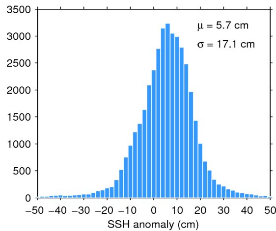
Figure 7. Histogram of flag-valid SSH anomaly over oceans and lakes for 21/10/2019. The mean ( \mu ) and standard deviation ( \sigma ) are also shown. Note that values outside [-50 50] cm are excluded from the histogram for the sake of readability but not from the computation of \mu and \sigma .
