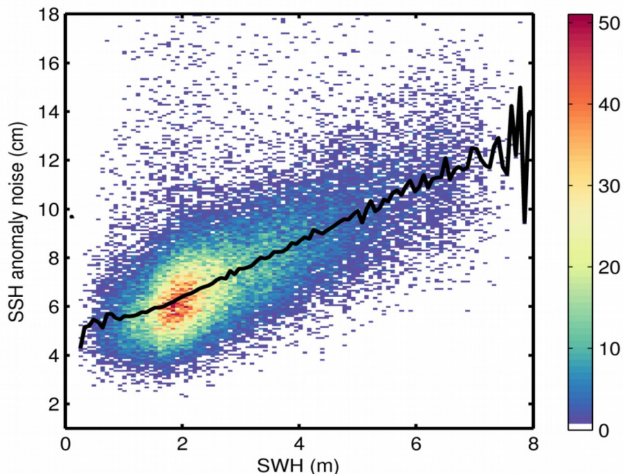
Figure 9. 2D histogram showing flag-valid SSH anomaly noise as a function of SWH for 21/10/2019. The black line denotes the median SSH anomaly noise as a function of SWH.
