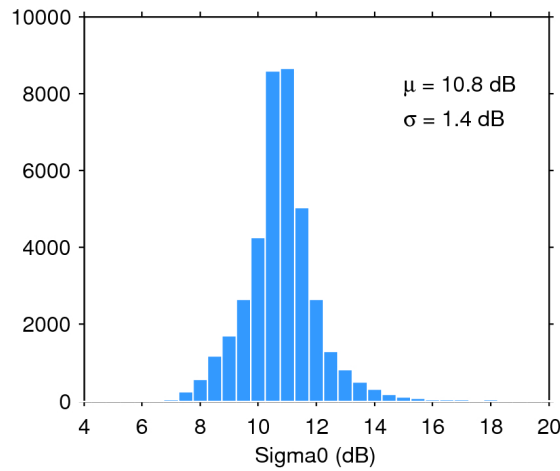
Figure 28. Histogram of science-valid sigma0 over oceans and lakes for 21/10/2019. The mean ( \mu ) and standard deviation ( \sigma ) are also shown. Note that values outside [4 20] dB are excluded from the histogram for the sake of readability but not from the computation of \mu and \sigma .
