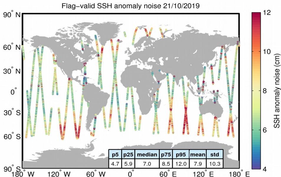
Figure 8. Geographical distribution of flag-valid 20-Hz SSH anomaly measurement noise over oceans and lakes for 21/10/2019. The statistical values shown in the table refer to the SSH anomaly noise and are calculated over all measurements shown in the figure.
