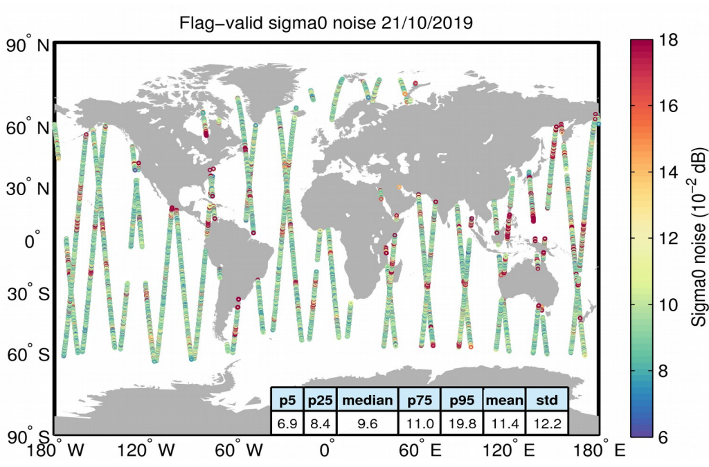
Figure 26. Geographical distribution of flag-valid 20-Hz sigma0 measurement noise over oceans and lakes for 21/10/2019. The statistical values shown in the table refer to the sigma0 noise and are calculated over all measurements shown in the figure.
