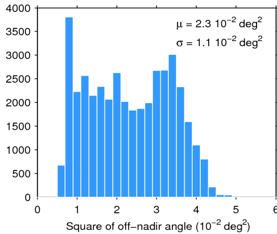
Figure 39. Histogram of flag-valid mispointing over oceans and lakes for 21/10/2019. The mean ( \mu ) and standard deviation ( \sigma ) are also shown. Note that values larger than 6 \cdot 10^{-2} \text{ deg}^2 are excluded from the histogram for the sake of readability but not from the computation of \mu and \sigma .
