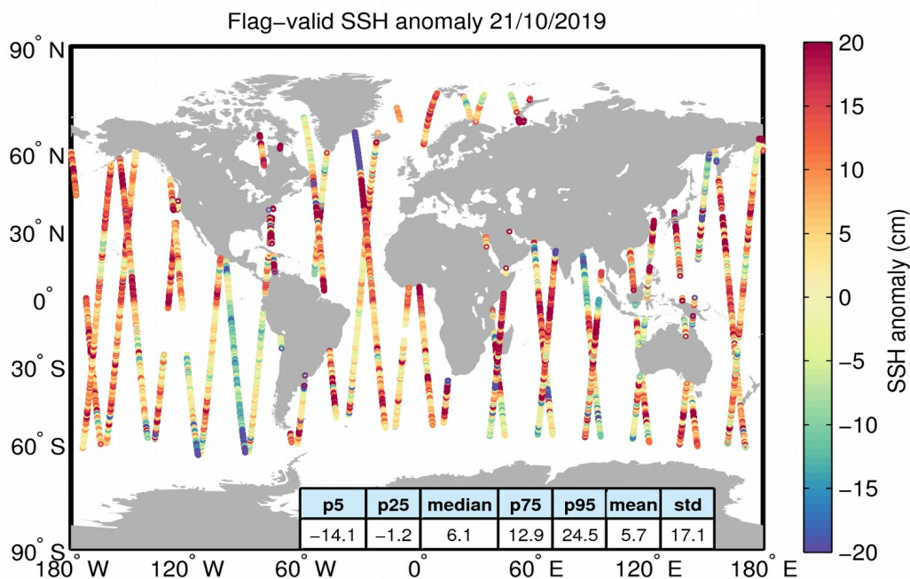
Figure 5. Geographical distribution of flag-valid 1-Hz SSH anomaly data over oceans and lakes for 21/10/2019. The statistical values shown in the table refer to the SSH anomaly in cm and are calculated over all measurements shown in the figure.
