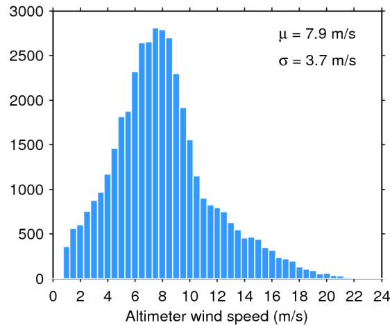
Figure 33. Histogram of flag-valid wind over oceans and lakes for 21/10/2019. The mean ( \mu ) and standard deviation ( \sigma ) are also shown. Note that values larger than 24 m/s are excluded from the histogram for the sake of readability but not from the computation of \mu and \sigma .
