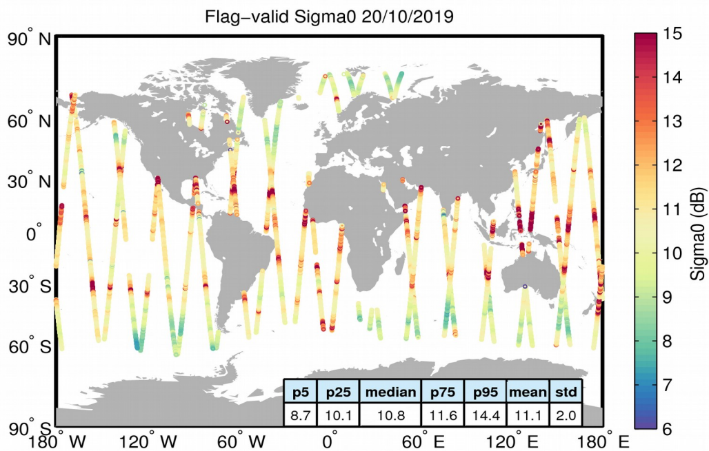
Figure 23. Geographical distribution of flag-valid sigma0 data over oceans and lakes for 20/10/2019. The statistical values shown in the table refer to the sigma0 in dB and are calculated over all measurements shown in the figure.
