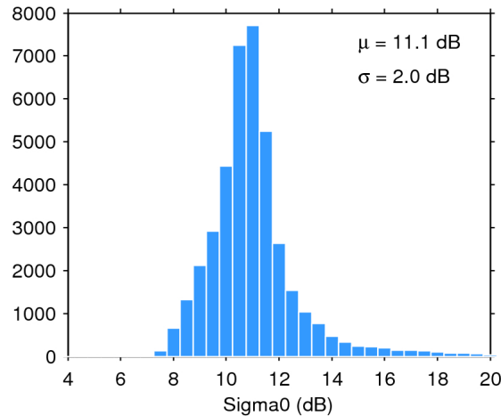
Figure 25. Histogram of flag-valid sigma0 over oceans and lakes for 20/10/2019. The mean ( \mu ) and standard deviation ( \sigma ) are also shown. Note that values outside [4 20] dB are excluded from the histogram for the sake of readability but not from the computation of \mu and \sigma .
