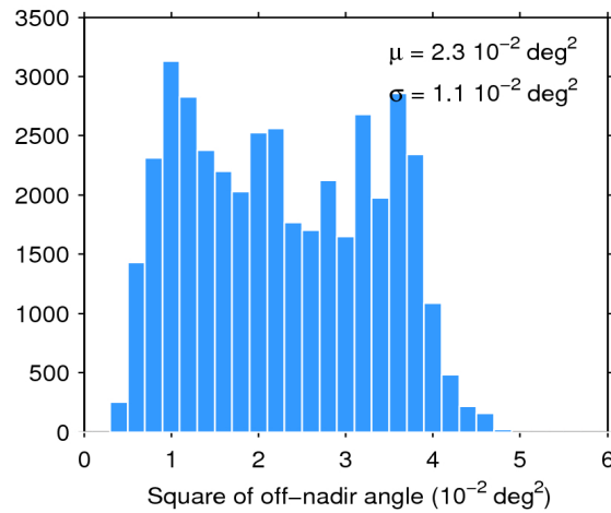
Figure 39. Histogram of flag-valid mispointing over oceans and lakes for 20/10/2019. The mean ( \mu ) and standard deviation ( \sigma ) are also shown. Note that values larger than 6 \cdot 10^{-2} \text{ deg}^2 are excluded from the histogram for the sake of readability but not from the computation of \mu and \sigma .
