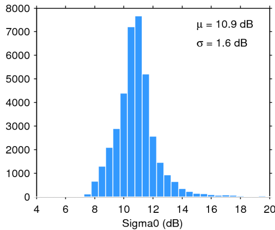
Figure 28. Histogram of science-valid sigma0 over oceans and lakes for 20/10/2019. The mean ( \mu ) and standard deviation ( \sigma ) are also shown. Note that values outside [4 20] dB are excluded from the histogram for the sake of readability but not from the computation of \mu and \sigma .
