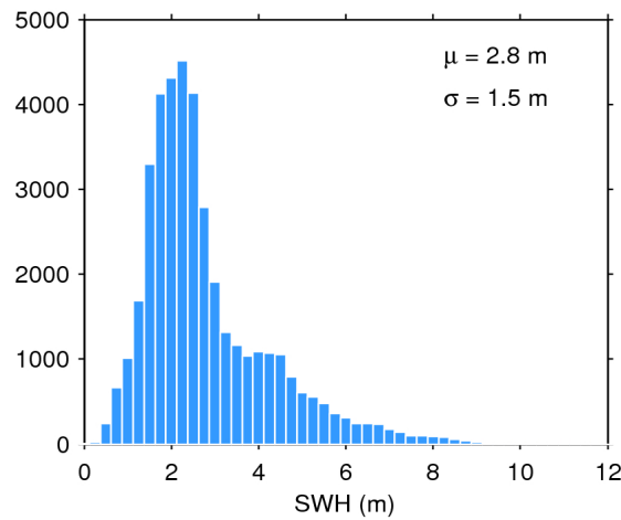
Figure 17. Histogram of flag-valid SWH over oceans and lakes for 20/10/2019. The mean ( \mu ) and standard deviation ( \sigma ) are also shown. Note that values larger than 12 m are excluded from the histogram for the sake of readability but not from the computation of \mu and \sigma .
