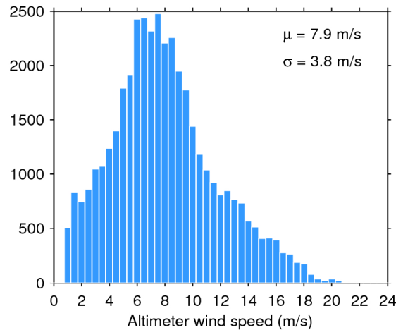
Figure 33. Histogram of flag-valid wind over oceans and lakes for 20/10/2019. The mean ( \mu ) and standard deviation ( \sigma ) are also shown. Note that values larger than 24 m/s are excluded from the histogram for the sake of readability but not from the computation of \mu and \sigma .
