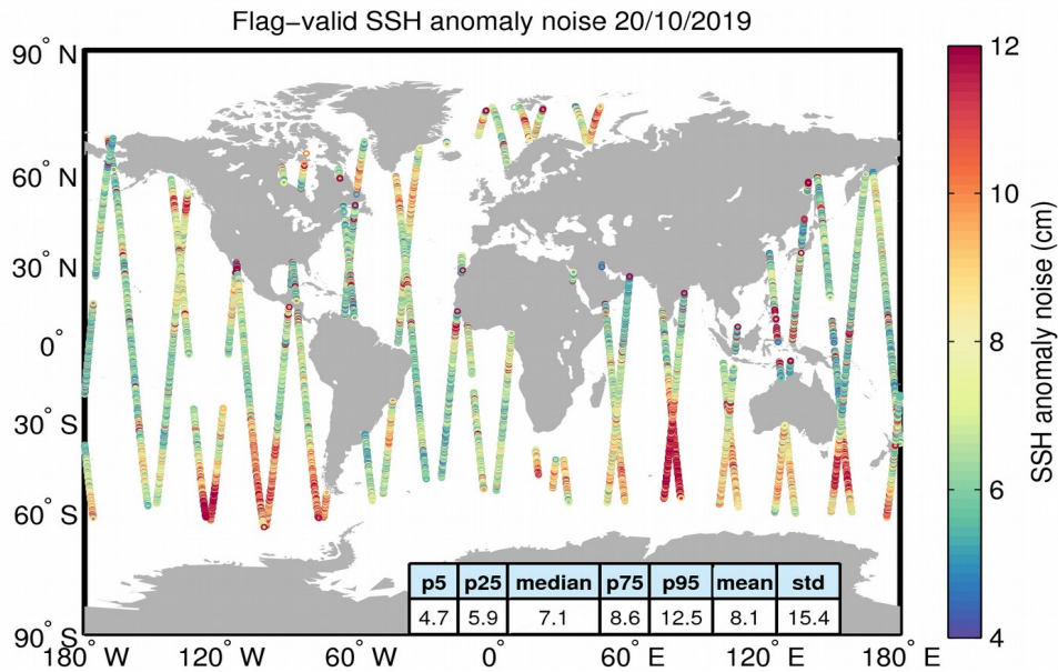
Figure 8. Geographical distribution of flag-valid 20-Hz SSH anomaly measurement noise over oceans and lakes for 20/10/2019. The statistical values shown in the table refer to the SSH anomaly noise and are calculated over all measurements shown in the figure.
