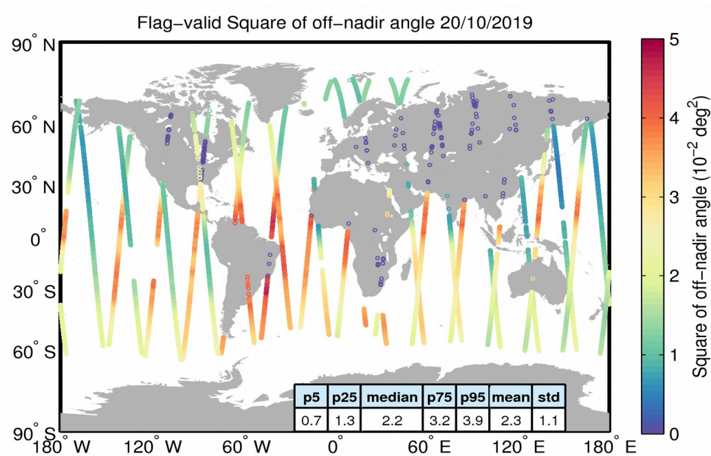
Figure 37. Geographical distribution of flag-valid mispointing data over oceans and lakes for 20/10/2019. The statistical values shown in the table refer to the mispointing in 10^{-2} deg 2 and are calculated over all measurements shown in the figure.
