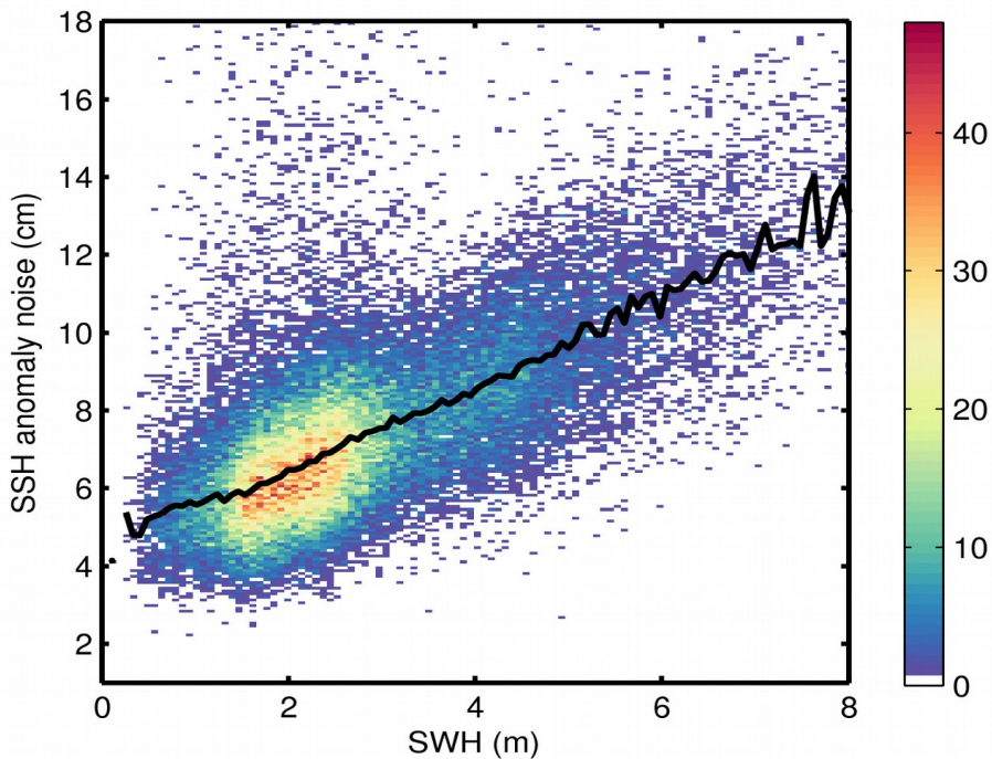
Figure 9. 2D histogram showing flag-valid SSH anomaly noise as a function of SWH for 20/10/2019. The black line denotes the median SSH anomaly noise as a function of SWH.
