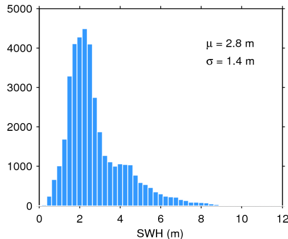
Figure 20. Histogram of science-valid SWH over oceans and lakes for 20/10/2019. The mean ( \mu ) and standard deviation ( \sigma ) are also shown. Note that values larger than 12 m are excluded from the histogram for the sake of readability but not from the computation of \mu and \sigma .
