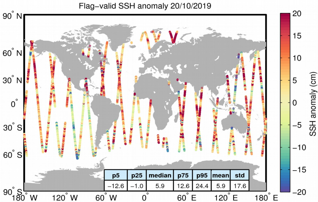
Figure 5. Geographical distribution of flag-valid 1-Hz SSH anomaly data over oceans and lakes for 20/10/2019. The statistical values shown in the table refer to the SSH anomaly in cm and are calculated over all measurements shown in the figure.
