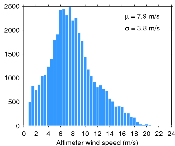
Figure 35. Histogram of science-valid wind over oceans and lakes for 20/10/2019. The mean ( \mu ) and standard deviation ( \sigma ) are also shown. Note that values larger than 24 m/s are excluded from the histogram for the sake of readability but not from the computation of \mu and \sigma .
