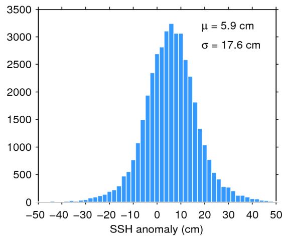
Figure 7. Histogram of flag-valid SSH anomaly over oceans and lakes for 20/10/2019. The mean ( \mu ) and standard deviation ( \sigma ) are also shown. Note that values outside [-50 50] cm are excluded from the histogram for the sake of readability but not from the computation of \mu and \sigma .
