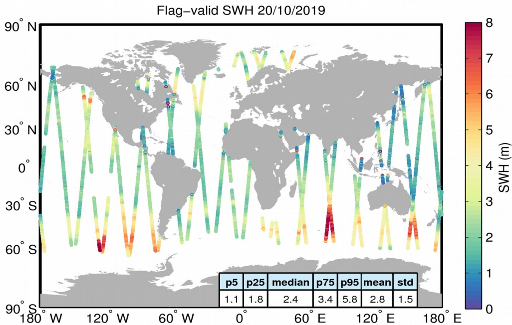
Figure 15. Geographical distribution of flag-valid SWH data over oceans and lakes for 20/10/2019. The statistical values shown in the table refer to the SWH in m and are calculated over all measurements shown in the figure.
