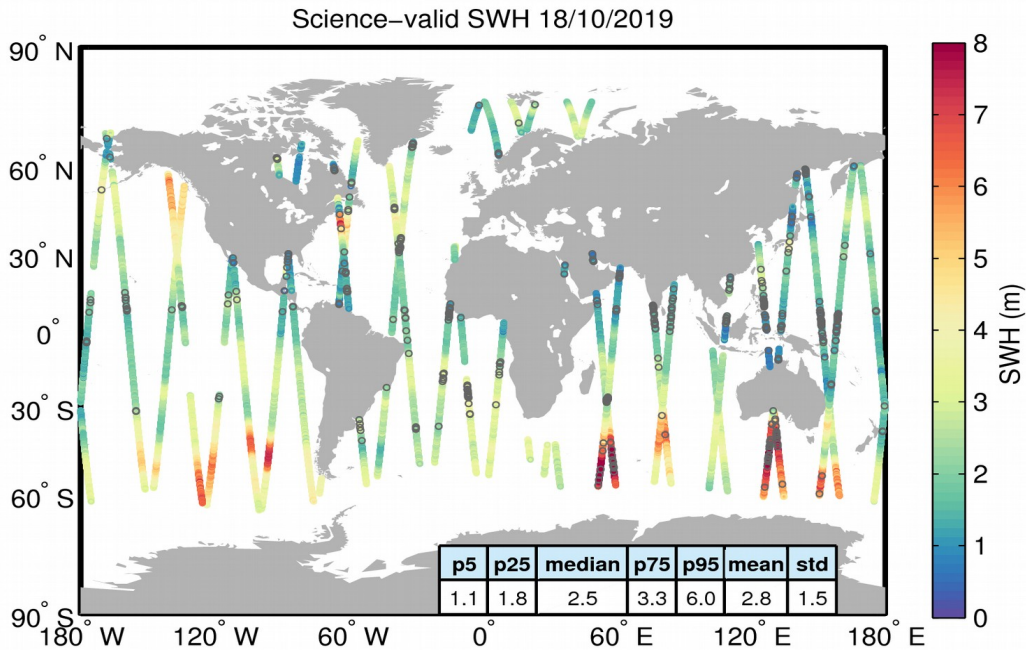
Figure 19. Geographical distribution of science-valid SWH data over oceans and lakes for 18/10/2019. The statistical values shown in the table refer to the SWH in m and are calculated over all measurements shown in the figure. Gray circles denote records that have been rejected based on the editing criteria described in Table 3.
