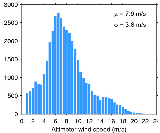
Figure 33. Histogram of flag-valid wind over oceans and lakes for 18/10/2019. The mean ( \mu ) and standard deviation ( \sigma ) are also shown. Note that values larger than 24 m/s are excluded from the histogram for the sake of readability but not from the computation of \mu and \sigma .
