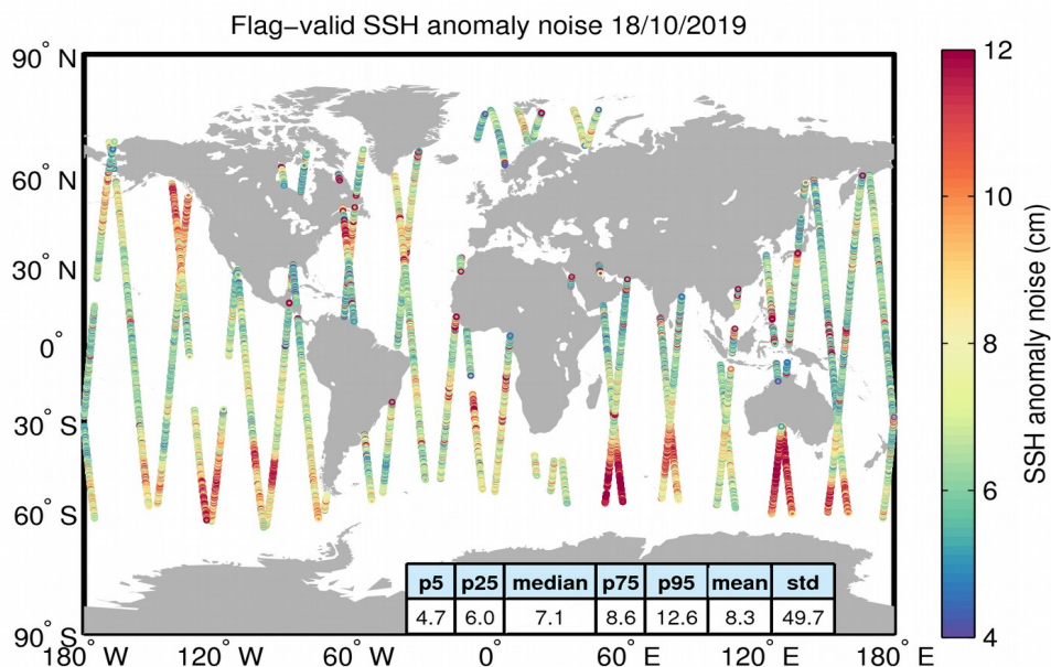
Figure 8. Geographical distribution of flag-valid 20-Hz SSH anomaly measurement noise over oceans and lakes for 18/10/2019. The statistical values shown in the table refer to the SSH anomaly noise and are calculated over all measurements shown in the figure.
