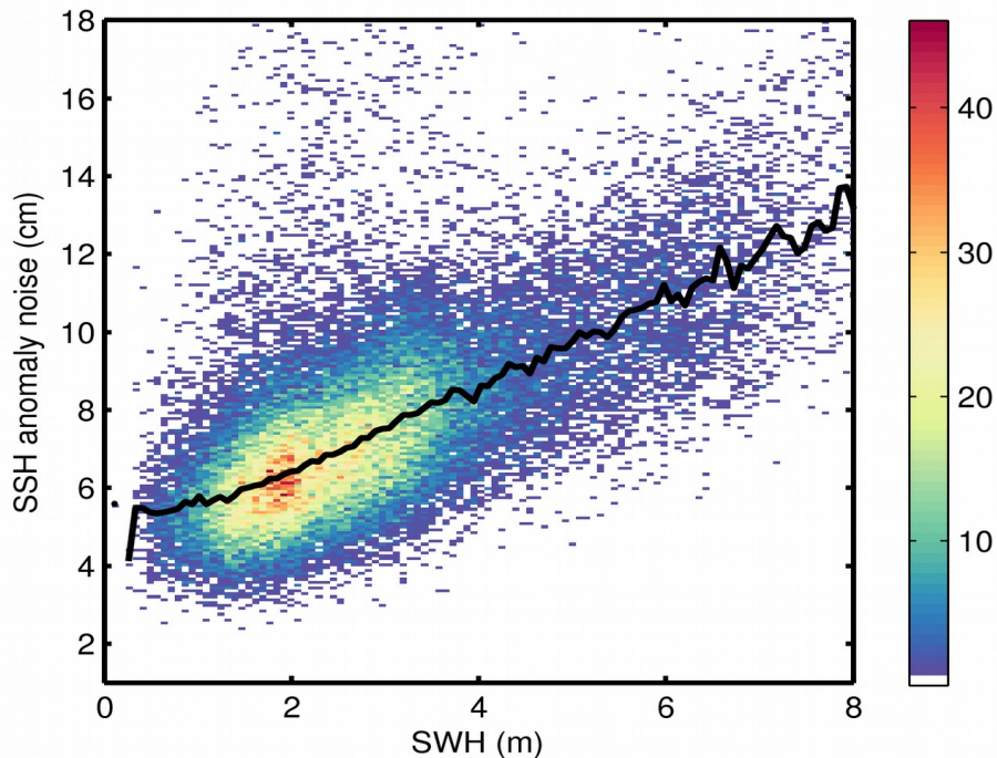
Figure 9. 2D histogram showing flag-valid SSH anomaly noise as a function of SWH for 18/10/2019. The black line denotes the median SSH anomaly noise as a function of SWH.
