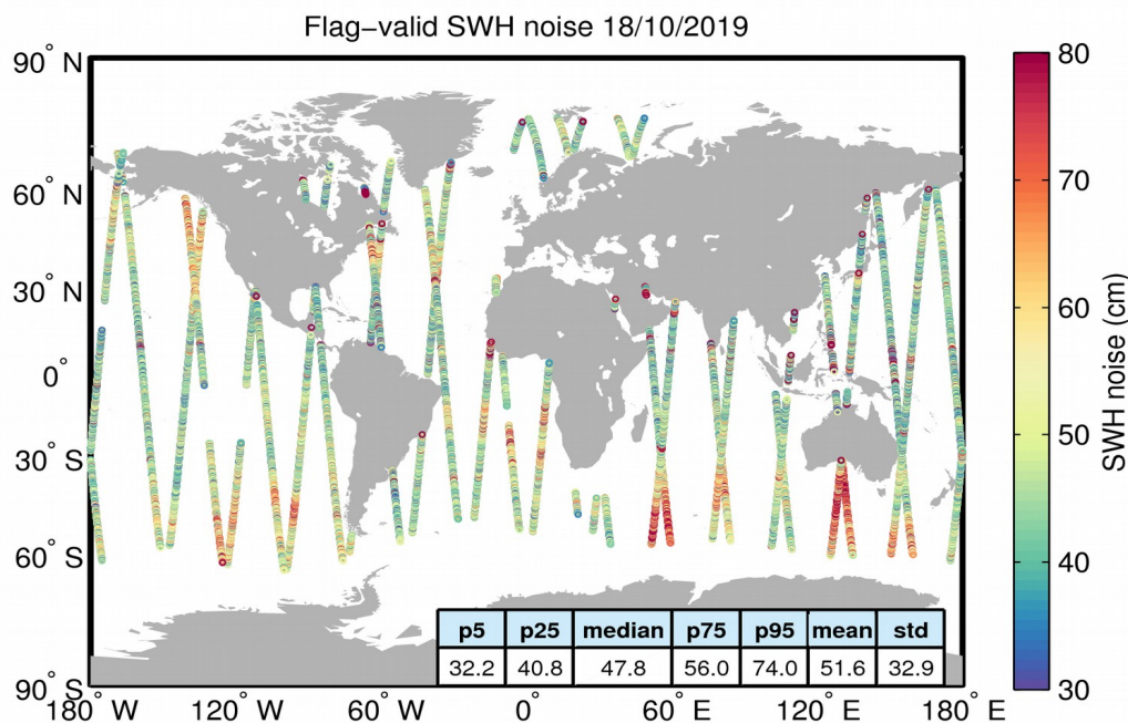
Figure 18. Geographical distribution of flag-valid 20-Hz SWH measurement noise over oceans and lakes for 18/10/2019. The statistical values shown in the figure refer to the SWH noise and are calculated over all measurements shown in the figure.
