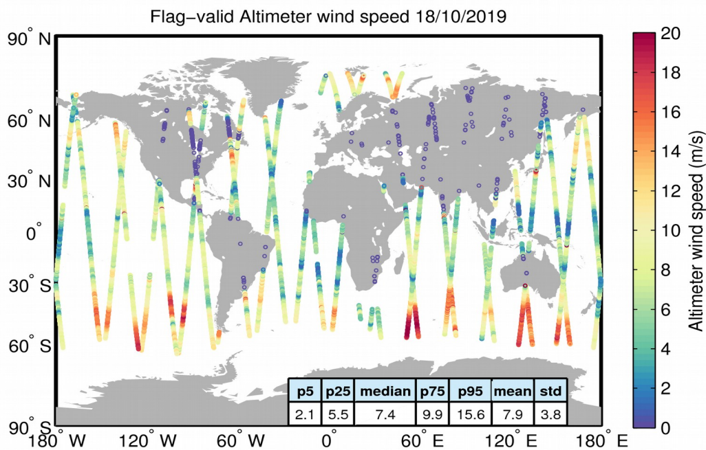
Figure 31. Geographical distribution of flag-valid wind data over oceans and lakes for 18/10/2019. The statistical values shown in the table refer to the wind in m/s and are calculated over all measurements shown in the figure.
