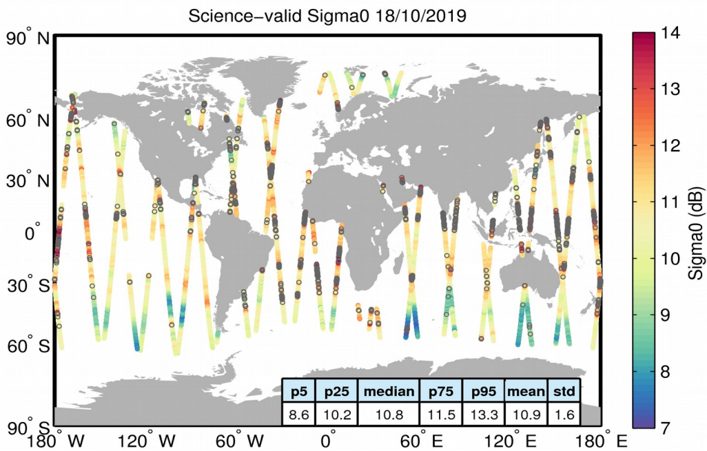
Figure 27. Geographical distribution of science-valid sigma0 data over oceans and lakes for 18/10/2019. The statistical values shown in the table refer to the sigma0 in dB and are calculated over all measurements shown in the figure. Gray circles denote records that have been rejected based on the editing criteria described in Table 4.
