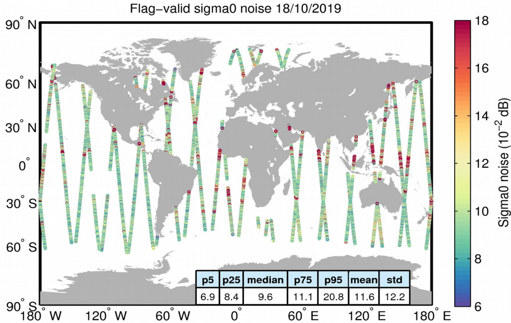
Figure 26. Geographical distribution of flag-valid 20-Hz sigma0 measurement noise over oceans and lakes for 18/10/2019. The statistical values shown in the table refer to the sigma0 noise and are calculated over all measurements shown in the figure.
