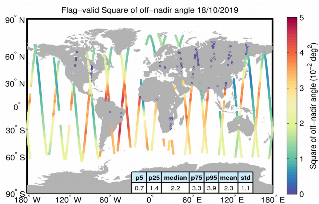
Figure 37. Geographical distribution of flag-valid mispointing data over oceans and lakes for 18/10/2019. The statistical values shown in the table refer to the mispointing in 10^{-2} \text{deg}^2 and are calculated over all measurements shown in the figure.
