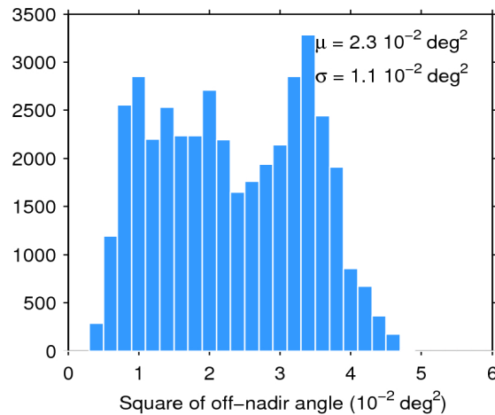
Figure 39. Histogram of flag-valid mispointing over oceans and lakes for 18/10/2019. The mean ( \mu ) and standard deviation ( \sigma ) are also shown. Note that values larger than 6 \cdot 10^{-2} \text{ deg}^2 are excluded from the histogram for the sake of readability but not from the computation of \mu and \sigma .
