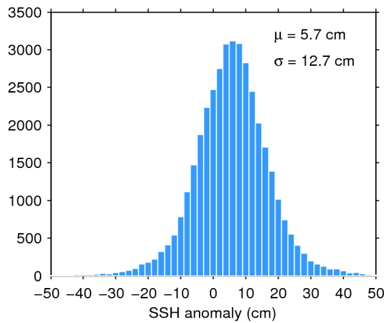
Figure 11. Histogram of science-valid SSH anomaly over oceans and lakes for 18/10/2019. The mean ( \mu ) and standard deviation ( \sigma ) are also shown. Note that values outside [-50 50] cm are excluded from the histogram for the sake of readability but not from the computation of \mu and \sigma .
