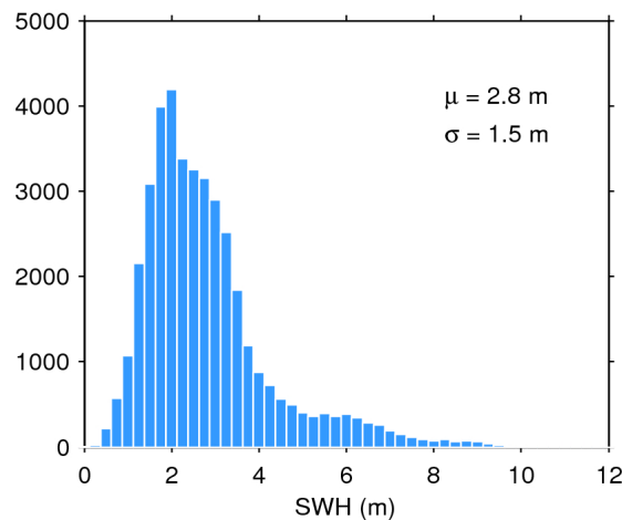
Figure 20. Histogram of science-valid SWH over oceans and lakes for 18/10/2019. The mean ( \mu ) and standard deviation ( \sigma ) are also shown. Note that values larger than 12 m are excluded from the histogram for the sake of readability but not from the computation of \mu and \sigma .
