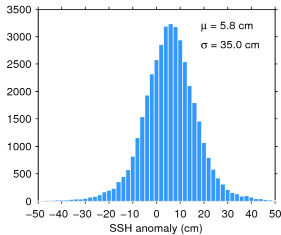
Figure 7. Histogram of flag-valid SSH anomaly over oceans and lakes for 18/10/2019. The mean ( \mu ) and standard deviation ( \sigma ) are also shown. Note that values outside [-50\ 50] cm are excluded from the histogram for the sake of readability but not from the computation of \mu and \sigma .
