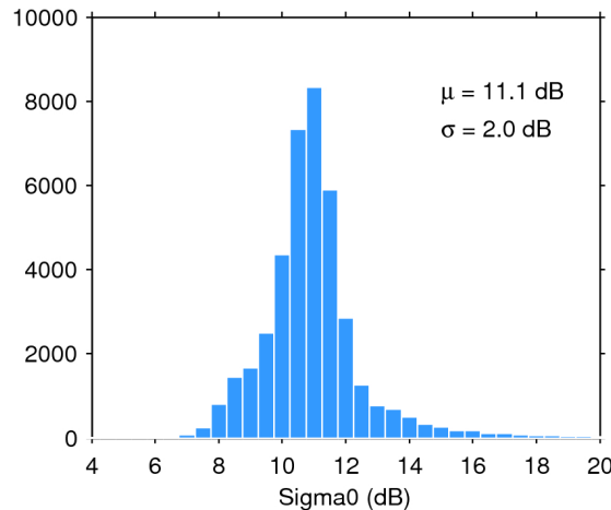
Figure 25. Histogram of flag-valid sigma0 over oceans and lakes for 18/10/2019. The mean ( \mu ) and standard deviation ( \sigma ) are also shown. Note that values outside [4 20] dB are excluded from the histogram for the sake of readability but not from the computation of \mu and \sigma .
