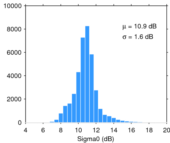
Figure 28. Histogram of science-valid sigma0 over oceans and lakes for 18/10/2019. The mean ( \mu ) and standard deviation ( \sigma ) are also shown. Note that values outside [4 20] dB are excluded from the histogram for the sake of readability but not from the computation of \mu and \sigma .
