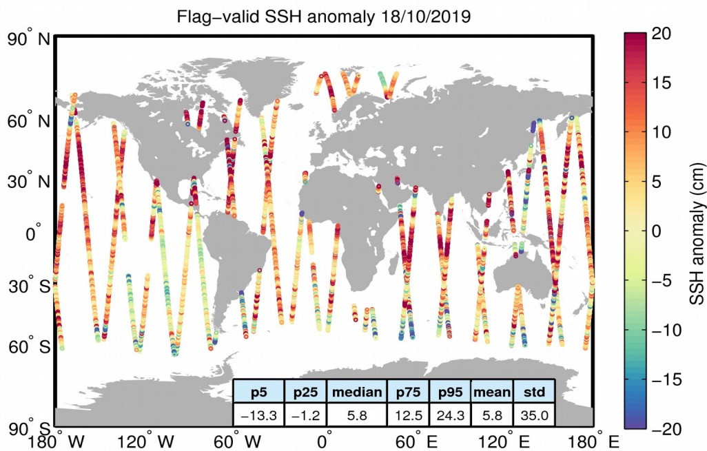
Figure 5. Geographical distribution of flag-valid 1-Hz SSH anomaly data over oceans and lakes for 18/10/2019. The statistical values shown in the table refer to the SSH anomaly in cm and are calculated over all measurements shown in the figure.
