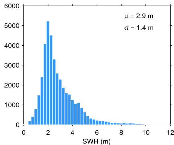
Figure 20. Histogram of science-valid SWH over oceans and lakes for 17/10/2019. The mean ( \mu ) and standard deviation ( \sigma ) are also shown. Note that values larger than 12 m are excluded from the histogram for the sake of readability but not from the computation of \mu and \sigma .
