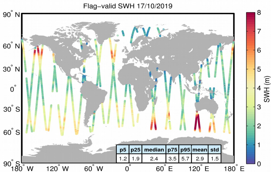
Figure 15. Geographical distribution of flag-valid SWH data over oceans and lakes for 17/10/2019. The statistical values shown in the table refer to the SWH in m and are calculated over all measurements shown in the figure.
