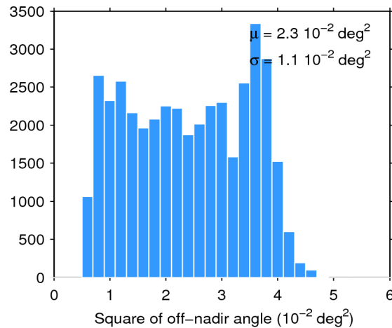
Figure 39. Histogram of flag-valid mispointing over oceans and lakes for 17/10/2019. The mean ( \mu ) and standard deviation ( \sigma ) are also shown. Note that values larger than 6 \cdot 10^{-2} \text{ deg}^2 are excluded from the histogram for the sake of readability but not from the computation of \mu and \sigma .
