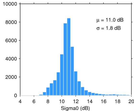
Figure 25. Histogram of flag-valid sigma0 over oceans and lakes for 17/10/2019. The mean ( \mu ) and standard deviation ( \sigma ) are also shown. Note that values outside [4 20] dB are excluded from the histogram for the sake of readability but not from the computation of \mu and \sigma .
