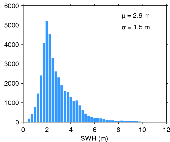
Figure 17. Histogram of flag-valid SWH over oceans and lakes for 17/10/2019. The mean ( \mu ) and standard deviation ( \sigma ) are also shown. Note that values larger than 12 m are excluded from the histogram for the sake of readability but not from the computation of \mu and \sigma .
