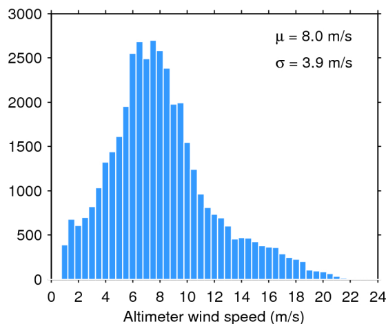
Figure 35. Histogram of science-valid wind over oceans and lakes for 17/10/2019. The mean ( \mu ) and standard deviation ( \sigma ) are also shown. Note that values larger than 24 m/s are excluded from the histogram for the sake of readability but not from the computation of \mu and \sigma .
