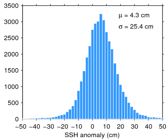
Figure 7. Histogram of flag-valid SSH anomaly over oceans and lakes for 17/10/2019. The mean ( \mu ) and standard deviation ( \sigma ) are also shown. Note that values outside [-50\ 50] cm are excluded from the histogram for the sake of readability but not from the computation of \mu and \sigma .
