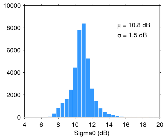
Figure 28. Histogram of science-valid sigma0 over oceans and lakes for 17/10/2019. The mean ( \mu ) and standard deviation ( \sigma ) are also shown. Note that values outside [4 20] dB are excluded from the histogram for the sake of readability but not from the computation of \mu and \sigma .
