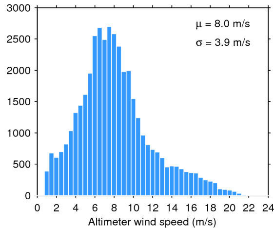
Figure 33. Histogram of flag-valid wind over oceans and lakes for 17/10/2019. The mean ( \mu ) and standard deviation ( \sigma ) are also shown. Note that values larger than 24 m/s are excluded from the histogram for the sake of readability but not from the computation of \mu and \sigma .
