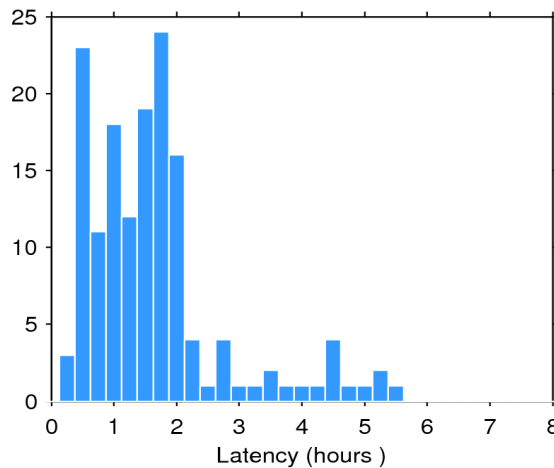
Figure 2. Histogram of the data latency for 17/10/2019. The y-axis denotes the number of files that are made available with a delay of x-hours with respect to the mean time of the records stored in the file.
