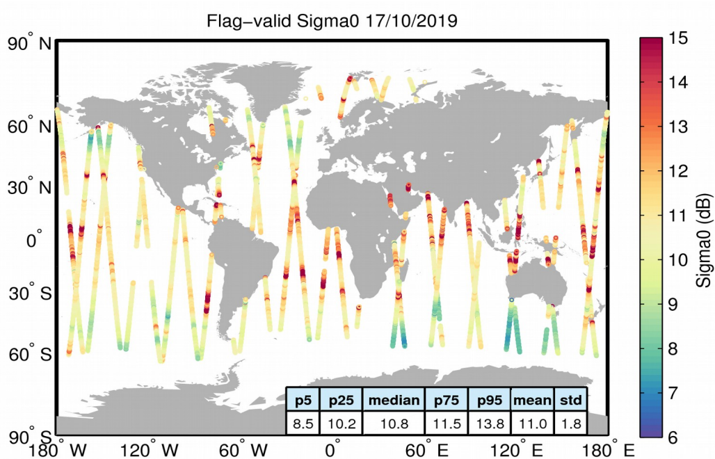
Figure 23. Geographical distribution of flag-valid sigma0 data over oceans and lakes for 17/10/2019. The statistical values shown in the table refer to the sigma0 in dB and are calculated over all measurements shown in the figure.
