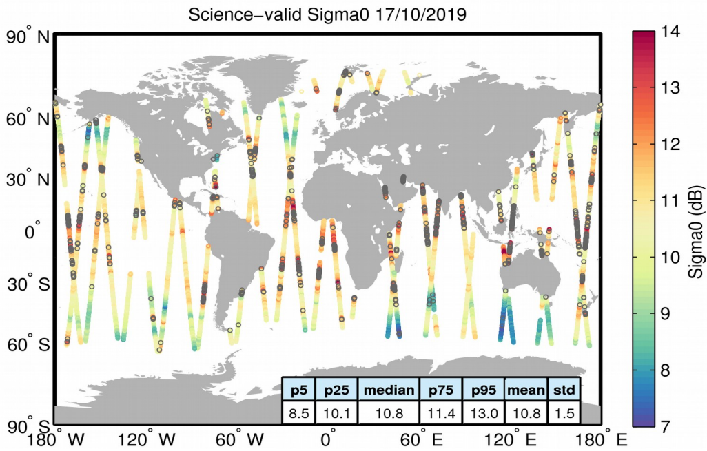
Figure 27. Geographical distribution of science-valid sigma0 data over oceans and lakes for 17/10/2019. The statistical values shown in the table refer to the sigma0 in dB and are calculated over all measurements shown in the figure. Gray circles denote records that have been rejected based on the editing criteria described in Table 4.
