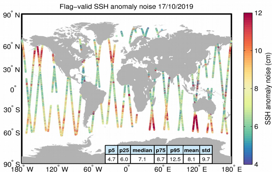
Figure 8. Geographical distribution of flag-valid 20-Hz SSH anomaly measurement noise over oceans and lakes for 17/10/2019. The statistical values shown in the table refer to the SSH anomaly noise and are calculated over all measurements shown in the figure.
