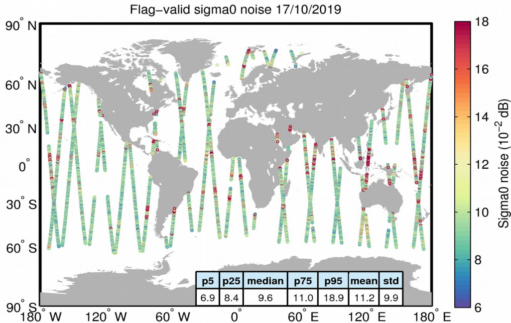
Figure 26. Geographical distribution of flag-valid 20-Hz sigma0 measurement noise over oceans and lakes for 17/10/2019. The statistical values shown in the table refer to the sigma0 noise and are calculated over all measurements shown in the figure.
