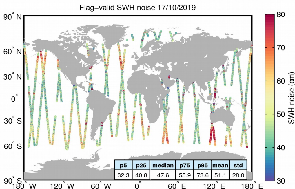
Figure 18. Geographical distribution of flag-valid 20-Hz SWH measurement noise over oceans and lakes for 17/10/2019. The statistical values shown in the figure refer to the SWH noise and are calculated over all measurements shown in the figure.
