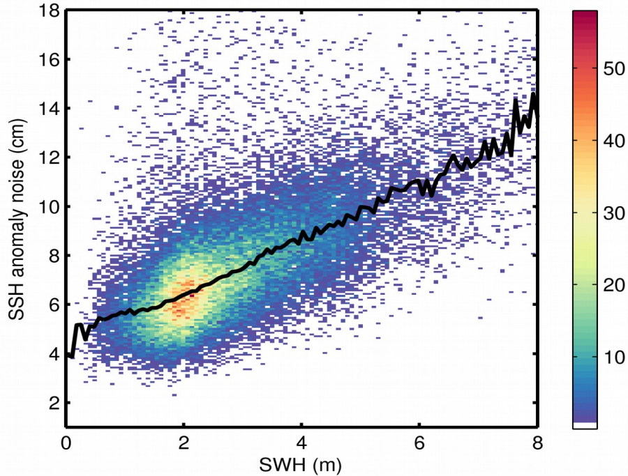
Figure 9. 2D histogram showing flag-valid SSH anomaly noise as a function of SWH for 17/10/2019. The black line denotes the median SSH anomaly noise as a function of SWH.
