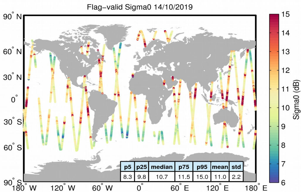
Figure 23. Geographical distribution of flag-valid sigma0 data over oceans and lakes for 14/10/2019. The statistical values shown in the table refer to the sigma0 in dB and are calculated over all measurements shown in the figure.
