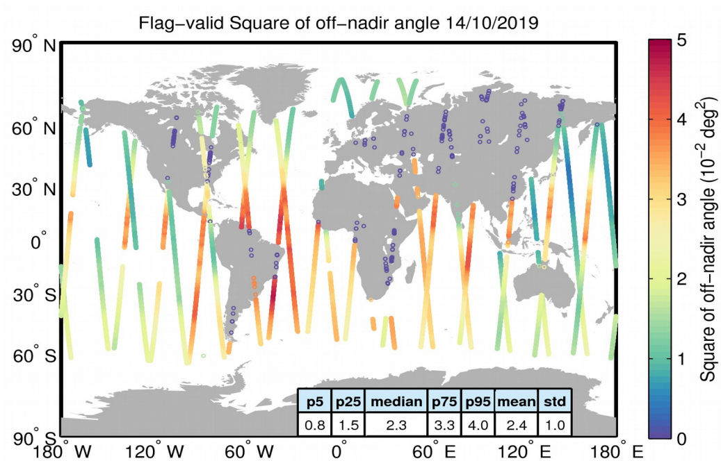
Figure 37. Geographical distribution of flag-valid mispointing data over oceans and lakes for 14/10/2019. The statistical values shown in the table refer to the mispointing in 10^{-2} deg 2 and are calculated over all measurements shown in the figure.
