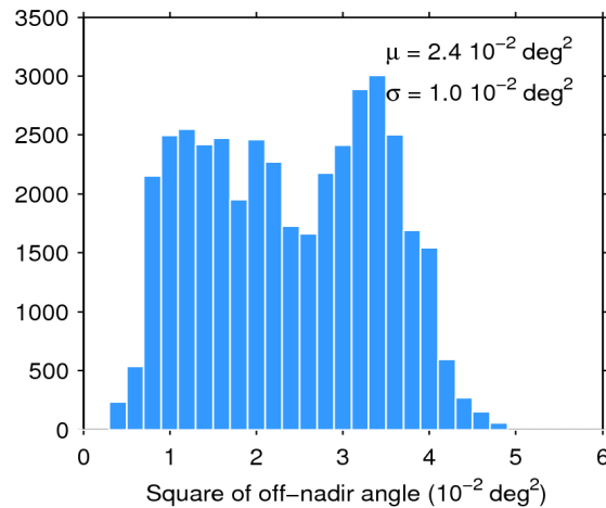
Figure 39. Histogram of flag-valid mispointing over oceans and lakes for 14/10/2019. The mean ( \mu ) and standard deviation ( \sigma ) are also shown. Note that values larger than 6 \cdot 10^{-2} \text{ deg}^2 are excluded from the histogram for the sake of readability but not from the computation of \mu and \sigma .
