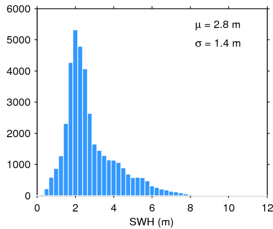
Figure 17. Histogram of flag-valid SWH over oceans and lakes for 14/10/2019. The mean ( \mu ) and standard deviation ( \sigma ) are also shown. Note that values larger than 12 m are excluded from the histogram for the sake of readability but not from the computation of \mu and \sigma .
