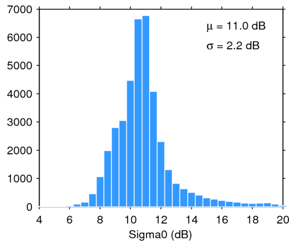
Figure 25. Histogram of flag-valid sigma0 over oceans and lakes for 14/10/2019. The mean ( \mu ) and standard deviation ( \sigma ) are also shown. Note that values outside [4 20] dB are excluded from the histogram for the sake of readability but not from the computation of \mu and \sigma .
