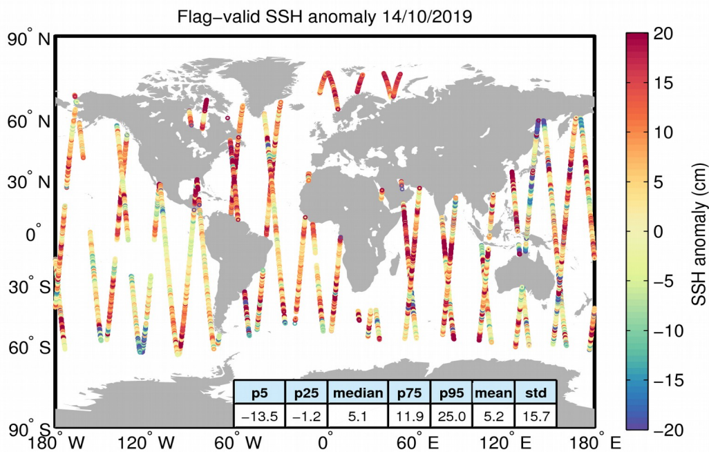
Figure 5. Geographical distribution of flag-valid 1-Hz SSH anomaly data over oceans and lakes for 14/10/2019. The statistical values shown in the table refer to the SSH anomaly in cm and are calculated over all measurements shown in the figure.
