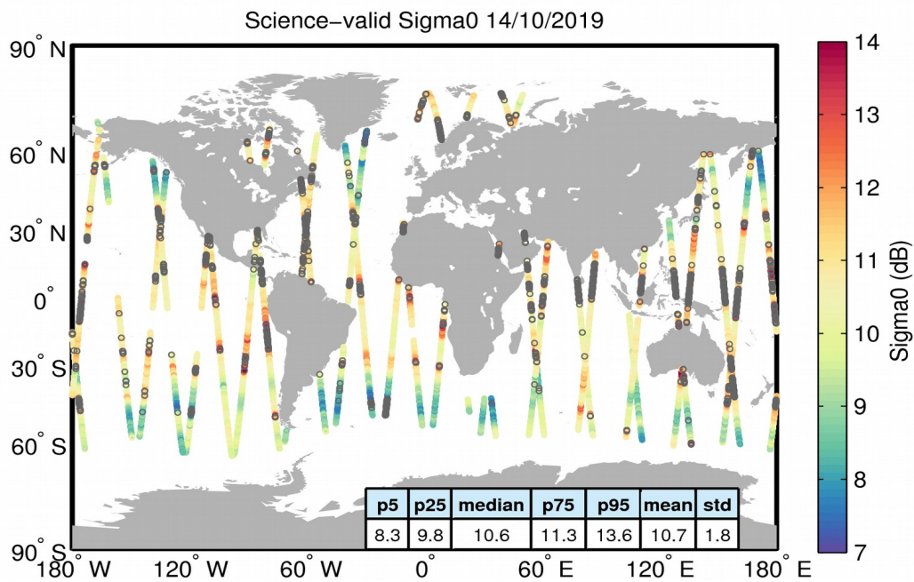
Figure 27. Geographical distribution of science-valid sigma0 data over oceans and lakes for 14/10/2019. The statistical values shown in the table refer to the sigma0 in dB and are calculated over all measurements shown in the figure. Gray circles denote records that have been rejected based on the editing criteria described in Table 4.
