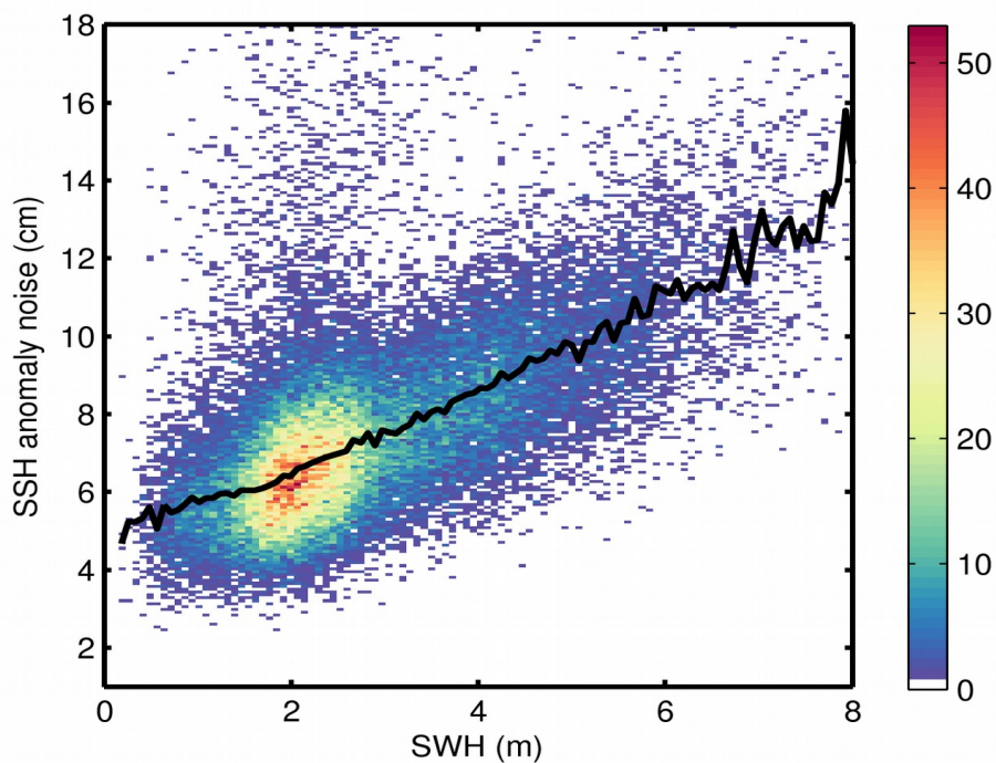
Figure 9. 2D histogram showing flag-valid SSH anomaly noise as a function of SWH for 14/10/2019. The black line denotes the median SSH anomaly noise as a function of SWH.
