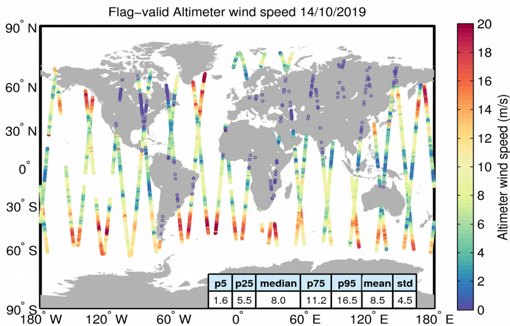
Figure 31. Geographical distribution of flag-valid wind data over oceans and lakes for 14/10/2019. The statistical values shown in the table refer to the wind in m/s and are calculated over all measurements shown in the figure.
