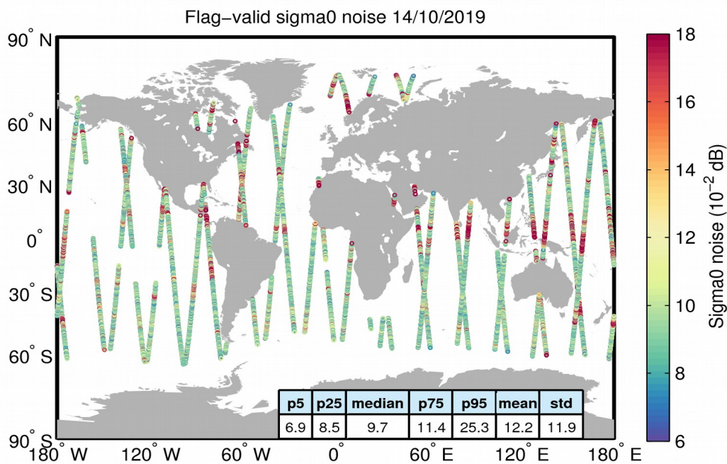
Figure 26. Geographical distribution of flag-valid 20-Hz sigma0 measurement noise over oceans and lakes for 14/10/2019. The statistical values shown in the table refer to the sigma0 noise and are calculated over all measurements shown in the figure.
