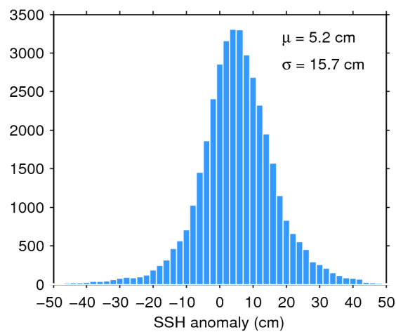
Figure 7. Histogram of flag-valid SSH anomaly over oceans and lakes for 14/10/2019. The mean ( \mu ) and standard deviation ( \sigma ) are also shown. Note that values outside [-50 \ 50] cm are excluded from the histogram for the sake of readability but not from the computation of \mu and \sigma .
