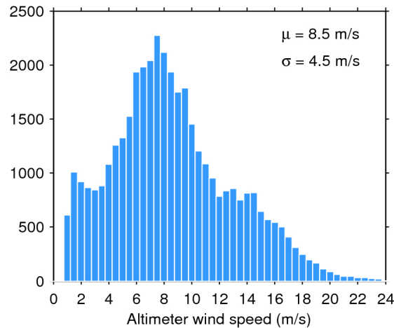
Figure 33. Histogram of flag-valid wind over oceans and lakes for 14/10/2019. The mean ( \mu ) and standard deviation ( \sigma ) are also shown. Note that values larger than 24 m/s are excluded from the histogram for the sake of readability but not from the computation of \mu and \sigma .
