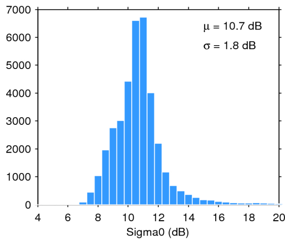
Figure 28. Histogram of science-valid sigma0 over oceans and lakes for 14/10/2019. The mean ( \mu ) and standard deviation ( \sigma ) are also shown. Note that values outside [4 20] dB are excluded from the histogram for the sake of readability but not from the computation of \mu and \sigma .
