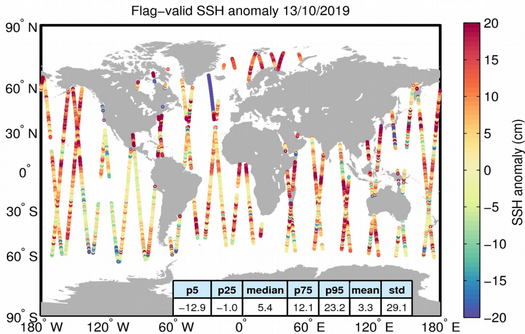
Figure 5. Geographical distribution of flag-valid 1-Hz SSH anomaly data over oceans and lakes for 13/10/2019. The statistical values shown in the table refer to the SSH anomaly in cm and are calculated over all measurements shown in the figure.
