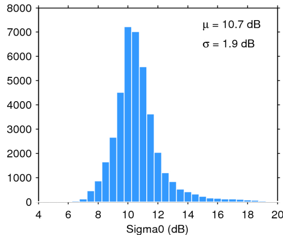
Figure 25. Histogram of flag-valid sigma0 over oceans and lakes for 13/10/2019. The mean ( \mu ) and standard deviation ( \sigma ) are also shown. Note that values outside [4 20] dB are excluded from the histogram for the sake of readability but not from the computation of \mu and \sigma .
