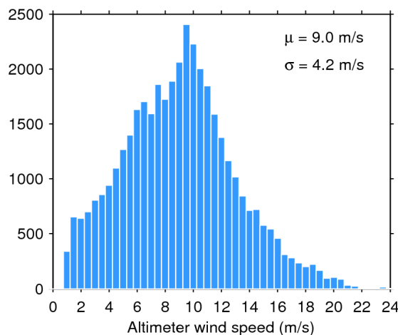
Figure 35. Histogram of science-valid wind over oceans and lakes for 13/10/2019. The mean ( \mu ) and standard deviation ( \sigma ) are also shown. Note that values larger than 24 m/s are excluded from the histogram for the sake of readability but not from the computation of \mu and \sigma .
