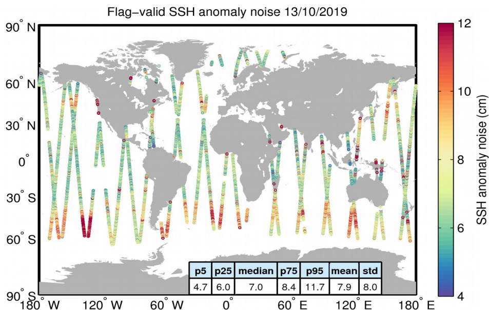
Figure 8. Geographical distribution of flag-valid 20-Hz SSH anomaly measurement noise over oceans and lakes for 13/10/2019. The statistical values shown in the table refer to the SSH anomaly noise and are calculated over all measurements shown in the figure.
