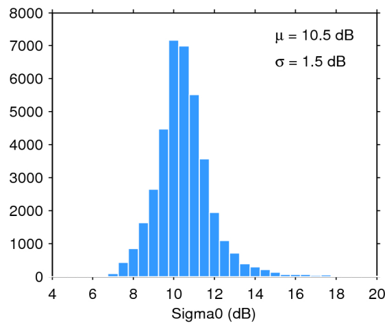
Figure 28. Histogram of science-valid sigma0 over oceans and lakes for 13/10/2019. The mean ( \mu ) and standard deviation ( \sigma ) are also shown. Note that values outside [4 20] dB are excluded from the histogram for the sake of readability but not from the computation of \mu and \sigma .
