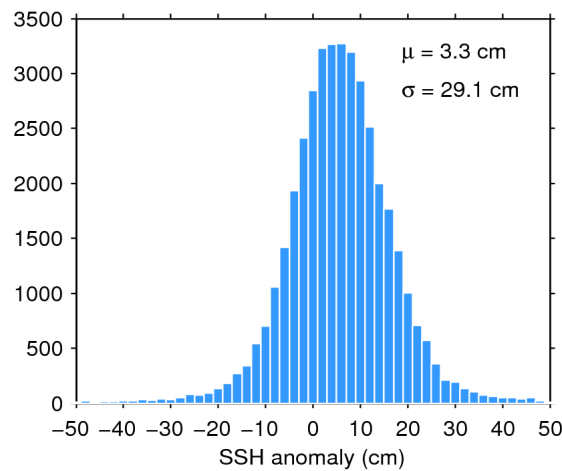
Figure 7. Histogram of flag-valid SSH anomaly over oceans and lakes for 13/10/2019. The mean ( \mu ) and standard deviation ( \sigma ) are also shown. Note that values outside [-50\ 50] cm are excluded from the histogram for the sake of readability but not from the computation of \mu and \sigma .
