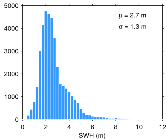
Figure 17. Histogram of flag-valid SWH over oceans and lakes for 13/10/2019. The mean ( \mu ) and standard deviation ( \sigma ) are also shown. Note that values larger than 12 m are excluded from the histogram for the sake of readability but not from the computation of \mu and \sigma .
