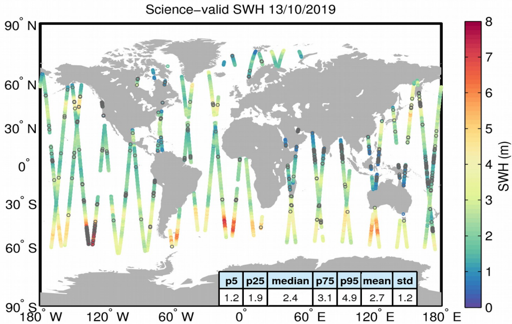
Figure 19. Geographical distribution of science-valid SWH data over oceans and lakes for 13/10/2019. The statistical values shown in the table refer to the SWH in m and are calculated over all measurements shown in the figure. Gray circles denote records that have been rejected based on the editing criteria described in Table 3.
