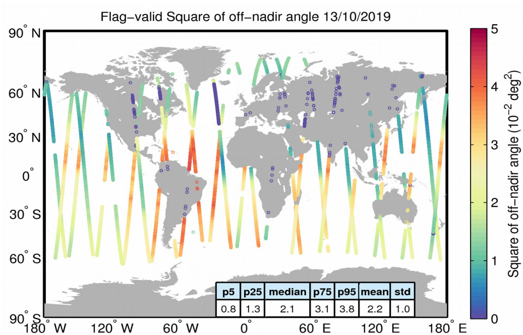
Figure 37. Geographical distribution of flag-valid mispointing data over oceans and lakes for 13/10/2019. The statistical values shown in the table refer to the mispointing in 10^{-2} \text{ deg}^2 and are calculated over all measurements shown in the figure.
