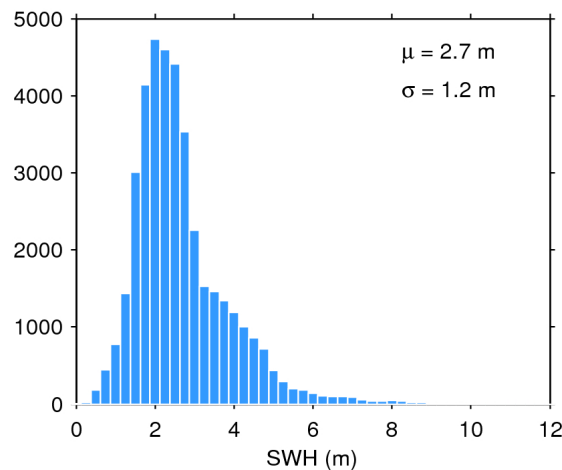
Figure 20. Histogram of science-valid SWH over oceans and lakes for 13/10/2019. The mean ( \mu ) and standard deviation ( \sigma ) are also shown. Note that values larger than 12 m are excluded from the histogram for the sake of readability but not from the computation of \mu and \sigma .
