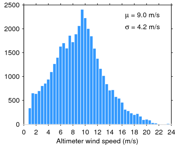
Figure 33. Histogram of flag-valid wind over oceans and lakes for 13/10/2019. The mean ( \mu ) and standard deviation ( \sigma ) are also shown. Note that values larger than 24 m/s are excluded from the histogram for the sake of readability but not from the computation of \mu and \sigma .
