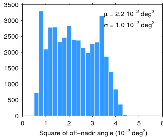
Figure 39. Histogram of flag-valid mispointing over oceans and lakes for 13/10/2019. The mean ( \mu ) and standard deviation ( \sigma ) are also shown. Note that values larger than 6 \cdot 10^{-2} \text{ deg}^2 are excluded from the histogram for the sake of readability but not from the computation of \mu and \sigma .
