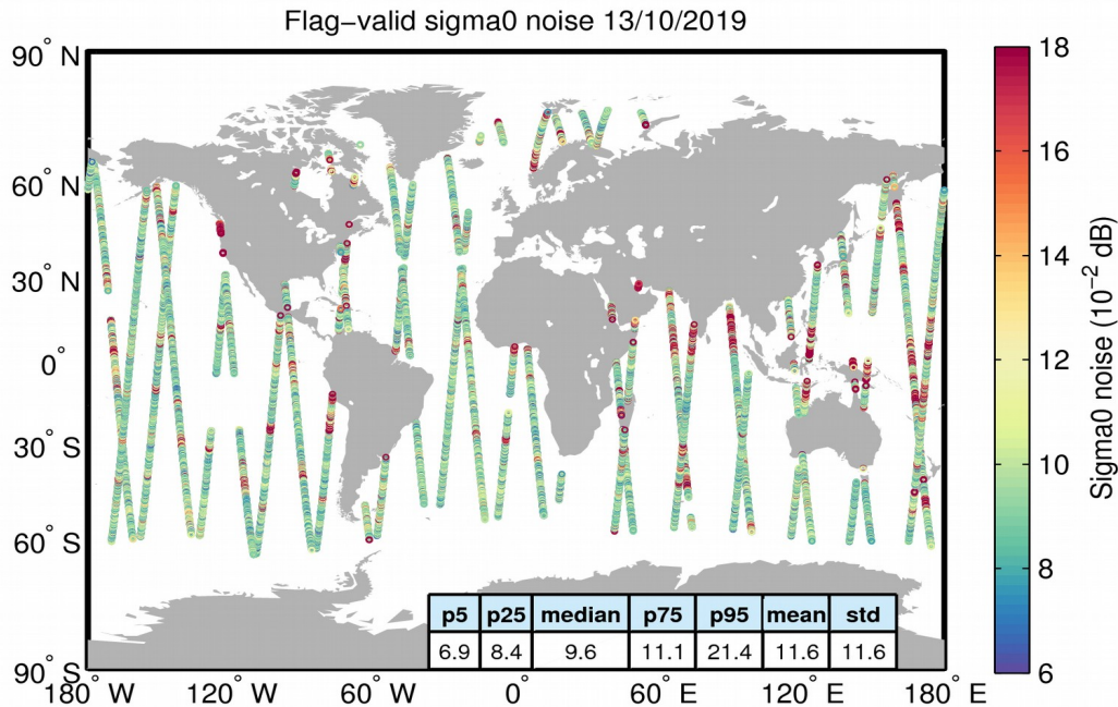
Figure 26. Geographical distribution of flag-valid 20-Hz sigma0 measurement noise over oceans and lakes for 13/10/2019. The statistical values shown in the table refer to the sigma0 noise and are calculated over all measurements shown in the figure.
