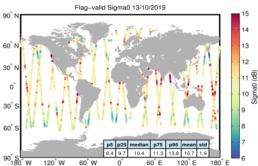
Figure 23. Geographical distribution of flag-valid sigma0 data over oceans and lakes for 13/10/2019. The statistical values shown in the table refer to the sigma0 in dB and are calculated over all measurements shown in the figure.
