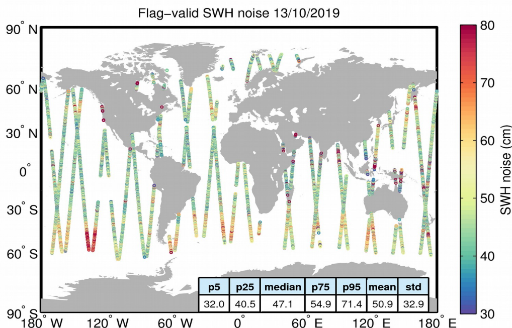
Figure 18. Geographical distribution of flag-valid 20-Hz SWH measurement noise over oceans and lakes for 13/10/2019. The statistical values shown in the figure refer to the SWH noise and are calculated over all measurements shown in the figure.
