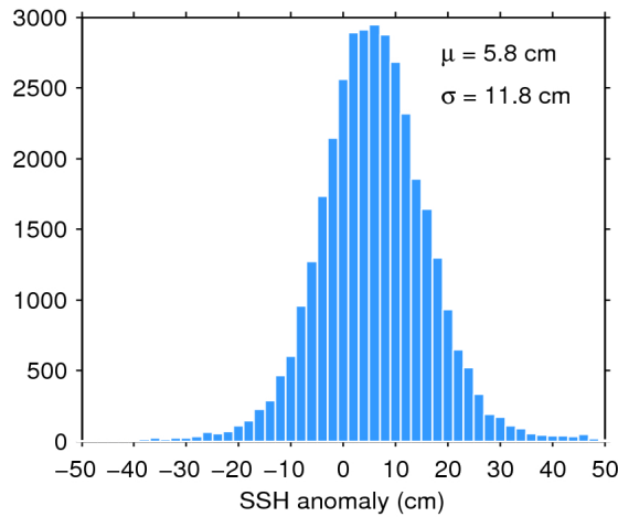
Figure 11. Histogram of science-valid SSH anomaly over oceans and lakes for 13/10/2019. The mean ( \mu ) and standard deviation ( \sigma ) are also shown. Note that values outside [-50 50] cm are excluded from the histogram for the sake of readability but not from the computation of \mu and \sigma .
