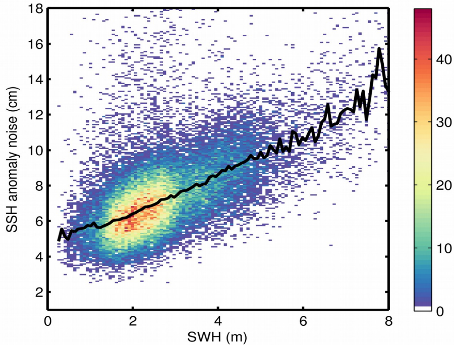
Figure 9. 2D histogram showing flag-valid SSH anomaly noise as a function of SWH for 13/10/2019. The black line denotes the median SSH anomaly noise as a function of SWH.
