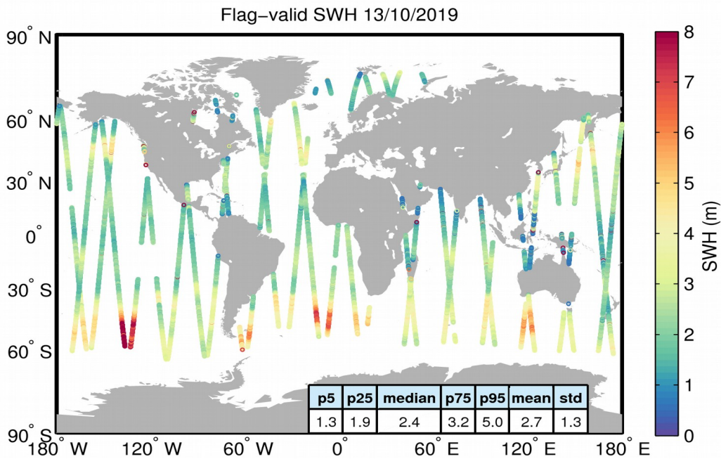
Figure 15. Geographical distribution of flag-valid SWH data over oceans and lakes for 13/10/2019. The statistical values shown in the table refer to the SWH in m and are calculated over all measurements shown in the figure.
