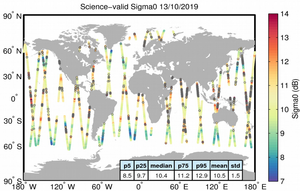
Figure 27. Geographical distribution of science-valid sigma0 data over oceans and lakes for 13/10/2019. The statistical values shown in the table refer to the sigma0 in dB and are calculated over all measurements shown in the figure. Gray circles denote records that have been rejected based on the editing criteria described in Table 4.
