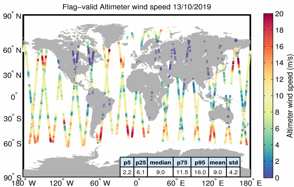
Figure 31. Geographical distribution of flag-valid wind data over oceans and lakes for 13/10/2019. The statistical values shown in the table refer to the wind in m/s and are calculated over all measurements shown in the figure.
