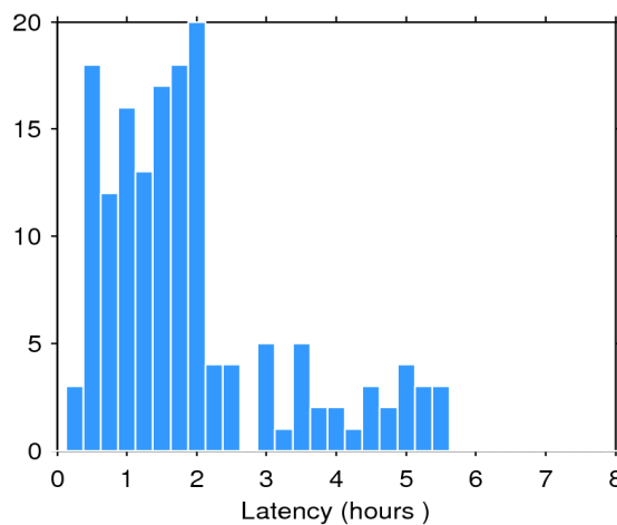
Figure 2. Histogram of the data latency for 13/10/2019. The y-axis denotes the number of files that are made available with a delay of x-hours with respect to the mean time of the records stored in the file.
