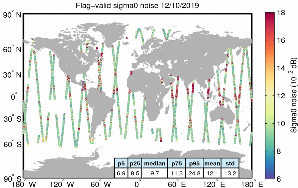
Figure 26. Geographical distribution of flag-valid 20-Hz sigma0 measurement noise over oceans and lakes for 12/10/2019. The statistical values shown in the table refer to the sigma0 noise and are calculated over all measurements shown in the figure.
