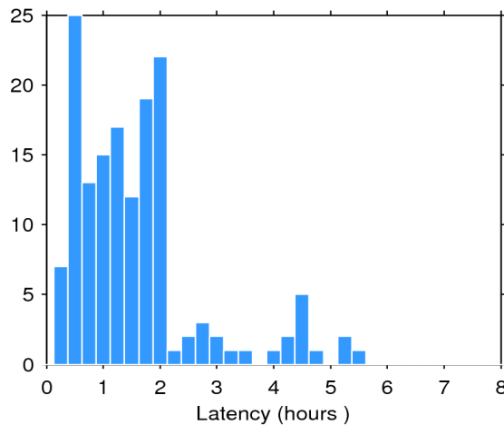
Figure 2. Histogram of the data latency for 12/10/2019. The y-axis denotes the number of files that are made available with a delay of x-hours with respect to the mean time of the records stored in the file.
