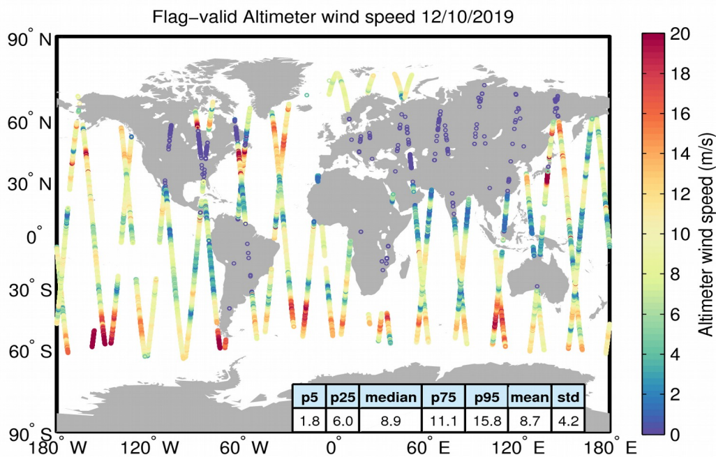
Figure 31. Geographical distribution of flag-valid wind data over oceans and lakes for 12/10/2019. The statistical values shown in the table refer to the wind in m/s and are calculated over all measurements shown in the figure.
