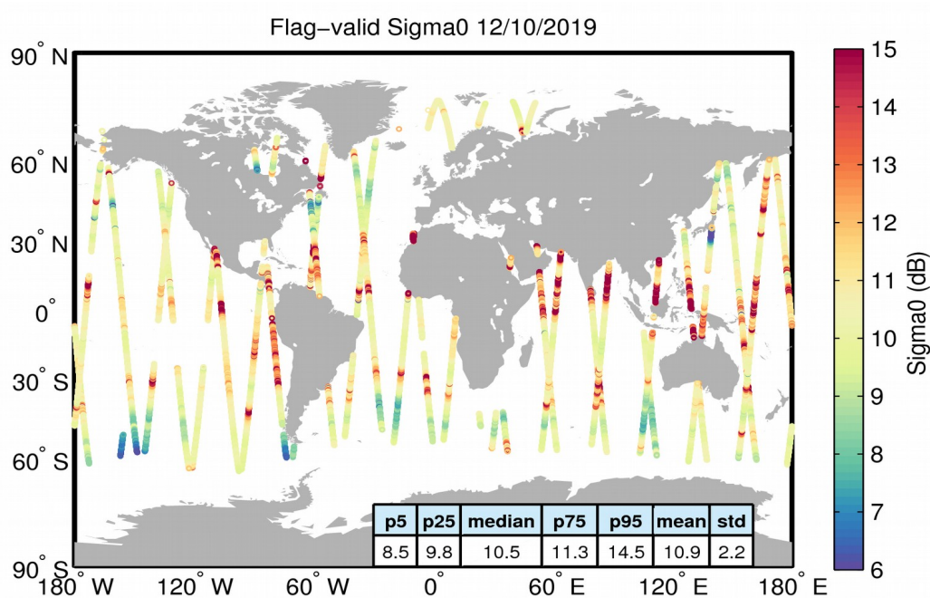
Figure 23. Geographical distribution of flag-valid sigma0 data over oceans and lakes for 12/10/2019. The statistical values shown in the table refer to the sigma0 in dB and are calculated over all measurements shown in the figure.
