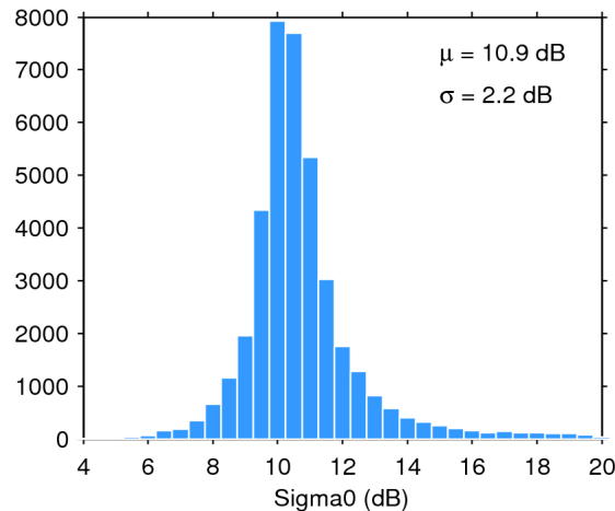
Figure 25. Histogram of flag-valid sigma0 over oceans and lakes for 12/10/2019. The mean ( \mu ) and standard deviation ( \sigma ) are also shown. Note that values outside [4 20] dB are excluded from the histogram for the sake of readability but not from the computation of \mu and \sigma .
