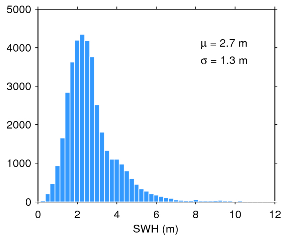
Figure 20. Histogram of science-valid SWH over oceans and lakes for 12/10/2019. The mean ( \mu ) and standard deviation ( \sigma ) are also shown. Note that values larger than 12 m are excluded from the histogram for the sake of readability but not from the computation of \mu and \sigma .
