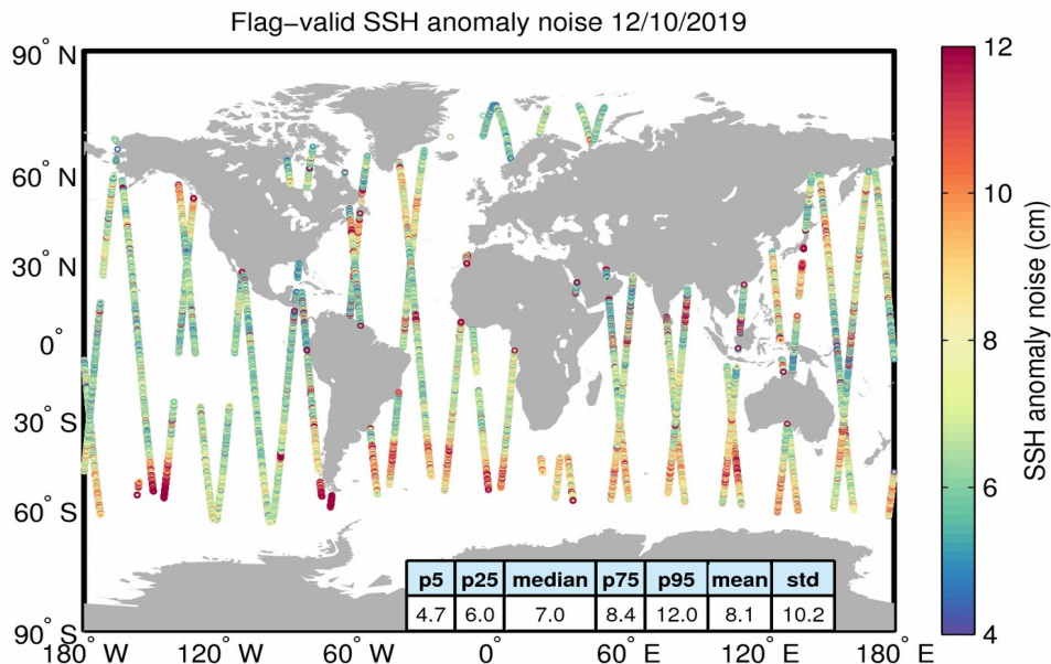
Figure 8. Geographical distribution of flag-valid 20-Hz SSH anomaly measurement noise over oceans and lakes for 12/10/2019. The statistical values shown in the table refer to the SSH anomaly noise and are calculated over all measurements shown in the figure.
