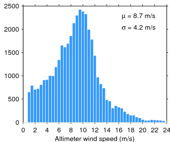
Figure 35. Histogram of science-valid wind over oceans and lakes for 12/10/2019. The mean ( \mu ) and standard deviation ( \sigma ) are also shown. Note that values larger than 24 m/s are excluded from the histogram for the sake of readability but not from the computation of \mu and \sigma .
