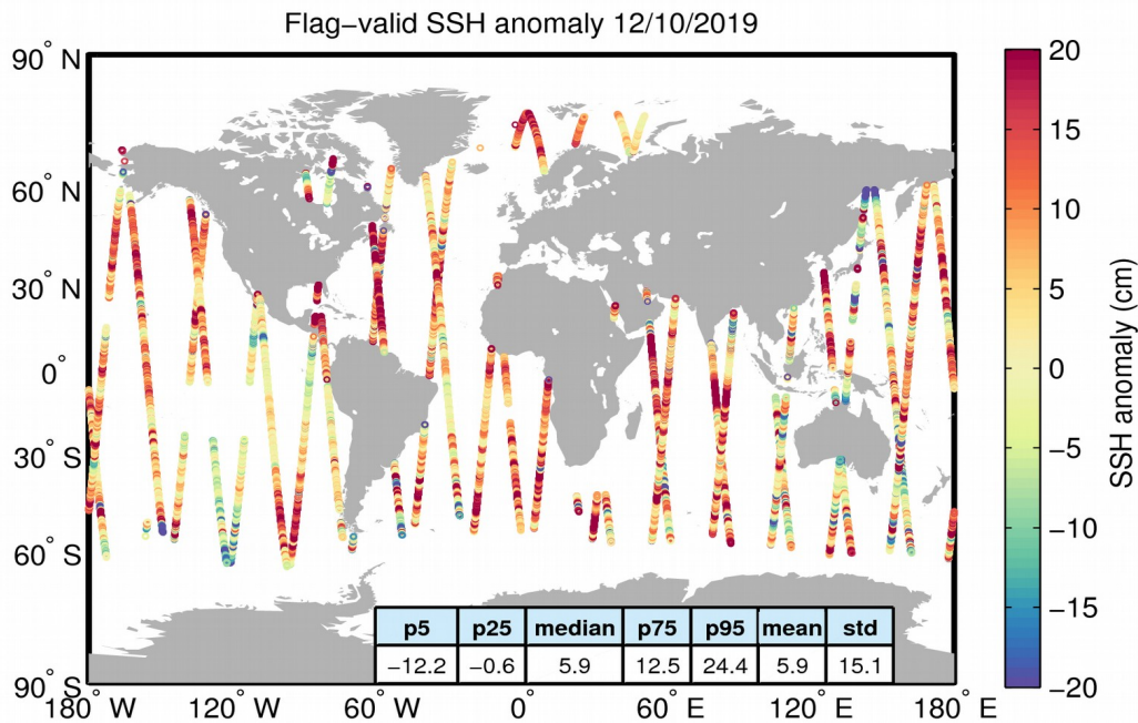
Figure 5. Geographical distribution of flag-valid 1-Hz SSH anomaly data over oceans and lakes for 12/10/2019. The statistical values shown in the table refer to the SSH anomaly in cm and are calculated over all measurements shown in the figure.
