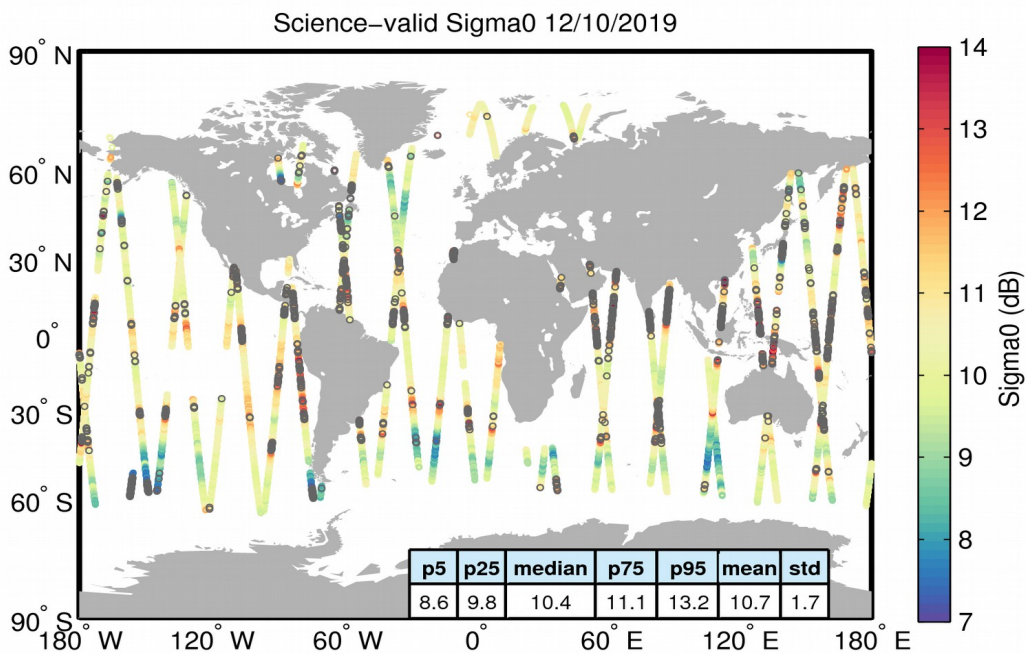
Figure 27. Geographical distribution of science-valid sigma0 data over oceans and lakes for 12/10/2019. The statistical values shown in the table refer to the sigma0 in dB and are calculated over all measurements shown in the figure. Gray circles denote records that have been rejected based on the editing criteria described in Table 4.
