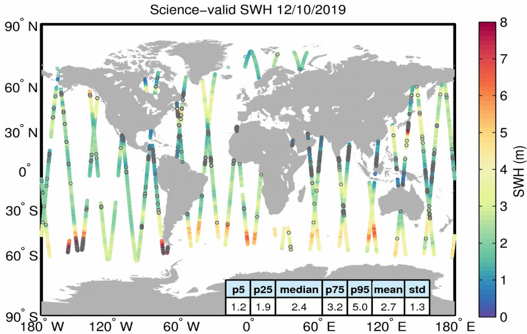
Figure 19. Geographical distribution of science-valid SWH data over oceans and lakes for 12/10/2019. The statistical values shown in the table refer to the SWH in m and are calculated over all measurements shown in the figure. Gray circles denote records that have been rejected based on the editing criteria described in Table 3.
