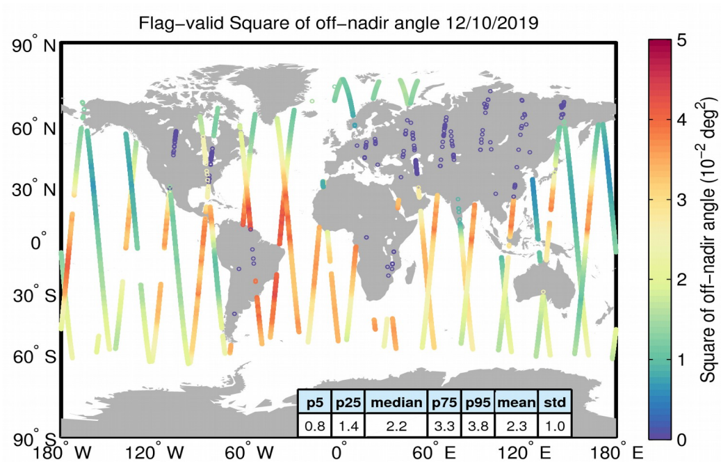
Figure 37. Geographical distribution of flag-valid mispointing data over oceans and lakes for 12/10/2019. The statistical values shown in the table refer to the mispointing in 10^{-2} \text{ deg}^2 and are calculated over all measurements shown in the figure.
