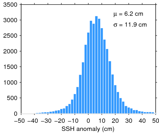
Figure 11. Histogram of science-valid SSH anomaly over oceans and lakes for 12/10/2019. The mean ( \mu ) and standard deviation ( \sigma ) are also shown. Note that values outside [-50 50] cm are excluded from the histogram for the sake of readability but not from the computation of \mu and \sigma .
