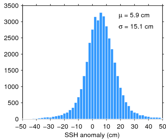
Figure 7. Histogram of flag-valid SSH anomaly over oceans and lakes for 12/10/2019. The mean ( \mu ) and standard deviation ( \sigma ) are also shown. Note that values outside [-50\ 50] cm are excluded from the histogram for the sake of readability but not from the computation of \mu and \sigma .
