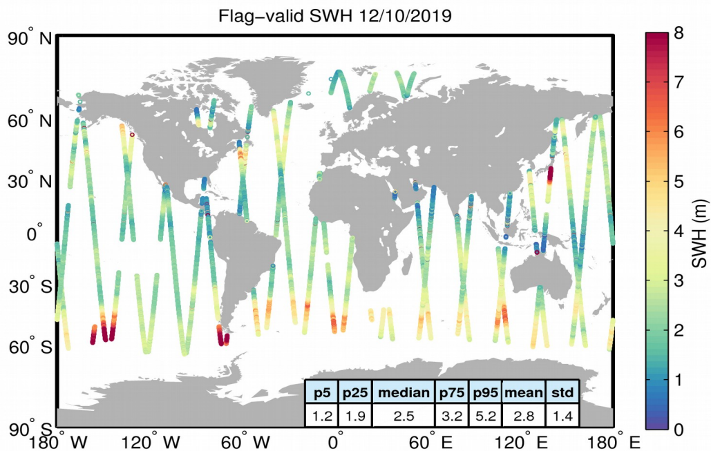
Figure 15. Geographical distribution of flag-valid SWH data over oceans and lakes for 12/10/2019. The statistical values shown in the table refer to the SWH in m and are calculated over all measurements shown in the figure.
