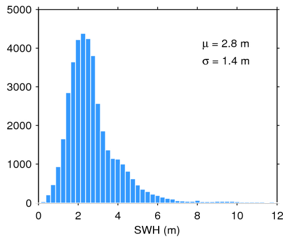
Figure 17. Histogram of flag-valid SWH over oceans and lakes for 12/10/2019. The mean ( \mu ) and standard deviation ( \sigma ) are also shown. Note that values larger than 12 m are excluded from the histogram for the sake of readability but not from the computation of \mu and \sigma .
