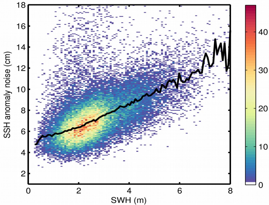
Figure 9. 2D histogram showing flag-valid SSH anomaly noise as a function of SWH for 12/10/2019. The black line denotes the median SSH anomaly noise as a function of SWH.
