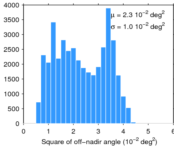
Figure 39. Histogram of flag-valid mispointing over oceans and lakes for 12/10/2019. The mean ( \mu ) and standard deviation ( \sigma ) are also shown. Note that values larger than 6 \cdot 10^{-2} \text{ deg}^2 are excluded from the histogram for the sake of readability but not from the computation of \mu and \sigma .
