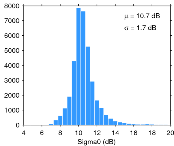
Figure 28. Histogram of science-valid sigma0 over oceans and lakes for 12/10/2019. The mean ( \mu ) and standard deviation ( \sigma ) are also shown. Note that values outside [4 20] dB are excluded from the histogram for the sake of readability but not from the computation of \mu and \sigma .
