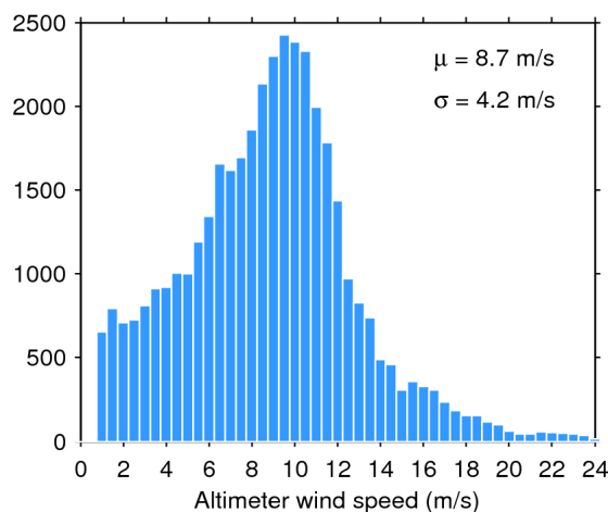
Figure 33. Histogram of flag-valid wind over oceans and lakes for 12/10/2019. The mean ( \mu ) and standard deviation ( \sigma ) are also shown. Note that values larger than 24 m/s are excluded from the histogram for the sake of readability but not from the computation of \mu and \sigma .
