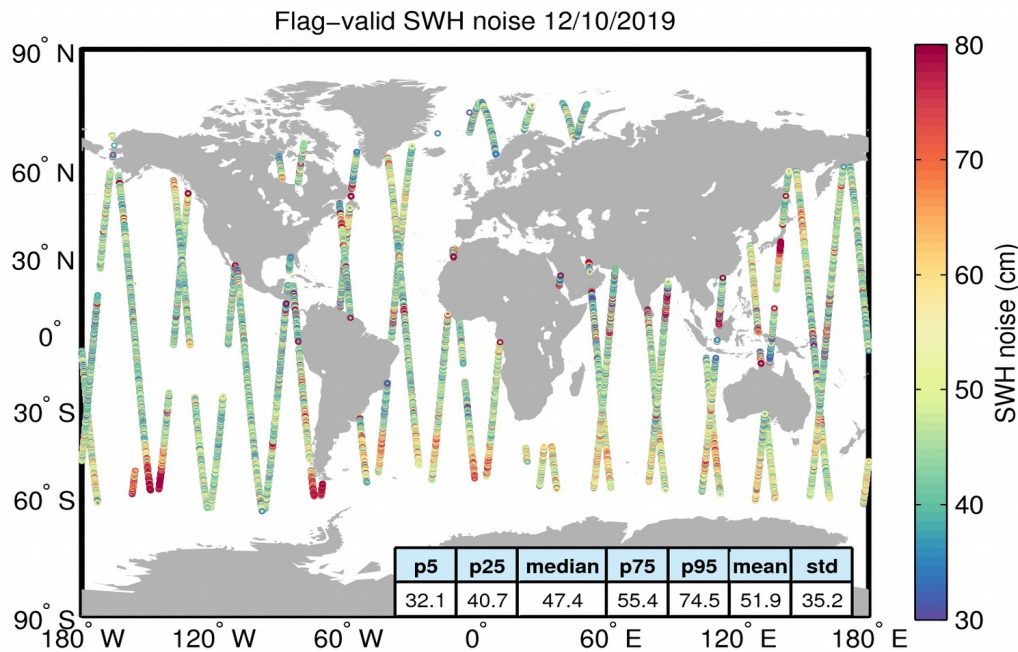
Figure 18. Geographical distribution of flag-valid 20-Hz SWH measurement noise over oceans and lakes for 12/10/2019. The statistical values shown in the figure refer to the SWH noise and are calculated over all measurements shown in the figure.
