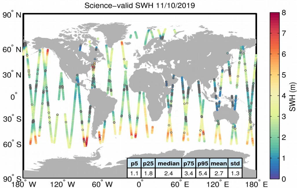
Figure 19. Geographical distribution of science-valid SWH data over oceans and lakes for 11/10/2019. The statistical values shown in the table refer to the SWH in m and are calculated over all measurements shown in the figure. Gray circles denote records that have been rejected based on the editing criteria described in Table 3.
