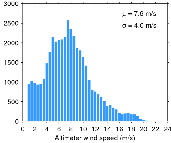
Figure 33. Histogram of flag-valid wind over oceans and lakes for 11/10/2019. The mean ( \mu ) and standard deviation ( \sigma ) are also shown. Note that values larger than 24 m/s are excluded from the histogram for the sake of readability but not from the computation of \mu and \sigma .
