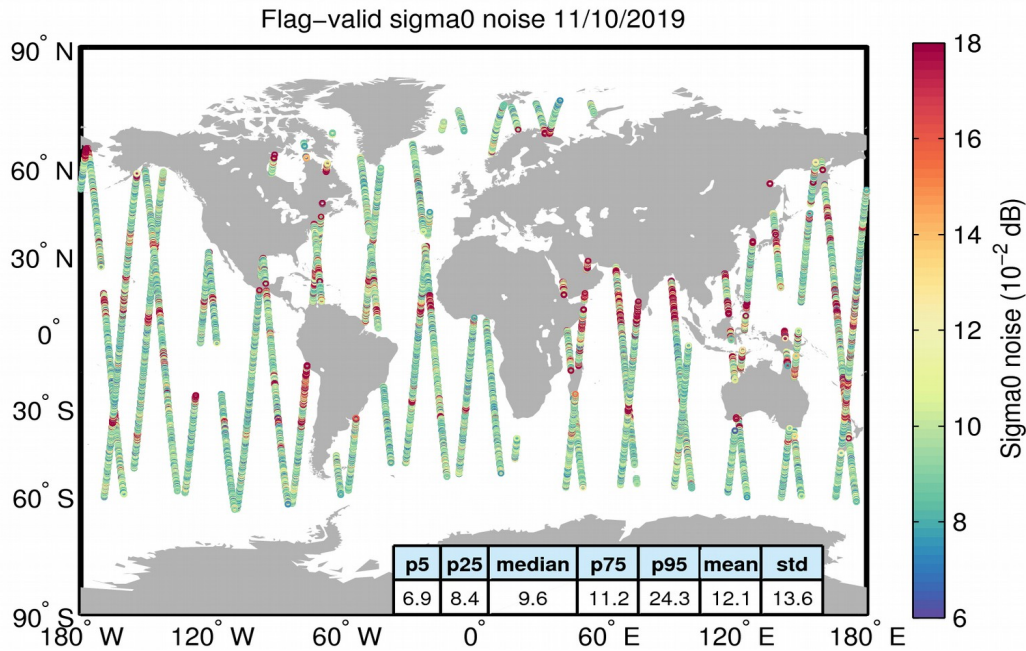
Figure 26. Geographical distribution of flag-valid 20-Hz sigma0 measurement noise over oceans and lakes for 11/10/2019. The statistical values shown in the table refer to the sigma0 noise and are calculated over all measurements shown in the figure.
