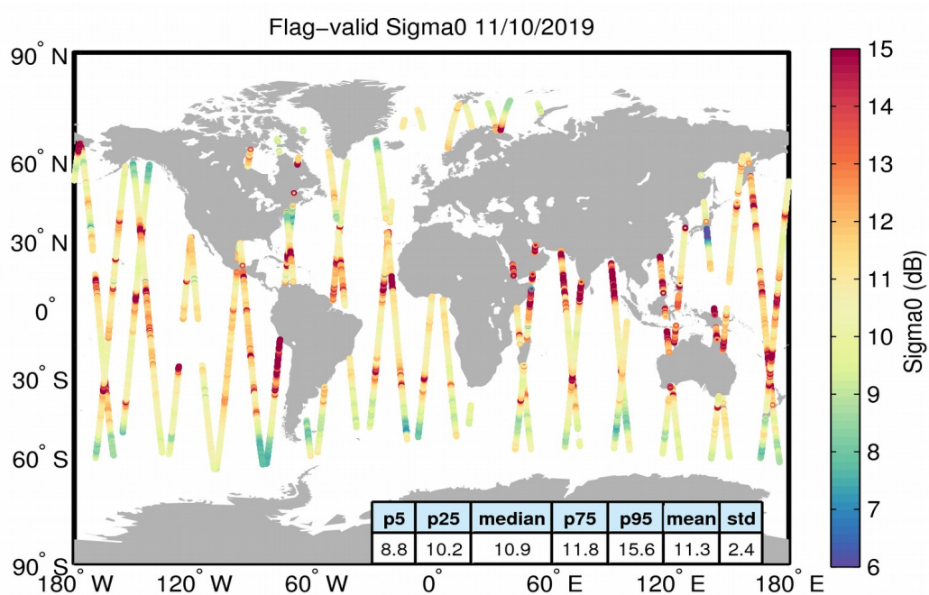
Figure 23. Geographical distribution of flag-valid sigma0 data over oceans and lakes for 11/10/2019. The statistical values shown in the table refer to the sigma0 in dB and are calculated over all measurements shown in the figure.
