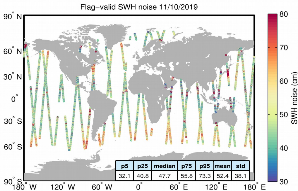
Figure 18. Geographical distribution of flag-valid 20-Hz SWH measurement noise over oceans and lakes for 11/10/2019. The statistical values shown in the figure refer to the SWH noise and are calculated over all measurements shown in the figure.
