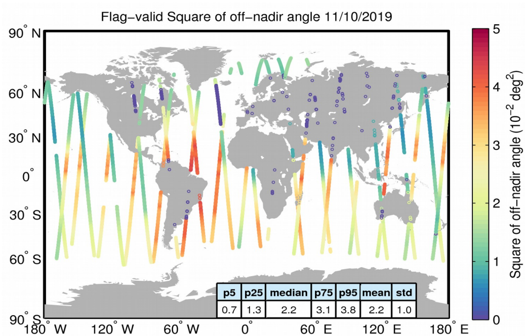
Figure 37. Geographical distribution of flag-valid mispointing data over oceans and lakes for 11/10/2019. The statistical values shown in the table refer to the mispointing in 10^{-2} \text{ deg}^2 and are calculated over all measurements shown in the figure.
