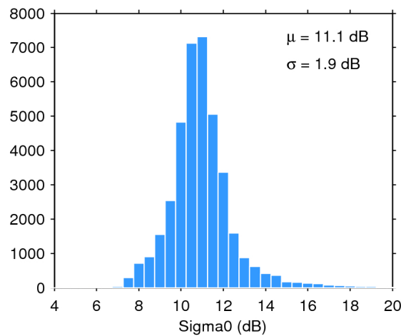
Figure 28. Histogram of science-valid sigma0 over oceans and lakes for 11/10/2019. The mean ( \mu ) and standard deviation ( \sigma ) are also shown. Note that values outside [4 20] dB are excluded from the histogram for the sake of readability but not from the computation of \mu and \sigma .
