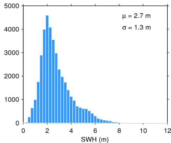
Figure 20. Histogram of science-valid SWH over oceans and lakes for 11/10/2019. The mean ( \mu ) and standard deviation ( \sigma ) are also shown. Note that values larger than 12 m are excluded from the histogram for the sake of readability but not from the computation of \mu and \sigma .
