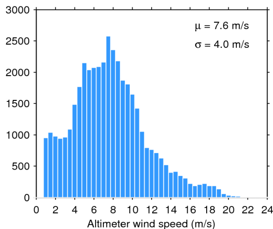
Figure 35. Histogram of science-valid wind over oceans and lakes for 11/10/2019. The mean ( \mu ) and standard deviation ( \sigma ) are also shown. Note that values larger than 24 m/s are excluded from the histogram for the sake of readability but not from the computation of \mu and \sigma .
