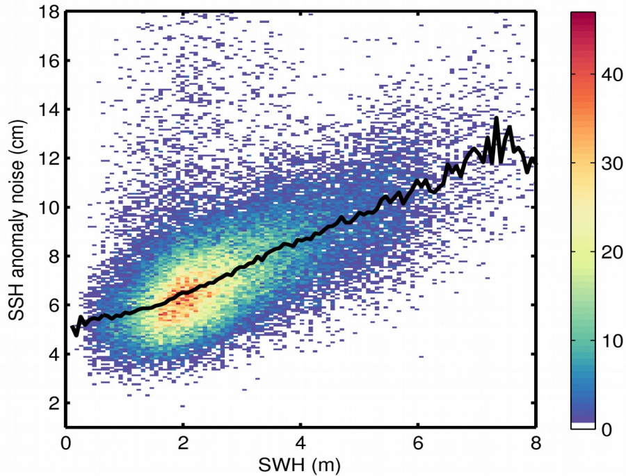
Figure 9. 2D histogram showing flag-valid SSH anomaly noise as a function of SWH for 11/10/2019. The black line denotes the median SSH anomaly noise as a function of SWH.
