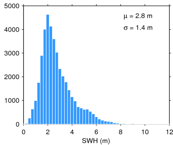
Figure 17. Histogram of flag-valid SWH over oceans and lakes for 11/10/2019. The mean ( \mu ) and standard deviation ( \sigma ) are also shown. Note that values larger than 12 m are excluded from the histogram for the sake of readability but not from the computation of \mu and \sigma .
