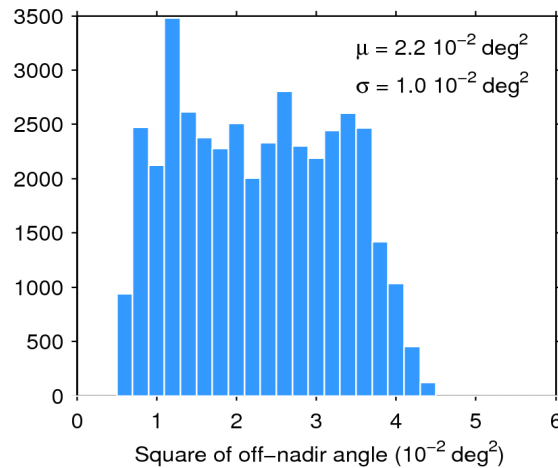
Figure 39. Histogram of flag-valid mispointing over oceans and lakes for 11/10/2019. The mean ( \mu ) and standard deviation ( \sigma ) are also shown. Note that values larger than 6 \cdot 10^{-2} \text{ deg}^2 are excluded from the histogram for the sake of readability but not from the computation of \mu and \sigma .
