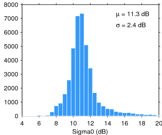
Figure 25. Histogram of flag-valid sigma0 over oceans and lakes for 11/10/2019. The mean ( \mu ) and standard deviation ( \sigma ) are also shown. Note that values outside [4 20] dB are excluded from the histogram for the sake of readability but not from the computation of \mu and \sigma .
