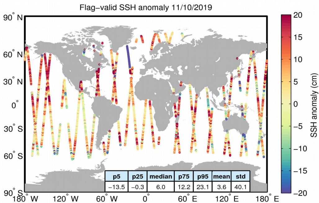
Figure 5. Geographical distribution of flag-valid 1-Hz SSH anomaly data over oceans and lakes for 11/10/2019. The statistical values shown in the table refer to the SSH anomaly in cm and are calculated over all measurements shown in the figure.
