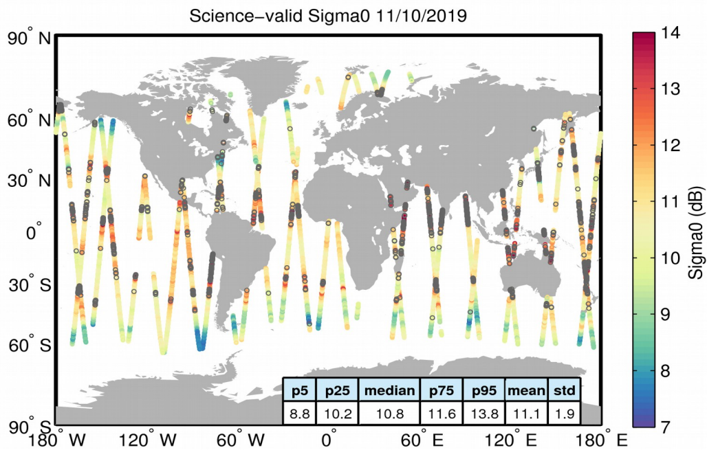
Figure 27. Geographical distribution of science-valid sigma0 data over oceans and lakes for 11/10/2019. The statistical values shown in the table refer to the sigma0 in dB and are calculated over all measurements shown in the figure. Gray circles denote records that have been rejected based on the editing criteria described in Table 4.
