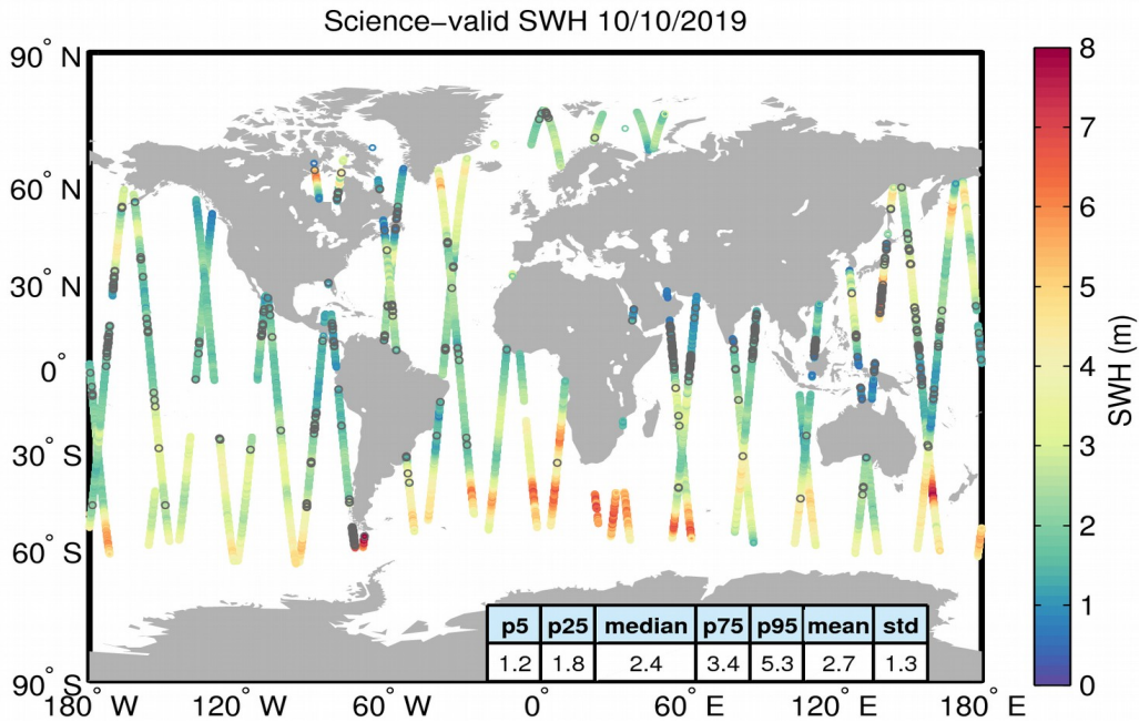
Figure 19. Geographical distribution of science-valid SWH data over oceans and lakes for 10/10/2019. The statistical values shown in the table refer to the SWH in m and are calculated over all measurements shown in the figure. Gray circles denote records that have been rejected based on the editing criteria described in Table 3.
