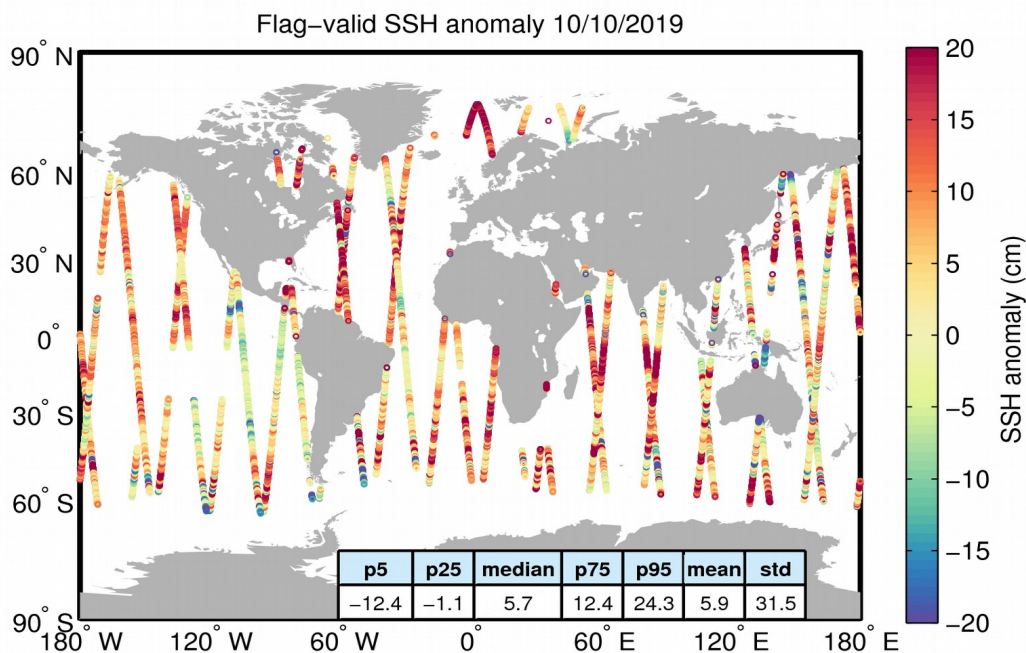
Figure 5. Geographical distribution of flag-valid 1-Hz SSH anomaly data over oceans and lakes for 10/10/2019. The statistical values shown in the table refer to the SSH anomaly in cm and are calculated over all measurements shown in the figure.
