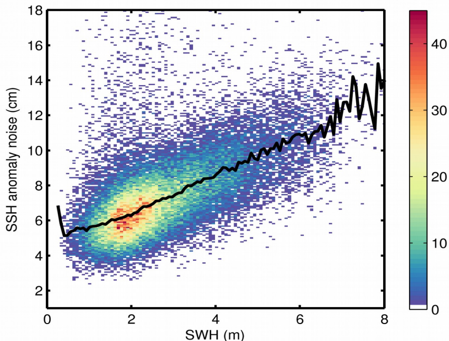
Figure 9. 2D histogram showing flag-valid SSH anomaly noise as a function of SWH for 10/10/2019. The black line denotes the median SSH anomaly noise as a function of SWH.
