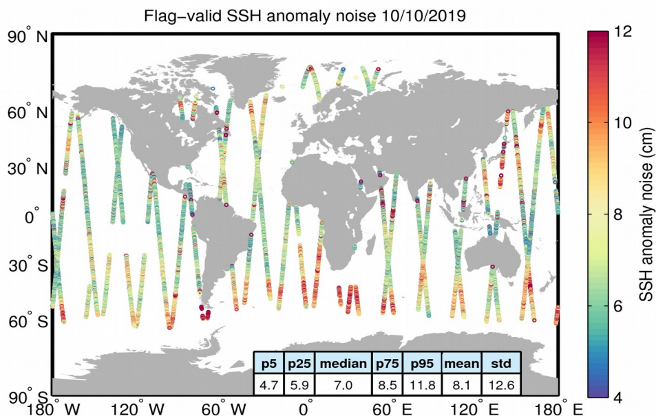
Figure 8. Geographical distribution of flag-valid 20-Hz SSH anomaly measurement noise over oceans and lakes for 10/10/2019. The statistical values shown in the table refer to the SSH anomaly noise and are calculated over all measurements shown in the figure.
