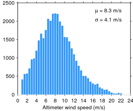
Figure 33. Histogram of flag-valid wind over oceans and lakes for 10/10/2019. The mean ( \mu ) and standard deviation ( \sigma ) are also shown. Note that values larger than 24 m/s are excluded from the histogram for the sake of readability but not from the computation of \mu and \sigma .
