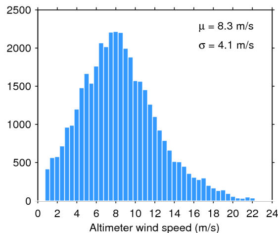
Figure 35. Histogram of science-valid wind over oceans and lakes for 10/10/2019. The mean ( \mu ) and standard deviation ( \sigma ) are also shown. Note that values larger than 24 m/s are excluded from the histogram for the sake of readability but not from the computation of \mu and \sigma .
