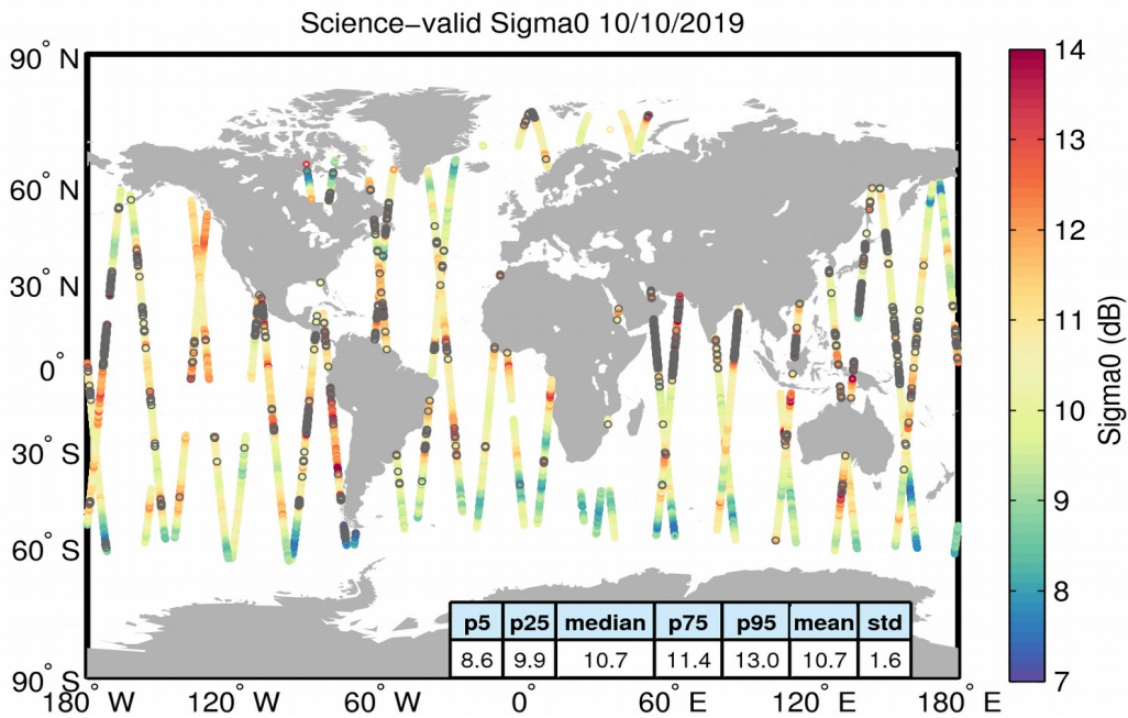
Figure 27. Geographical distribution of science-valid sigma0 data over oceans and lakes for 10/10/2019. The statistical values shown in the table refer to the sigma0 in dB and are calculated over all measurements shown in the figure. Gray circles denote records that have been rejected based on the editing criteria described in Table 4.
