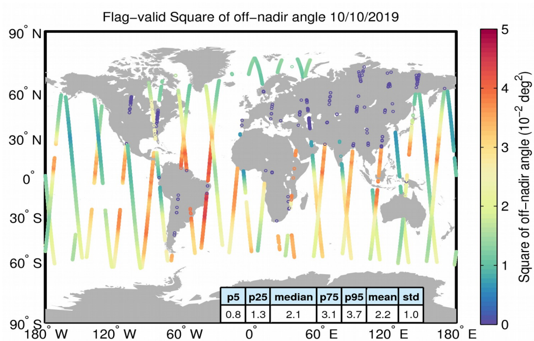
Figure 37. Geographical distribution of flag-valid mispointing data over oceans and lakes for 10/10/2019. The statistical values shown in the table refer to the mispointing in 10^{-2} deg 2 and are calculated over all measurements shown in the figure.
