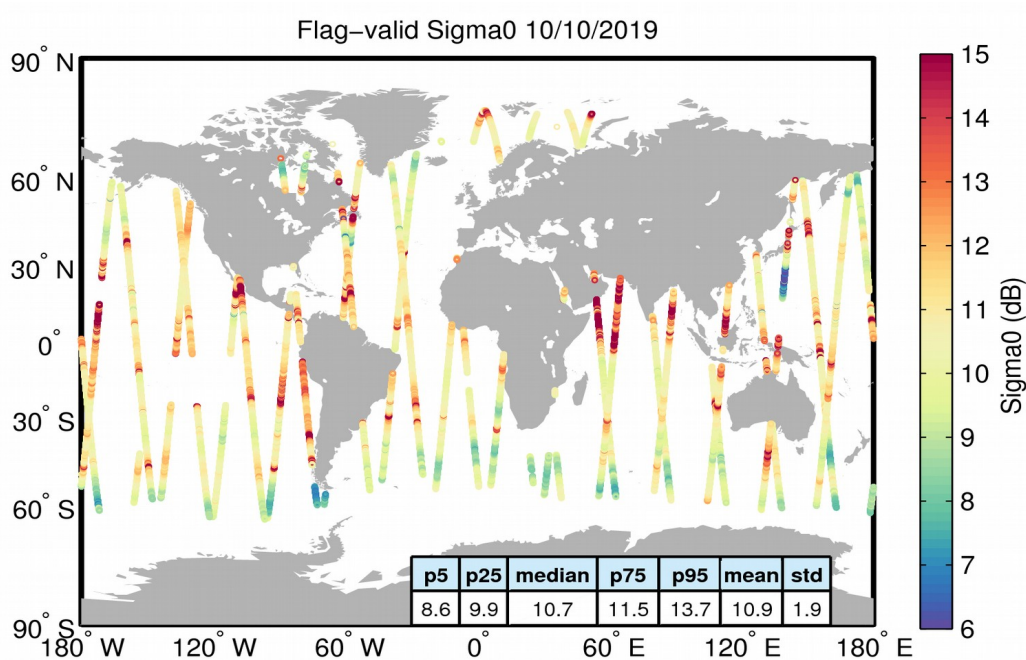
Figure 23. Geographical distribution of flag-valid sigma0 data over oceans and lakes for 10/10/2019. The statistical values shown in the table refer to the sigma0 in dB and are calculated over all measurements shown in the figure.
