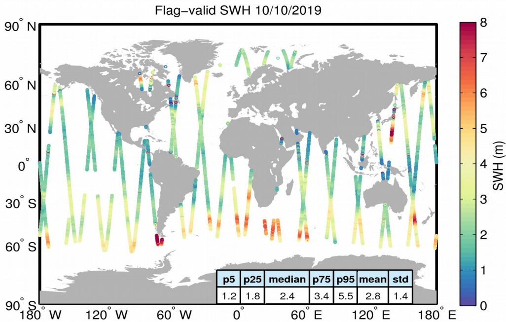
Figure 15. Geographical distribution of flag-valid SWH data over oceans and lakes for 10/10/2019. The statistical values shown in the table refer to the SWH in m and are calculated over all measurements shown in the figure.
