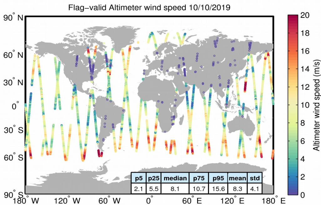
Figure 31. Geographical distribution of flag-valid wind data over oceans and lakes for 10/10/2019. The statistical values shown in the table refer to the wind in m/s and are calculated over all measurements shown in the figure.
