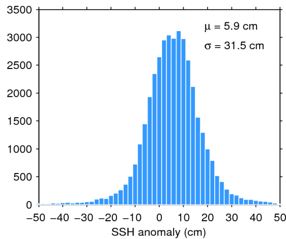
Figure 7. Histogram of flag-valid SSH anomaly over oceans and lakes for 10/10/2019. The mean ( \mu ) and standard deviation ( \sigma ) are also shown. Note that values outside [-50\ 50] cm are excluded from the histogram for the sake of readability but not from the computation of \mu and \sigma .
