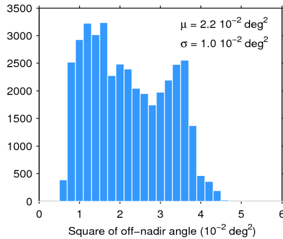
Figure 39. Histogram of flag-valid mispointing over oceans and lakes for 10/10/2019. The mean ( \mu ) and standard deviation ( \sigma ) are also shown. Note that values larger than 6 \cdot 10^{-2} \text{ deg}^2 are excluded from the histogram for the sake of readability but not from the computation of \mu and \sigma .
