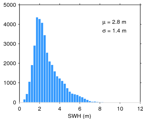
Figure 17. Histogram of flag-valid SWH over oceans and lakes for 10/10/2019. The mean ( \mu ) and standard deviation ( \sigma ) are also shown. Note that values larger than 12 m are excluded from the histogram for the sake of readability but not from the computation of \mu and \sigma .
