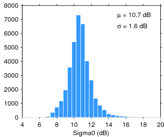
Figure 28. Histogram of science-valid sigma0 over oceans and lakes for 10/10/2019. The mean ( \mu ) and standard deviation ( \sigma ) are also shown. Note that values outside [4 20] dB are excluded from the histogram for the sake of readability but not from the computation of \mu and \sigma .
