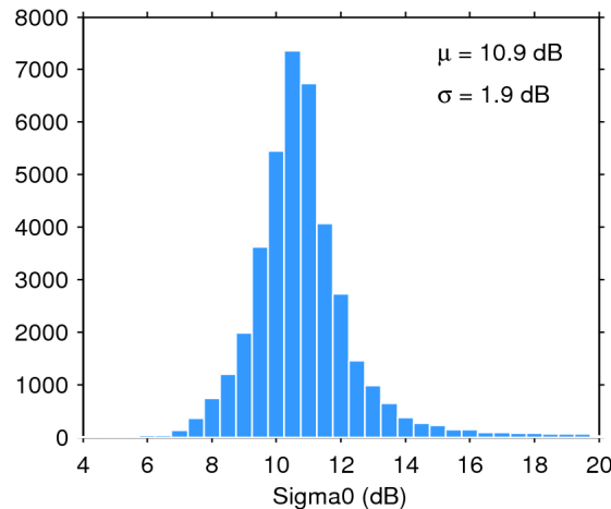
Figure 25. Histogram of flag-valid sigma0 over oceans and lakes for 10/10/2019. The mean ( \mu ) and standard deviation ( \sigma ) are also shown. Note that values outside [4 20] dB are excluded from the histogram for the sake of readability but not from the computation of \mu and \sigma .
