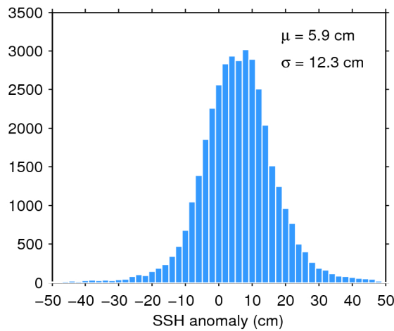
Figure 11. Histogram of science-valid SSH anomaly over oceans and lakes for 10/10/2019. The mean ( \mu ) and standard deviation ( \sigma ) are also shown. Note that values outside [-50 50] cm are excluded from the histogram for the sake of readability but not from the computation of \mu and \sigma .
