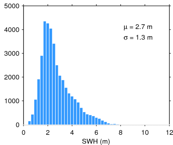
Figure 20. Histogram of science-valid SWH over oceans and lakes for 10/10/2019. The mean ( \mu ) and standard deviation ( \sigma ) are also shown. Note that values larger than 12 m are excluded from the histogram for the sake of readability but not from the computation of \mu and \sigma .
