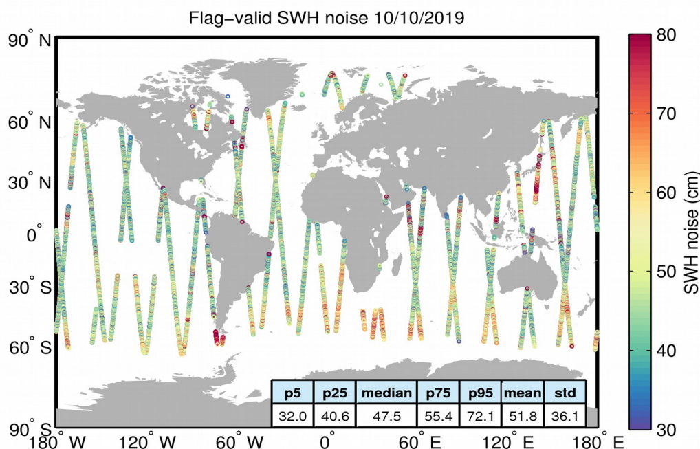
Figure 18. Geographical distribution of flag-valid 20-Hz SWH measurement noise over oceans and lakes for 10/10/2019. The statistical values shown in the table refer to the SWH noise and are calculated over all measurements shown in the figure.
