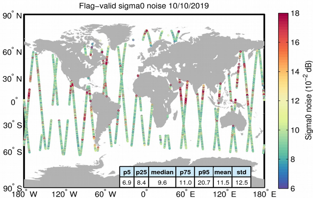
Figure 26. Geographical distribution of flag-valid 20-Hz sigma0 measurement noise over oceans and lakes for 10/10/2019. The statistical values shown in the table refer to the sigma0 noise and are calculated over all measurements shown in the figure.
