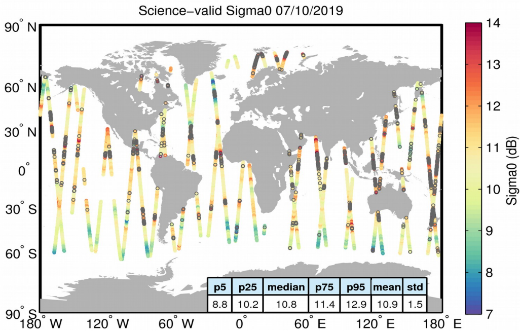
Figure 27. Geographical distribution of science-valid sigma0 data over oceans and lakes for 07/10/2019. The statistical values shown in the table refer to the sigma0 in dB and are calculated over all measurements shown in the figure. Gray circles denote records that have been rejected based on the editing criteria described in Table 4.
