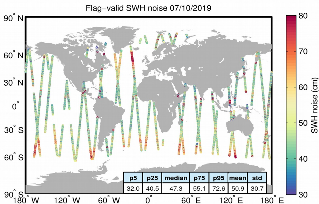
Figure 18. Geographical distribution of flag-valid 20-Hz SWH measurement noise over oceans and lakes for 07/10/2019. The statistical values shown in the figure refer to the SWH noise and are calculated over all measurements shown in the figure.
