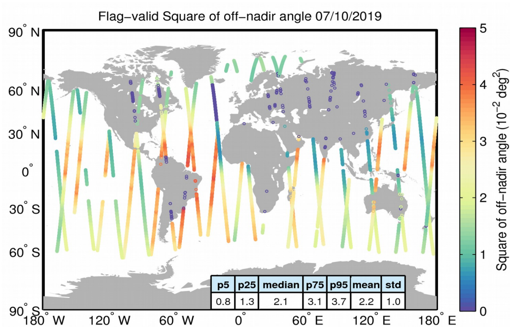
Figure 37. Geographical distribution of flag-valid mispointing data over oceans and lakes for 07/10/2019. The statistical values shown in the table refer to the mispointing in 10^{-2} \text{ deg}^2 and are calculated over all measurements shown in the figure.
