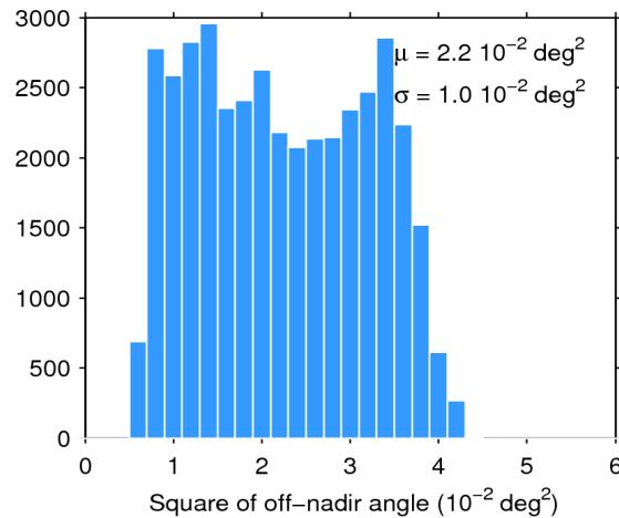
Figure 39. Histogram of flag-valid mispointing over oceans and lakes for 07/10/2019. The mean ( \mu ) and standard deviation ( \sigma ) are also shown. Note that values larger than 6 \cdot 10^{-2} \text{ deg}^2 are excluded from the histogram for the sake of readability but not from the computation of \mu and \sigma .
