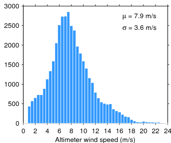
Figure 35. Histogram of science-valid wind over oceans and lakes for 07/10/2019. The mean ( \mu ) and standard deviation ( \sigma ) are also shown. Note that values larger than 24 m/s are excluded from the histogram for the sake of readability but not from the computation of \mu and \sigma .
