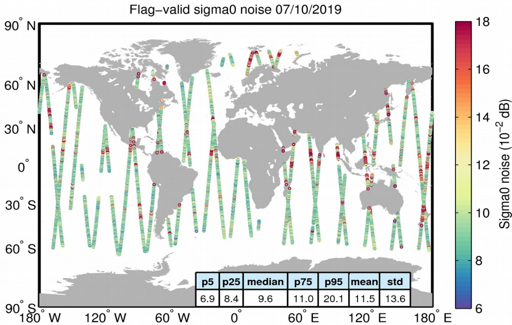
Figure 26. Geographical distribution of flag-valid 20-Hz sigma0 measurement noise over oceans and lakes for 07/10/2019. The statistical values shown in the table refer to the sigma0 noise and are calculated over all measurements shown in the figure.
