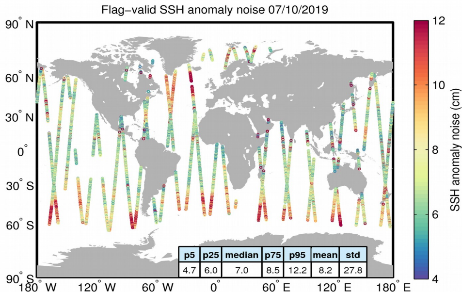
Figure 8. Geographical distribution of flag-valid 20-Hz SSH anomaly measurement noise over oceans and lakes for 07/10/2019. The statistical values shown in the table refer to the SSH anomaly noise and are calculated over all measurements shown in the figure.
