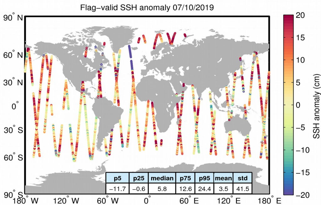
Figure 5. Geographical distribution of flag-valid 1-Hz SSH anomaly data over oceans and lakes for 07/10/2019. The statistical values shown in the table refer to the SSH anomaly in cm and are calculated over all measurements shown in the figure.
