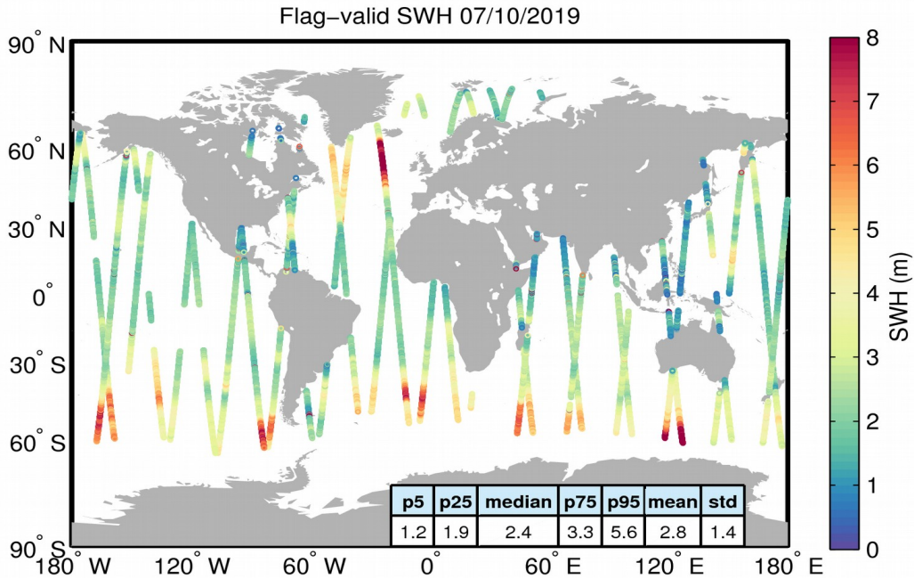
Figure 15. Geographical distribution of flag-valid SWH data over oceans and lakes for 07/10/2019. The statistical values shown in the table refer to the SWH in m and are calculated over all measurements shown in the figure.
