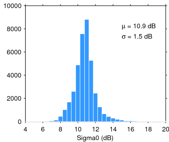
Figure 28. Histogram of science-valid sigma0 over oceans and lakes for 07/10/2019. The mean ( \mu ) and standard deviation ( \sigma ) are also shown. Note that values outside [4 20] dB are excluded from the histogram for the sake of readability but not from the computation of \mu and \sigma .
