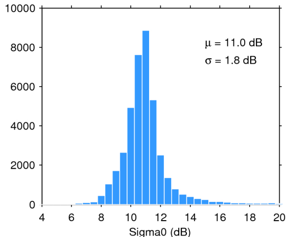
Figure 25. Histogram of flag-valid sigma0 over oceans and lakes for 07/10/2019. The mean ( \mu ) and standard deviation ( \sigma ) are also shown. Note that values outside [4 20] dB are excluded from the histogram for the sake of readability but not from the computation of \mu and \sigma .
