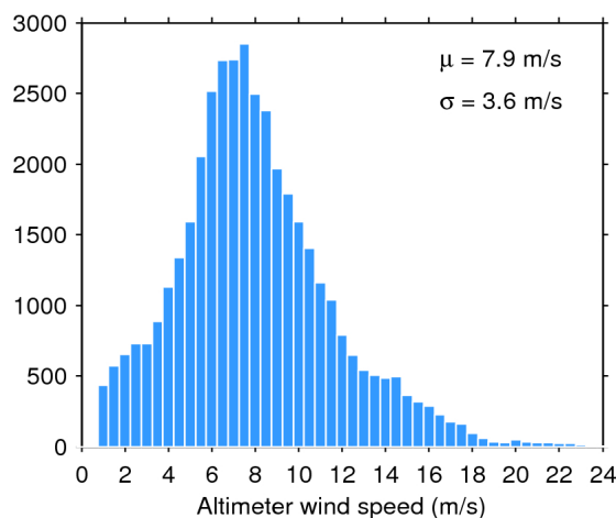
Figure 33. Histogram of flag-valid wind over oceans and lakes for 07/10/2019. The mean ( \mu ) and standard deviation ( \sigma ) are also shown. Note that values larger than 24 m/s are excluded from the histogram for the sake of readability but not from the computation of \mu and \sigma .
