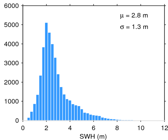
Figure 20. Histogram of science-valid SWH over oceans and lakes for 07/10/2019. The mean ( \mu ) and standard deviation ( \sigma ) are also shown. Note that values larger than 12 m are excluded from the histogram for the sake of readability but not from the computation of \mu and \sigma .
