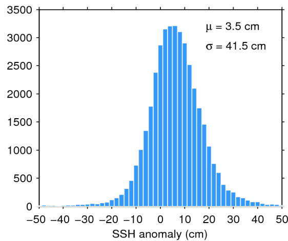
Figure 7. Histogram of flag-valid SSH anomaly over oceans and lakes for 07/10/2019. The mean ( \mu ) and standard deviation ( \sigma ) are also shown. Note that values outside [-50\ 50] cm are excluded from the histogram for the sake of readability but not from the computation of \mu and \sigma .
