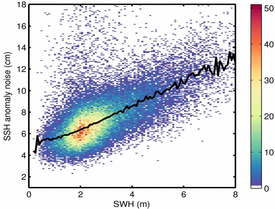
Figure 9. 2D histogram showing flag-valid SSH anomaly noise as a function of SWH for 07/10/2019. The black line denotes the median SSH anomaly noise as a function of SWH.
