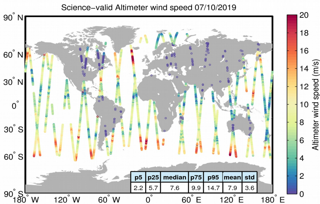
Figure 34. Geographical distribution of science-valid wind data over oceans and lakes for 07/10/2019. The statistical values shown in the table refer to the wind in m/s and are calculated over all measurements shown in the figure. Gray circles denote records that have been rejected based on the editing criteria described in Table 5.
