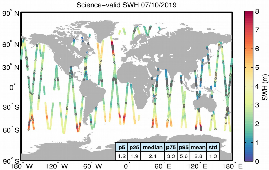
Figure 19. Geographical distribution of science-valid SWH data over oceans and lakes for 07/10/2019. The statistical values shown in the table refer to the SWH in m and are calculated over all measurements shown in the figure. Gray circles denote records that have been rejected based on the editing criteria described in Table 3.
