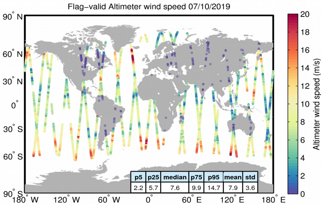
Figure 31. Geographical distribution of flag-valid wind data over oceans and lakes for 07/10/2019. The statistical values shown in the table refer to the wind in m/s and are calculated over all measurements shown in the figure.
