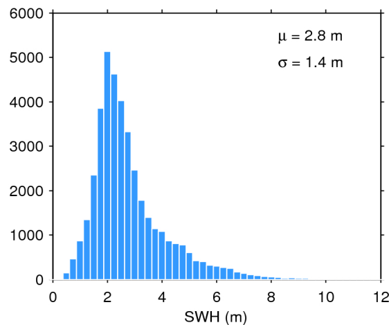
Figure 17. Histogram of flag-valid SWH over oceans and lakes for 07/10/2019. The mean ( \mu ) and standard deviation ( \sigma ) are also shown. Note that values larger than 12 m are excluded from the histogram for the sake of readability but not from the computation of \mu and \sigma .
