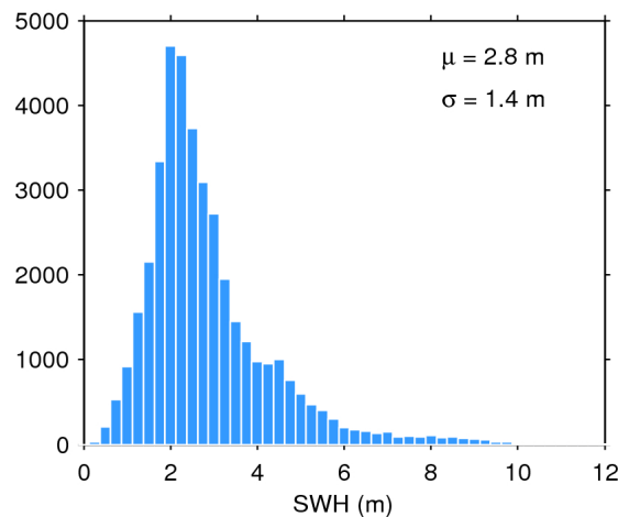
Figure 20. Histogram of science-valid SWH over oceans and lakes for 06/10/2019. The mean ( \mu ) and standard deviation ( \sigma ) are also shown. Note that values larger than 12 m are excluded from the histogram for the sake of readability but not from the computation of \mu and \sigma .
