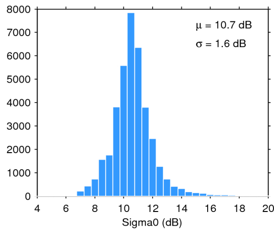
Figure 28. Histogram of science-valid sigma0 over oceans and lakes for 06/10/2019. The mean ( \mu ) and standard deviation ( \sigma ) are also shown. Note that values outside [4 20] dB are excluded from the histogram for the sake of readability but not from the computation of \mu and \sigma .
