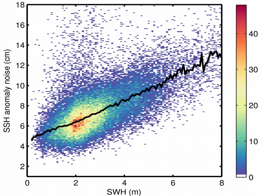
Figure 9. 2D histogram showing flag-valid SSH anomaly noise as a function of SWH for 06/10/2019. The black line denotes the median SSH anomaly noise as a function of SWH.
