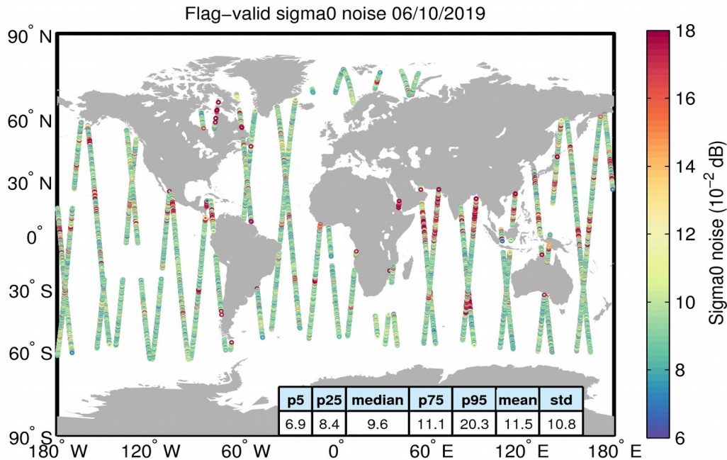
Figure 26. Geographical distribution of flag-valid 20-Hz sigma0 measurement noise over oceans and lakes for 06/10/2019. The statistical values shown in the table refer to the sigma0 noise and are calculated over all measurements shown in the figure.
