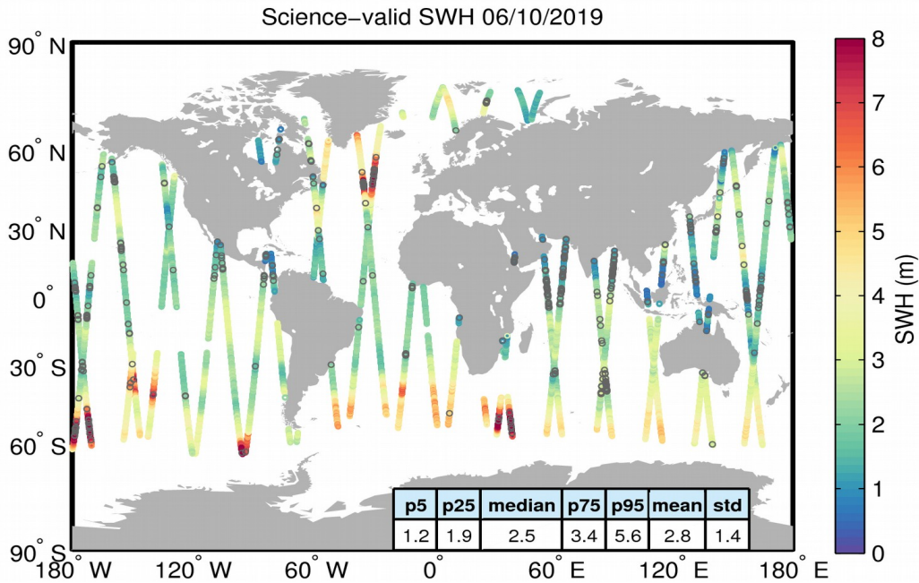
Figure 19. Geographical distribution of science-valid SWH data over oceans and lakes for 06/10/2019. The statistical values shown in the table refer to the SWH in m and are calculated over all measurements shown in the figure. Gray circles denote records that have been rejected based on the editing criteria described in Table 3.
