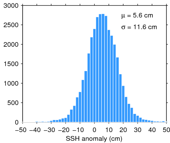
Figure 11. Histogram of science-valid SSH anomaly over oceans and lakes for 06/10/2019. The mean ( \mu ) and standard deviation ( \sigma ) are also shown. Note that values outside [-50 50] cm are excluded from the histogram for the sake of readability but not from the computation of \mu and \sigma .
