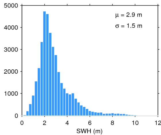
Figure 17. Histogram of flag-valid SWH over oceans and lakes for 06/10/2019. The mean ( \mu ) and standard deviation ( \sigma ) are also shown. Note that values larger than 12 m are excluded from the histogram for the sake of readability but not from the computation of \mu and \sigma .
