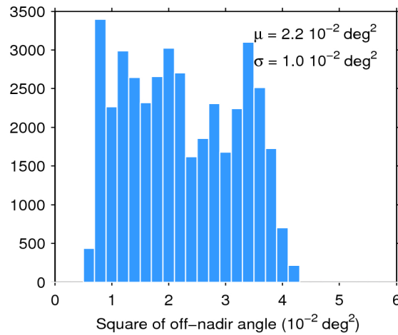
Figure 39. Histogram of flag-valid mispointing over oceans and lakes for 06/10/2019. The mean ( \mu ) and standard deviation ( \sigma ) are also shown. Note that values larger than 6 \cdot 10^{-2} \text{ deg}^2 are excluded from the histogram for the sake of readability but not from the computation of \mu and \sigma .
