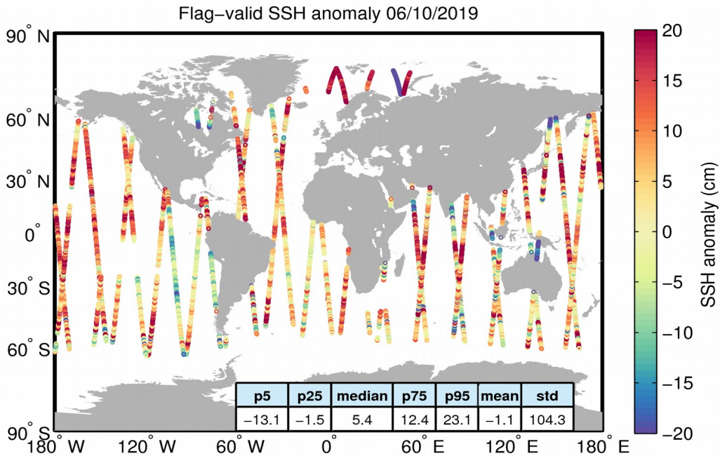
Figure 5. Geographical distribution of flag-valid 1-Hz SSH anomaly data over oceans and lakes for 06/10/2019. The statistical values shown in the table refer to the SSH anomaly in cm and are calculated over all measurements shown in the figure.
