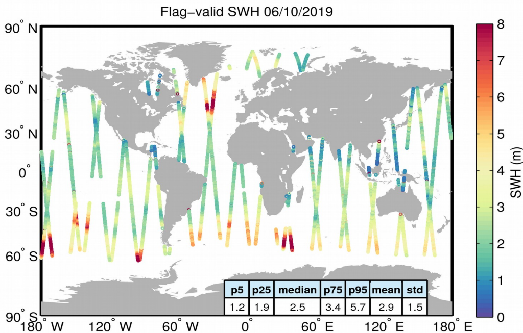
Figure 15. Geographical distribution of flag-valid SWH data over oceans and lakes for 06/10/2019. The statistical values shown in the table refer to the SWH in m and are calculated over all measurements shown in the figure.
