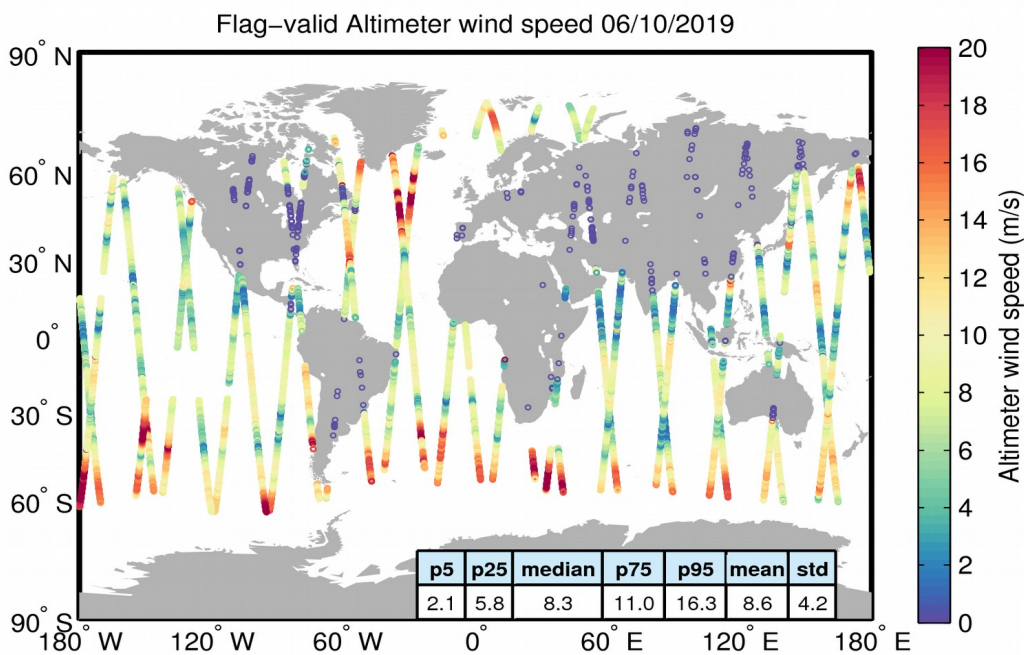
Figure 31. Geographical distribution of flag-valid wind data over oceans and lakes for 06/10/2019. The statistical values shown in the table refer to the wind in m/s and are calculated over all measurements shown in the figure.
