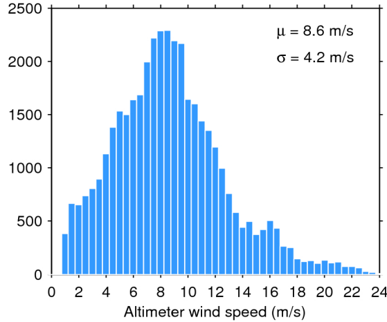
Figure 33. Histogram of flag-valid wind over oceans and lakes for 06/10/2019. The mean ( \mu ) and standard deviation ( \sigma ) are also shown. Note that values larger than 24 m/s are excluded from the histogram for the sake of readability but not from the computation of \mu and \sigma .
