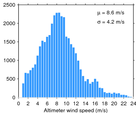
Figure 35. Histogram of science-valid wind over oceans and lakes for 06/10/2019. The mean ( \mu ) and standard deviation ( \sigma ) are also shown. Note that values larger than 24 m/s are excluded from the histogram for the sake of readability but not from the computation of \mu and \sigma .
