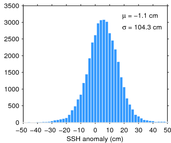
Figure 7. Histogram of flag-valid SSH anomaly over oceans and lakes for 06/10/2019. The mean ( \mu ) and standard deviation ( \sigma ) are also shown. Note that values outside [-50\ 50] cm are excluded from the histogram for the sake of readability but not from the computation of \mu and \sigma .
