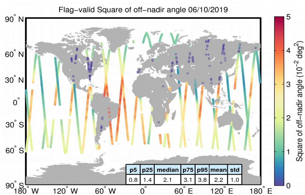
Figure 37. Geographical distribution of flag-valid mispointing data over oceans and lakes for 06/10/2019. The statistical values shown in the table refer to the mispointing in 10^{-2} \text{ deg}^2 and are calculated over all measurements shown in the figure.
