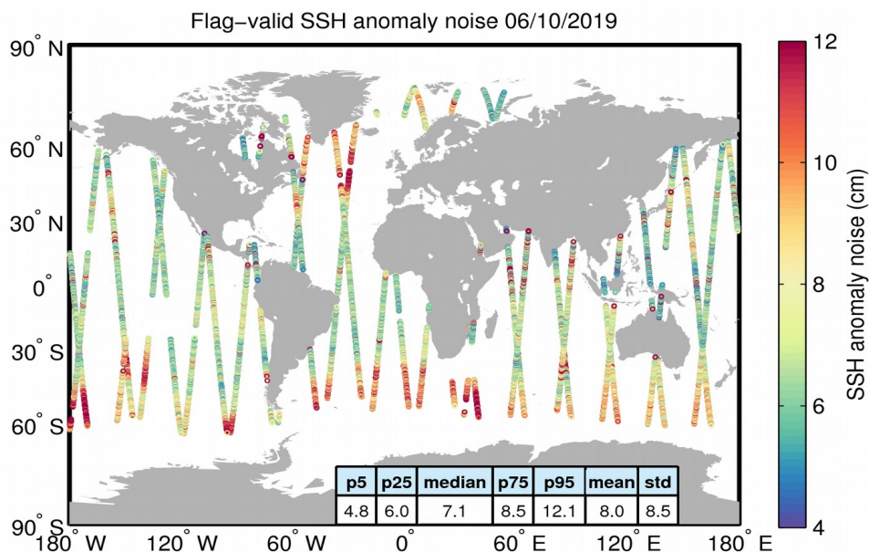
Figure 8. Geographical distribution of flag-valid 20-Hz SSH anomaly measurement noise over oceans and lakes for 06/10/2019. The statistical values shown in the table refer to the SSH anomaly noise and are calculated over all measurements shown in the figure.
