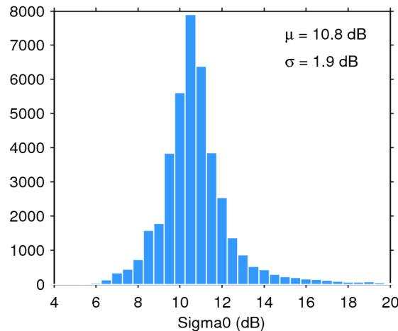
Figure 25. Histogram of flag-valid sigma0 over oceans and lakes for 06/10/2019. The mean ( \mu ) and standard deviation ( \sigma ) are also shown. Note that values outside [4 20] dB are excluded from the histogram for the sake of readability but not from the computation of \mu and \sigma .
