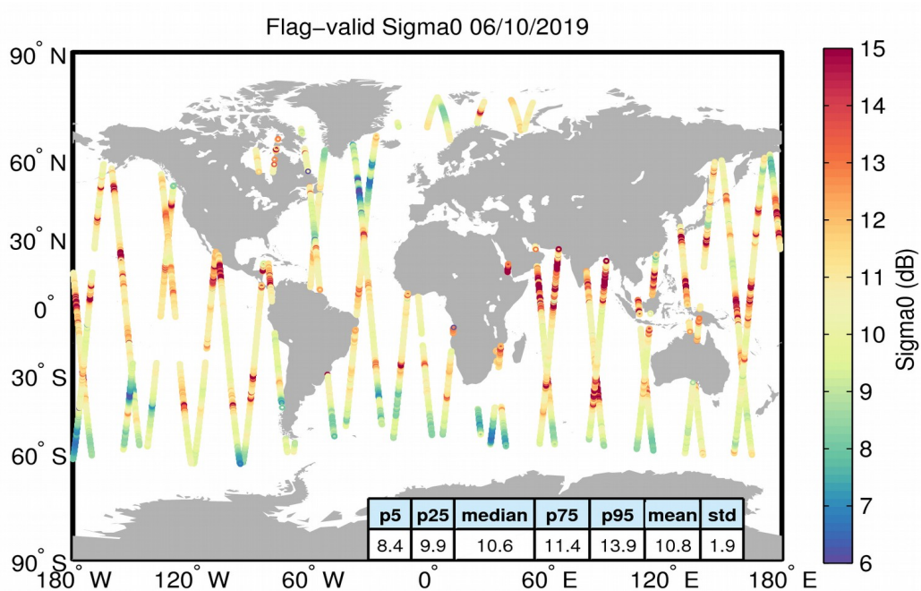
Figure 23. Geographical distribution of flag-valid sigma0 data over oceans and lakes for 06/10/2019. The statistical values shown in the table refer to the sigma0 in dB and are calculated over all measurements shown in the figure.
