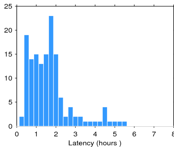
Figure 2. Histogram of the data latency for 06/10/2019. The y-axis denotes the number of files that are made available with a delay of x-hours with respect to the mean time of the records stored in the file.
