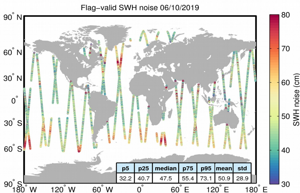
Figure 18. Geographical distribution of flag-valid 20-Hz SWH measurement noise over oceans and lakes for 06/10/2019. The statistical values shown in the table refer to the SWH noise and are calculated over all measurements shown in the figure.
