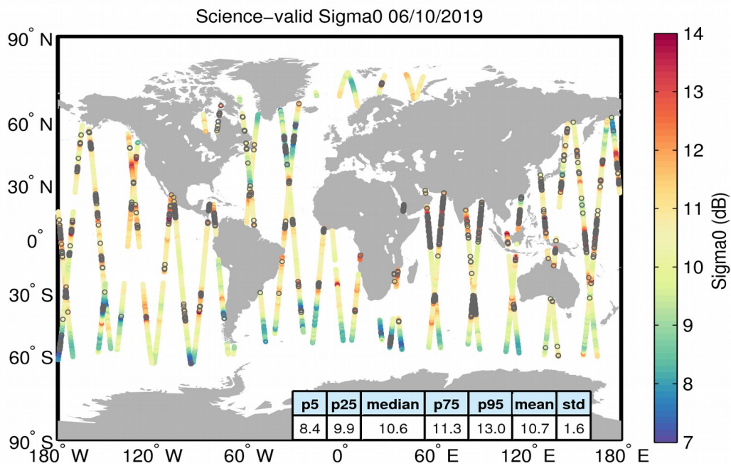
Figure 27. Geographical distribution of science-valid sigma0 data over oceans and lakes for 06/10/2019. The statistical values shown in the table refer to the sigma0 in dB and are calculated over all measurements shown in the figure. Gray circles denote records that have been rejected based on the editing criteria described in Table 4.
