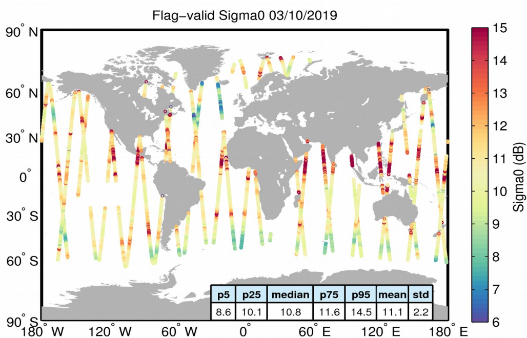
Figure 23. Geographical distribution of flag-valid sigma0 data over oceans and lakes for 03/10/2019. The statistical values shown in the table refer to the sigma0 in dB and are calculated over all measurements shown in the figure.
