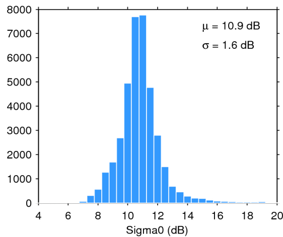
Figure 28. Histogram of science-valid sigma0 over oceans and lakes for 03/10/2019. The mean ( \mu ) and standard deviation ( \sigma ) are also shown. Note that values outside [4 20] dB are excluded from the histogram for the sake of readability but not from the computation of \mu and \sigma .
