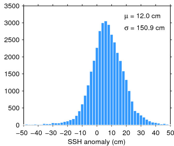
Figure 7. Histogram of flag-valid SSH anomaly over oceans and lakes for 03/10/2019. The mean ( \mu ) and standard deviation ( \sigma ) are also shown. Note that values outside [-50\ 50] cm are excluded from the histogram for the sake of readability but not from the computation of \mu and \sigma .
