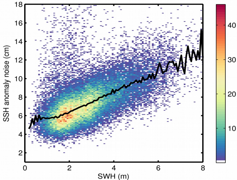
Figure 9. 2D histogram showing flag-valid SSH anomaly noise as a function of SWH for 03/10/2019. The black line denotes the median SSH anomaly noise as a function of SWH.
