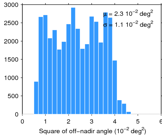
Figure 39. Histogram of flag-valid mispointing over oceans and lakes for 03/10/2019. The mean ( \mu ) and standard deviation ( \sigma ) are also shown. Note that values larger than 6 \cdot 10^{-2} \text{ deg}^2 are excluded from the histogram for the sake of readability but not from the computation of \mu and \sigma .
