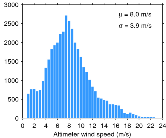
Figure 33. Histogram of flag-valid wind over oceans and lakes for 03/10/2019. The mean ( \mu ) and standard deviation ( \sigma ) are also shown. Note that values larger than 24 m/s are excluded from the histogram for the sake of readability but not from the computation of \mu and \sigma .
