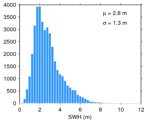
Figure 20. Histogram of science-valid SWH over oceans and lakes for 03/10/2019. The mean ( \mu ) and standard deviation ( \sigma ) are also shown. Note that values larger than 12 m are excluded from the histogram for the sake of readability but not from the computation of \mu and \sigma .
