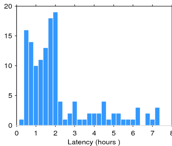
Figure 2. Histogram of the data latency for 03/10/2019. The y-axis denotes the number of files that are made available with a delay of x-hours with respect to the mean time of the records stored in the file.
