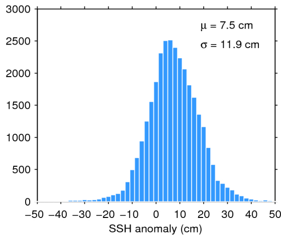
Figure 11. Histogram of science-valid SSH anomaly over oceans and lakes for 03/10/2019. The mean ( \mu ) and standard deviation ( \sigma ) are also shown. Note that values outside [-50 50] cm are excluded from the histogram for the sake of readability but not from the computation of \mu and \sigma .
