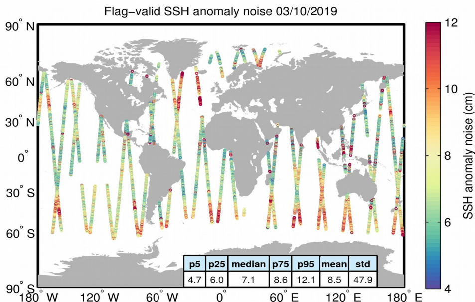
Figure 8. Geographical distribution of flag-valid 20-Hz SSH anomaly measurement noise over oceans and lakes for 03/10/2019. The statistical values shown in the table refer to the SSH anomaly noise and are calculated over all measurements shown in the figure.
