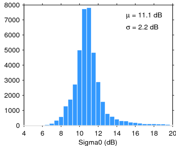
Figure 25. Histogram of flag-valid sigma0 over oceans and lakes for 03/10/2019. The mean ( \mu ) and standard deviation ( \sigma ) are also shown. Note that values outside [4 20] dB are excluded from the histogram for the sake of readability but not from the computation of \mu and \sigma .
