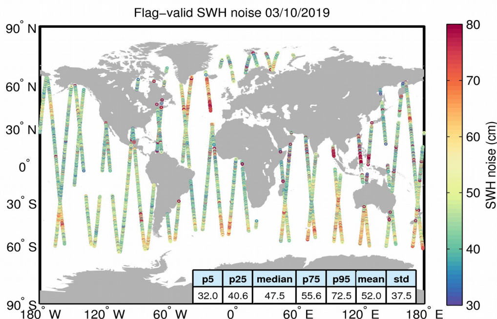
Figure 18. Geographical distribution of flag-valid 20-Hz SWH measurement noise over oceans and lakes for 03/10/2019. The statistical values shown in the figure refer to the SWH noise and are calculated over all measurements shown in the figure.
