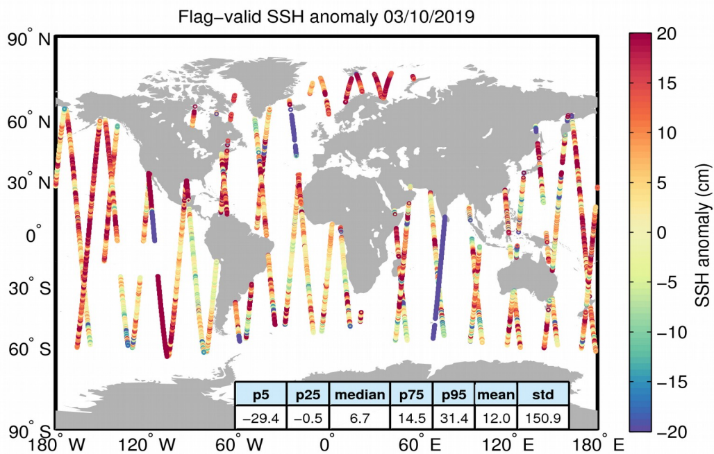
Figure 5. Geographical distribution of flag-valid 1-Hz SSH anomaly data over oceans and lakes for 03/10/2019. The statistical values shown in the table refer to the SSH anomaly in cm and are calculated over all measurements shown in the figure.
