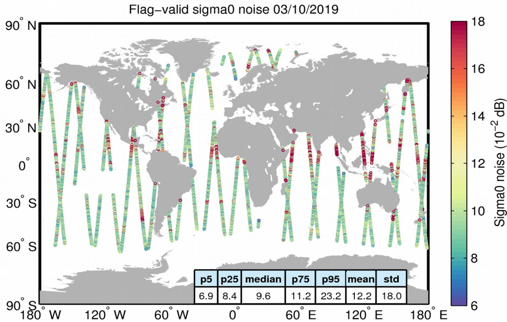
Figure 26. Geographical distribution of flag-valid 20-Hz sigma0 measurement noise over oceans and lakes for 03/10/2019. The statistical values shown in the table refer to the sigma0 noise and are calculated over all measurements shown in the figure.
