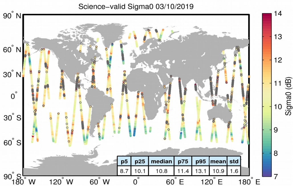
Figure 27. Geographical distribution of science-valid sigma0 data over oceans and lakes for 03/10/2019. The statistical values shown in the table refer to the sigma0 in dB and are calculated over all measurements shown in the figure. Gray circles denote records that have been rejected based on the editing criteria described in Table 4.
