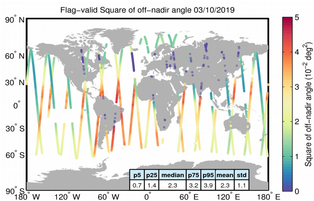
Figure 37. Geographical distribution of flag-valid mispointing data over oceans and lakes for 03/10/2019. The statistical values shown in the table refer to the mispointing in 10^{-2} \text{ deg}^2 and are calculated over all measurements shown in the figure.
