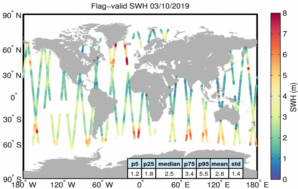
Figure 15. Geographical distribution of flag-valid SWH data over oceans and lakes for 03/10/2019. The statistical values shown in the table refer to the SWH in m and are calculated over all measurements shown in the figure.
