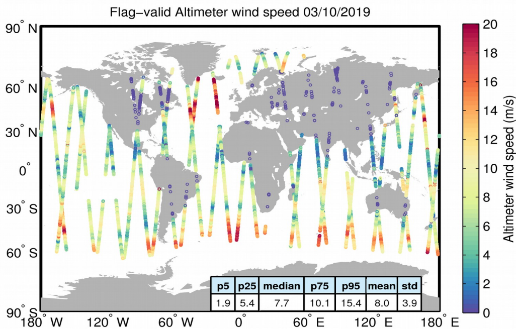
Figure 31. Geographical distribution of flag-valid wind data over oceans and lakes for 03/10/2019. The statistical values shown in the table refer to the wind in m/s and are calculated over all measurements shown in the figure.
