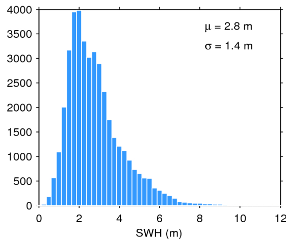
Figure 17. Histogram of flag-valid SWH over oceans and lakes for 03/10/2019. The mean ( \mu ) and standard deviation ( \sigma ) are also shown. Note that values larger than 12 m are excluded from the histogram for the sake of readability but not from the computation of \mu and \sigma .
