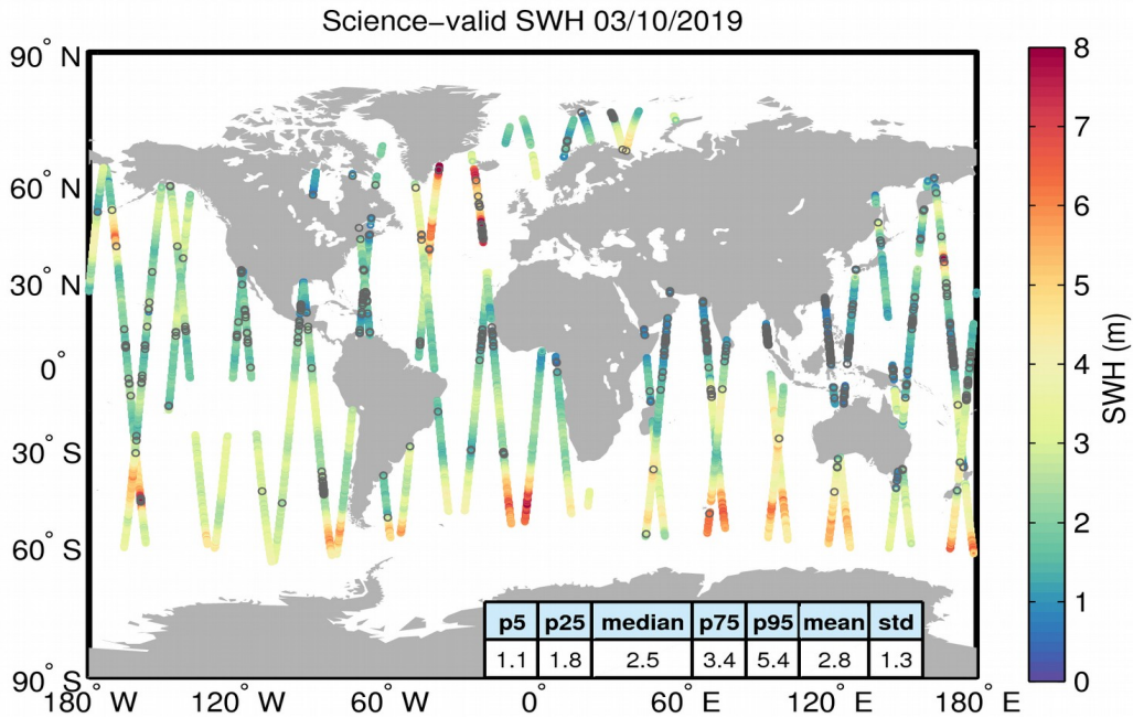
Figure 19. Geographical distribution of science-valid SWH data over oceans and lakes for 03/10/2019. The statistical values shown in the table refer to the SWH in m and are calculated over all measurements shown in the figure. Gray circles denote records that have been rejected based on the editing criteria described in Table 3.
