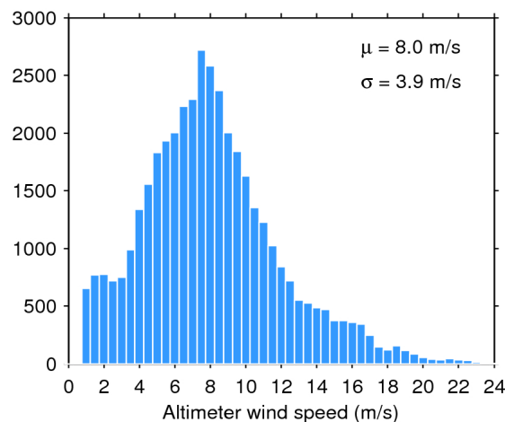
Figure 35. Histogram of science-valid wind over oceans and lakes for 03/10/2019. The mean ( \mu ) and standard deviation ( \sigma ) are also shown. Note that values larger than 24 m/s are excluded from the histogram for the sake of readability but not from the computation of \mu and \sigma .
