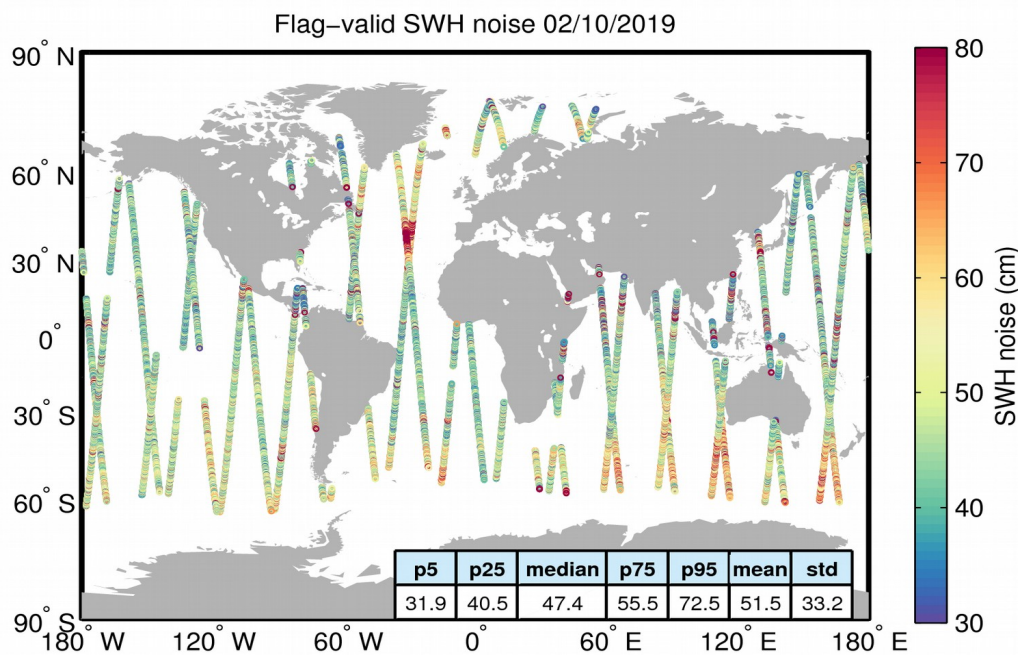
Figure 18. Geographical distribution of flag-valid 20-Hz SWH measurement noise over oceans and lakes for 02/10/2019. The statistical values shown in the table refer to the SWH noise and are calculated over all measurements shown in the figure.
