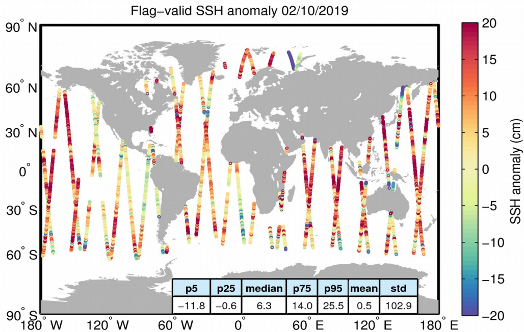
Figure 5. Geographical distribution of flag-valid 1-Hz SSH anomaly data over oceans and lakes for 02/10/2019. The statistical values shown in the table refer to the SSH anomaly in cm and are calculated over all measurements shown in the figure.
