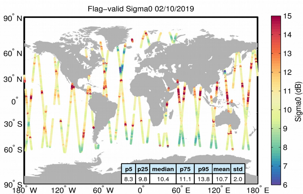
Figure 23. Geographical distribution of flag-valid sigma0 data over oceans and lakes for 02/10/2019. The statistical values shown in the table refer to the sigma0 in dB and are calculated over all measurements shown in the figure.
