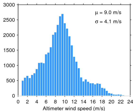
Figure 35. Histogram of science-valid wind over oceans and lakes for 02/10/2019. The mean ( \mu ) and standard deviation ( \sigma ) are also shown. Note that values larger than 24 m/s are excluded from the histogram for the sake of readability but not from the computation of \mu and \sigma .
