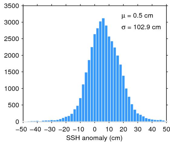
Figure 7. Histogram of flag-valid SSH anomaly over oceans and lakes for 02/10/2019. The mean ( \mu ) and standard deviation ( \sigma ) are also shown. Note that values outside [-50\ 50] cm are excluded from the histogram for the sake of readability but not from the computation of \mu and \sigma .
