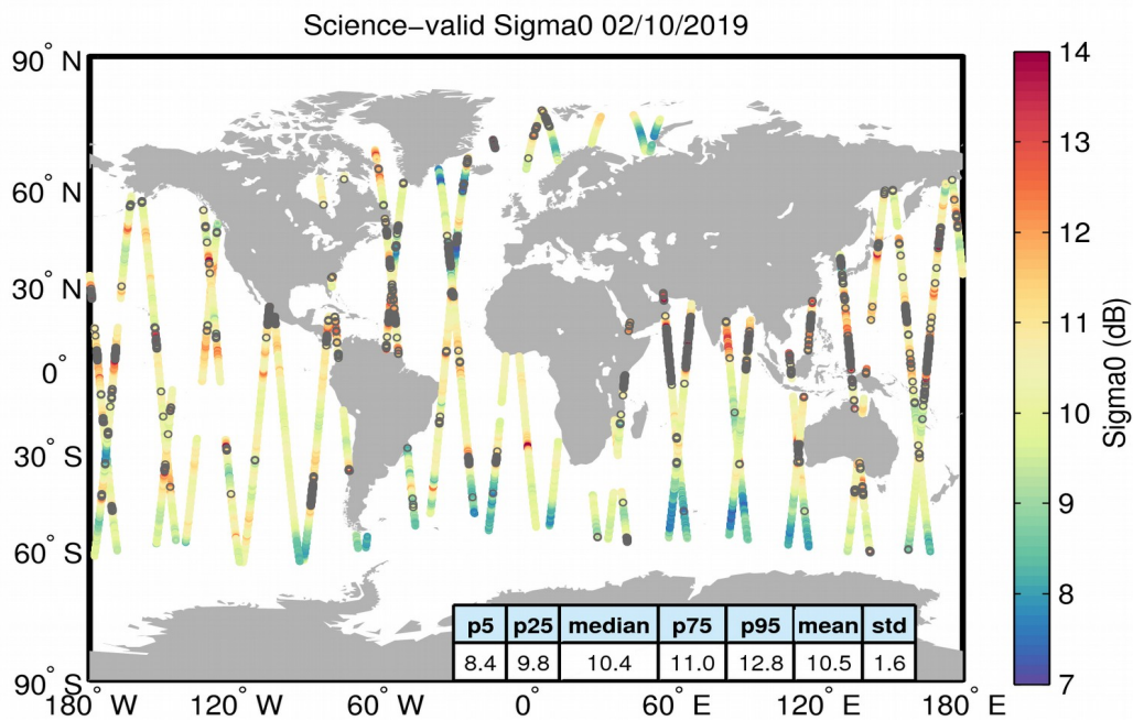
Figure 27. Geographical distribution of science-valid sigma0 data over oceans and lakes for 02/10/2019. The statistical values shown in the table refer to the sigma0 in dB and are calculated over all measurements shown in the figure. Gray circles denote records that have been rejected based on the editing criteria described in Table 4.
