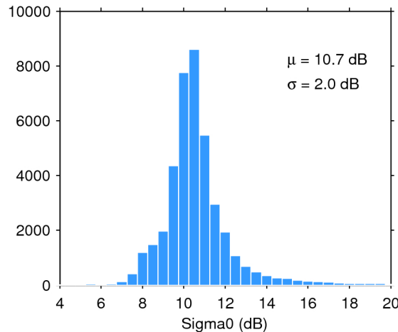
Figure 25. Histogram of flag-valid sigma0 over oceans and lakes for 02/10/2019. The mean ( \mu ) and standard deviation ( \sigma ) are also shown. Note that values outside [4 20] dB are excluded from the histogram for the sake of readability but not from the computation of \mu and \sigma .
