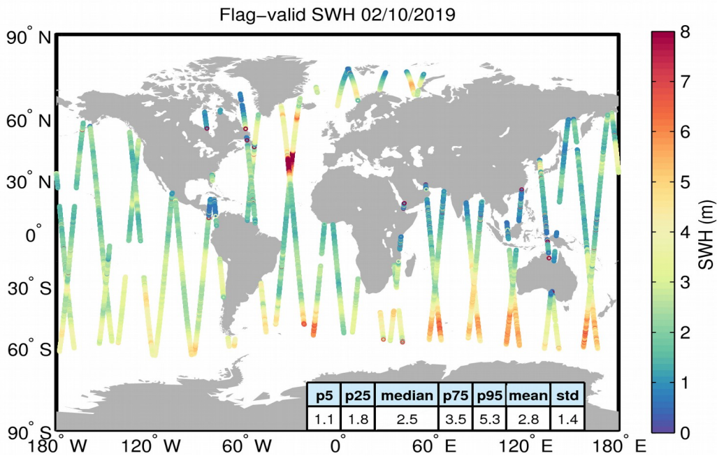
Figure 15. Geographical distribution of flag-valid SWH data over oceans and lakes for 02/10/2019. The statistical values shown in the table refer to the SWH in m and are calculated over all measurements shown in the figure.
