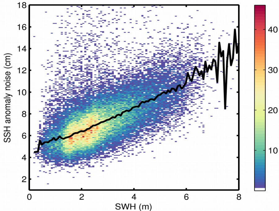
Figure 9. 2D histogram showing flag-valid SSH anomaly noise as a function of SWH for 02/10/2019. The black line denotes the median SSH anomaly noise as a function of SWH.
