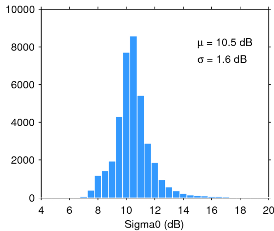
Figure 28. Histogram of science-valid sigma0 over oceans and lakes for 02/10/2019. The mean ( \mu ) and standard deviation ( \sigma ) are also shown. Note that values outside [4 20] dB are excluded from the histogram for the sake of readability but not from the computation of \mu and \sigma .
