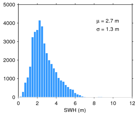
Figure 20. Histogram of science-valid SWH over oceans and lakes for 02/10/2019. The mean ( \mu ) and standard deviation ( \sigma ) are also shown. Note that values larger than 12 m are excluded from the histogram for the sake of readability but not from the computation of \mu and \sigma .
