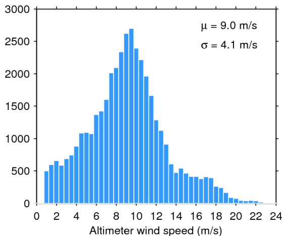
Figure 33. Histogram of flag-valid wind over oceans and lakes for 02/10/2019. The mean ( \mu ) and standard deviation ( \sigma ) are also shown. Note that values larger than 24 m/s are excluded from the histogram for the sake of readability but not from the computation of \mu and \sigma .
