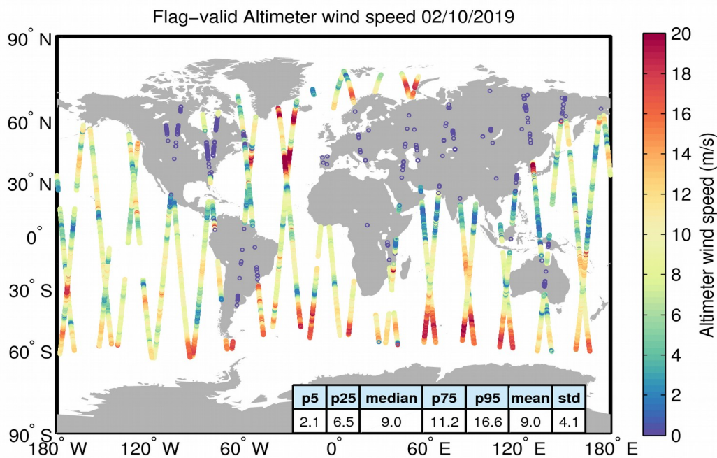
Figure 31. Geographical distribution of flag-valid wind data over oceans and lakes for 02/10/2019. The statistical values shown in the table refer to the wind in m/s and are calculated over all measurements shown in the figure.
