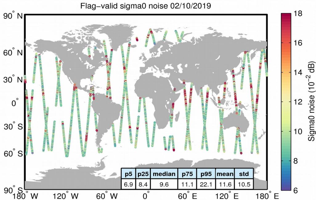
Figure 26. Geographical distribution of flag-valid 20-Hz sigma0 measurement noise over oceans and lakes for 02/10/2019. The statistical values shown in the table refer to the sigma0 noise and are calculated over all measurements shown in the figure.
