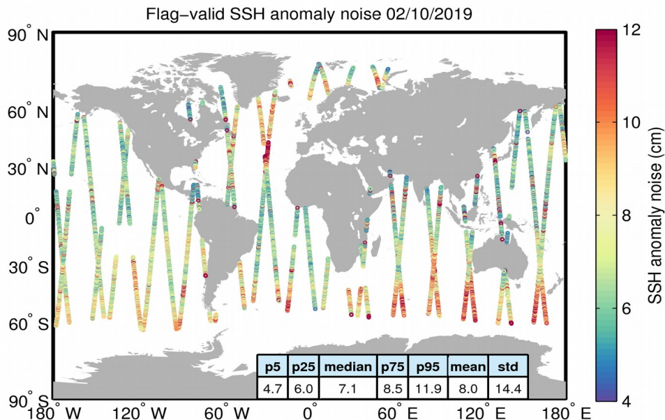
Figure 8. Geographical distribution of flag-valid 20-Hz SSH anomaly measurement noise over oceans and lakes for 02/10/2019. The statistical values shown in the table refer to the SSH anomaly noise and are calculated over all measurements shown in the figure.
