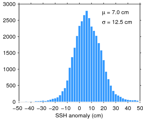
Figure 11. Histogram of science-valid SSH anomaly over oceans and lakes for 02/10/2019. The mean ( \mu ) and standard deviation ( \sigma ) are also shown. Note that values outside [-50 50] cm are excluded from the histogram for the sake of readability but not from the computation of \mu and \sigma .
