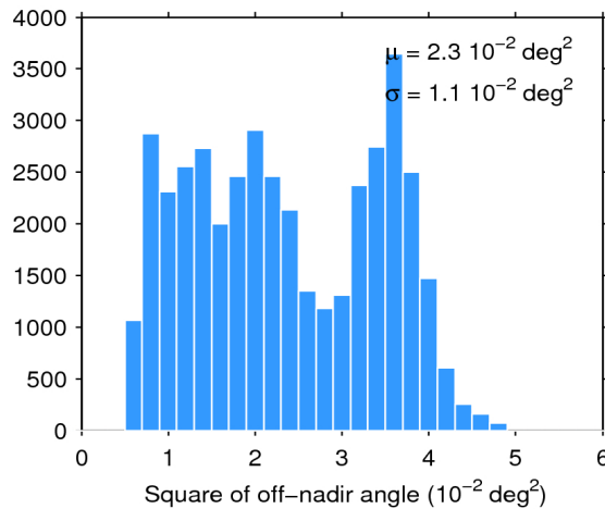
Figure 39. Histogram of flag-valid mispointing over oceans and lakes for 02/10/2019. The mean ( \mu ) and standard deviation ( \sigma ) are also shown. Note that values larger than 6 \cdot 10^{-2} \text{ deg}^2 are excluded from the histogram for the sake of readability but not from the computation of \mu and \sigma .
