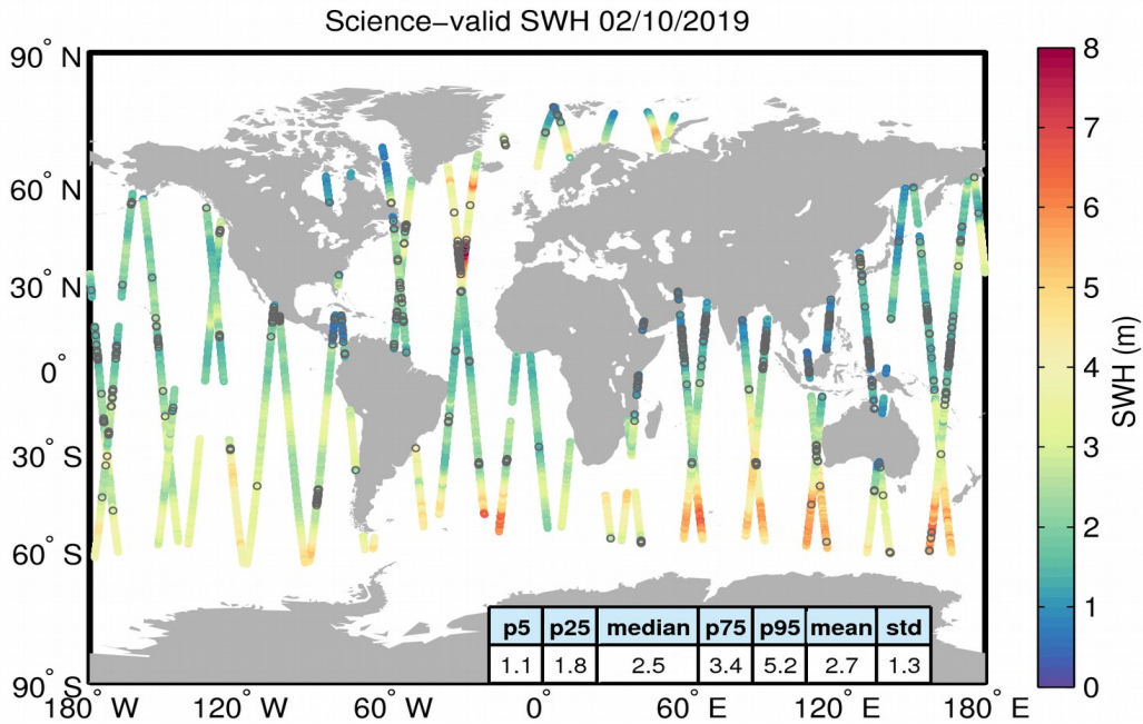
Figure 19. Geographical distribution of science-valid SWH data over oceans and lakes for 02/10/2019. The statistical values shown in the table refer to the SWH in m and are calculated over all measurements shown in the figure. Gray circles denote records that have been rejected based on the editing criteria described in Table 3.
