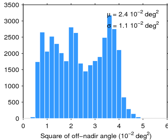
Figure 39. Histogram of flag-valid mispointing over oceans and lakes for 01/10/2019. The mean ( \mu ) and standard deviation ( \sigma ) are also shown. Note that values larger than 6 \cdot 10^{-2} \text{ deg}^2 are excluded from the histogram for the sake of readability but not from the computation of \mu and \sigma .
