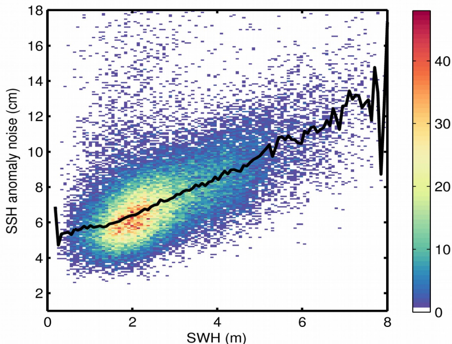
Figure 9. 2D histogram showing flag-valid SSH anomaly noise as a function of SWH for 01/10/2019. The black line denotes the median SSH anomaly noise as a function of SWH.
