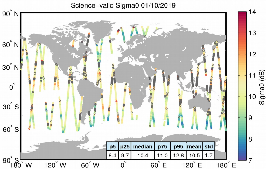
Figure 27. Geographical distribution of science-valid sigma0 data over oceans and lakes for 01/10/2019. The statistical values shown in the table refer to the sigma0 in dB and are calculated over all measurements shown in the figure. Gray circles denote records that have been rejected based on the editing criteria described in Table 4.
