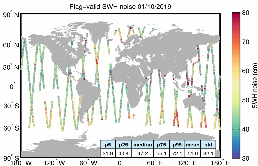
Figure 18. Geographical distribution of flag-valid 20-Hz SWH measurement noise over oceans and lakes for 01/10/2019. The statistical values shown in the table refer to the SWH noise and are calculated over all measurements shown in the figure.
