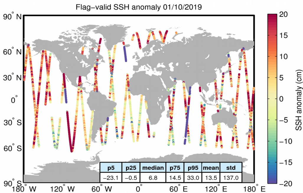
Figure 5. Geographical distribution of flag-valid 1-Hz SSH anomaly data over oceans and lakes for 01/10/2019. The statistical values shown in the table refer to the SSH anomaly in cm and are calculated over all measurements shown in the figure.
