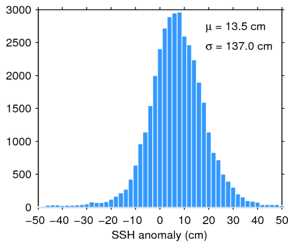
Figure 7. Histogram of flag-valid SSH anomaly over oceans and lakes for 01/10/2019. The mean ( \mu ) and standard deviation ( \sigma ) are also shown. Note that values outside [-50 50] cm are excluded from the histogram for the sake of readability but not from the computation of \mu and \sigma .
