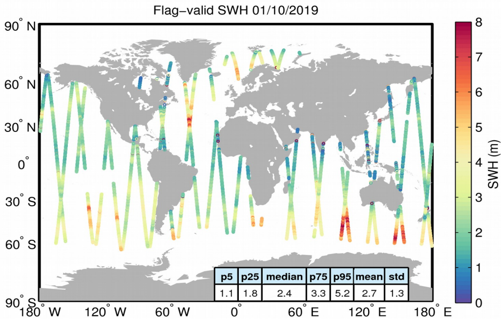
Figure 15. Geographical distribution of flag-valid SWH data over oceans and lakes for 01/10/2019. The statistical values shown in the table refer to the SWH in m and are calculated over all measurements shown in the figure.
