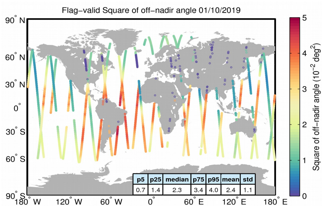
Figure 37. Geographical distribution of flag-valid mispointing data over oceans and lakes for 01/10/2019. The statistical values shown in the table refer to the mispointing in 10^{-2} \text{ deg}^2 and are calculated over all measurements shown in the figure.
