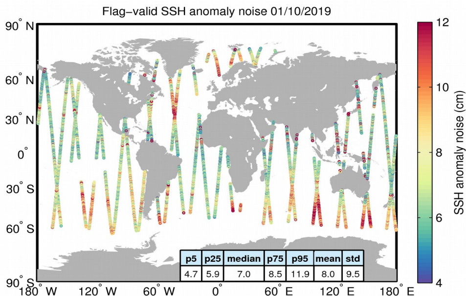
Figure 8. Geographical distribution of flag-valid 20-Hz SSH anomaly measurement noise over oceans and lakes for 01/10/2019. The statistical values shown in the table refer to the SSH anomaly noise and are calculated over all measurements shown in the figure.
