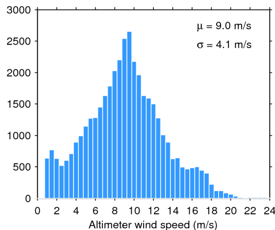
Figure 35. Histogram of science-valid wind over oceans and lakes for 01/10/2019. The mean ( \mu ) and standard deviation ( \sigma ) are also shown. Note that values larger than 24 m/s are excluded from the histogram for the sake of readability but not from the computation of \mu and \sigma .
