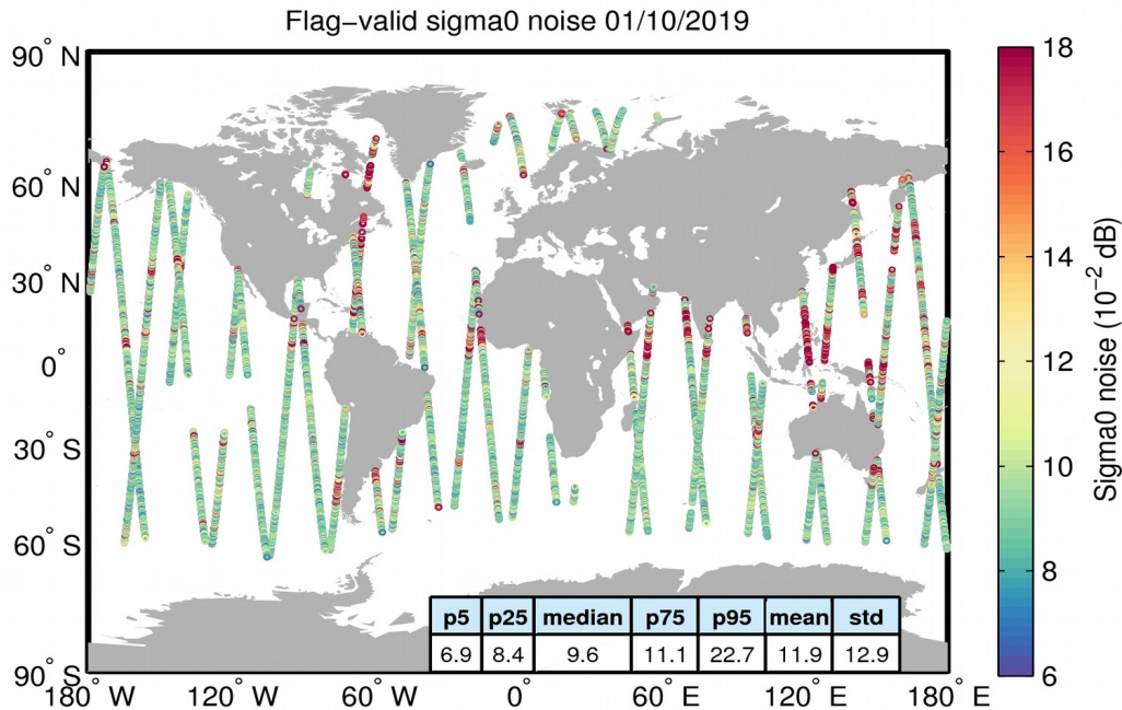
Figure 26. Geographical distribution of flag-valid 20-Hz sigma0 measurement noise over oceans and lakes for 01/10/2019. The statistical values shown in the table refer to the sigma0 noise and are calculated over all measurements shown in the figure.
