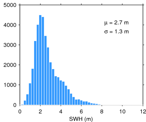
Figure 20. Histogram of science-valid SWH over oceans and lakes for 01/10/2019. The mean ( \mu ) and standard deviation ( \sigma ) are also shown. Note that values larger than 12 m are excluded from the histogram for the sake of readability but not from the computation of \mu and \sigma .
