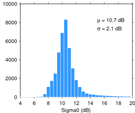
Figure 25. Histogram of flag-valid sigma0 over oceans and lakes for 01/10/2019. The mean ( \mu ) and standard deviation ( \sigma ) are also shown. Note that values outside [4 20] dB are excluded from the histogram for the sake of readability but not from the computation of \mu and \sigma .
