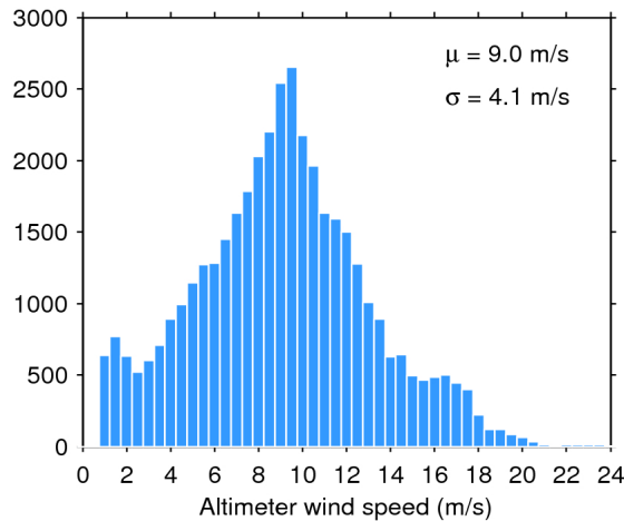
Figure 33. Histogram of flag-valid wind over oceans and lakes for 01/10/2019. The mean ( \mu ) and standard deviation ( \sigma ) are also shown. Note that values larger than 24 m/s are excluded from the histogram for the sake of readability but not from the computation of \mu and \sigma .
