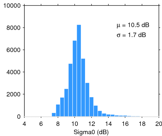
Figure 28. Histogram of science-valid sigma0 over oceans and lakes for 01/10/2019. The mean ( \mu ) and standard deviation ( \sigma ) are also shown. Note that values outside [4 20] dB are excluded from the histogram for the sake of readability but not from the computation of \mu and \sigma .
