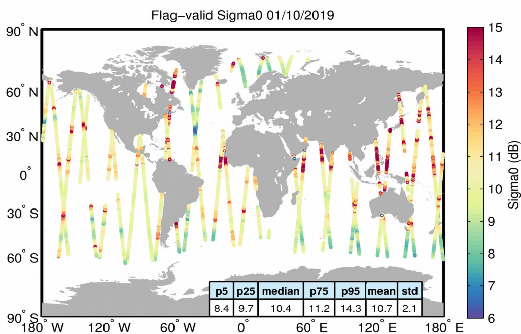
Figure 23. Geographical distribution of flag-valid sigma0 data over oceans and lakes for 01/10/2019. The statistical values shown in the table refer to the sigma0 in dB and are calculated over all measurements shown in the figure.
