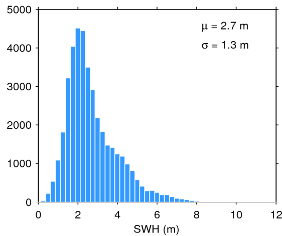
Figure 17. Histogram of flag-valid SWH over oceans and lakes for 01/10/2019. The mean ( \mu ) and standard deviation ( \sigma ) are also shown. Note that values larger than 12 m are excluded from the histogram for the sake of readability but not from the computation of \mu and \sigma .
