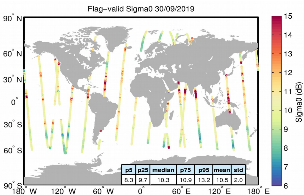
Figure 23. Geographical distribution of flag-valid sigma0 data over oceans and lakes for 30/09/2019. The statistical values shown in the table refer to the sigma0 in dB and are calculated over all measurements shown in the figure.
