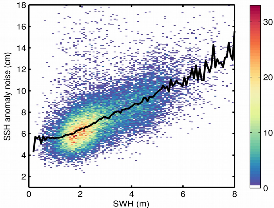
Figure 9. 2D histogram showing flag-valid SSH anomaly noise as a function of SWH for 30/09/2019. The black line denotes the median SSH anomaly noise as a function of SWH.
