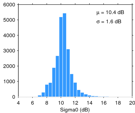
Figure 28. Histogram of science-valid sigma0 over oceans and lakes for 30/09/2019. The mean ( \mu ) and standard deviation ( \sigma ) are also shown. Note that values outside [4 20] dB are excluded from the histogram for the sake of readability but not from the computation of \mu and \sigma .
