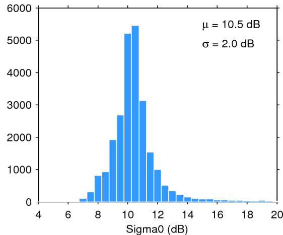
Figure 25. Histogram of flag-valid sigma0 over oceans and lakes for 30/09/2019. The mean ( \mu ) and standard deviation ( \sigma ) are also shown. Note that values outside [4 20] dB are excluded from the histogram for the sake of readability but not from the computation of \mu and \sigma .
