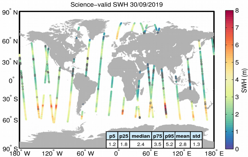
Figure 19. Geographical distribution of science-valid SWH data over oceans and lakes for 30/09/2019. The statistical values shown in the table refer to the SWH in m and are calculated over all measurements shown in the figure. Gray circles denote records that have been rejected based on the editing criteria described in Table 3.
