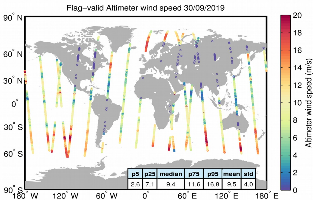
Figure 31. Geographical distribution of flag-valid wind data over oceans and lakes for 30/09/2019. The statistical values shown in the table refer to the wind in m/s and are calculated over all measurements shown in the figure.
