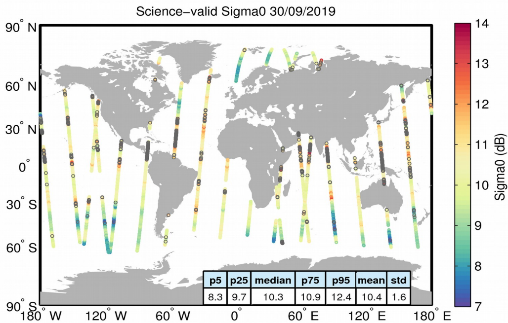
Figure 27. Geographical distribution of science-valid sigma0 data over oceans and lakes for 30/09/2019. The statistical values shown in the table refer to the sigma0 in dB and are calculated over all measurements shown in the figure. Gray circles denote records that have been rejected based on the editing criteria described in Table 4.
