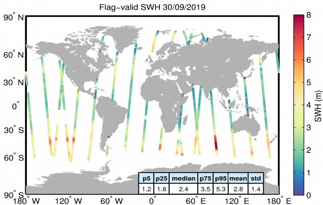
Figure 15. Geographical distribution of flag-valid SWH data over oceans and lakes for 30/09/2019. The statistical values shown in the table refer to the SWH in m and are calculated over all measurements shown in the figure.
