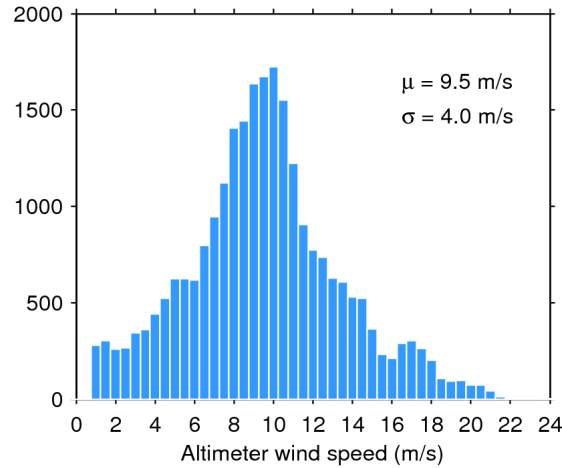
Figure 33. Histogram of flag-valid wind over oceans and lakes for 30/09/2019. The mean ( \mu ) and standard deviation ( \sigma ) are also shown. Note that values larger than 24 m/s are excluded from the histogram for the sake of readability but not from the computation of \mu and \sigma .
