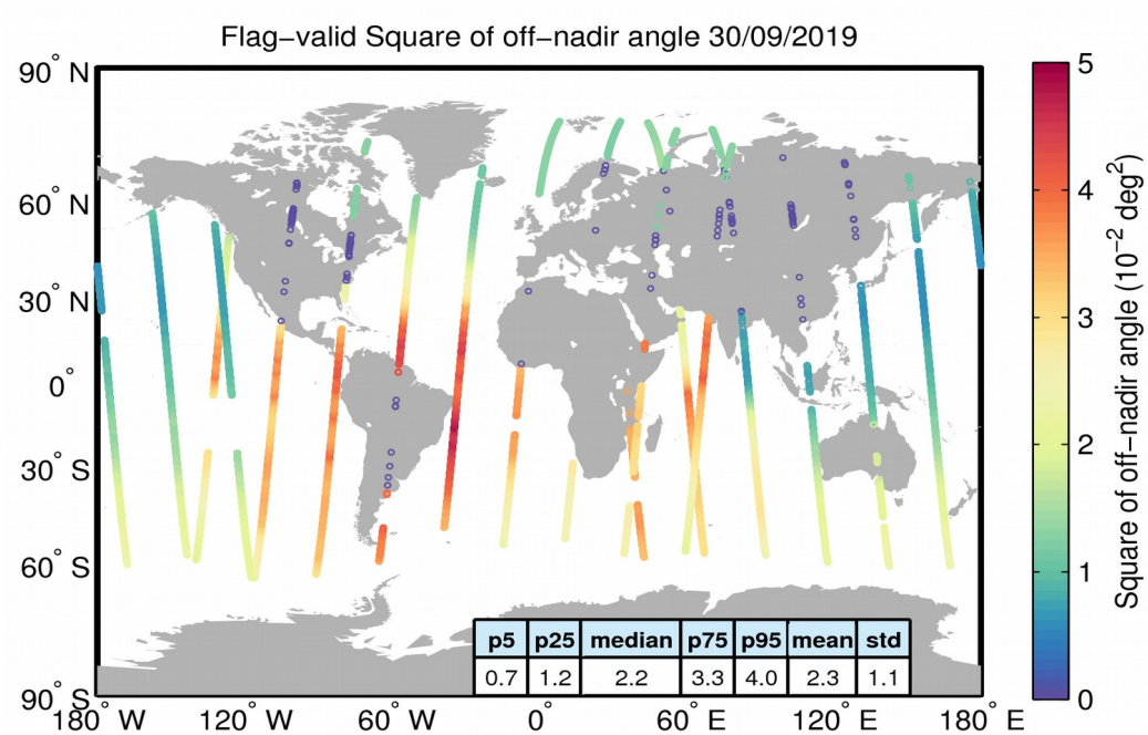
Figure 37. Geographical distribution of flag-valid mispointing data over oceans and lakes for 30/09/2019. The statistical values shown in the table refer to the mispointing in 10^{-2} \text{ deg}^2 and are calculated over all measurements shown in the figure.
