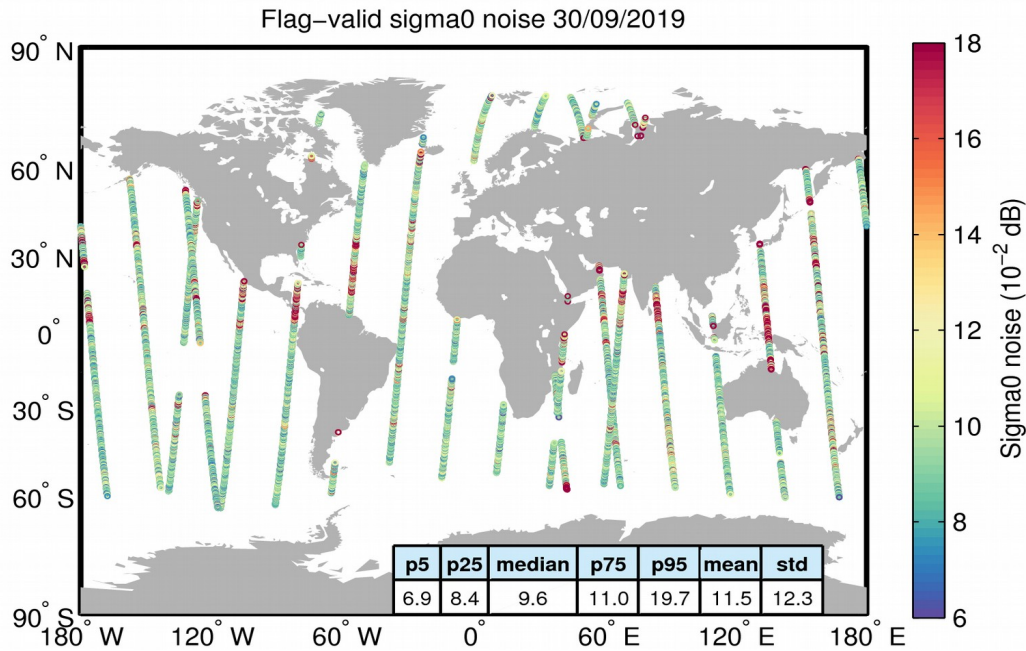
Figure 26. Geographical distribution of flag-valid 20-Hz sigma0 measurement noise over oceans and lakes for 30/09/2019. The statistical values shown in the table refer to the sigma0 noise and are calculated over all measurements shown in the figure.
