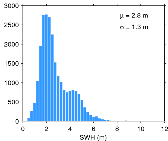
Figure 20. Histogram of science-valid SWH over oceans and lakes for 30/09/2019. The mean ( \mu ) and standard deviation ( \sigma ) are also shown. Note that values larger than 12 m are excluded from the histogram for the sake of readability but not from the computation of \mu and \sigma .
