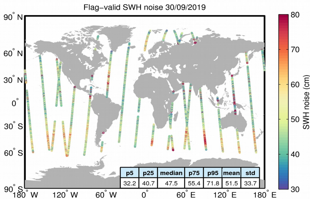
Figure 18. Geographical distribution of flag-valid 20-Hz SWH measurement noise over oceans and lakes for 30/09/2019. The statistical values shown in the figure refer to the SWH noise and are calculated over all measurements shown in the figure.
