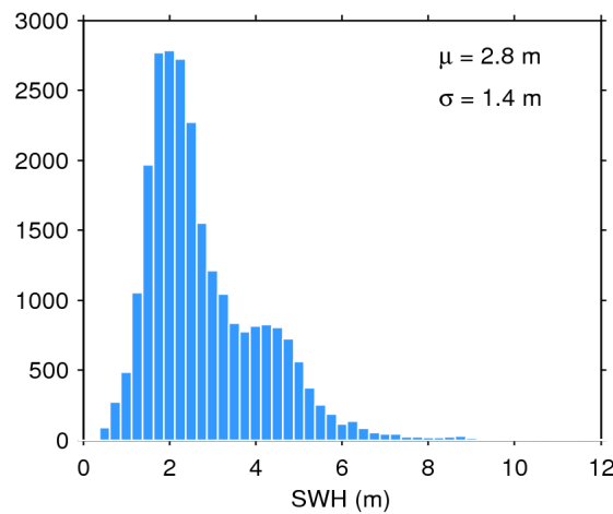
Figure 17. Histogram of flag-valid SWH over oceans and lakes for 30/09/2019. The mean ( \mu ) and standard deviation ( \sigma ) are also shown. Note that values larger than 12 m are excluded from the histogram for the sake of readability but not from the computation of \mu and \sigma .
