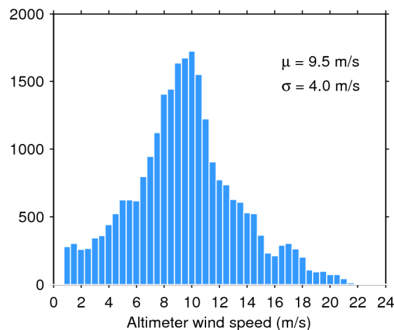
Figure 35. Histogram of science-valid wind over oceans and lakes for 30/09/2019. The mean ( \mu ) and standard deviation ( \sigma ) are also shown. Note that values larger than 24 m/s are excluded from the histogram for the sake of readability but not from the computation of \mu and \sigma .
