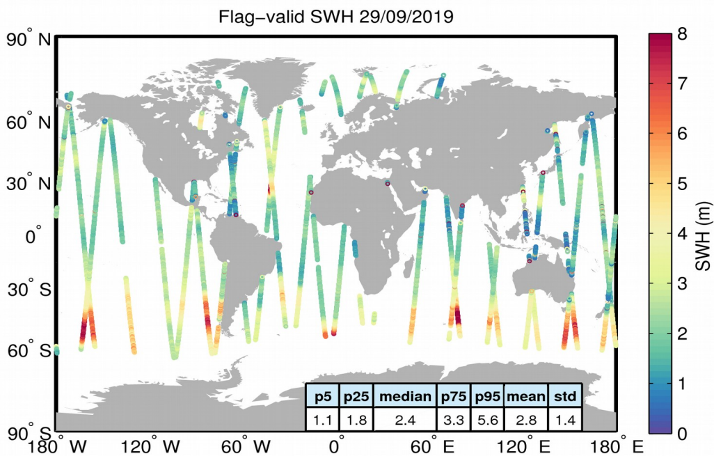
Figure 15. Geographical distribution of flag-valid SWH data over oceans and lakes for 29/09/2019. The statistical values shown in the table refer to the SWH in m and are calculated over all measurements shown in the figure.
