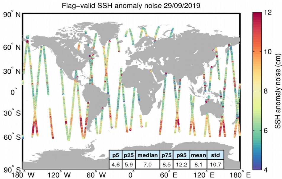
Figure 8. Geographical distribution of flag-valid 20-Hz SSH anomaly measurement noise over oceans and lakes for 29/09/2019. The statistical values shown in the table refer to the SSH anomaly noise and are calculated over all measurements shown in the figure.
