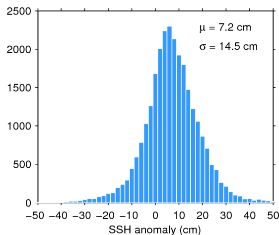
Figure 11. Histogram of science-valid SSH anomaly over oceans and lakes for 29/09/2019. The mean ( \mu ) and standard deviation ( \sigma ) are also shown. Note that values outside [-50 50] cm are excluded from the histogram for the sake of readability but not from the computation of \mu and \sigma .
