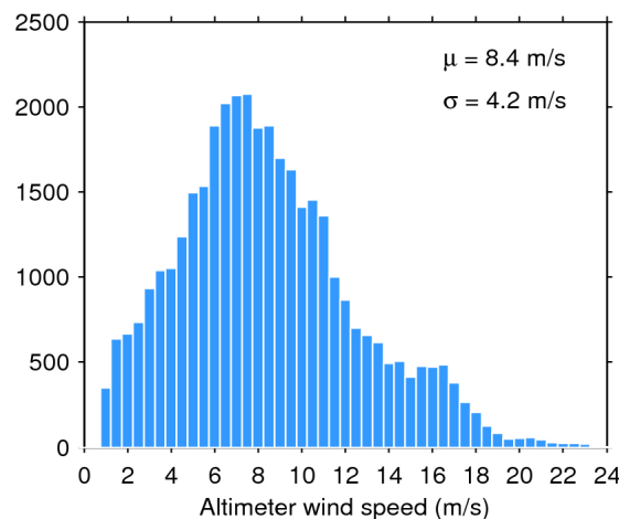
Figure 35. Histogram of science-valid wind over oceans and lakes for 29/09/2019. The mean ( \mu ) and standard deviation ( \sigma ) are also shown. Note that values larger than 24 m/s are excluded from the histogram for the sake of readability but not from the computation of \mu and \sigma .
