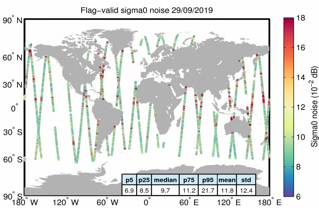
Figure 26. Geographical distribution of flag-valid 20-Hz sigma0 measurement noise over oceans and lakes for 29/09/2019. The statistical values shown in the table refer to the sigma0 noise and are calculated over all measurements shown in the figure.
