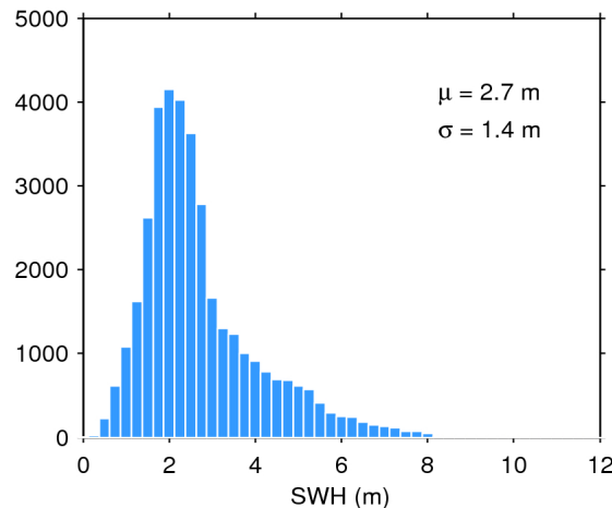
Figure 20. Histogram of science-valid SWH over oceans and lakes for 29/09/2019. The mean ( \mu ) and standard deviation ( \sigma ) are also shown. Note that values larger than 12 m are excluded from the histogram for the sake of readability but not from the computation of \mu and \sigma .
