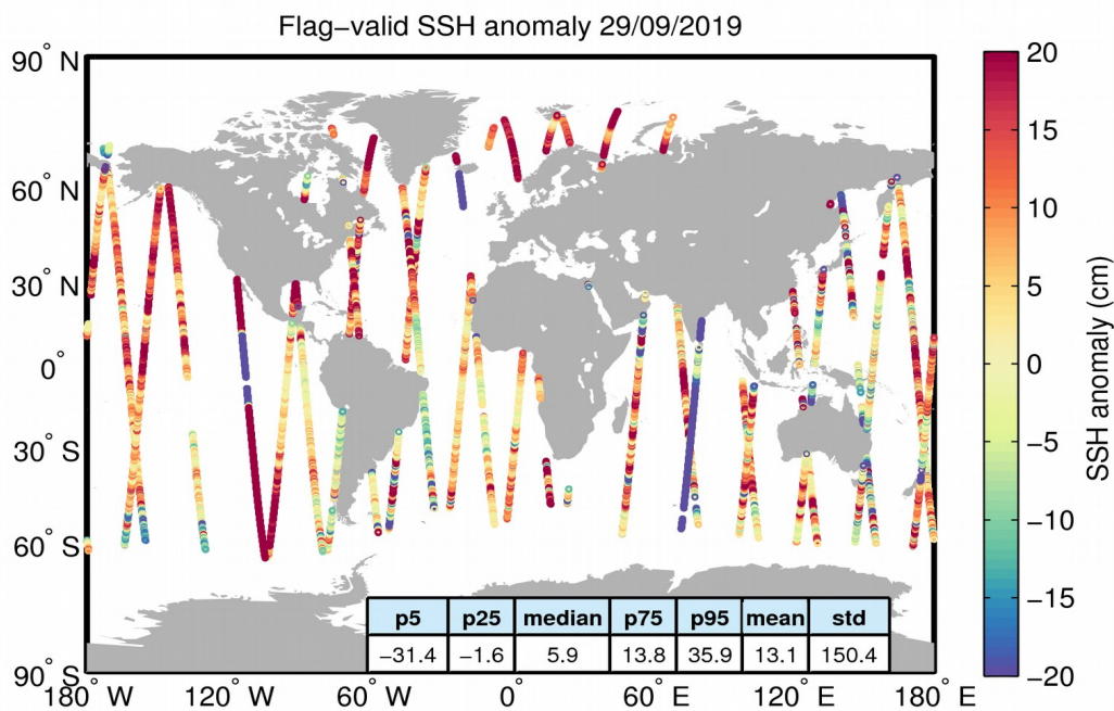
Figure 5. Geographical distribution of flag-valid 1-Hz SSH anomaly data over oceans and lakes for 29/09/2019. The statistical values shown in the table refer to the SSH anomaly in cm and are calculated over all measurements shown in the figure.
