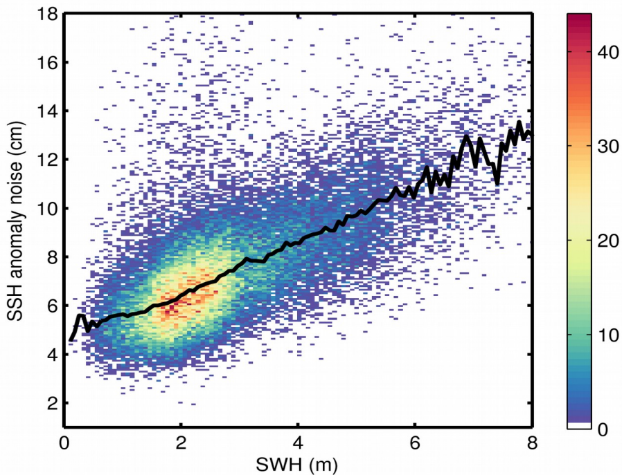
Figure 9. 2D histogram showing flag-valid SSH anomaly noise as a function of SWH for 29/09/2019. The black line denotes the median SSH anomaly noise as a function of SWH.
