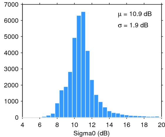
Figure 25. Histogram of flag-valid sigma0 over oceans and lakes for 29/09/2019. The mean ( \mu ) and standard deviation ( \sigma ) are also shown. Note that values outside [4 20] dB are excluded from the histogram for the sake of readability but not from the computation of \mu and \sigma .
