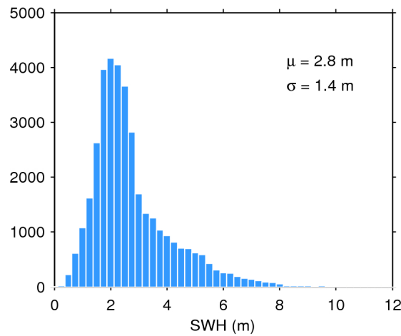
Figure 17. Histogram of flag-valid SWH over oceans and lakes for 29/09/2019. The mean ( \mu ) and standard deviation ( \sigma ) are also shown. Note that values larger than 12 m are excluded from the histogram for the sake of readability but not from the computation of \mu and \sigma .
