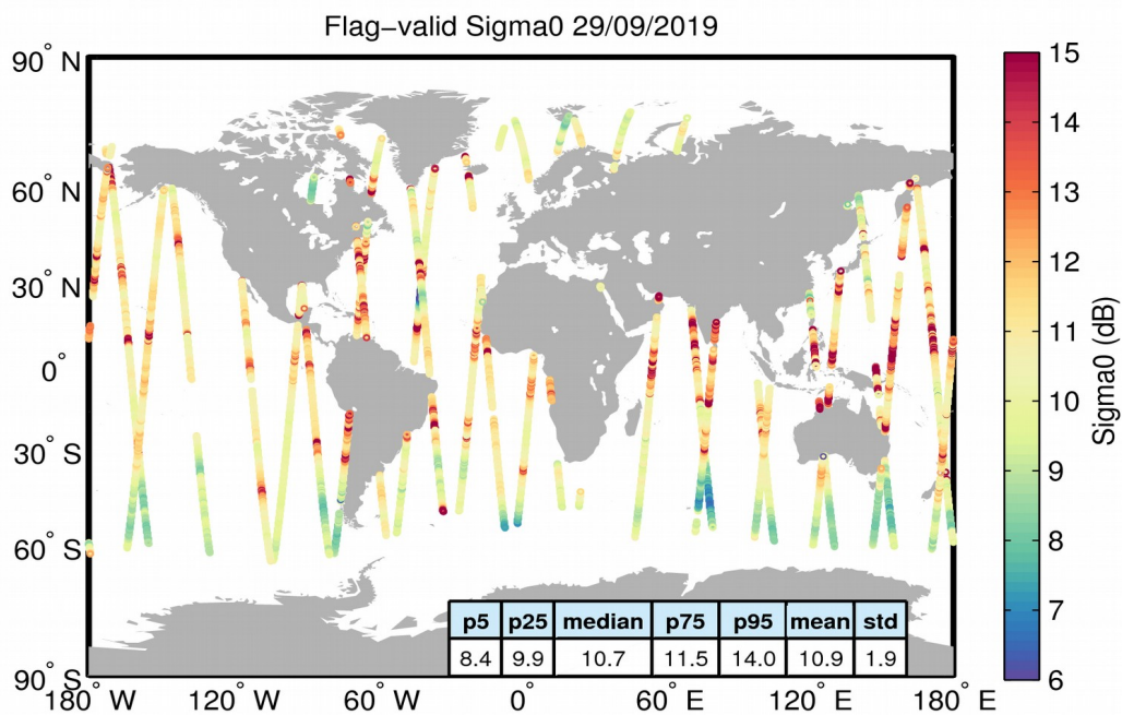
Figure 23. Geographical distribution of flag-valid sigma0 data over oceans and lakes for 29/09/2019. The statistical values shown in the table refer to the sigma0 in dB and are calculated over all measurements shown in the figure.
