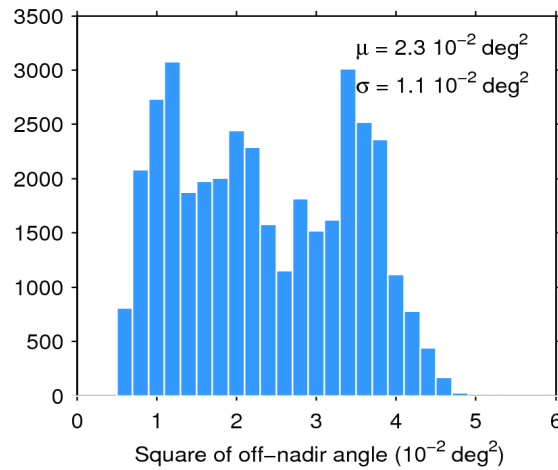
Figure 39. Histogram of flag-valid mispointing over oceans and lakes for 29/09/2019. The mean ( \mu ) and standard deviation ( \sigma ) are also shown. Note that values larger than 6 \cdot 10^{-2} \text{ deg}^2 are excluded from the histogram for the sake of readability but not from the computation of \mu and \sigma .
