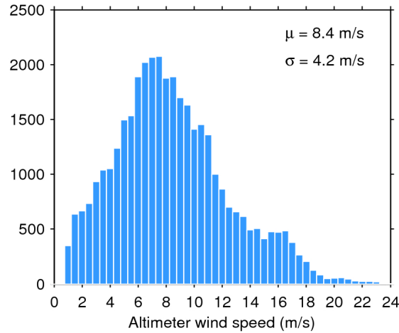
Figure 33. Histogram of flag-valid wind over oceans and lakes for 29/09/2019. The mean ( \mu ) and standard deviation ( \sigma ) are also shown. Note that values larger than 24 m/s are excluded from the histogram for the sake of readability but not from the computation of \mu and \sigma .
