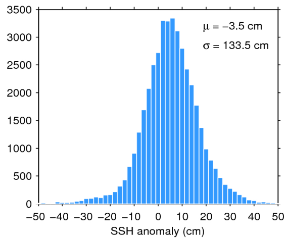
Figure 7. Histogram of flag-valid SSH anomaly over oceans and lakes for 28/09/2019. The mean ( \mu ) and standard deviation ( \sigma ) are also shown. Note that values outside [-50 50] cm are excluded from the histogram for the sake of readability but not from the computation of \mu and \sigma .
