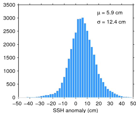
Figure 11. Histogram of science-valid SSH anomaly over oceans and lakes for 28/09/2019. The mean ( \mu ) and standard deviation ( \sigma ) are also shown. Note that values outside [-50 50] cm are excluded from the histogram for the sake of readability but not from the computation of \mu and \sigma .
