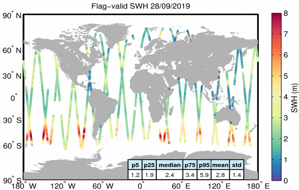
Figure 15. Geographical distribution of flag-valid SWH data over oceans and lakes for 28/09/2019. The statistical values shown in the table refer to the SWH in m and are calculated over all measurements shown in the figure.
