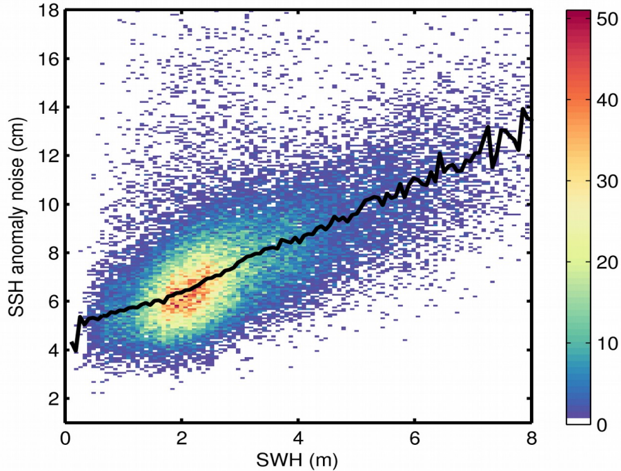
Figure 9. 2D histogram showing flag-valid SSH anomaly noise as a function of SWH for 28/09/2019. The black line denotes the median SSH anomaly noise as a function of SWH.
