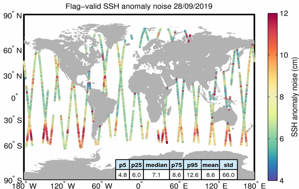
Figure 8. Geographical distribution of flag-valid 20-Hz SSH anomaly measurement noise over oceans and lakes for 28/09/2019. The statistical values shown in the table refer to the SSH anomaly noise and are calculated over all measurements shown in the figure.
