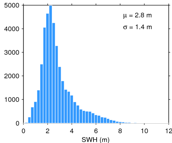
Figure 20. Histogram of science-valid SWH over oceans and lakes for 28/09/2019. The mean ( \mu ) and standard deviation ( \sigma ) are also shown. Note that values larger than 12 m are excluded from the histogram for the sake of readability but not from the computation of \mu and \sigma .
