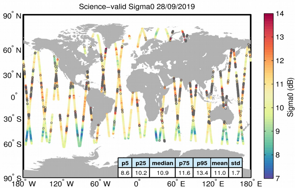
Figure 27. Geographical distribution of science-valid sigma0 data over oceans and lakes for 28/09/2019. The statistical values shown in the table refer to the sigma0 in dB and are calculated over all measurements shown in the figure. Gray circles denote records that have been rejected based on the editing criteria described in Table 4.
