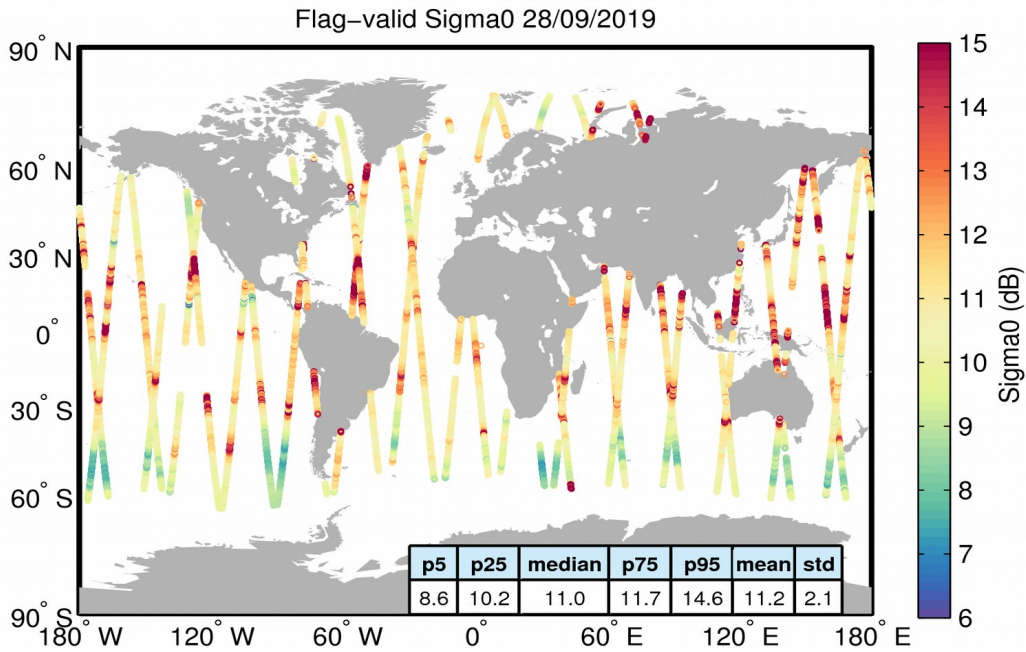
Figure 23. Geographical distribution of flag-valid sigma0 data over oceans and lakes for 28/09/2019. The statistical values shown in the table refer to the sigma0 in dB and are calculated over all measurements shown in the figure.
