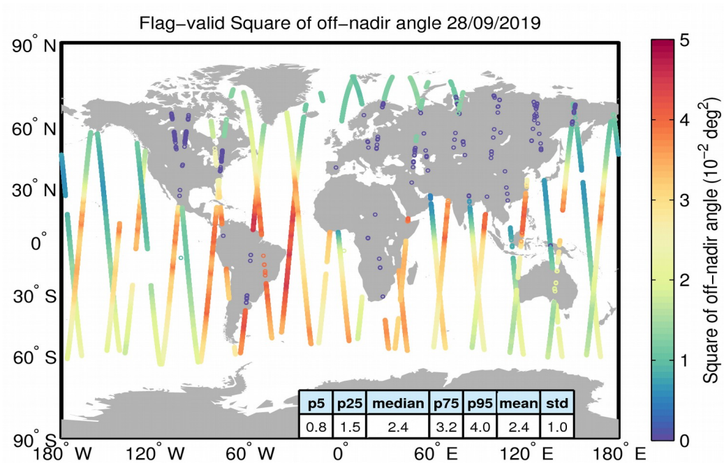
Figure 37. Geographical distribution of flag-valid mispointing data over oceans and lakes for 28/09/2019. The statistical values shown in the table refer to the mispointing in 10^{-2} deg 2 and are calculated over all measurements shown in the figure.
