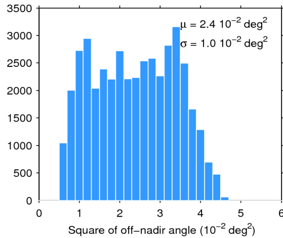
Figure 39. Histogram of flag-valid mispointing over oceans and lakes for 28/09/2019. The mean ( \mu ) and standard deviation ( \sigma ) are also shown. Note that values larger than 6 \cdot 10^{-2} \text{ deg}^2 are excluded from the histogram for the sake of readability but not from the computation of \mu and \sigma .
