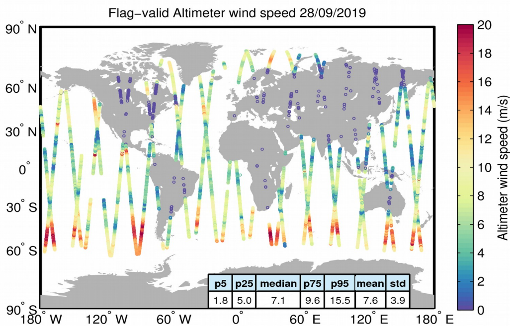
Figure 31. Geographical distribution of flag-valid wind data over oceans and lakes for 28/09/2019. The statistical values shown in the table refer to the wind in m/s and are calculated over all measurements shown in the figure.
