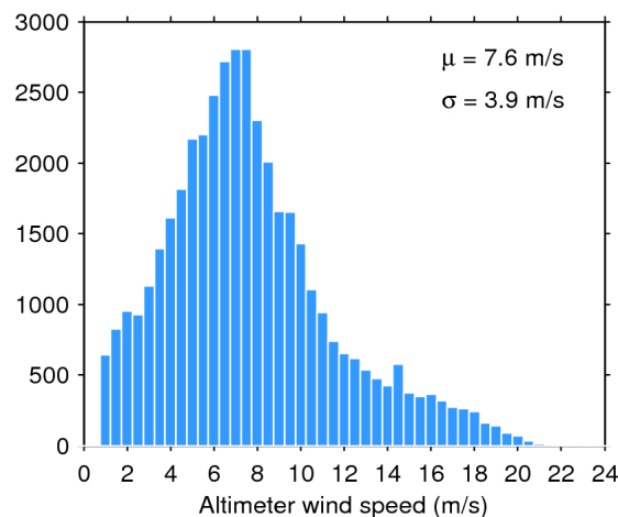
Figure 35. Histogram of science-valid wind over oceans and lakes for 28/09/2019. The mean ( \mu ) and standard deviation ( \sigma ) are also shown. Note that values larger than 24 m/s are excluded from the histogram for the sake of readability but not from the computation of \mu and \sigma .
