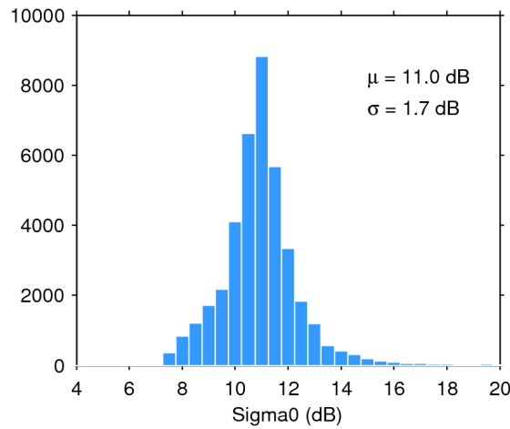
Figure 28. Histogram of science-valid sigma0 over oceans and lakes for 28/09/2019. The mean ( \mu ) and standard deviation ( \sigma ) are also shown. Note that values outside [4 20] dB are excluded from the histogram for the sake of readability but not from the computation of \mu and \sigma .
