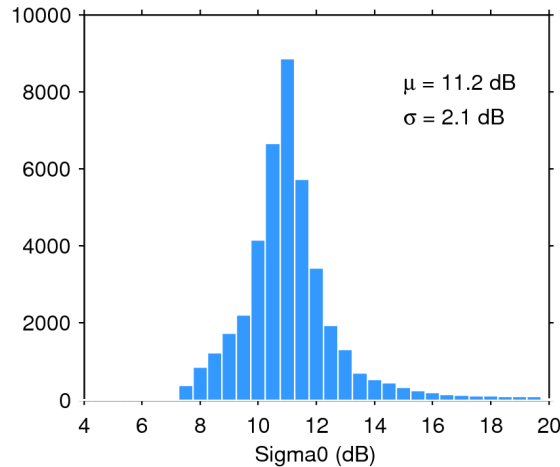
Figure 25. Histogram of flag-valid sigma0 over oceans and lakes for 28/09/2019. The mean ( \mu ) and standard deviation ( \sigma ) are also shown. Note that values outside [4 20] dB are excluded from the histogram for the sake of readability but not from the computation of \mu and \sigma .
