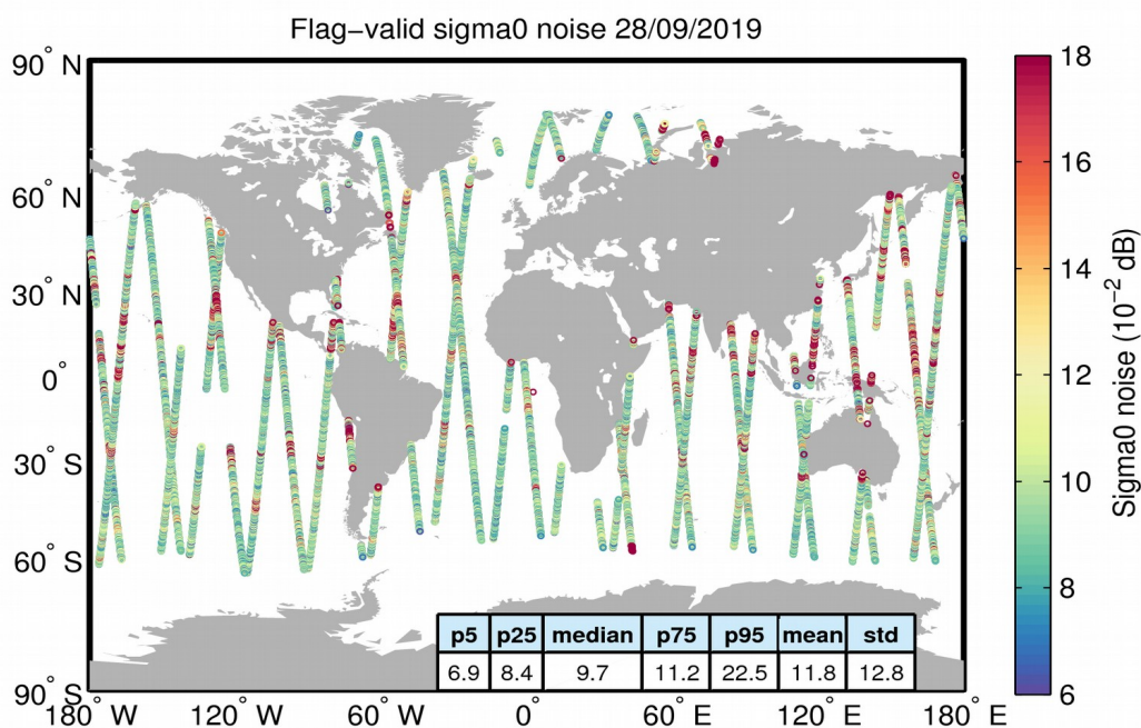
Figure 26. Geographical distribution of flag-valid 20-Hz sigma0 measurement noise over oceans and lakes for 28/09/2019. The statistical values shown in the table refer to the sigma0 noise and are calculated over all measurements shown in the figure.
