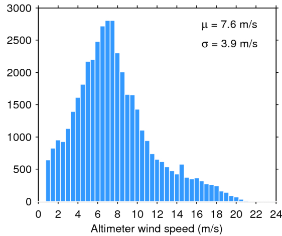
Figure 33. Histogram of flag-valid wind over oceans and lakes for 28/09/2019. The mean ( \mu ) and standard deviation ( \sigma ) are also shown. Note that values larger than 24 m/s are excluded from the histogram for the sake of readability but not from the computation of \mu and \sigma .
